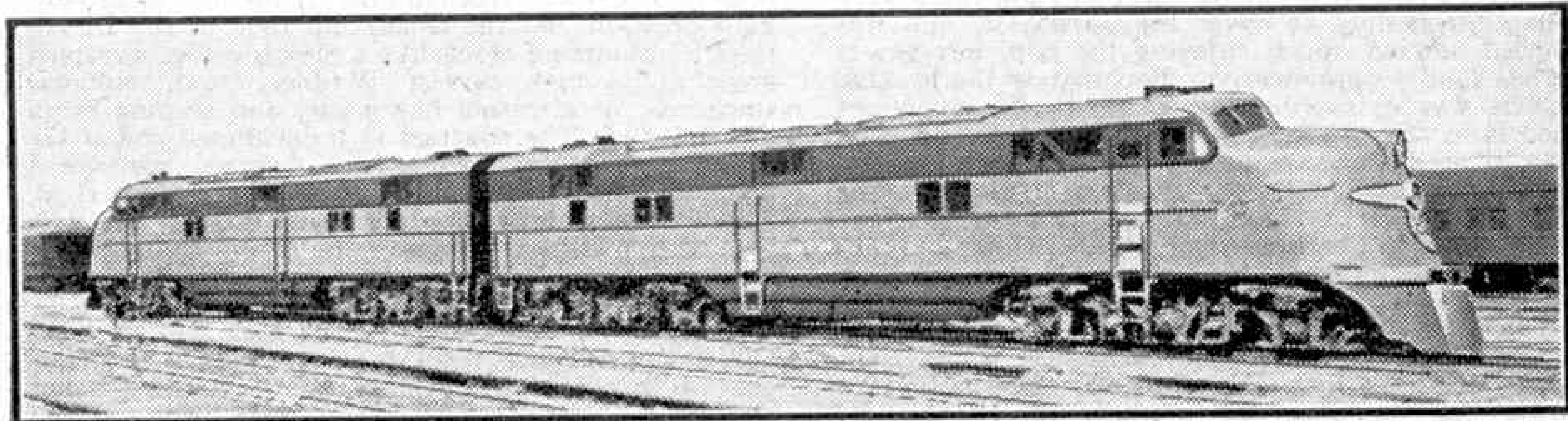
A 4,000 h.p. Diesel-electric locomotive of the C. and N.W.R. It is made up of two similar units, with a cab at each end, so that turntables are not required, and it houses eight traction motors.
