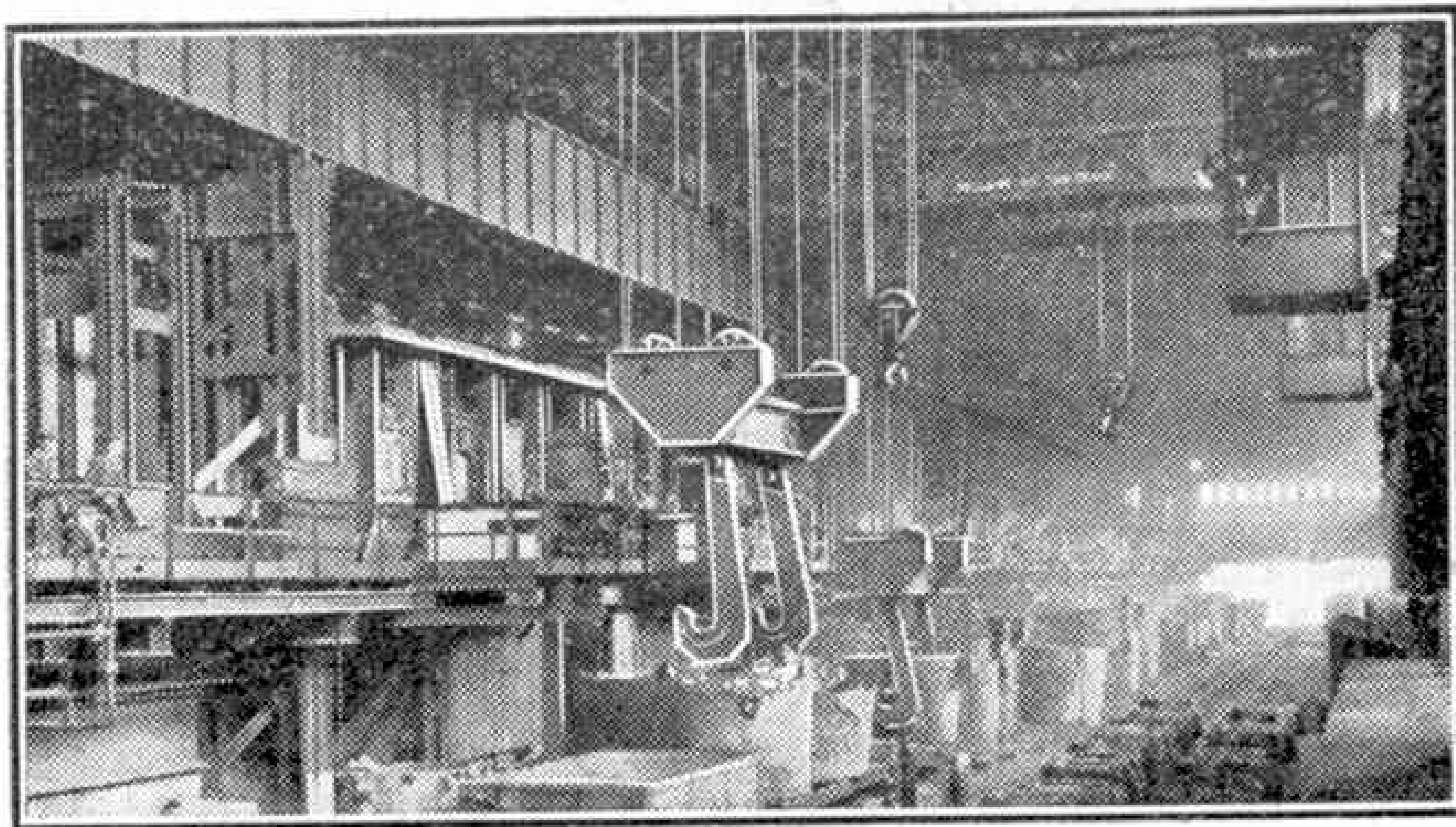
Fig. 4. Two 125-ton Ladle Cranes.
