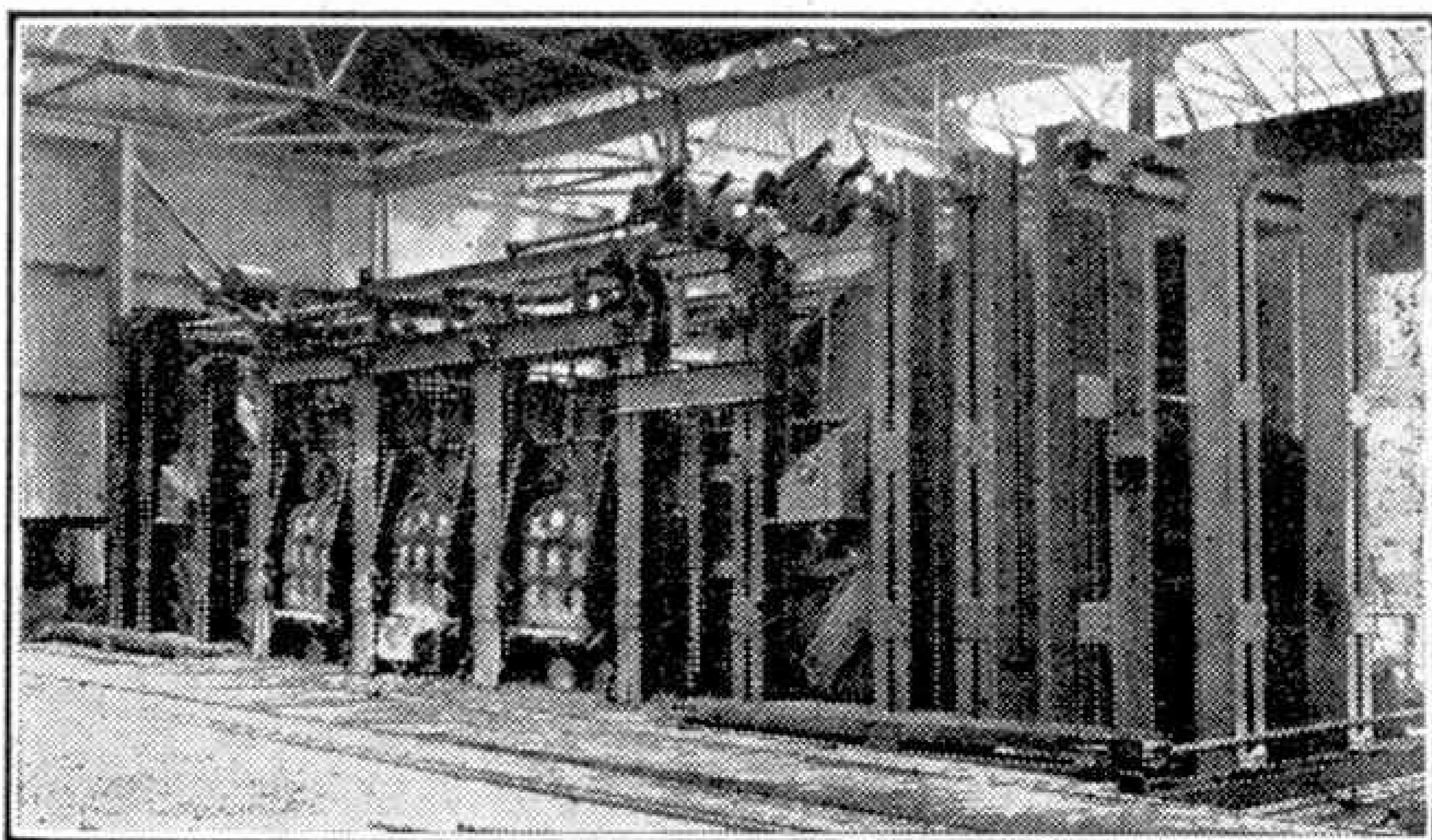
Fig. 1. Fixed Open Hearth Steel Furnace, view at charging side. Photographs by courtesy of The Wellman Smith Owen Engineering Corporation Ltd.
