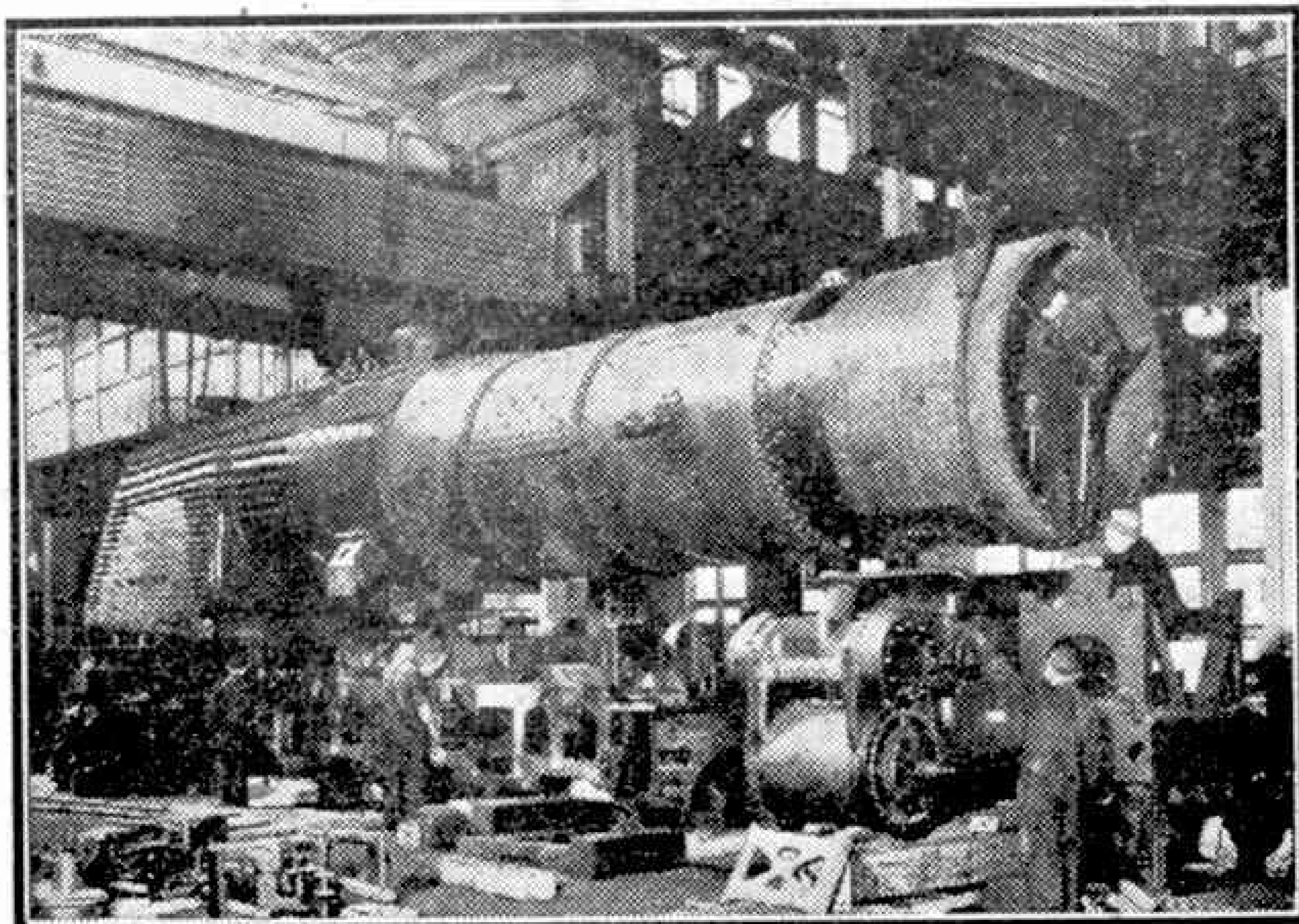
"Locomotive War Babies" (see page 336). Mounting the boiler on the new frame. Photograph by courtesy of Baltimore and Ohio Railroad, U.S.A.
