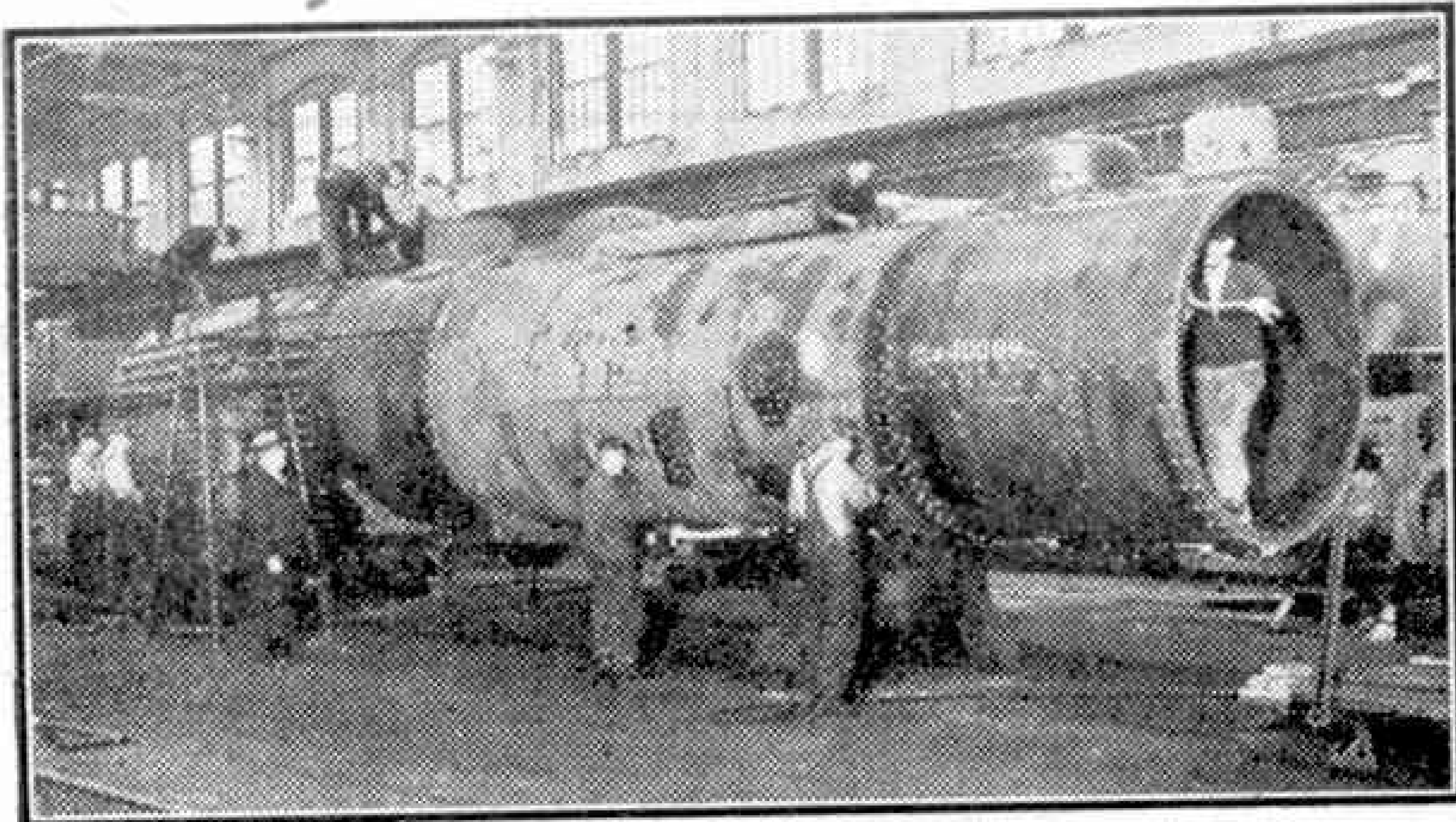
A section is added to lengthen the boiler.
