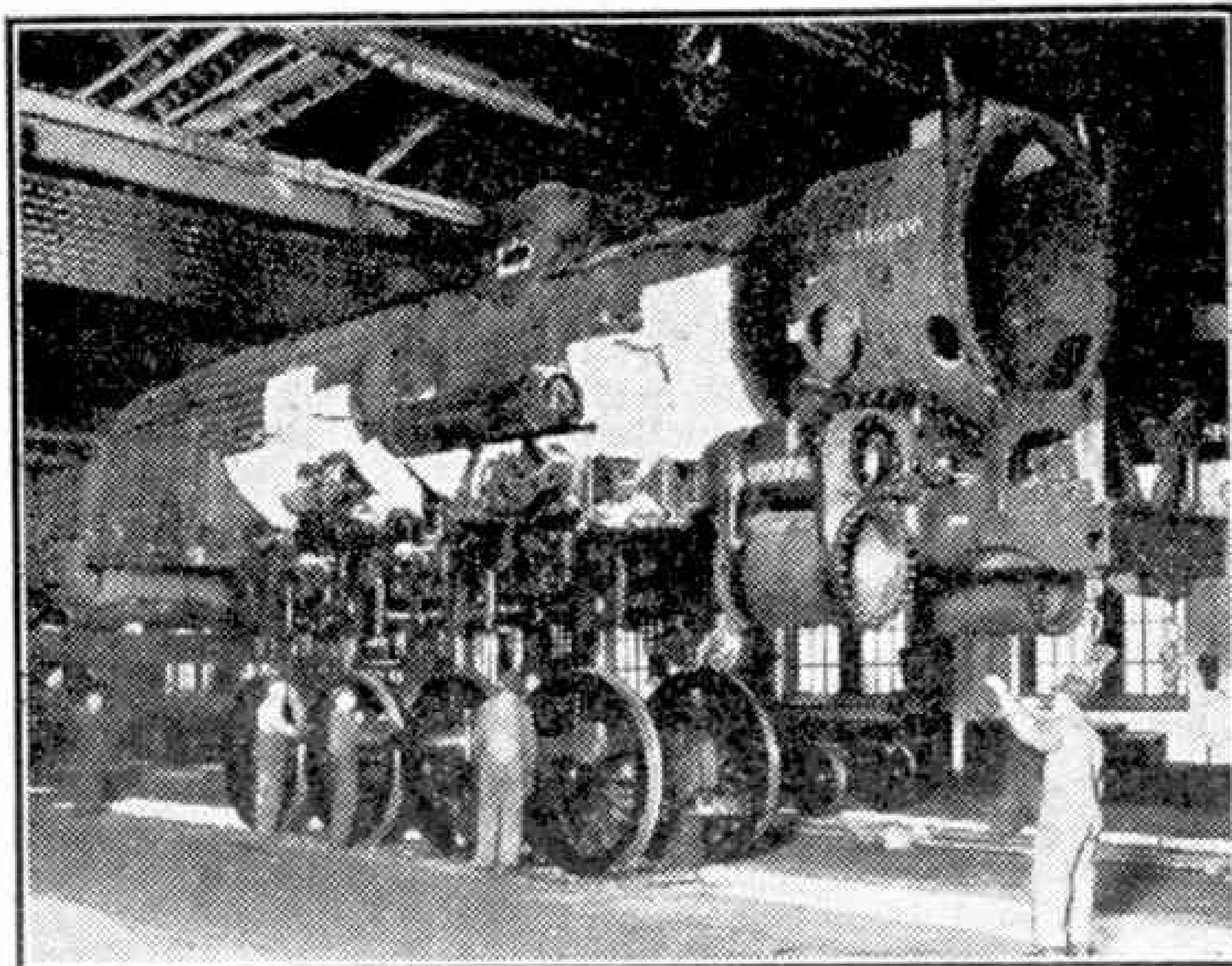
Boiler and frame being lowered on to the driving wheels.
