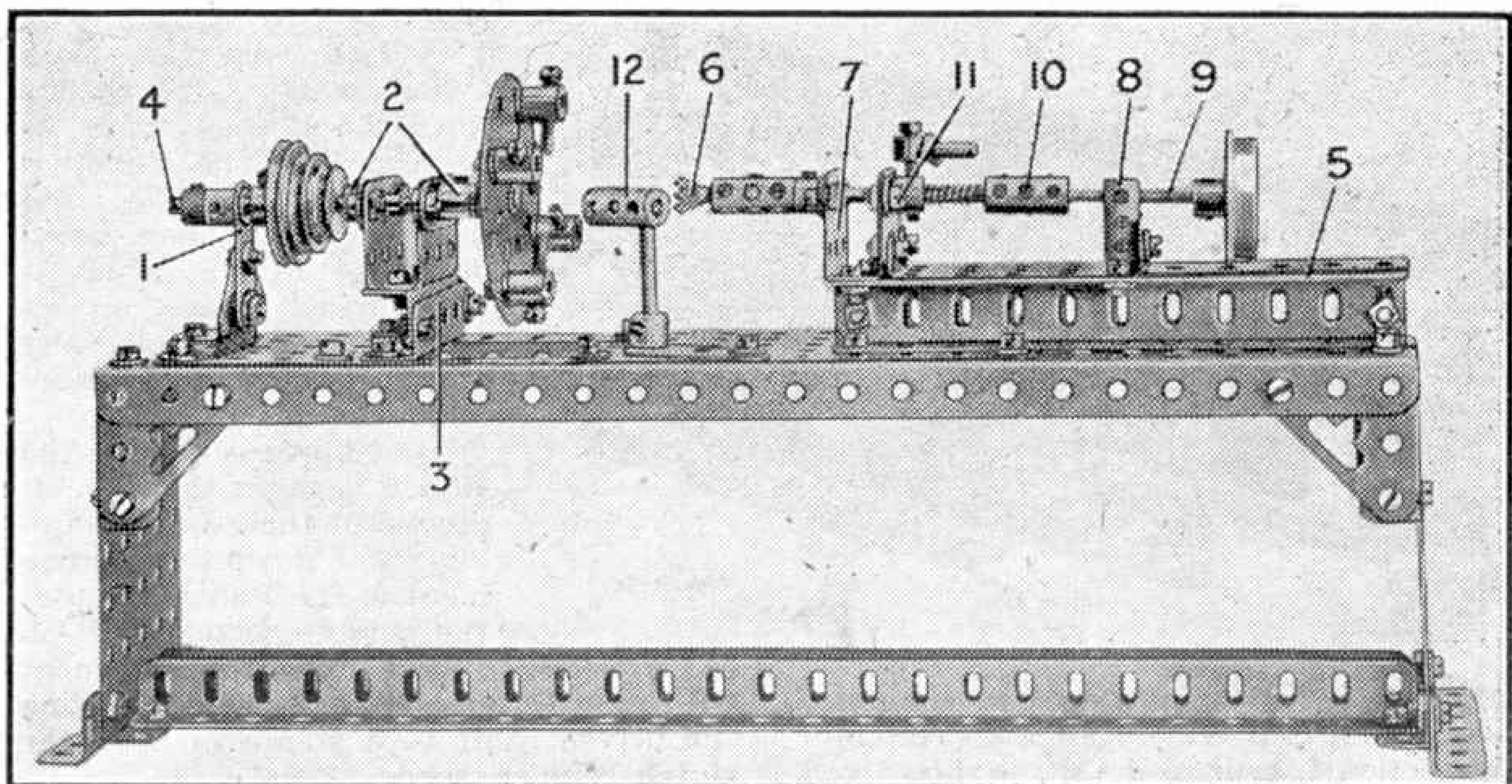
Fig. 1. A sturdily built Meccano lathe that can actually be used for turning small articles in wood or wax.
