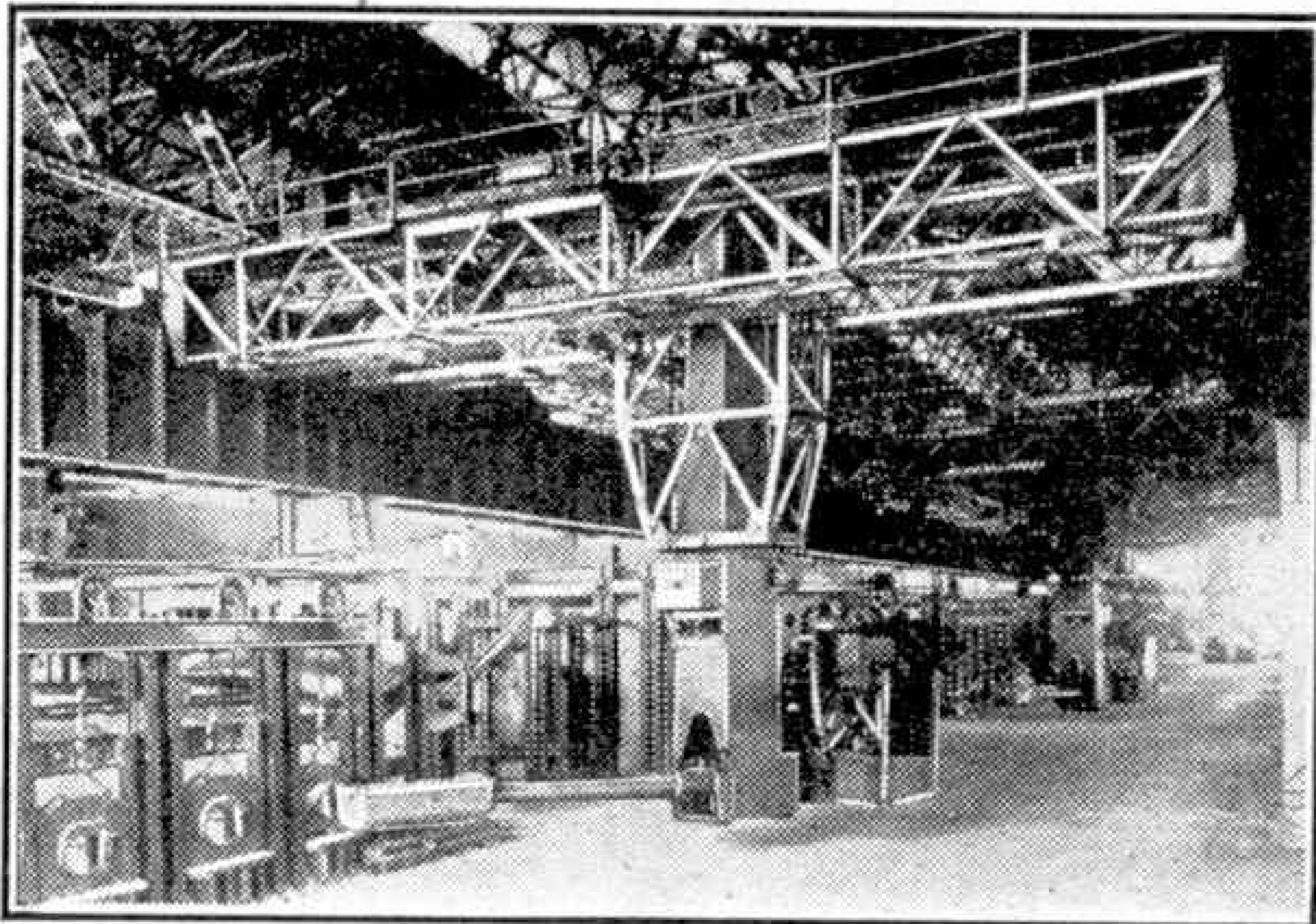
Fig. 2. Open Hearth Steel Plant equipped with three Wellman Chargers, each 3-tons capacity, serving a Battery of nine Wellman 70-ton Open Hearth Furnaces.
