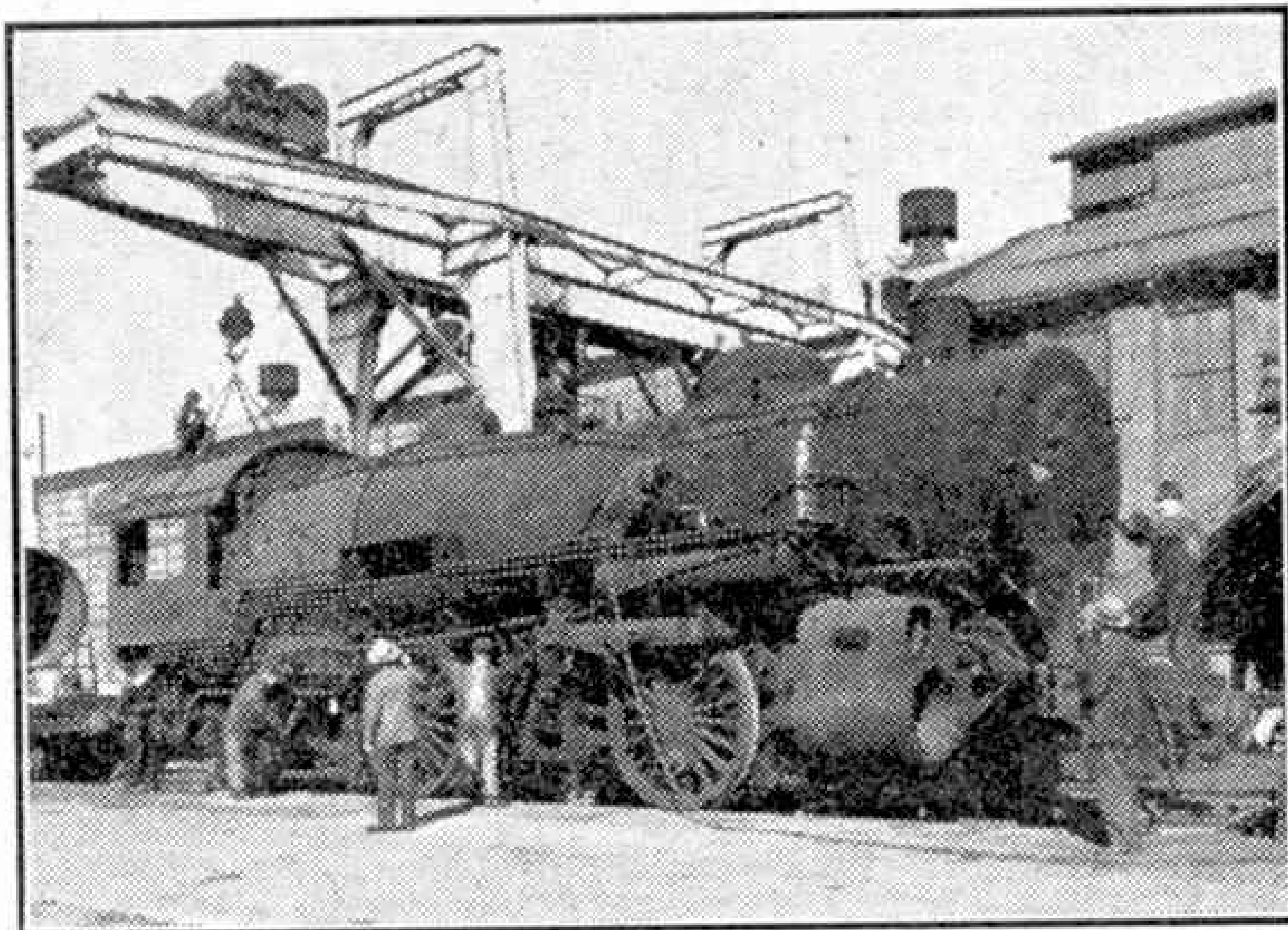
Dismantling a 2-8-2 engine prior to rebuilding it as a more powerful 4-8-2 "Mountain" type.
