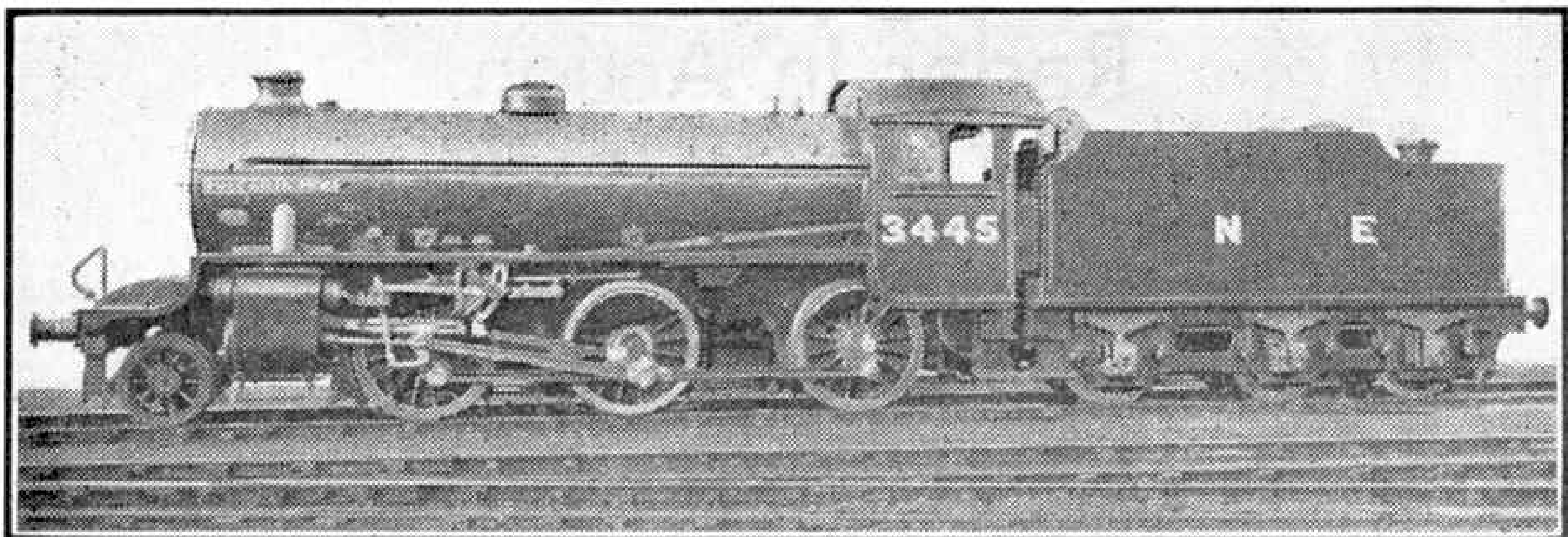
L.N.E.R. No. 3445 "Mac Cailin Mor," of the "K4" class, which has been converted to two-cylinder instead of three-cylinder propulsion, with a boiler at 225 lb. per sq. in. pressure and other changes. This engine will be the first of the new class "K1." Photograph by courtesy of the L.N.E.R.
