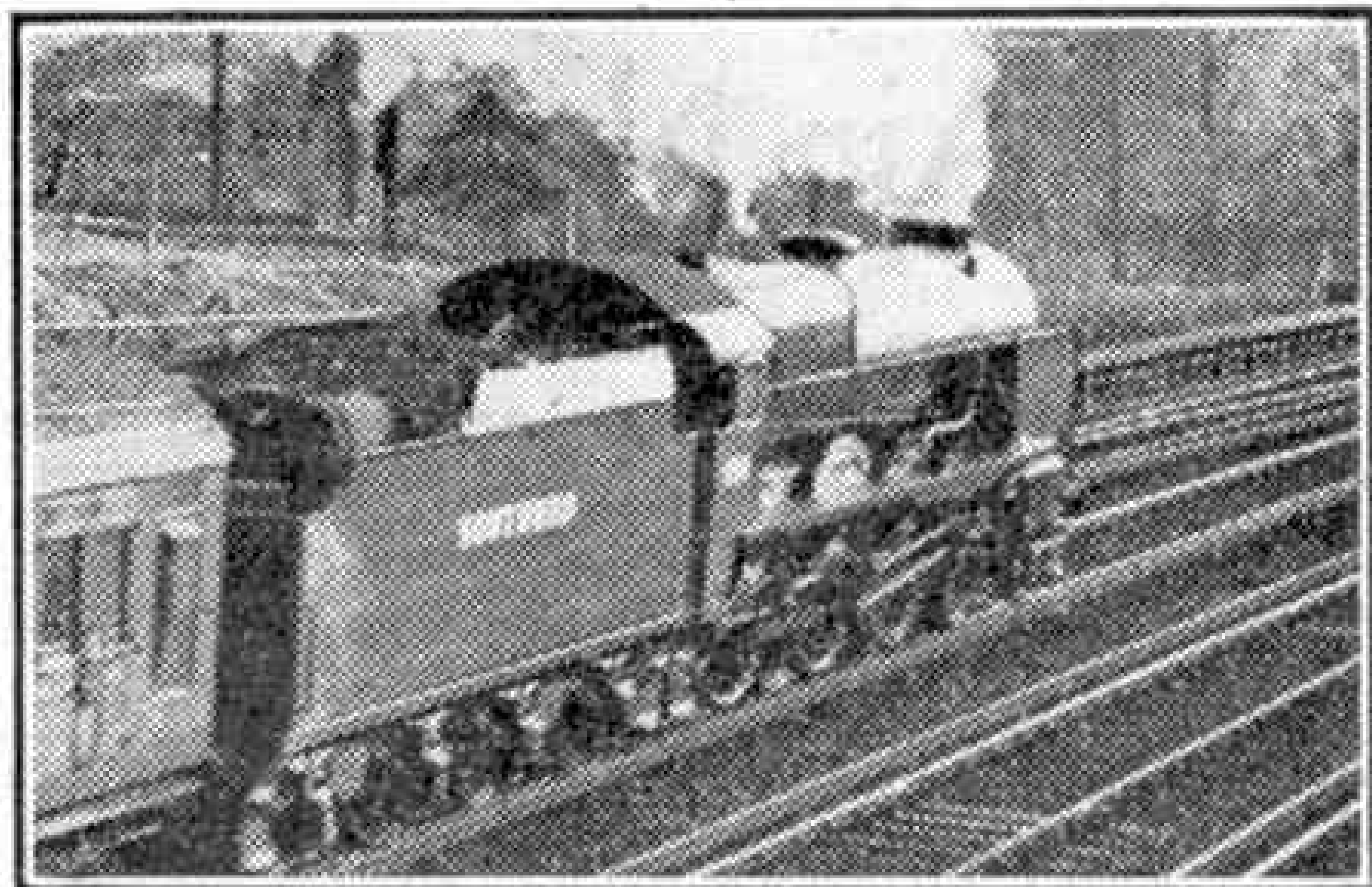
S.R. "Lord Nelson" class No. 864 accelerating after speed check. 40 m.p.h. Regulator full open and 30 per cent. cut-off.
