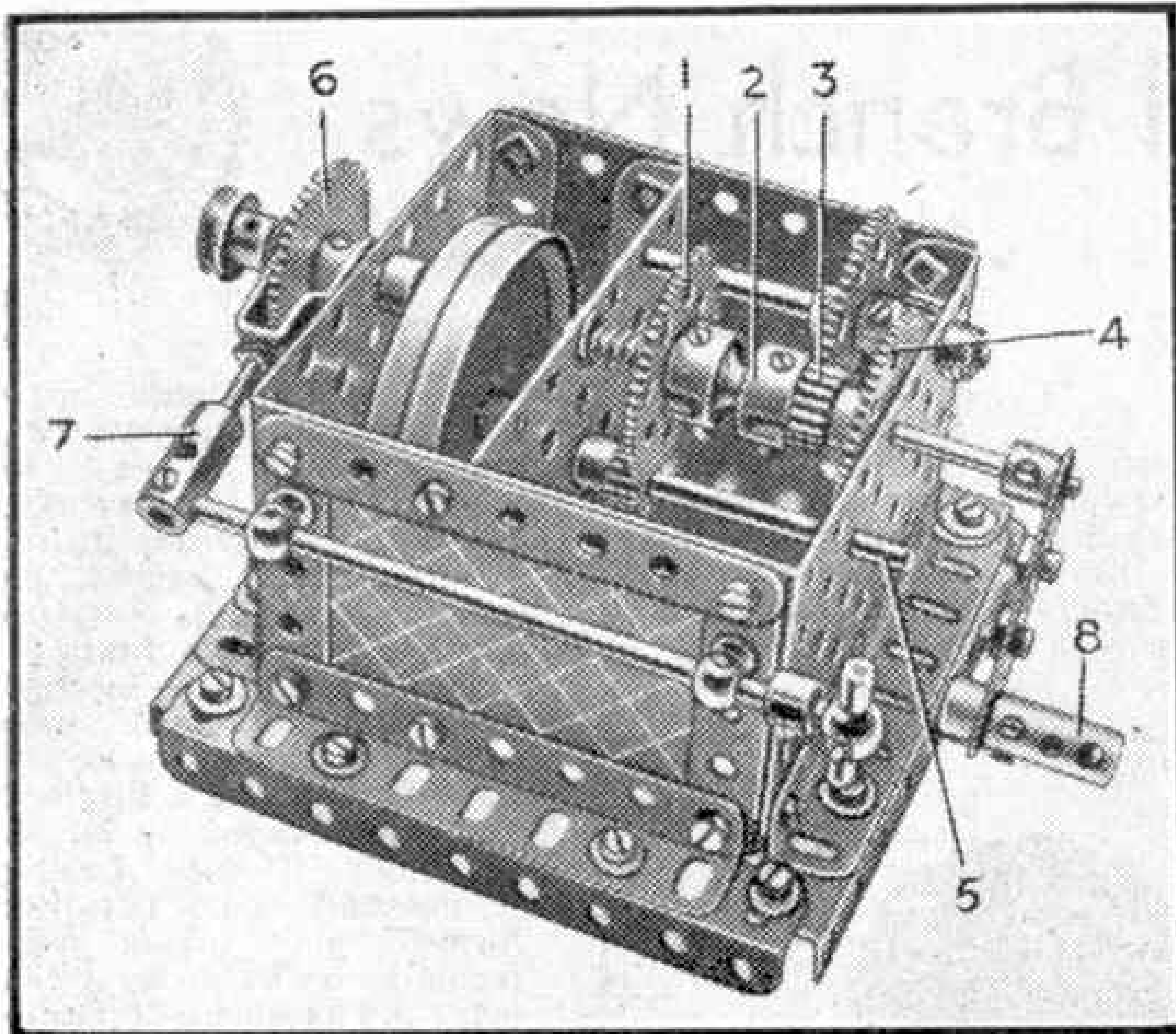
Fig. 3. A useful momentum motor.
