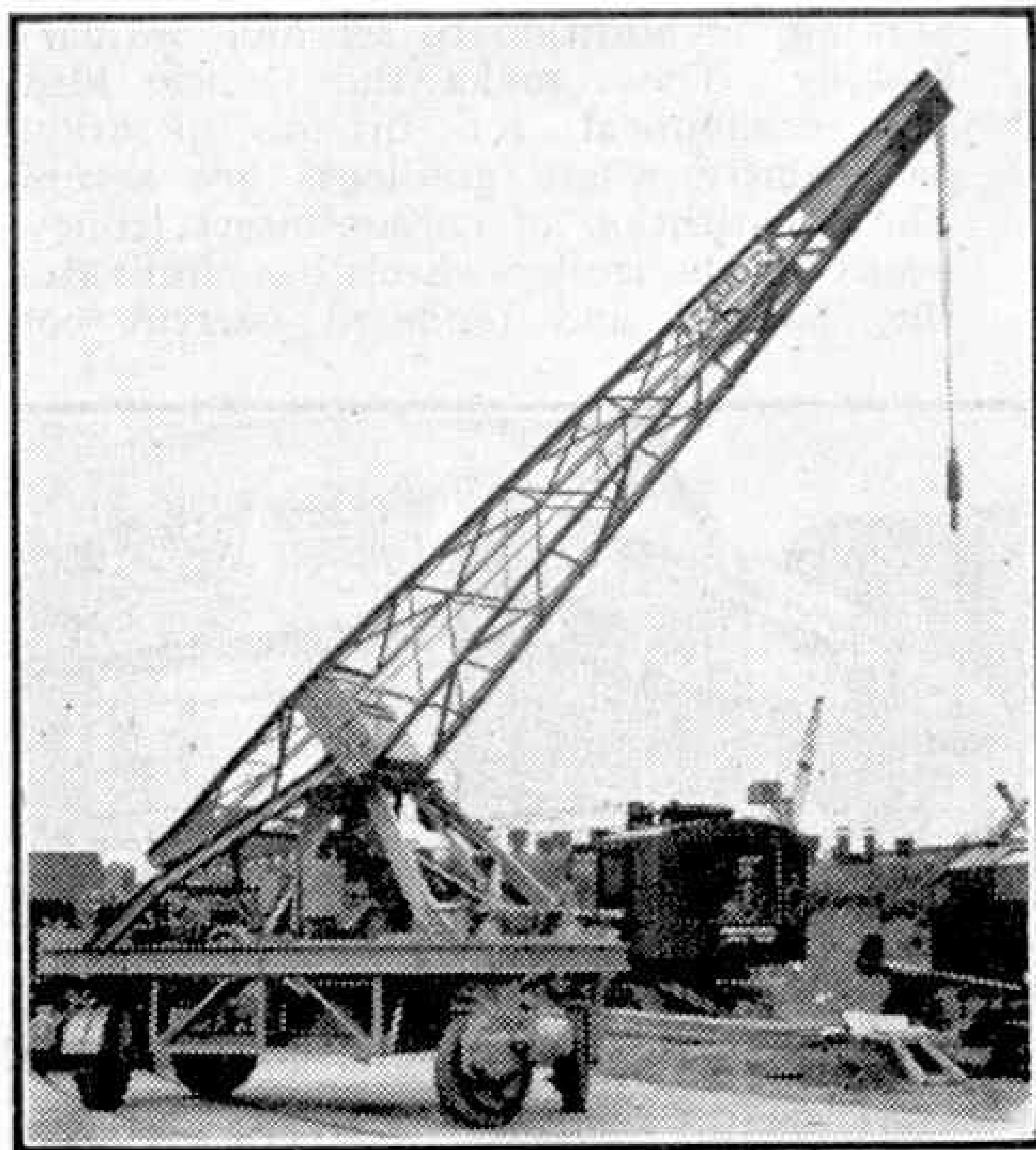
The "Centurn" Mobile Crane described on this page. We are indebted to Ransomes and Rapier Ltd., Ipswich, for our illustrations.
