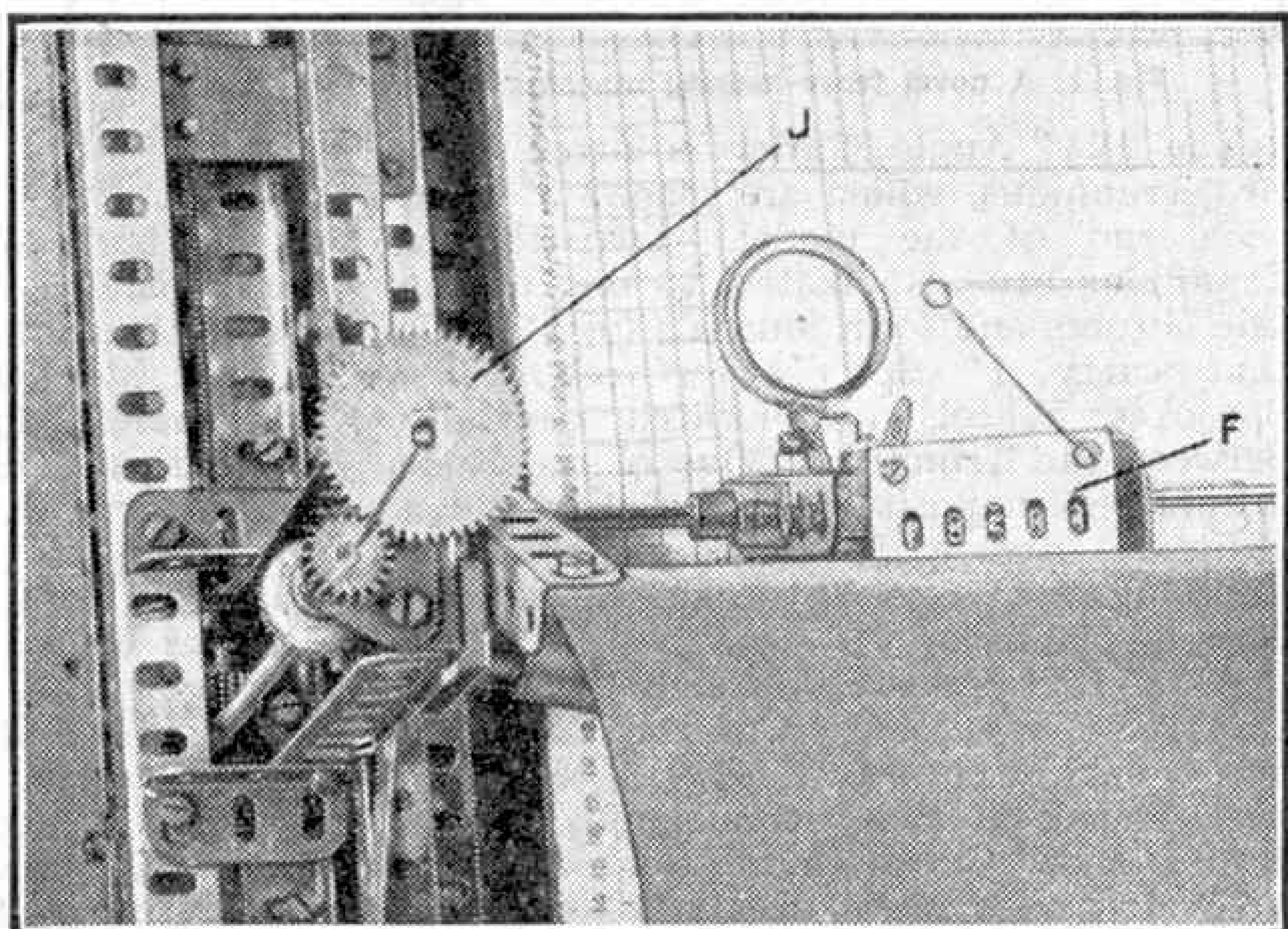
Fig. 4. A plan view of the tracing sight and unit counter. At the left can be seen the indicating dial J referred to in the accompanying article.
