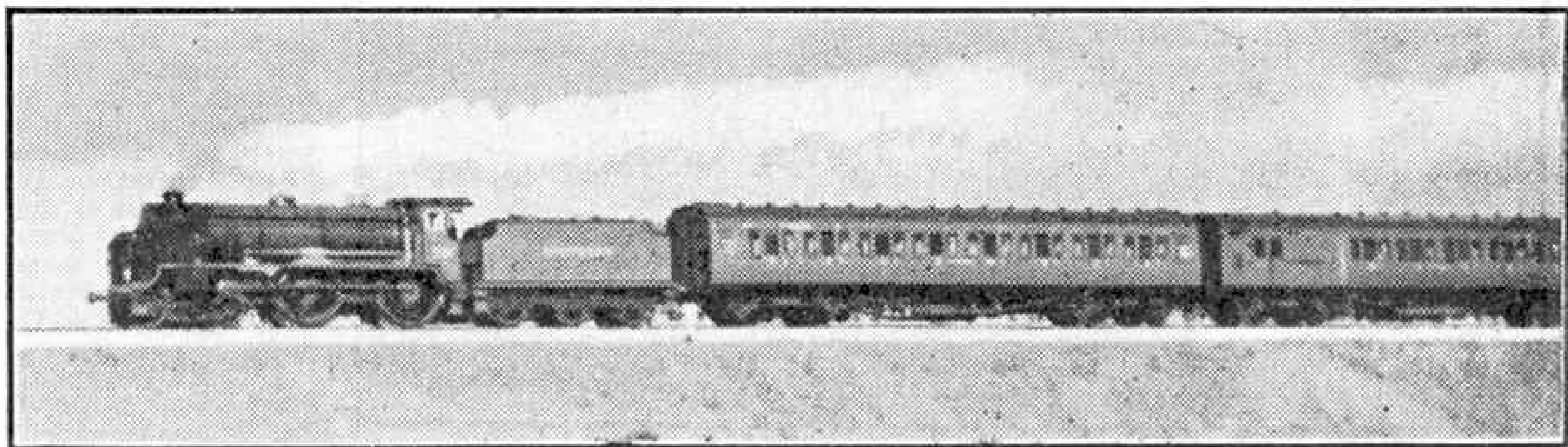
S.R. "Schools" class No. 928 running at 70 m.p.h. with regulator \frac{1}{2} -open and 15 per cent. cut-off.
