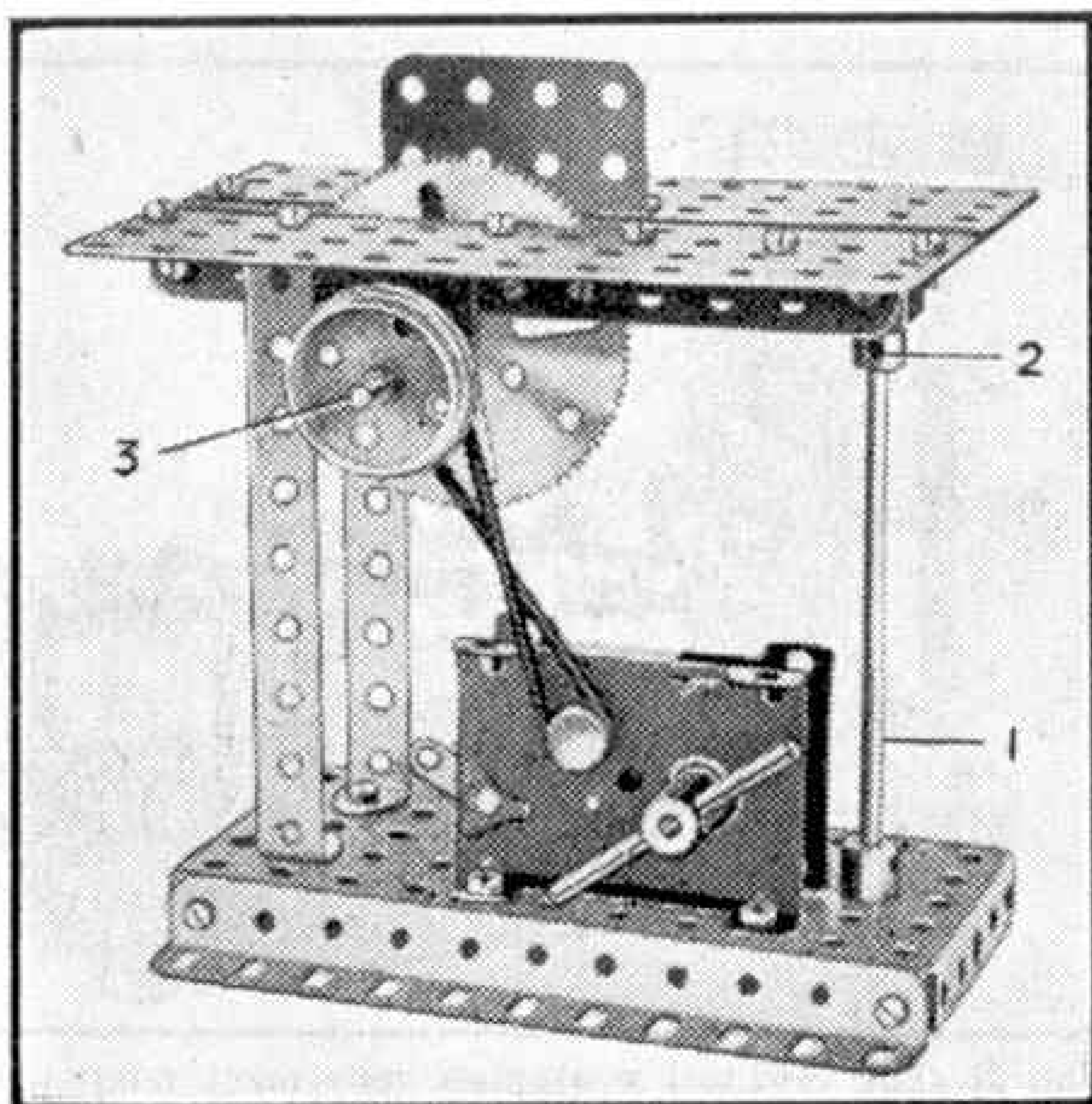
Fig. 4. An easily-built circular saw driven by a Magic Motor.
