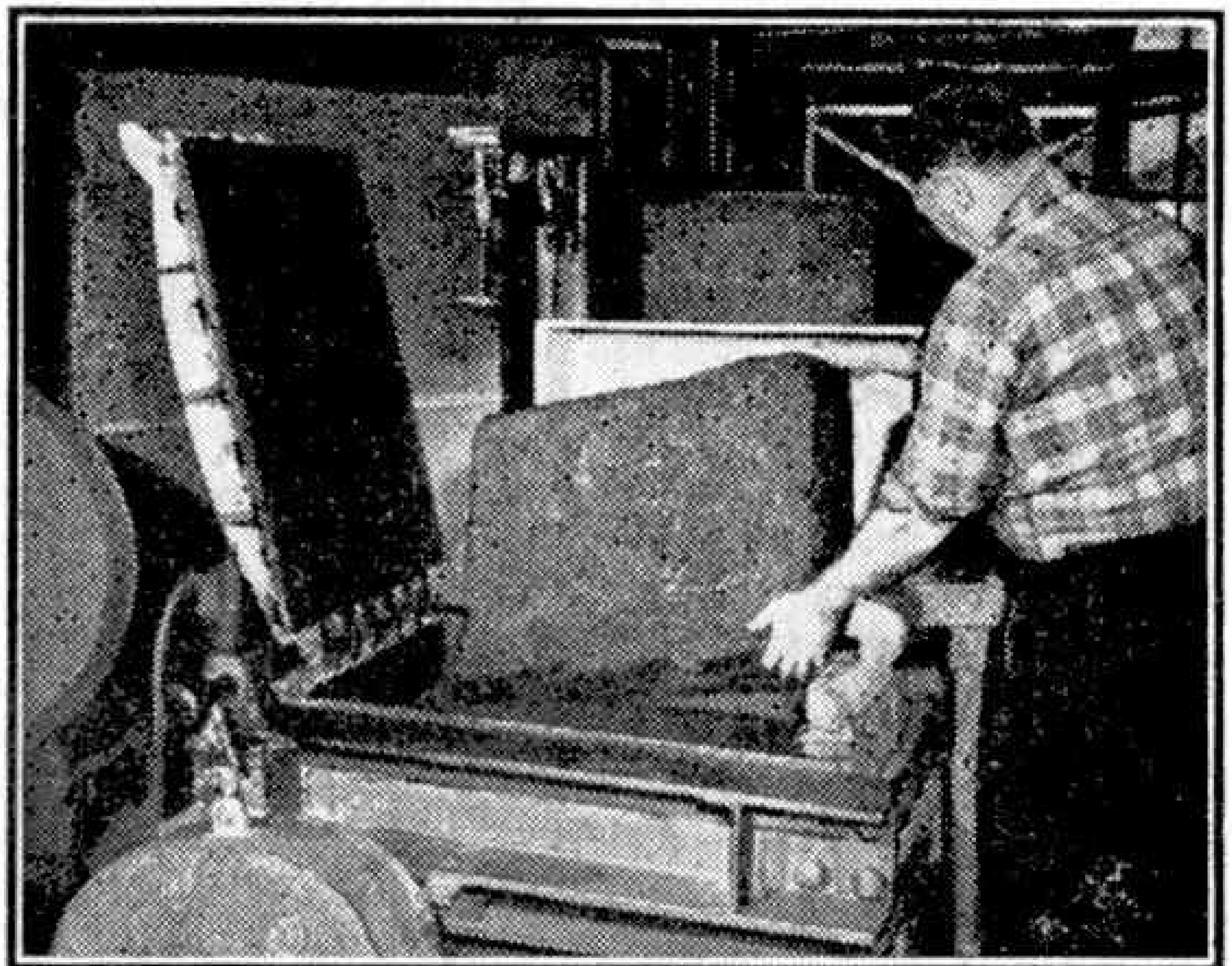
Guayule rubber pressed into 100 lb. slabs.
