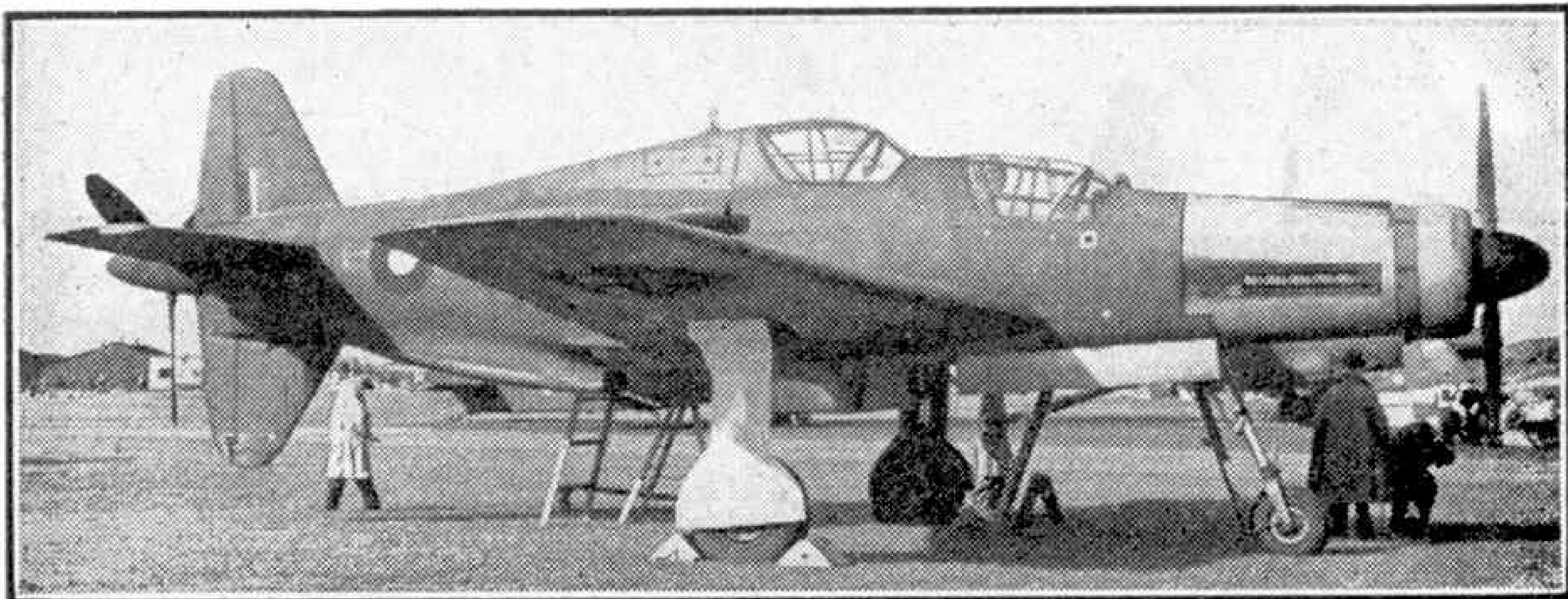
Dornier 335 fighter. This odd-looking machine has an engine at each end, and can be flown on either of them. Photograph "The Aeroplane" Copyright.
