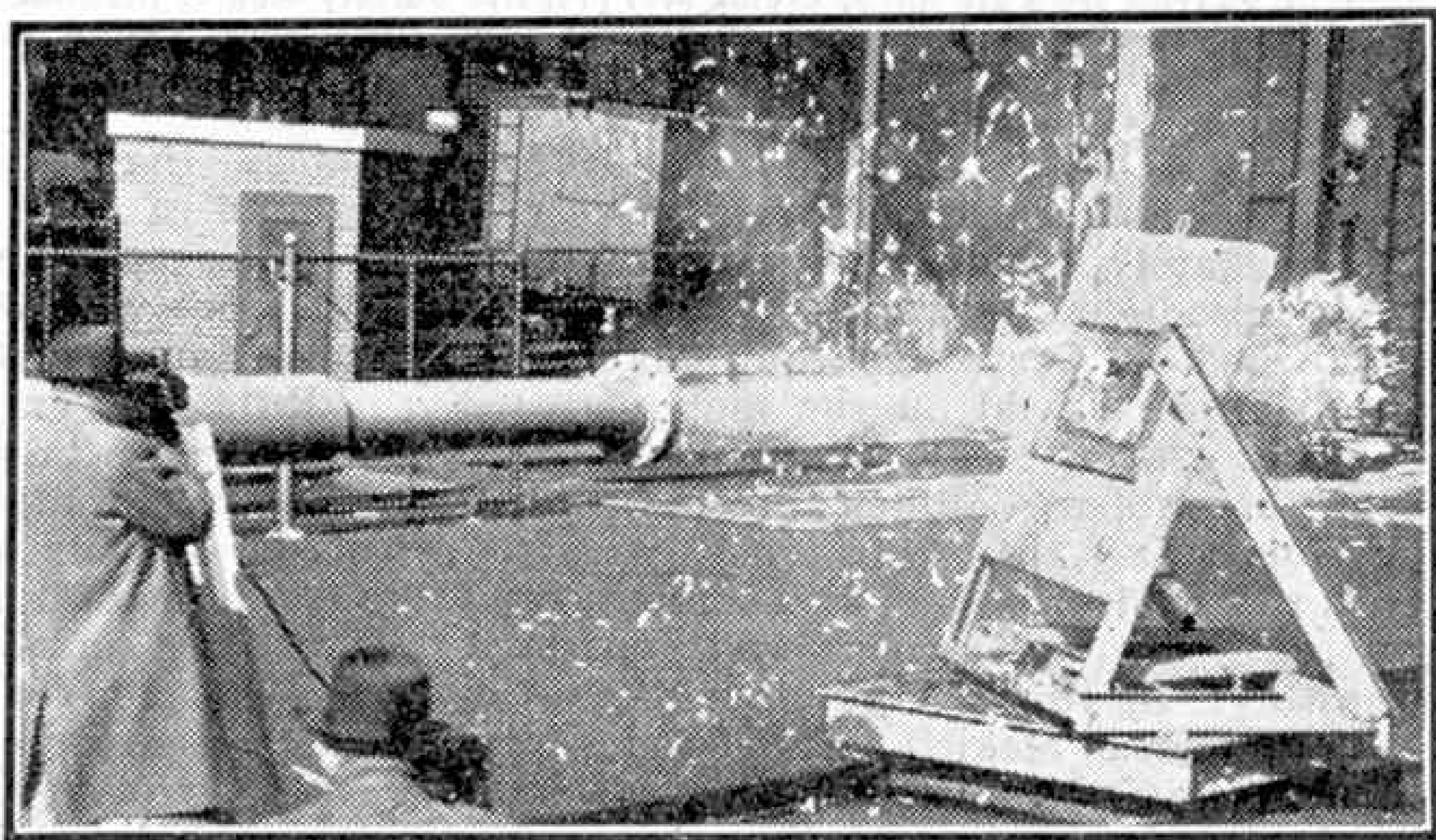
An aeroplane windshield fails during a test with a compressed air gun.
