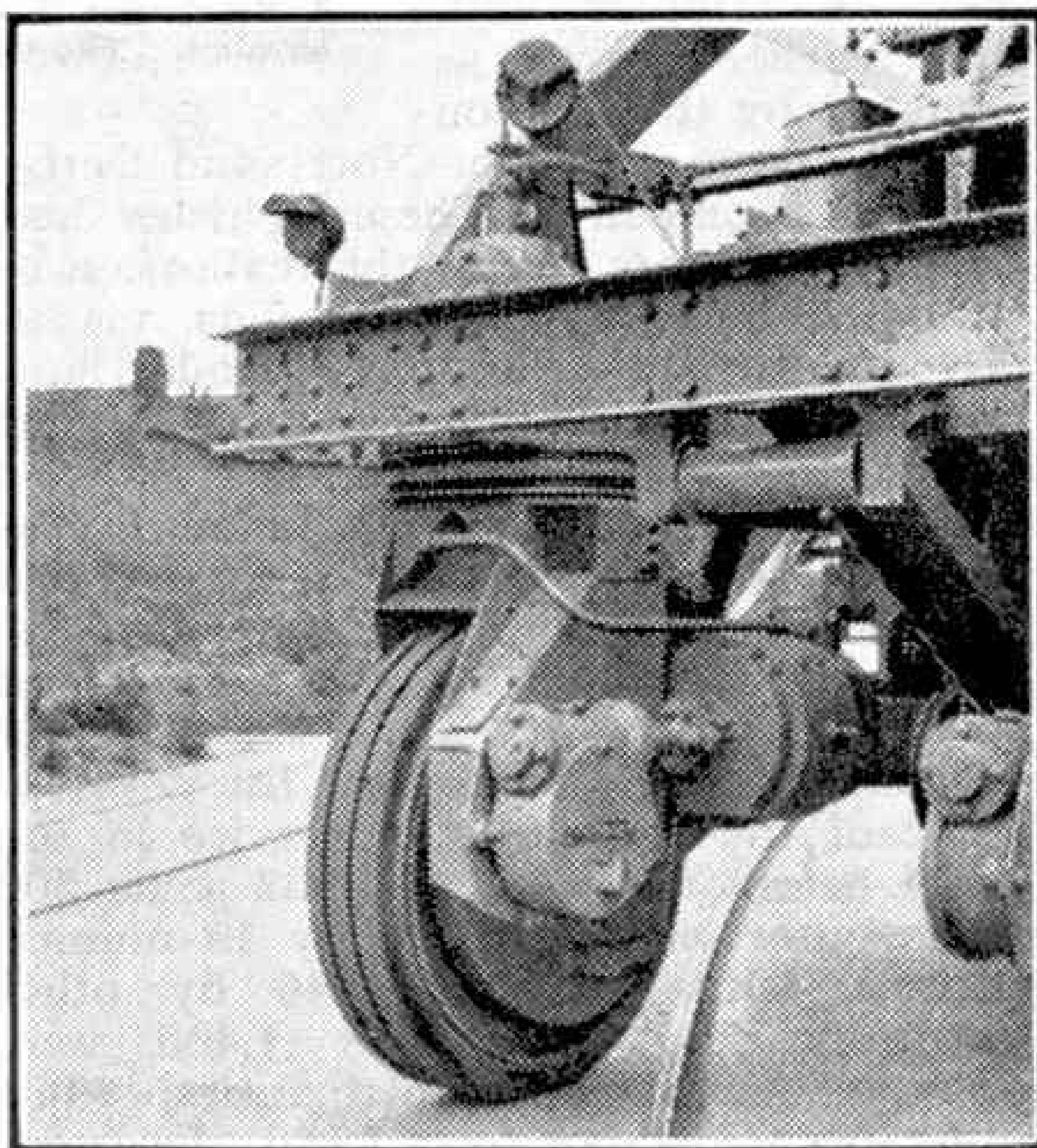
A close-up view of a castor of the "Centurn" Crane.
