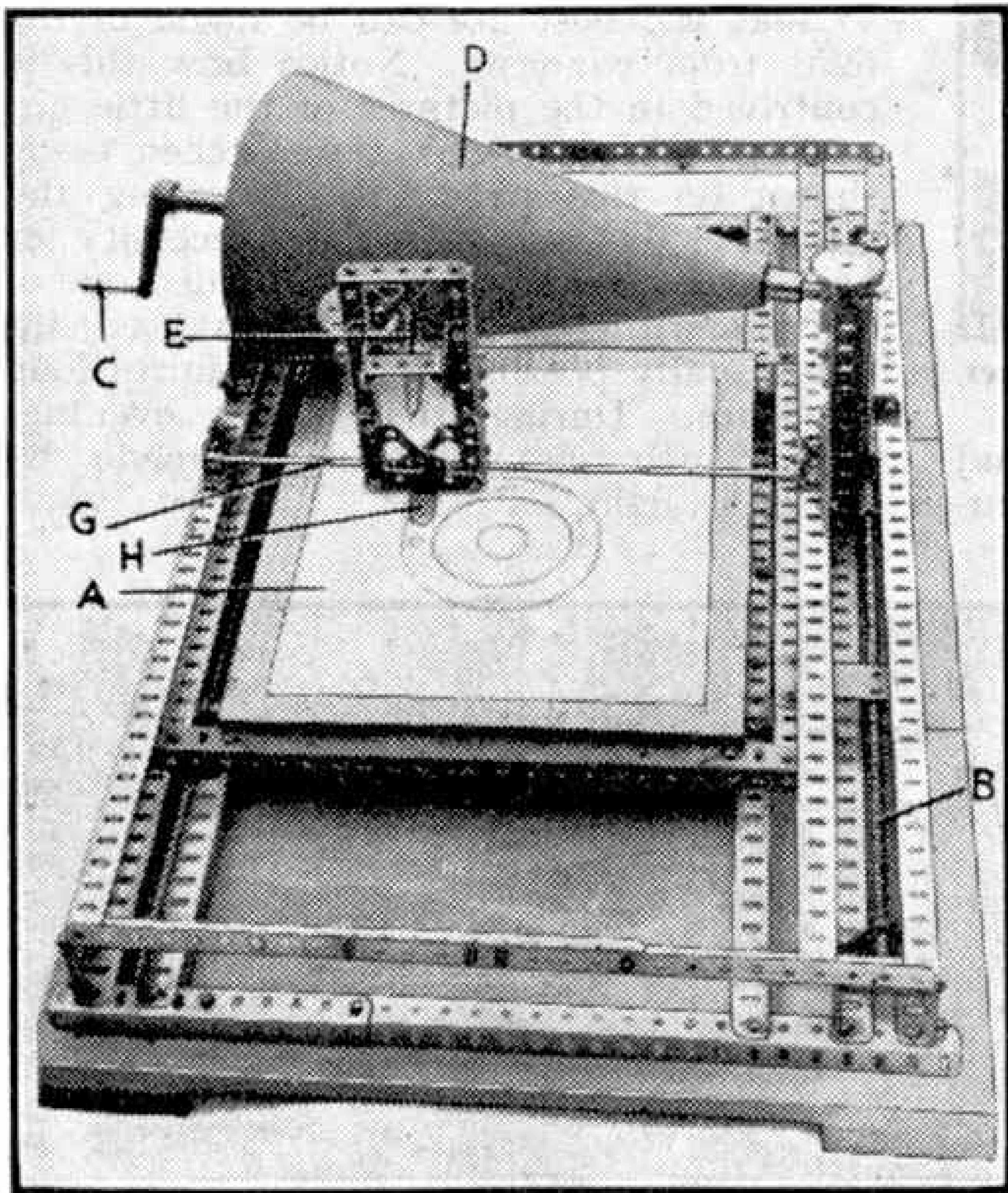
Fig. 1. General view of the Meccano planimeter designed and built by Mr. G. R. Sankey. It is shown here fitted with a counter and tracing sight made from Meccano parts.
