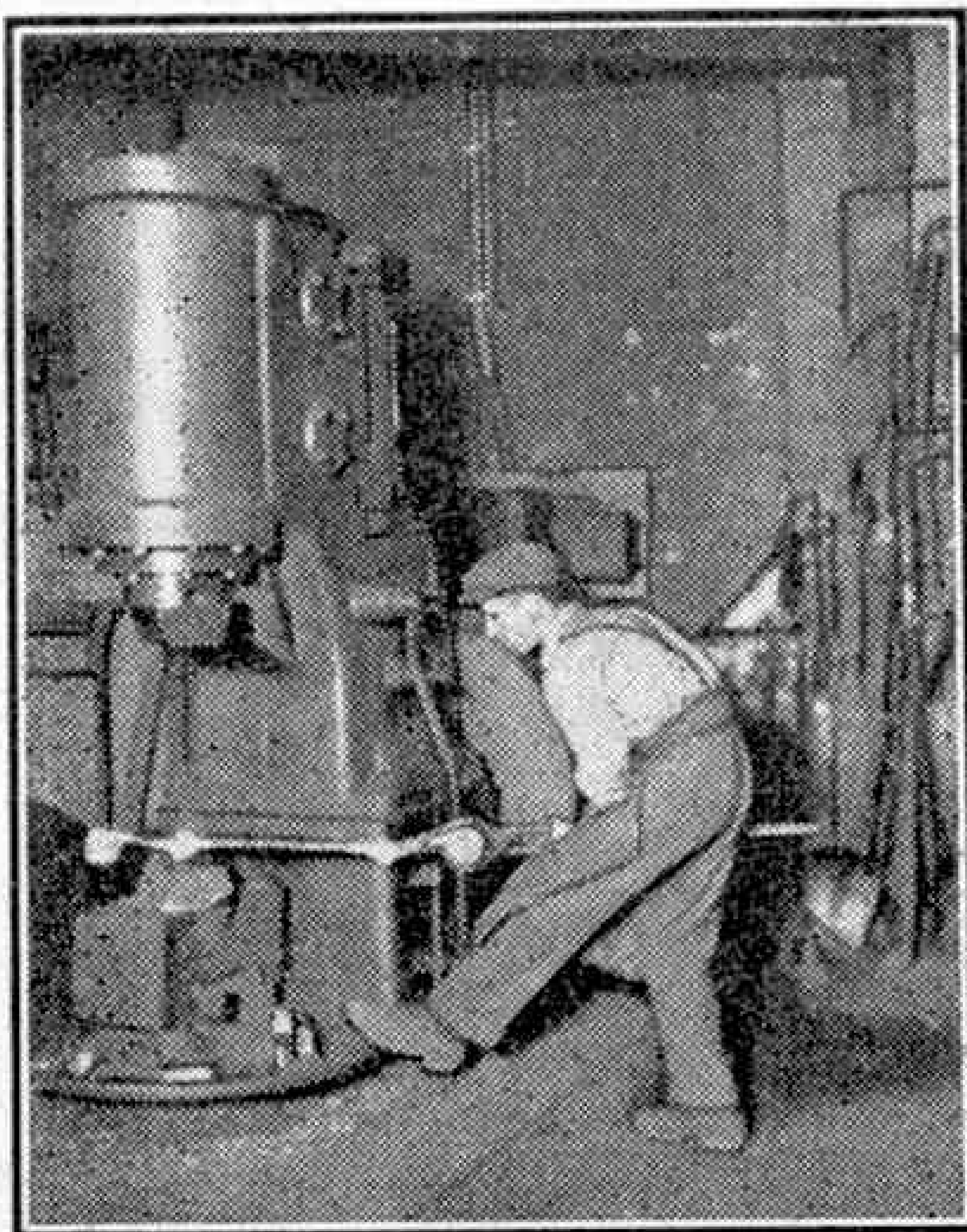
A Massey "Clear Space" pneumatic hammer at work. Photograph by courtesy of B. and S. Massey Ltd., Openshaw, Manchester.
