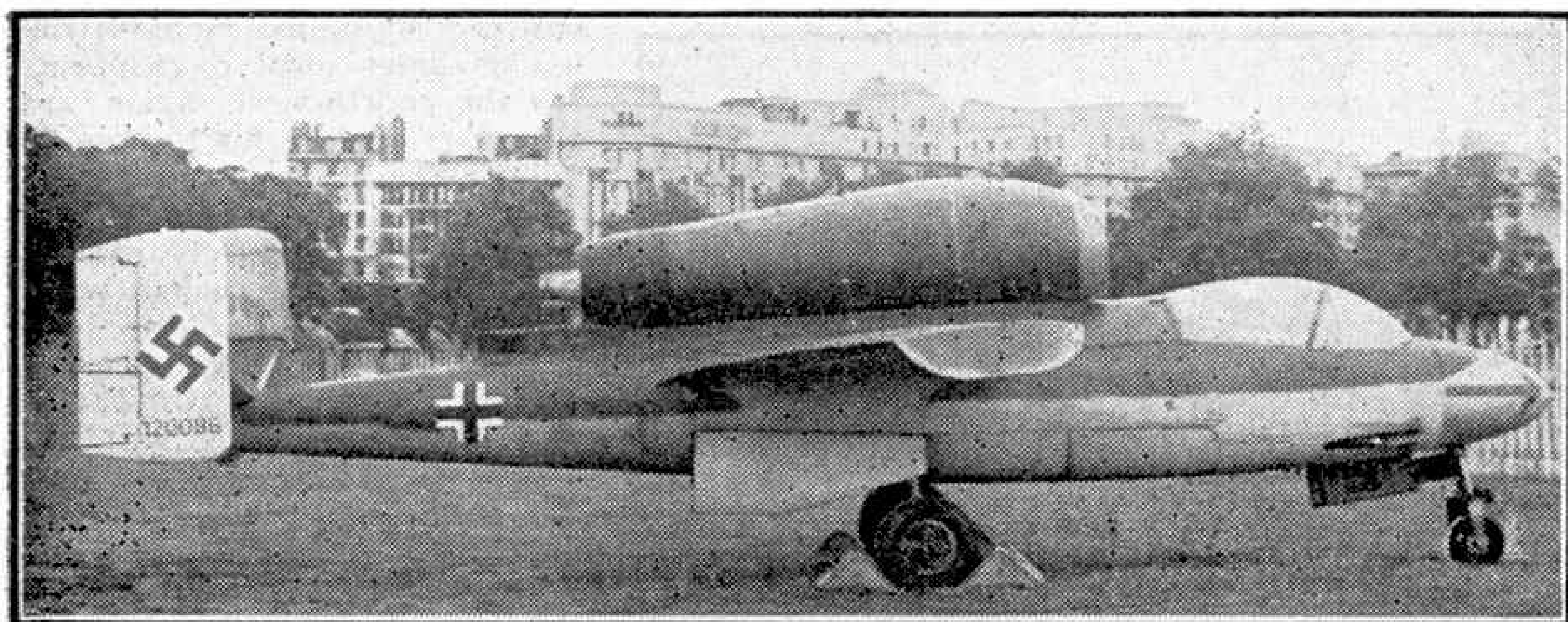
The Heinkel 162 "Volksjaeger" jet-propelled fighter. Photograph "The Aeroplane" Copyright.
