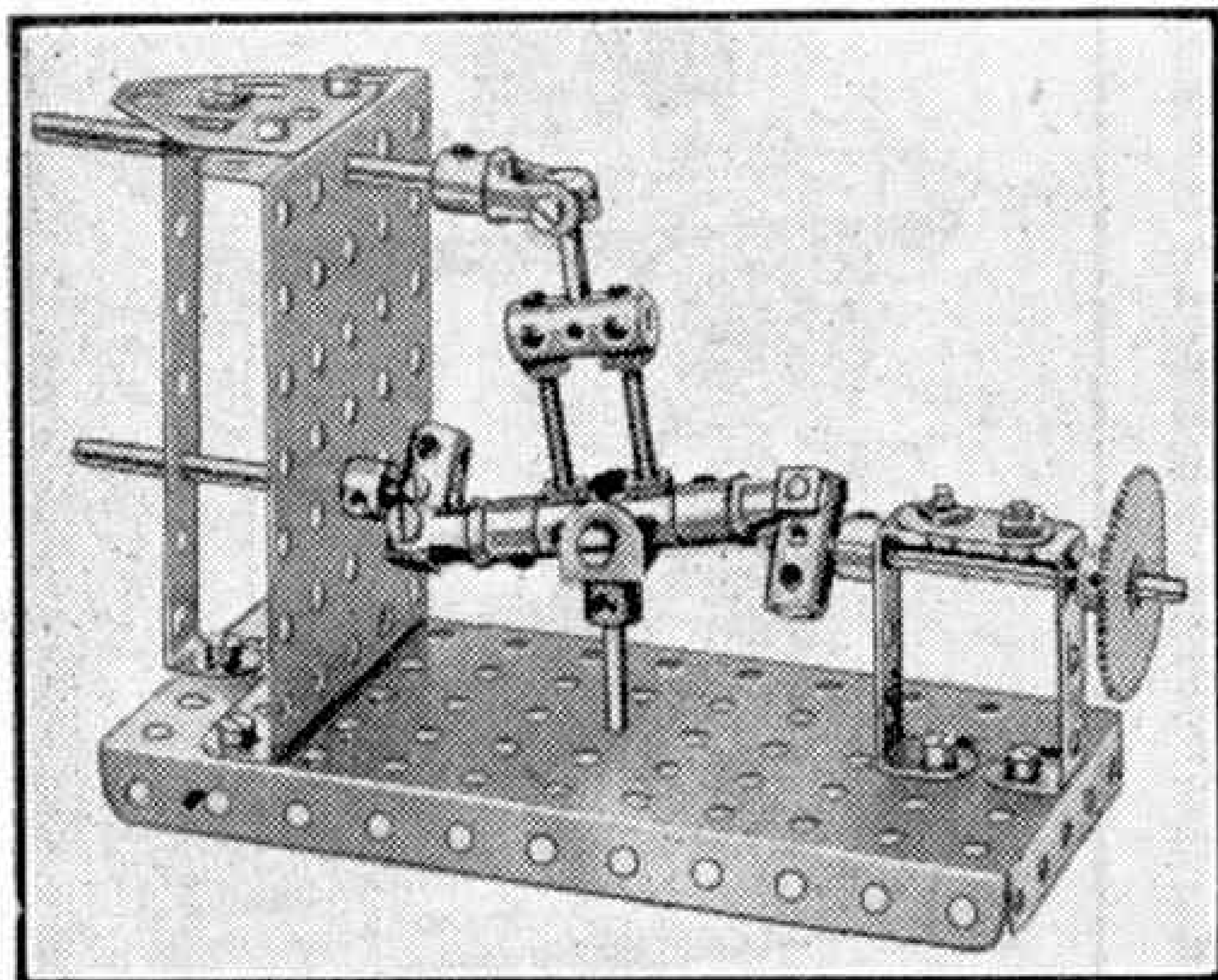
Fig. 1. The modified swashplate movement referred to on this page.
