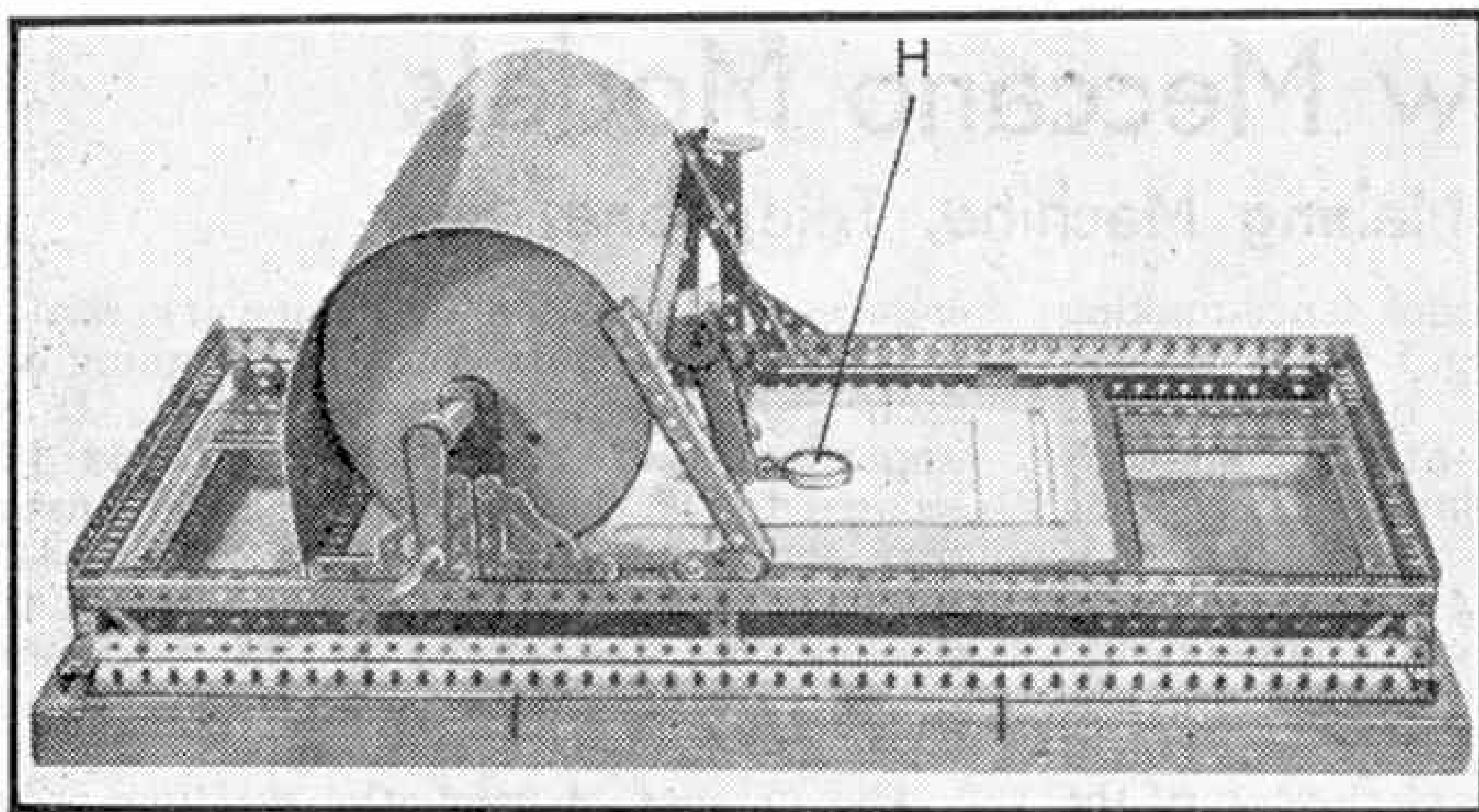
Fig. 3. The planimeter fitted with a commercial counter, a glass disc tracing sight and protective cover over the cone.
