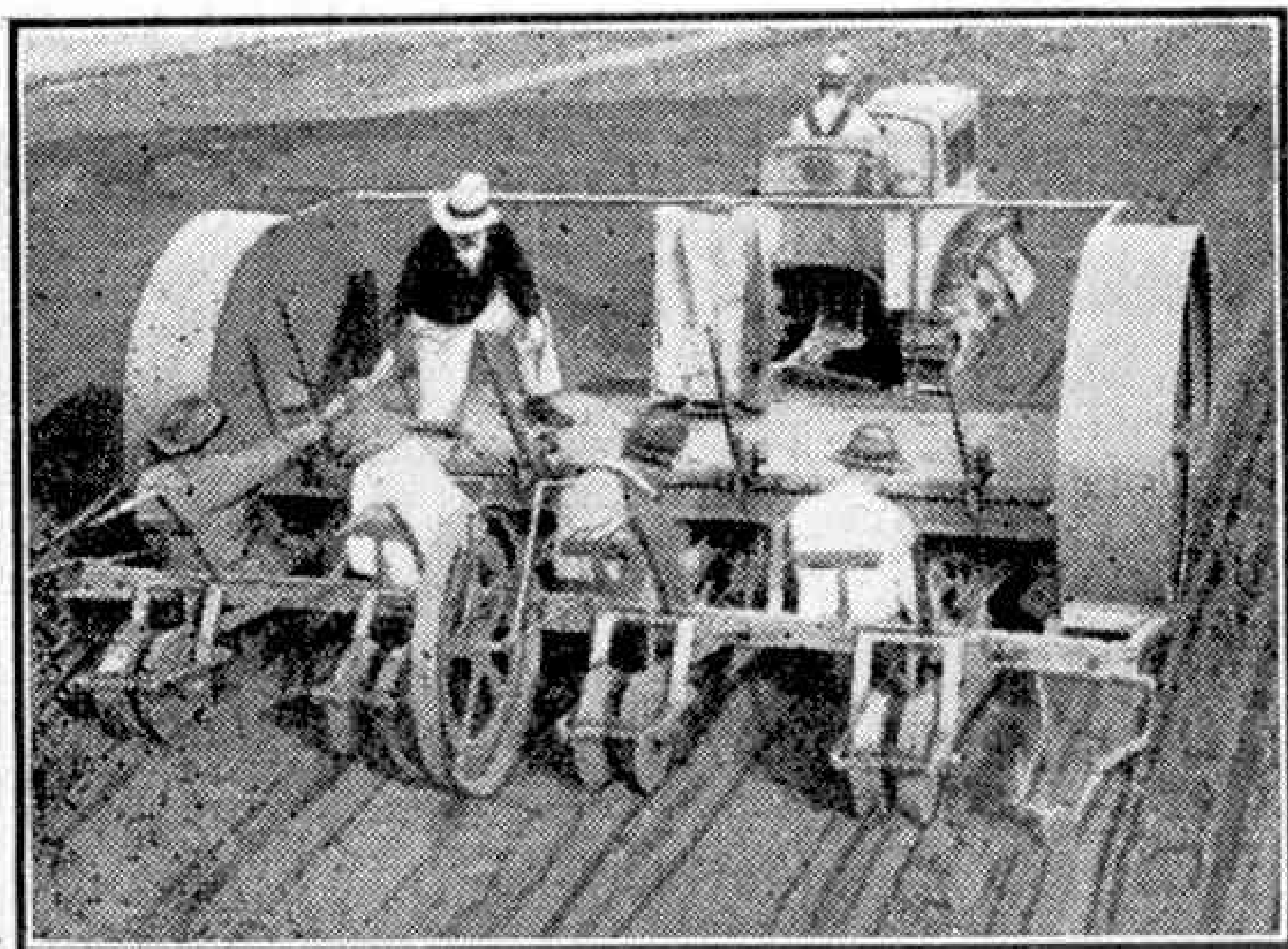
Transplanting guayule seedlings. The machine prepares the holes and covers the roots of the seedlings dropped in by the workmen, each of whom plants 60 seedlings a minute.
