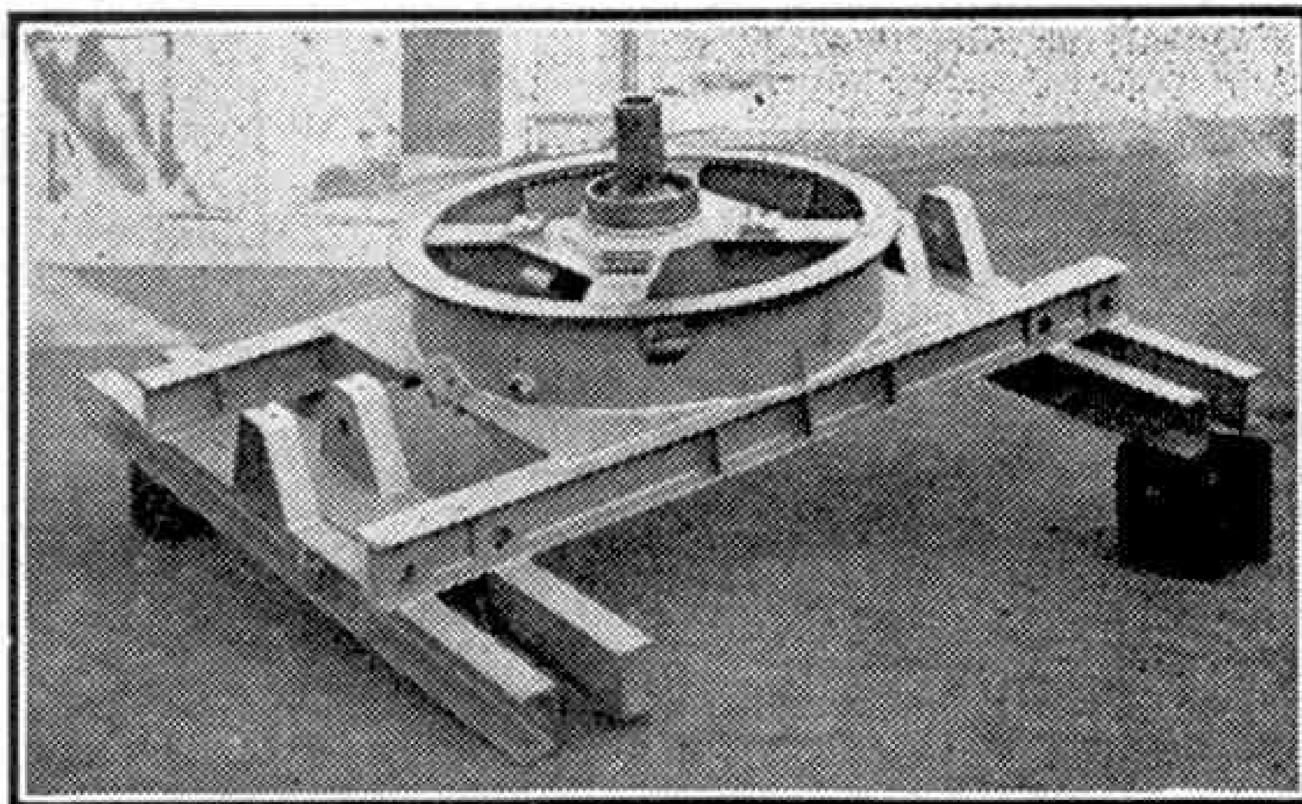
The car body of the N.C.H. Excavator. It is of all-welded construction.
