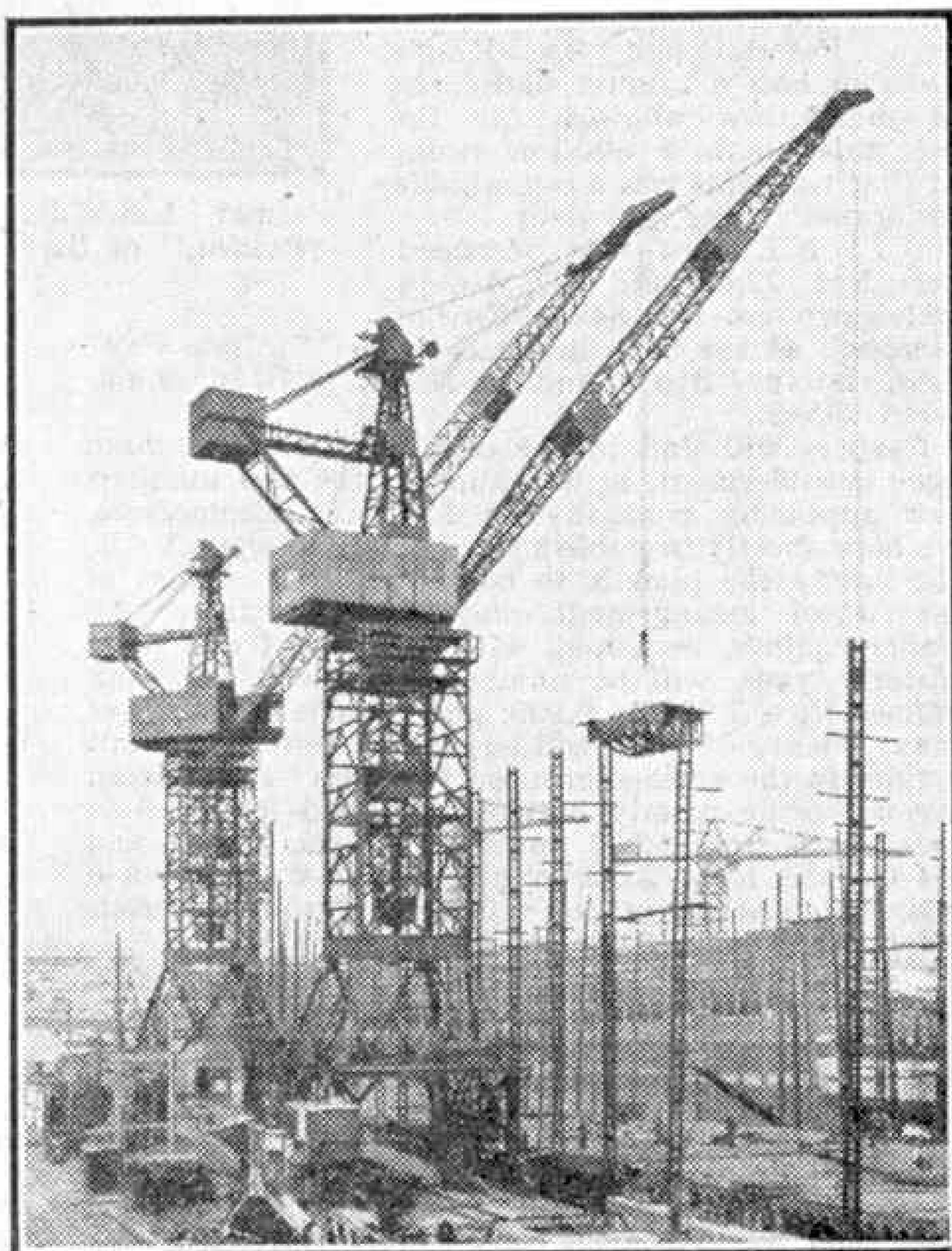
Fifteen-ton travelling Monotower cranes alongside a ship-building berth. The jibs of these cranes are 127 ft. 6 in. long, and the towers themselves have a height of 76 ft. 6 in. For our cover, and for the above illustration, we are indebted to Butters Bros. and Co. Ltd., Glasgow.
