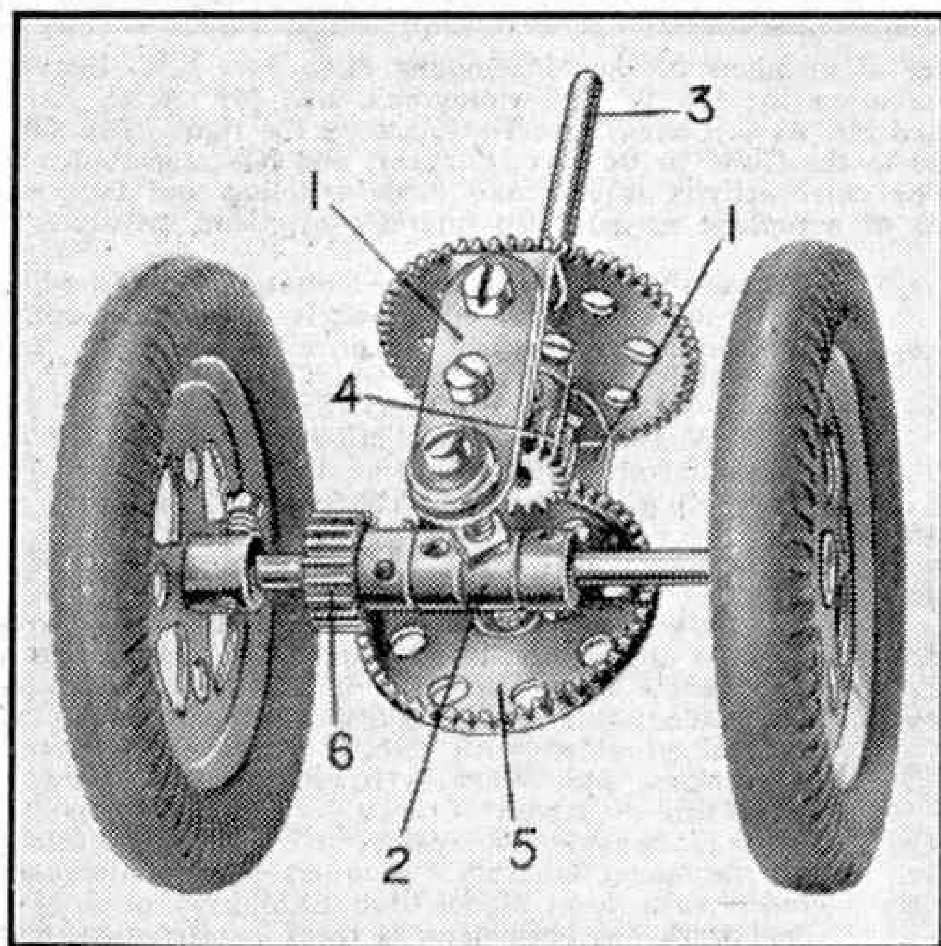
Fig. 1. A novel castor mechanism for mobile cranes.
