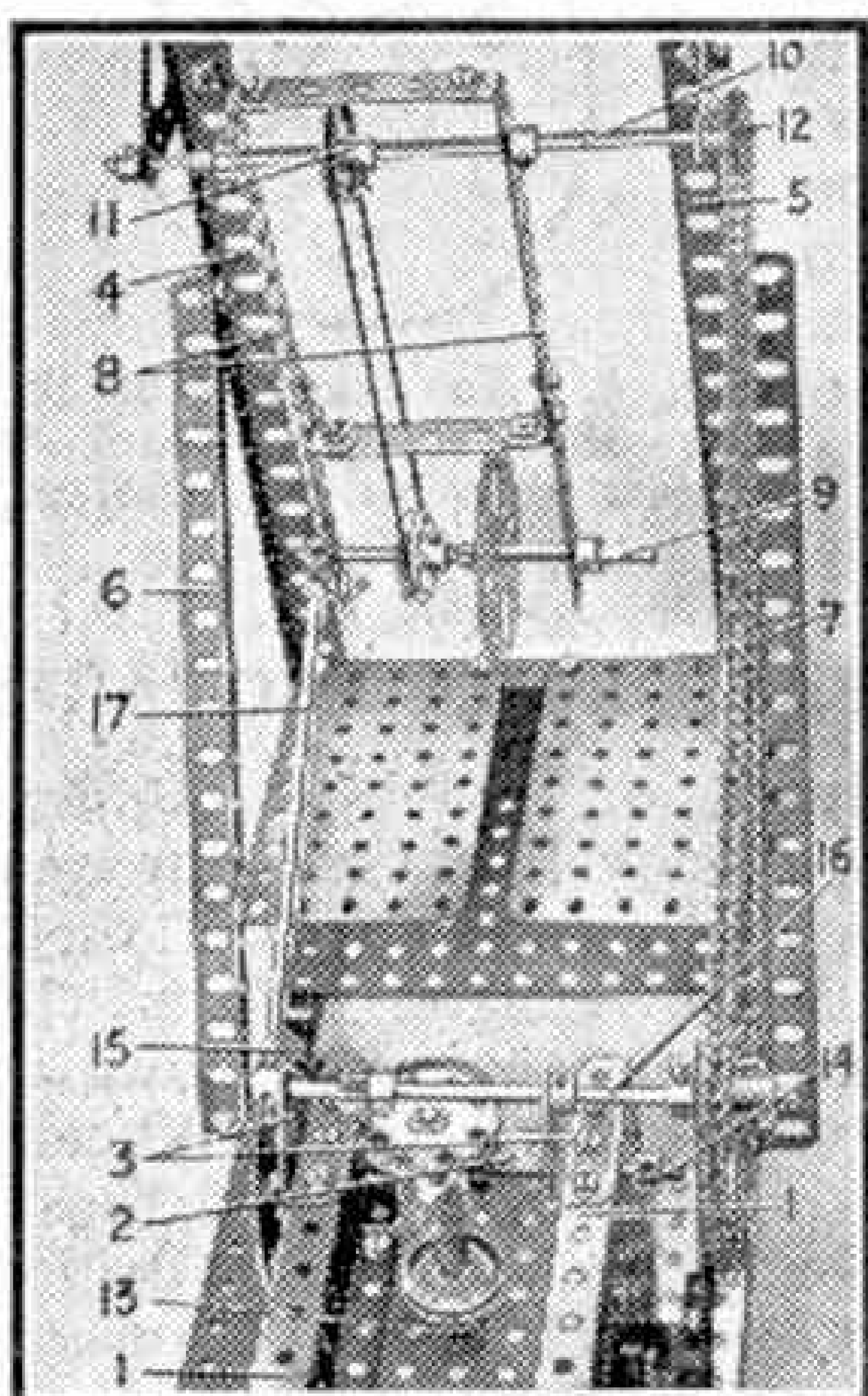
Fig. 2. A close up view of the sawing machine showing mechanism.
