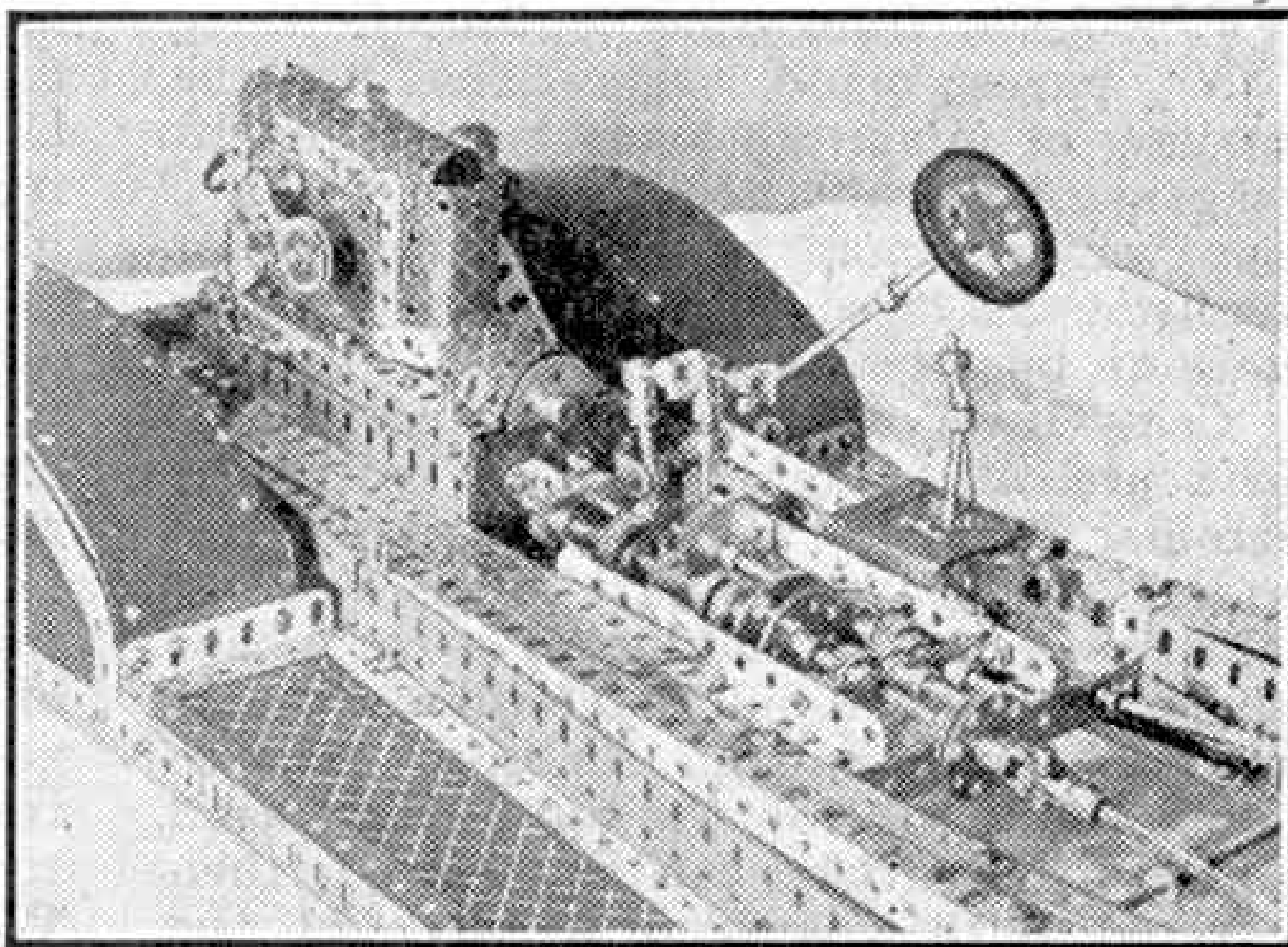
The engine unit and gear-box of G. P. Alcock's prize-winning motor chassis.
