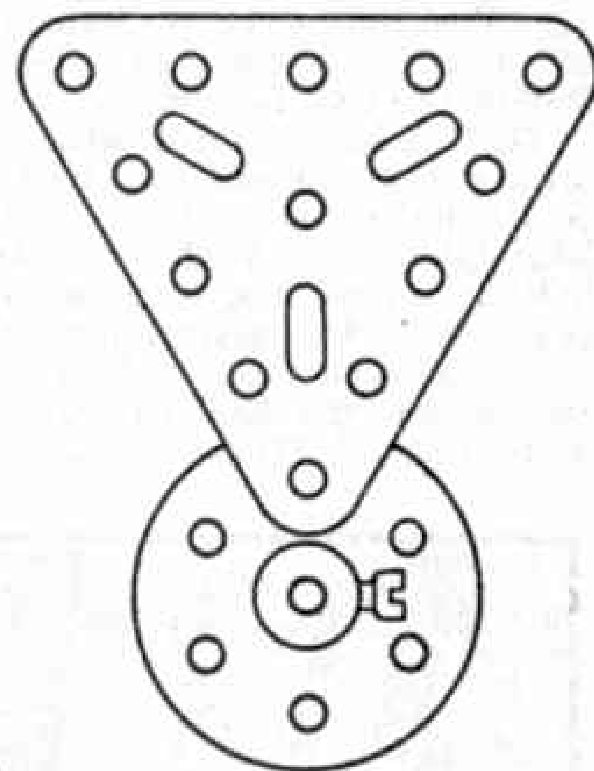
Fig. 4. An example of the use of a six-hole wheel as suggested by Mr. E. Armitage, Liverpool.
