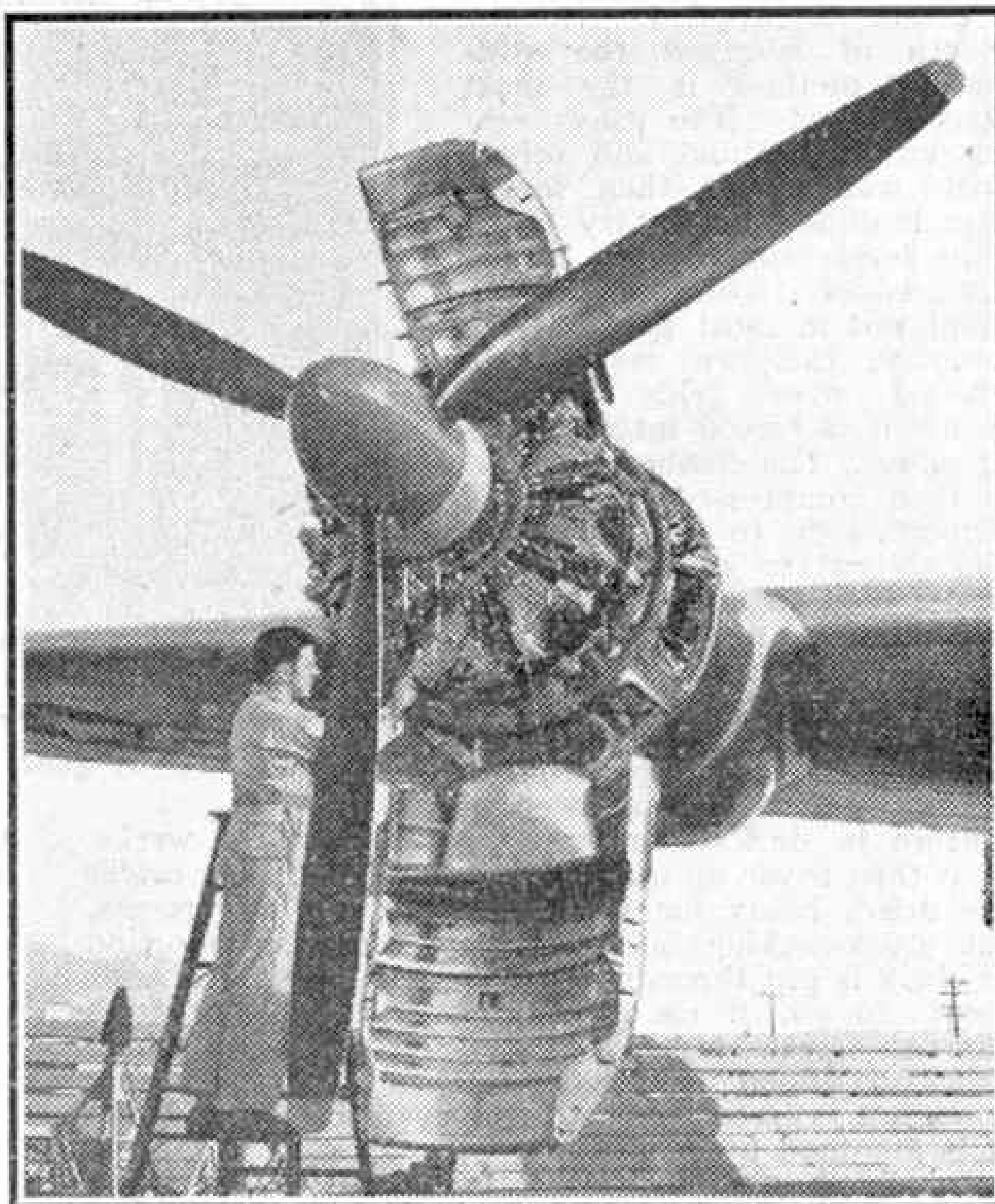
New type engine cowling for the "Constellation." The side panels of the cowling have been detached and the upper and lower panels, looking like giant jaws, have been swung out of the way while the mechanic works on the engine. Photograph by courtesy of Lockheed Aircraft Corporation, U.S.A.
