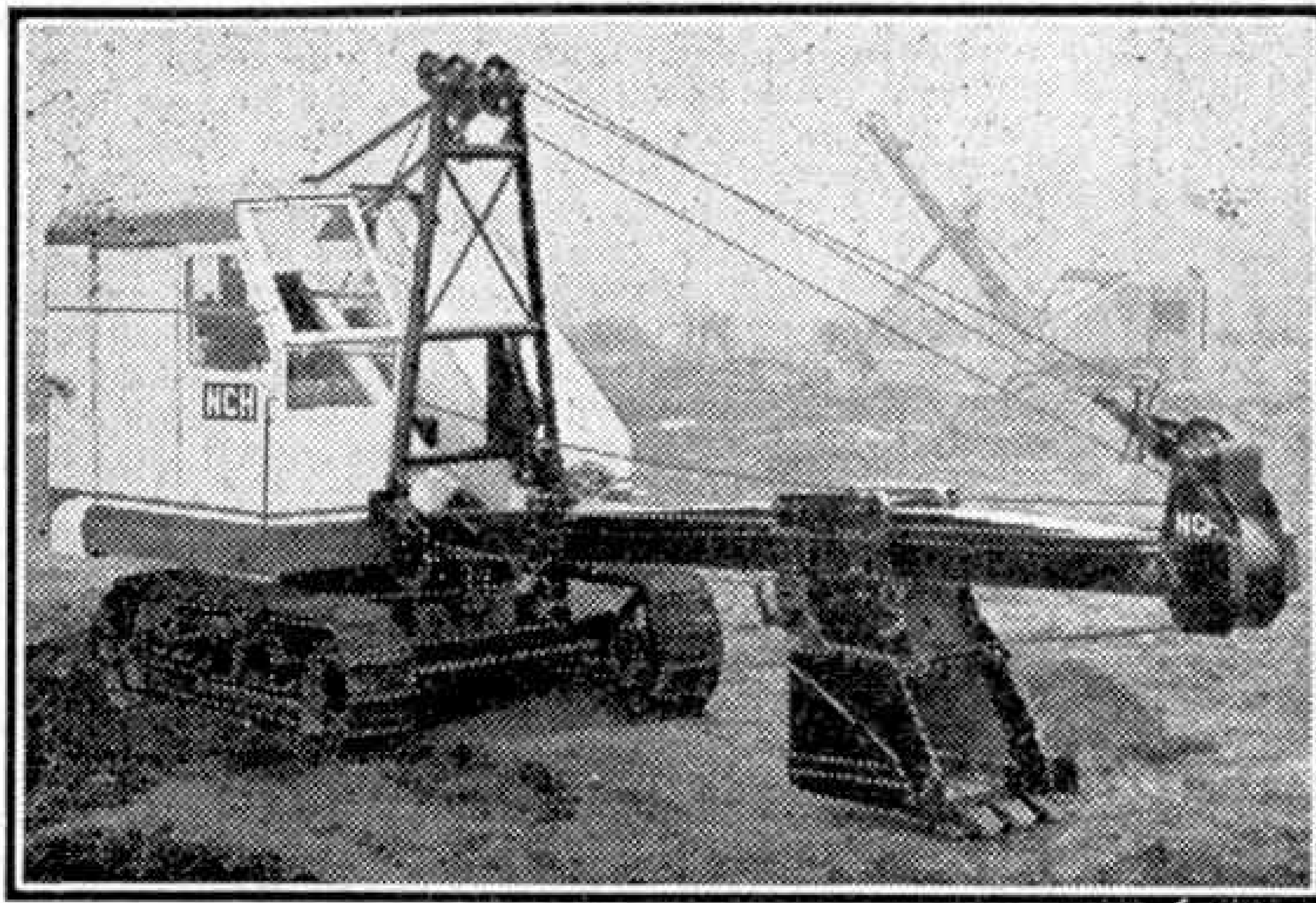
The N.C.H. Excavator described on this page. It is a product of Newton Chambers & Co. Ltd., Thorncliffe, to whom we are indebted for our illustrations.
