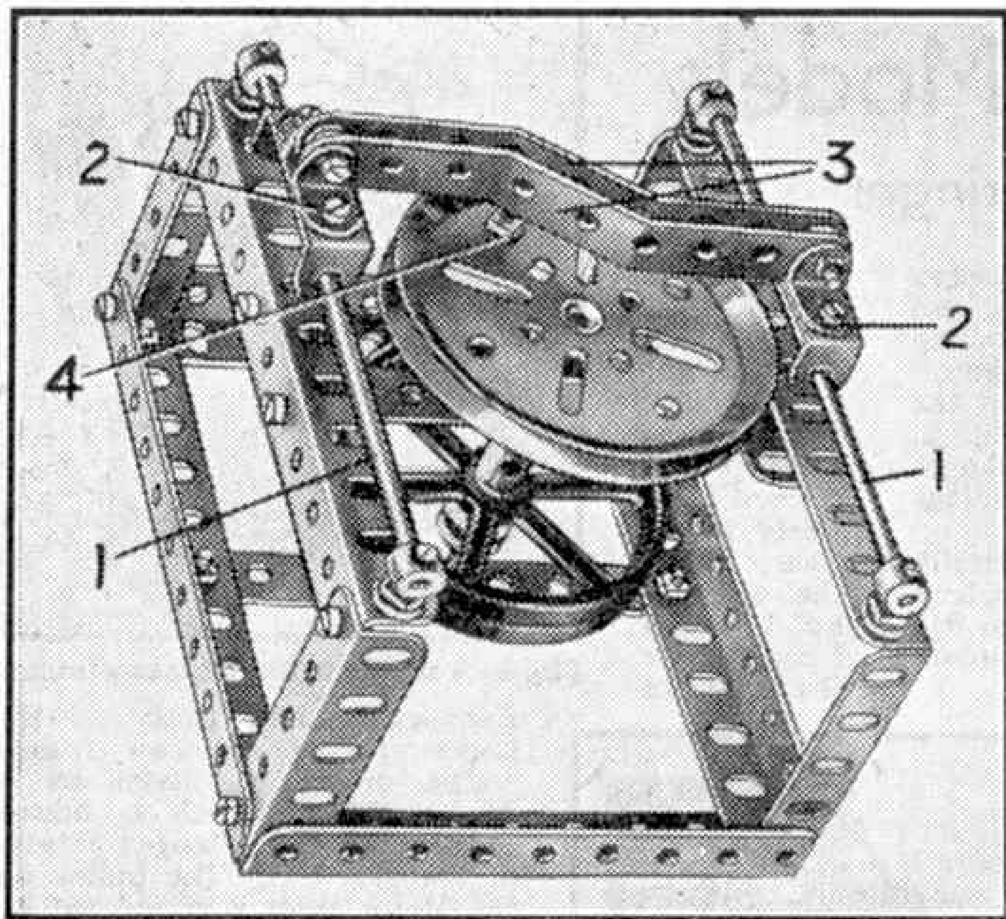
Fig. 3. The novel motion converter referred to on this page.
