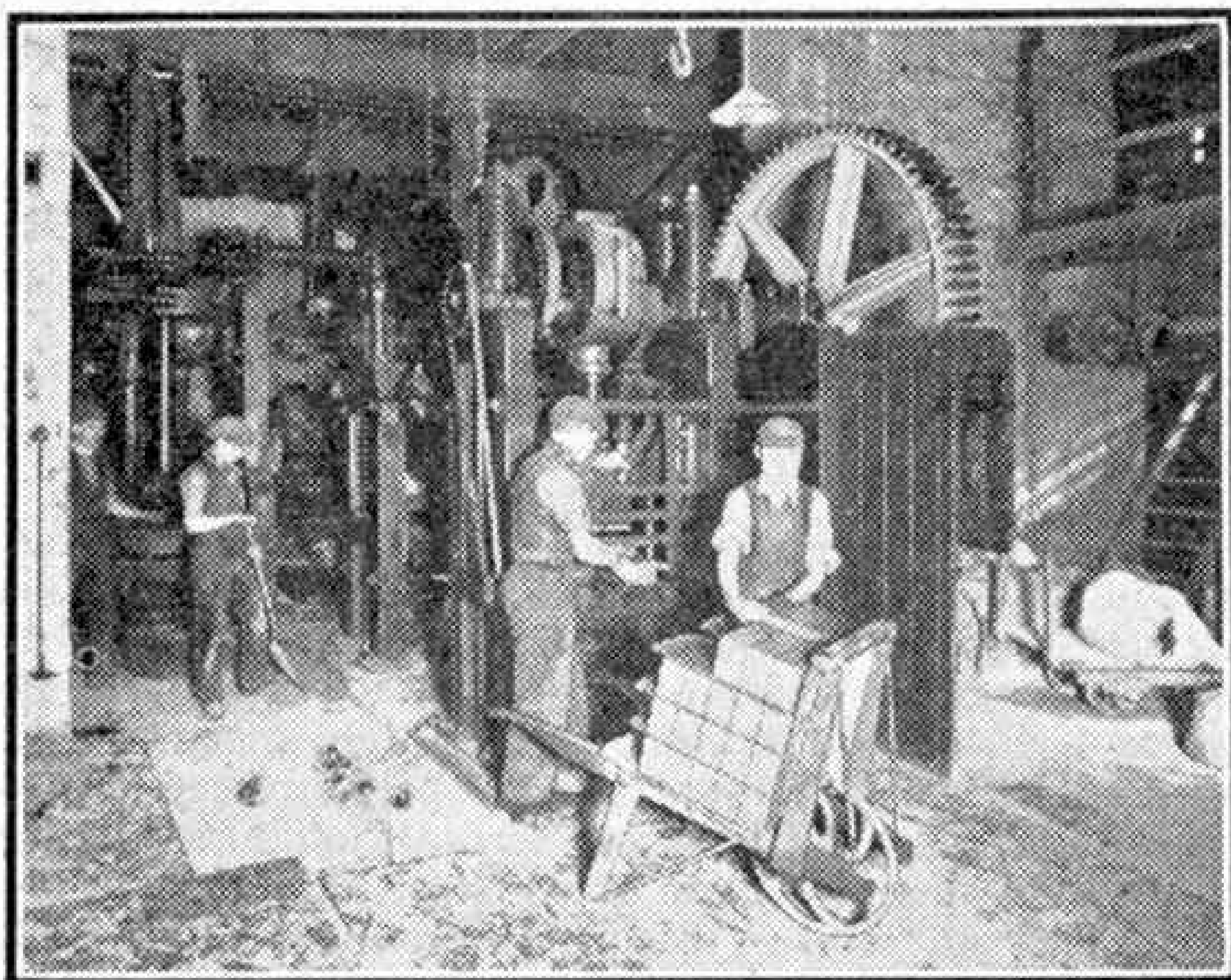
Bricks being taken off a stiff-plastic facing brick machine. The illustrations to this article are reproduced by courtesy of the Brick Marketing Co. Ltd., Doncaster.
