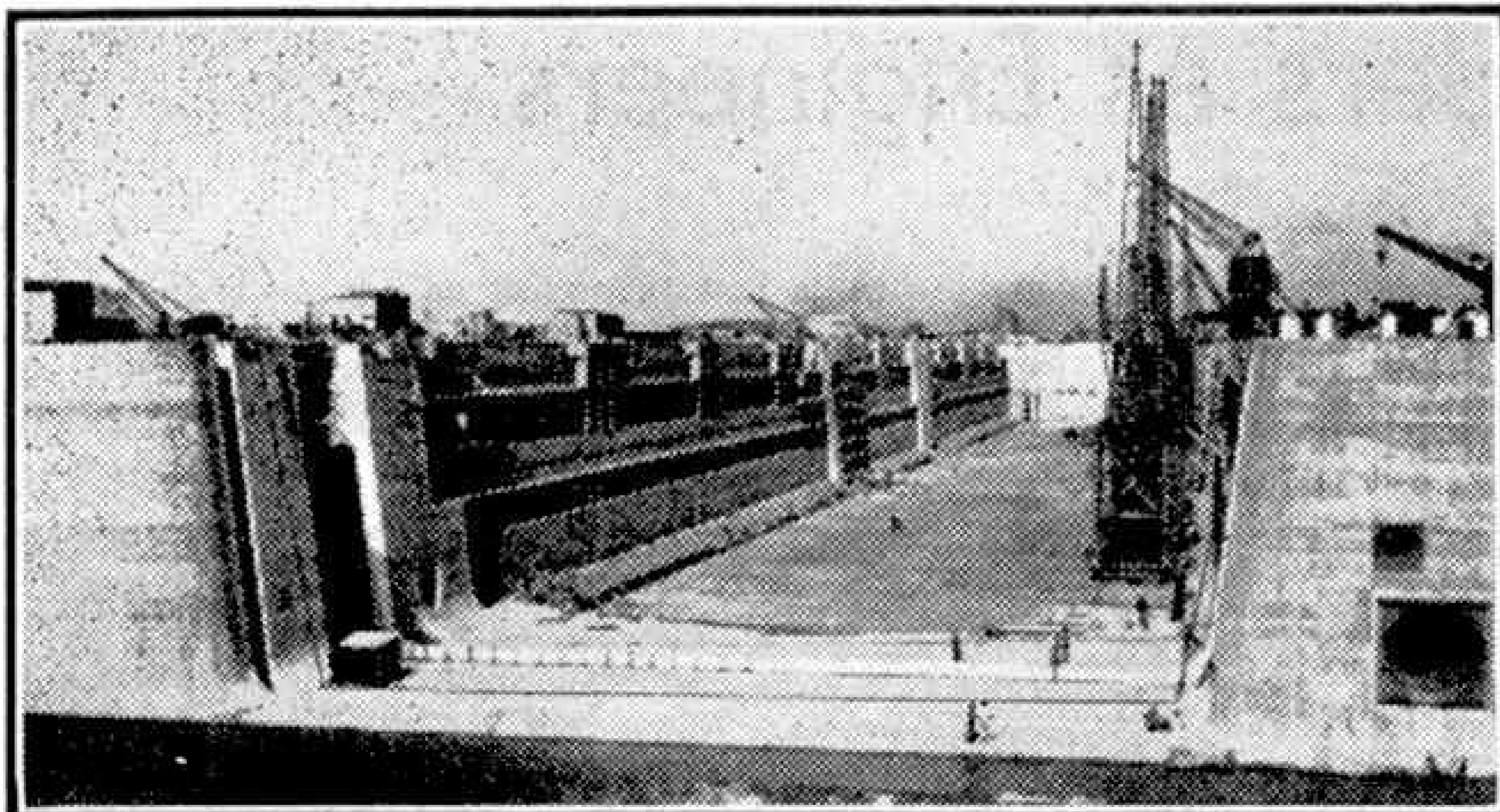
The construction of the Sturrock Dock is well shown in this illustration. Photograph by courtesy of the South African Railways and Harbours Administration.
