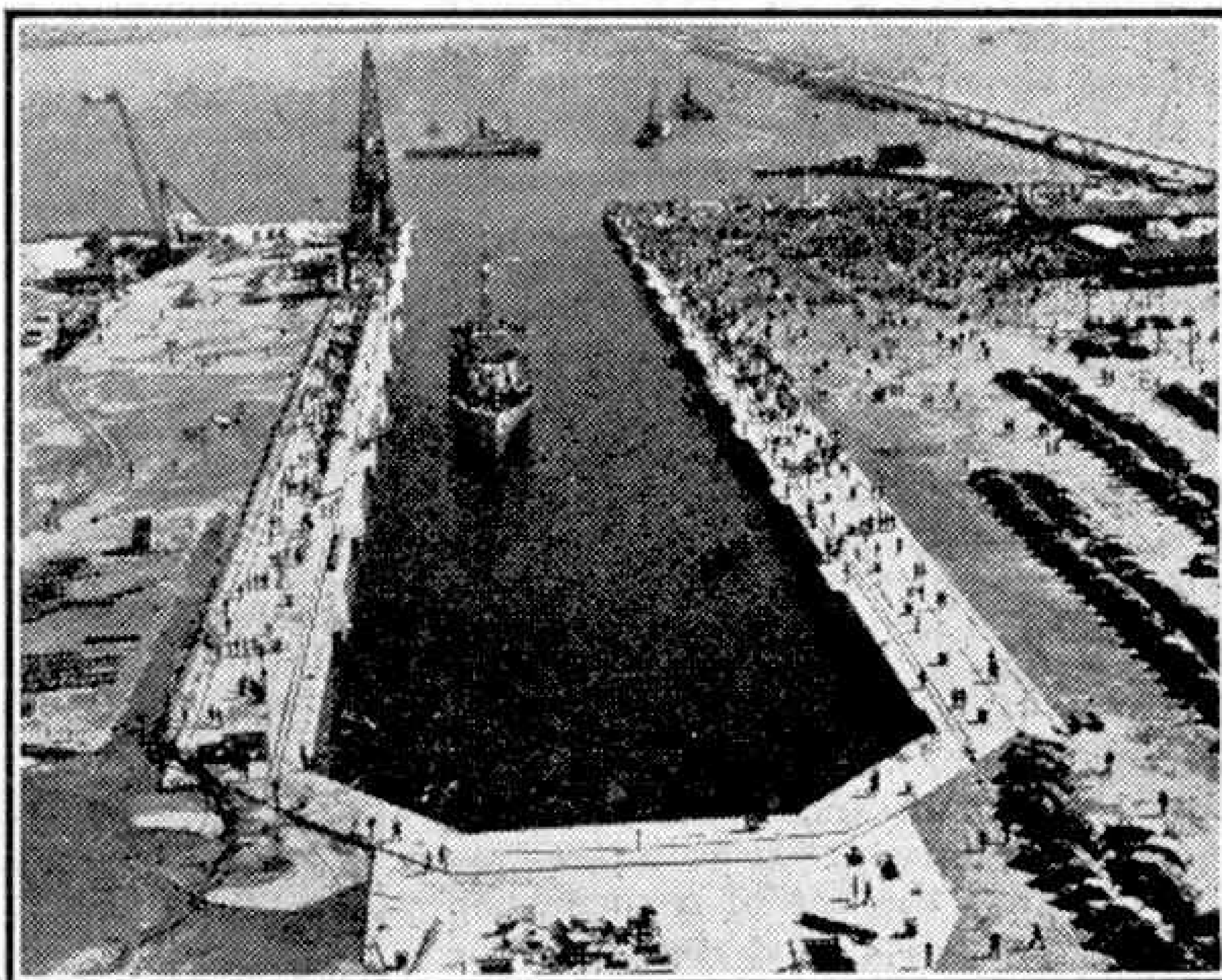
The Sturrock Graving Dock, Cape Town, immediately after the opening ceremony on 18th September 1945. Photograph by courtesy of the South African Railways and Harbours Administration.
