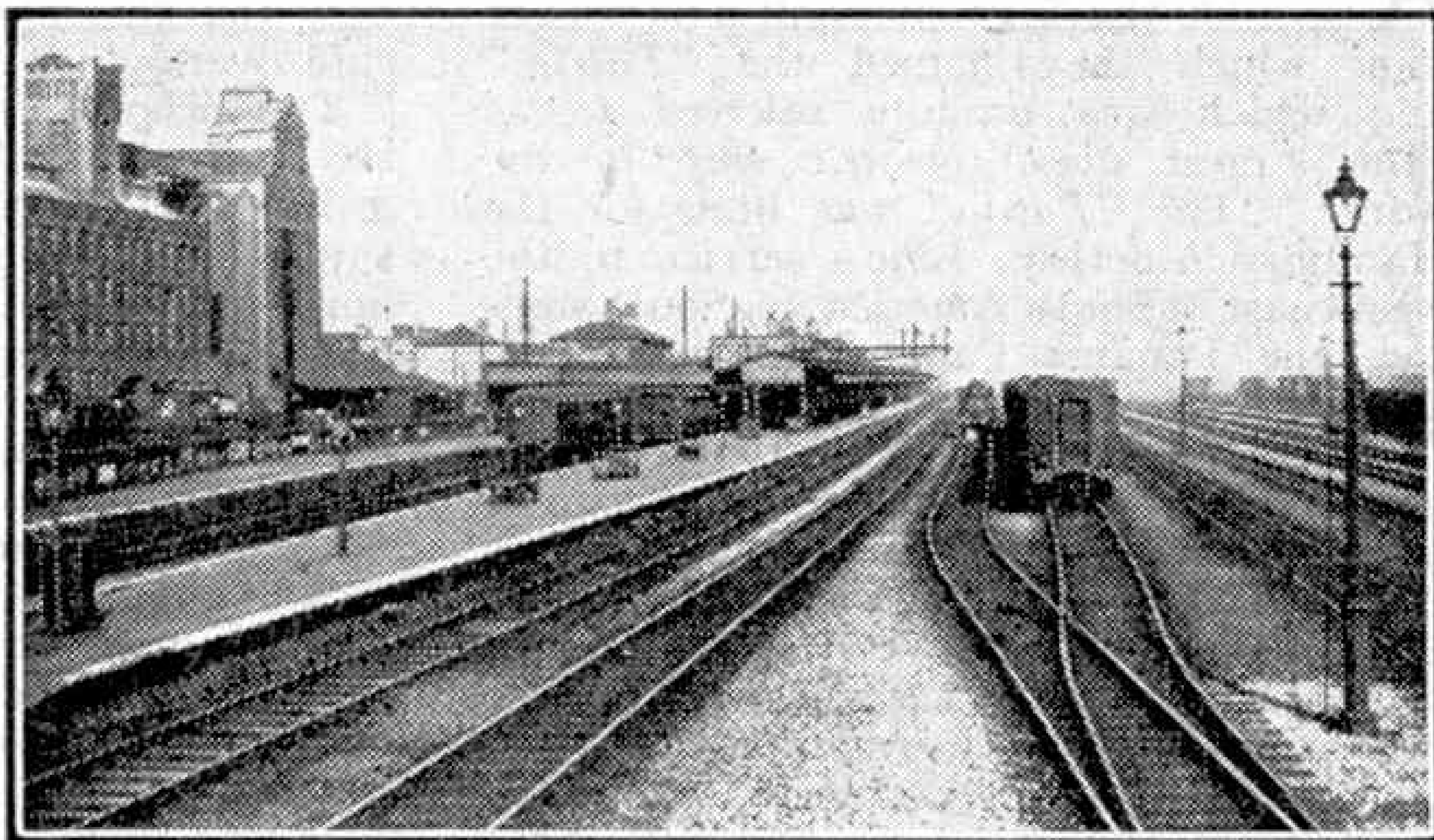
Cambridge station from South Signal Box, showing bay platforms and signals halfway along main platform. Photograph by courtesy of the L.N.E.R.
