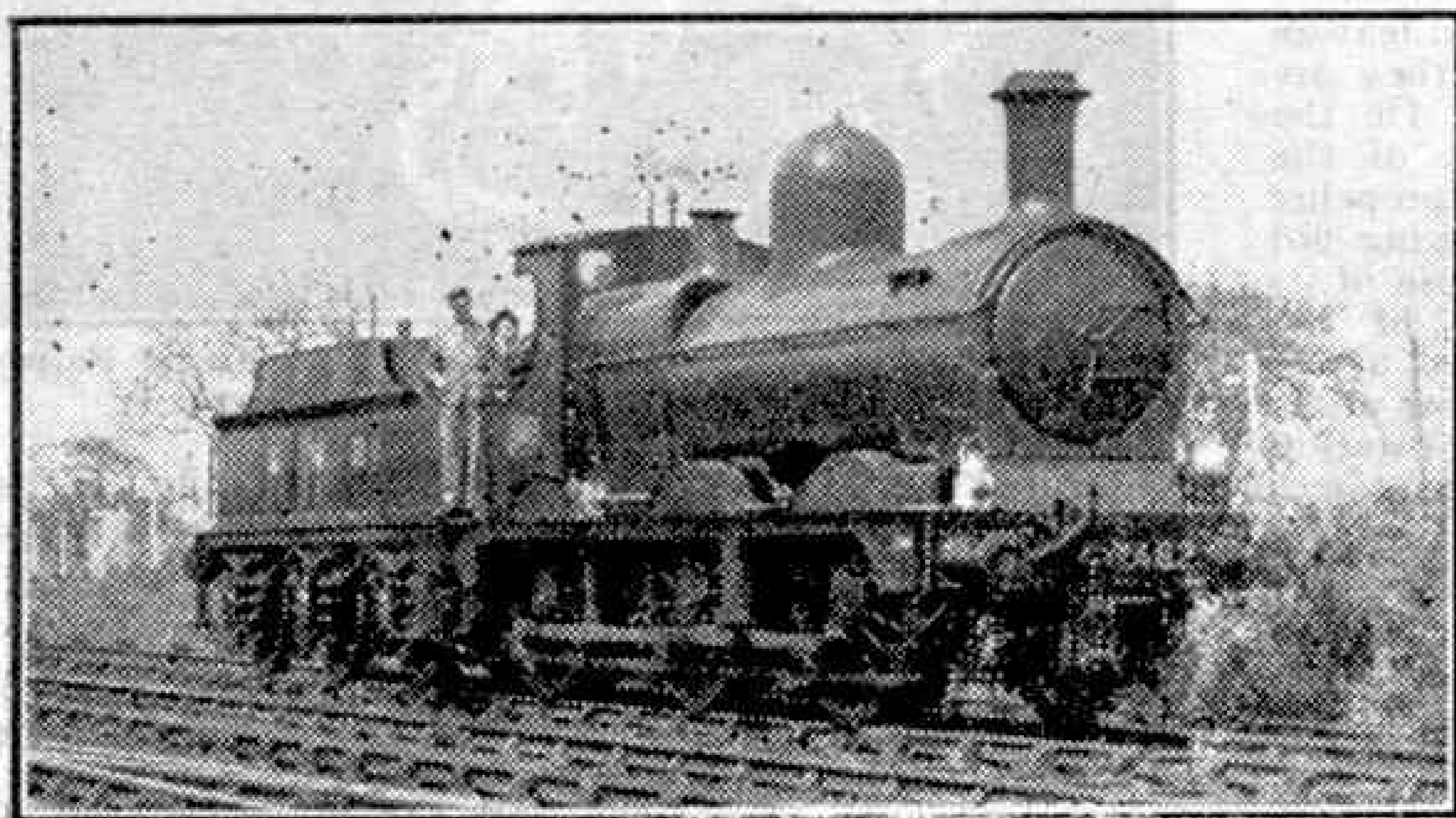
G.W.R. "Dean" 0-6-0 No. 2482 on a trial run after overhaul at Wolverhampton. This is typical of the inside framed engines. The photographs to this article are by D. A. Tipper.
