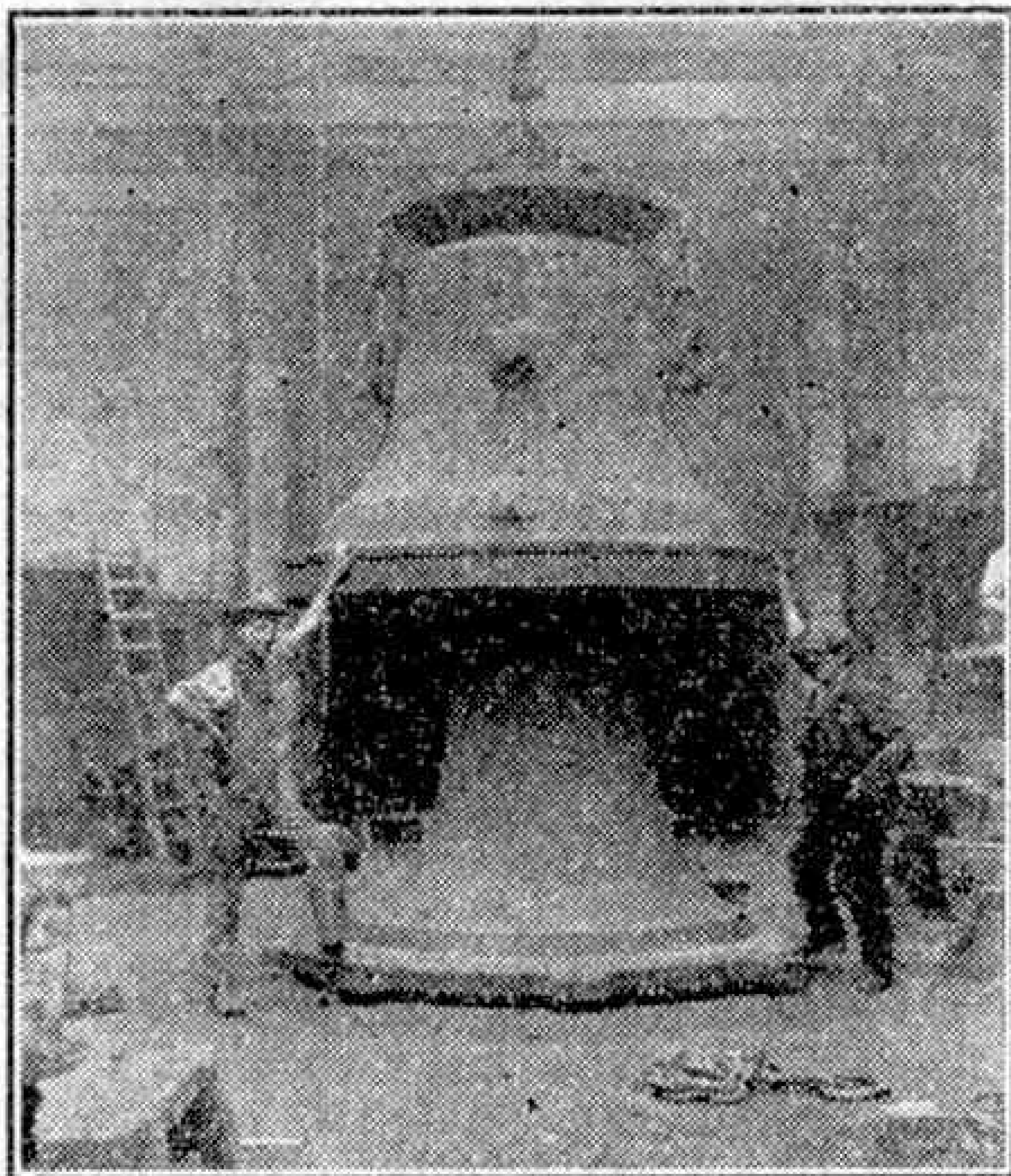
Cope and core, two parts of the mould for a bell. made as complete as it will be when installed ready for use.
