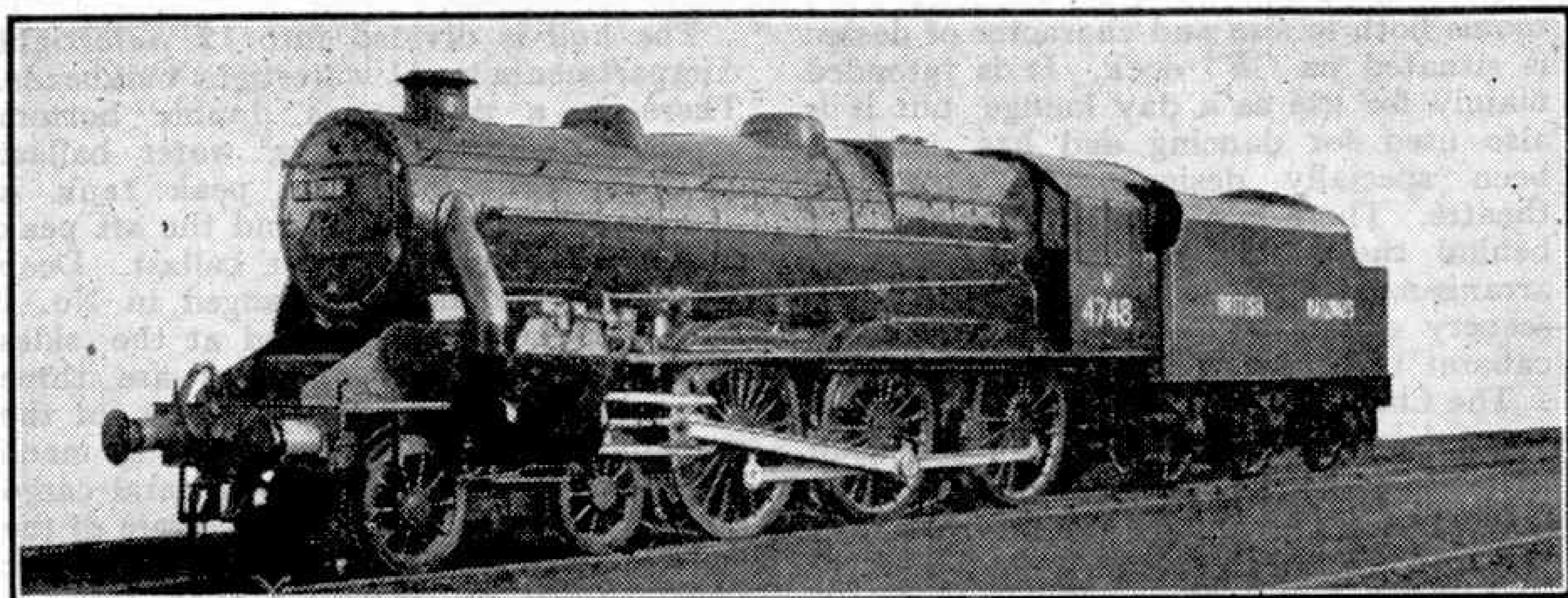
One of the new 4-6-0 locomotives with poppet valves and gear. This design has been developed from the familiar Class 5 4-6-0 of the former L.M.S. (London Midland Region photographs).
