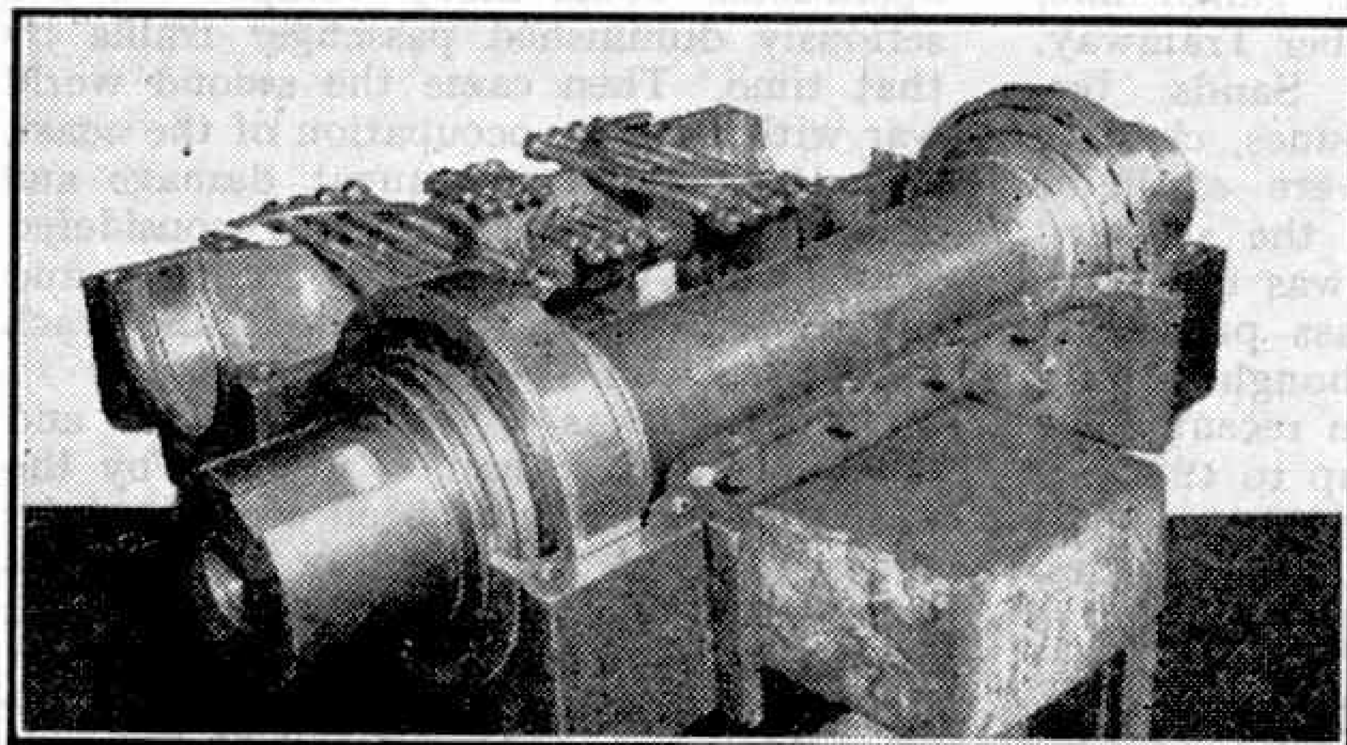
Roller bearing driving axle assembly showing the split cannon-box arrangement housing the axle.
