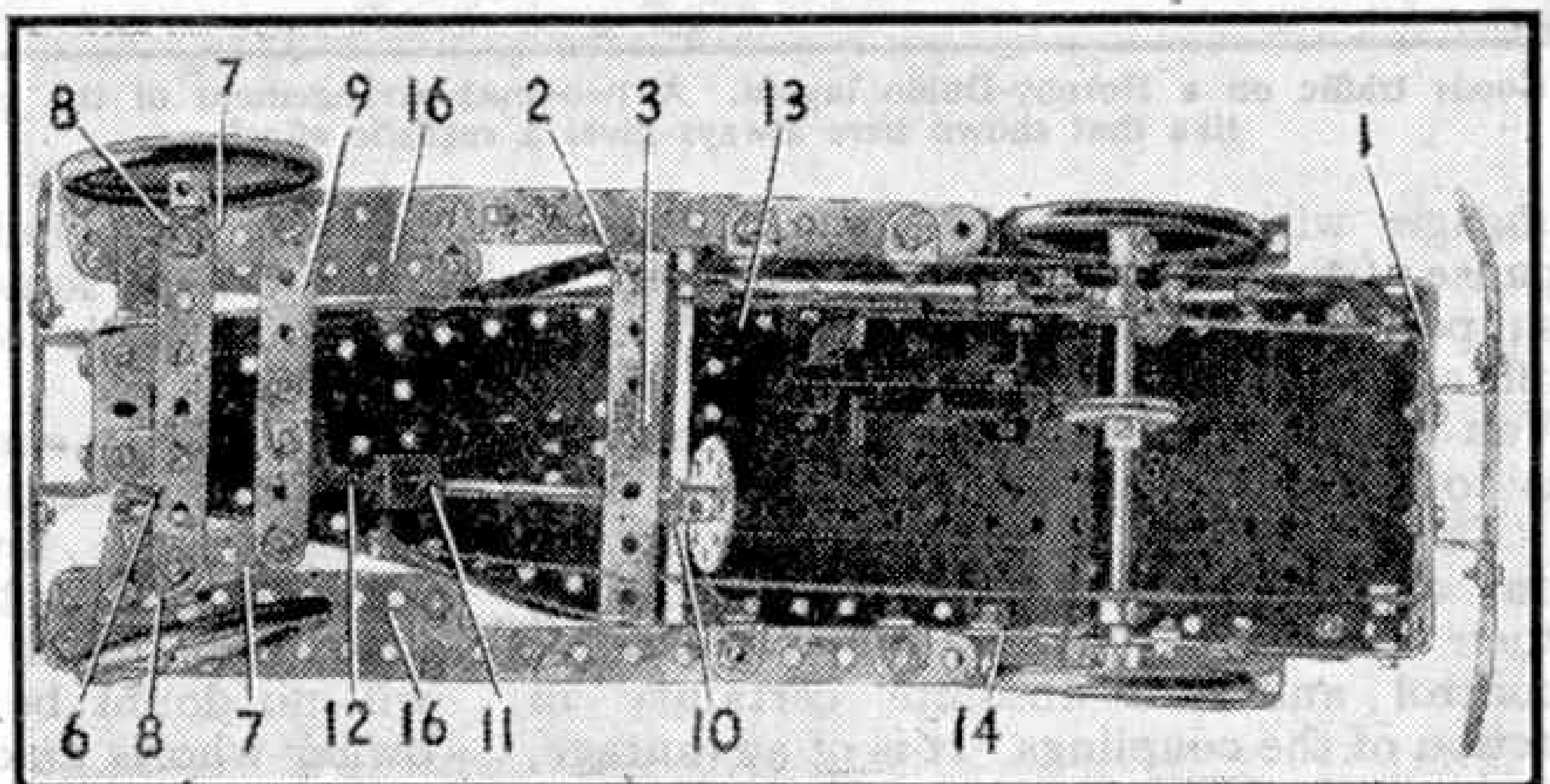
Fig. 3. An underneath view of the saloon car.
