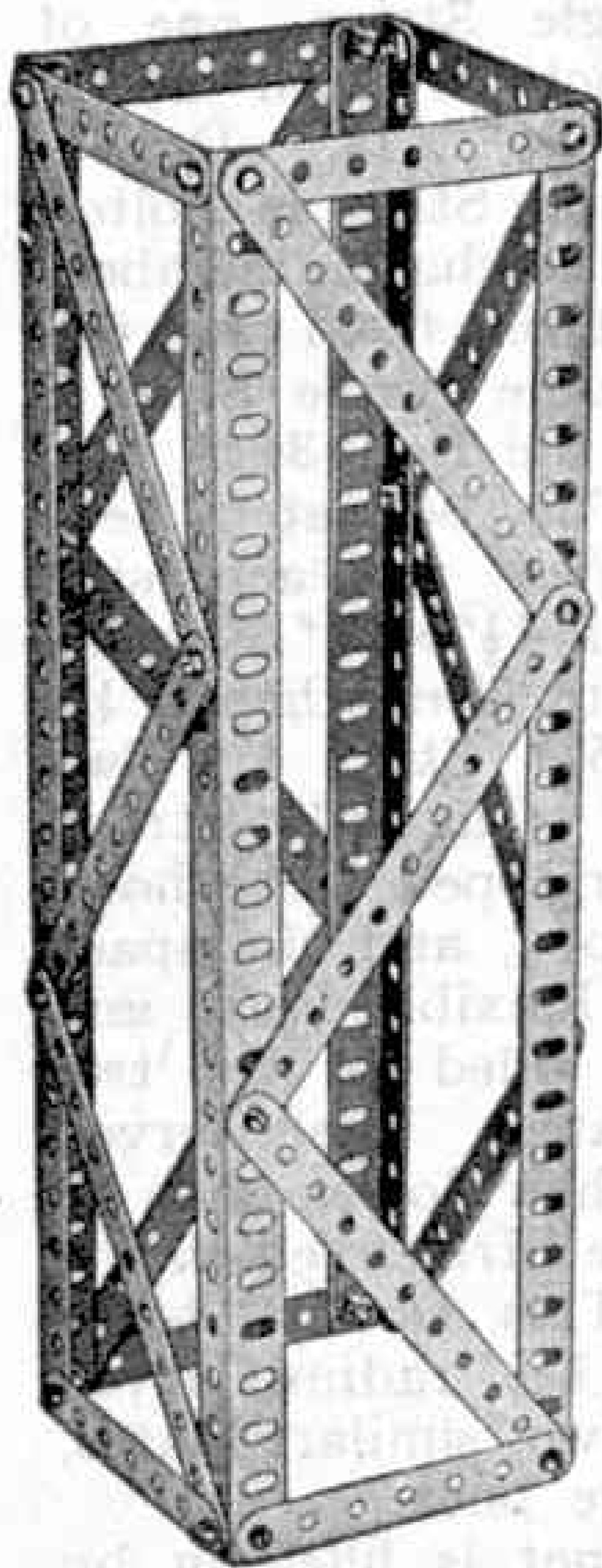
Fig. 3. A box column braced by Meccano Strips to form a rigid and strong structure.
