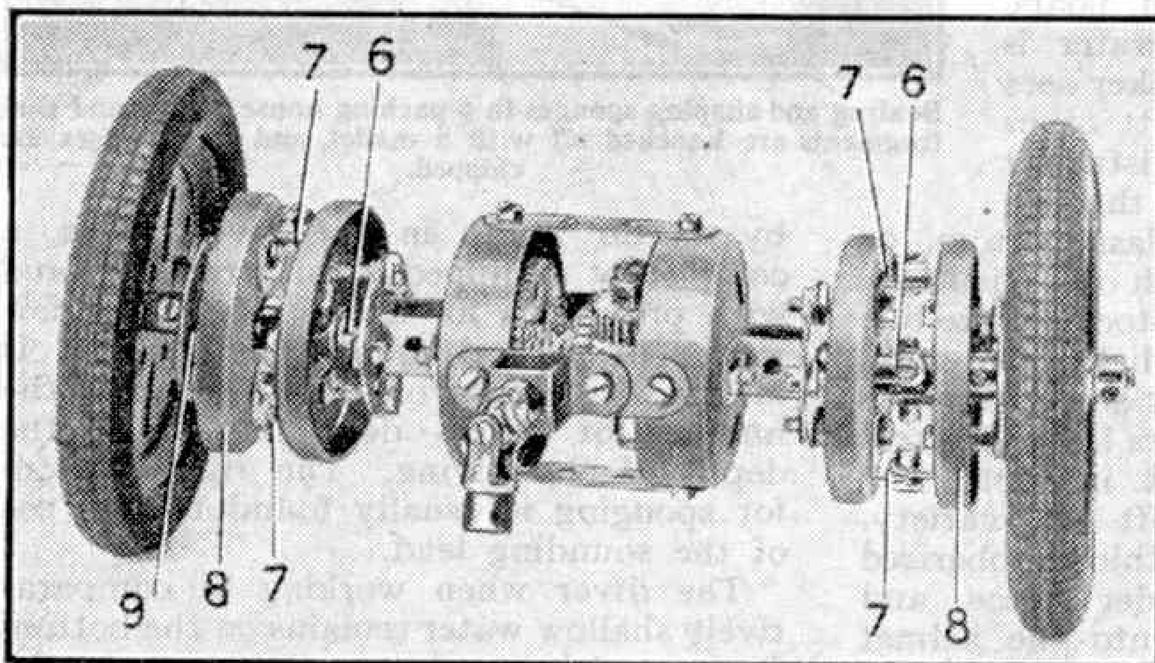
Fig. 1. Front-wheel drive mechanism for a model vehicle.
