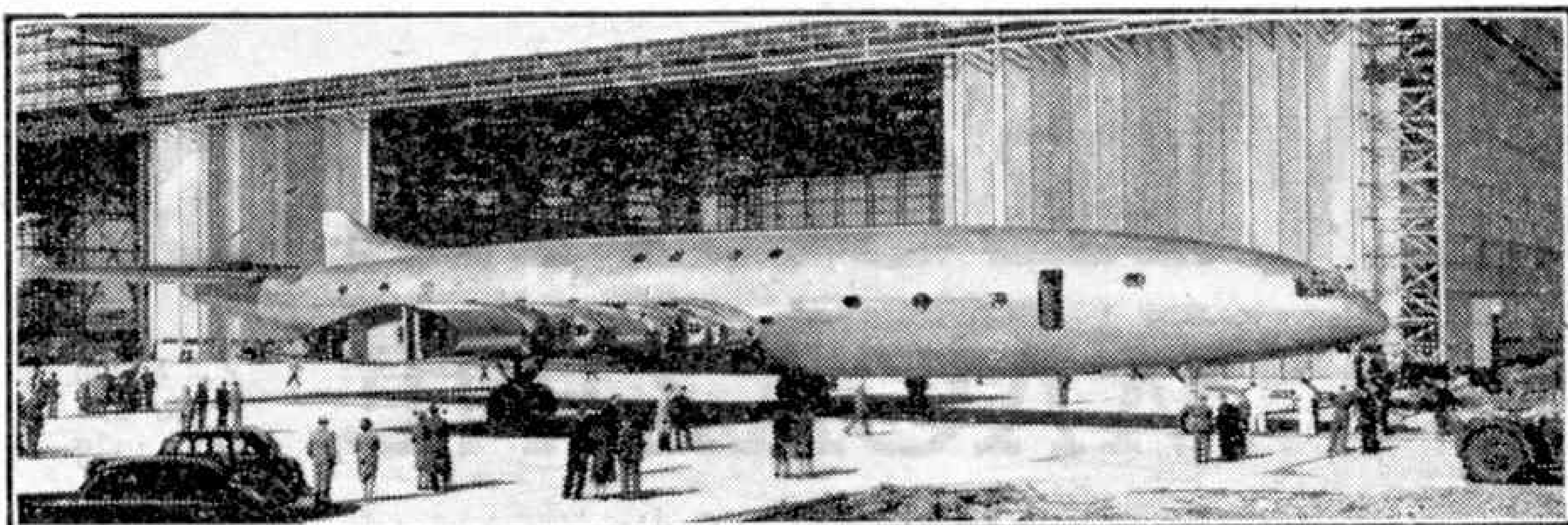
The fuselage of the Bristol "Brabazon" outside the hangar which has been built to accommodate this huge aircraft. Photograph by courtesy of The Bristol Aeroplane Co. Ltd.
