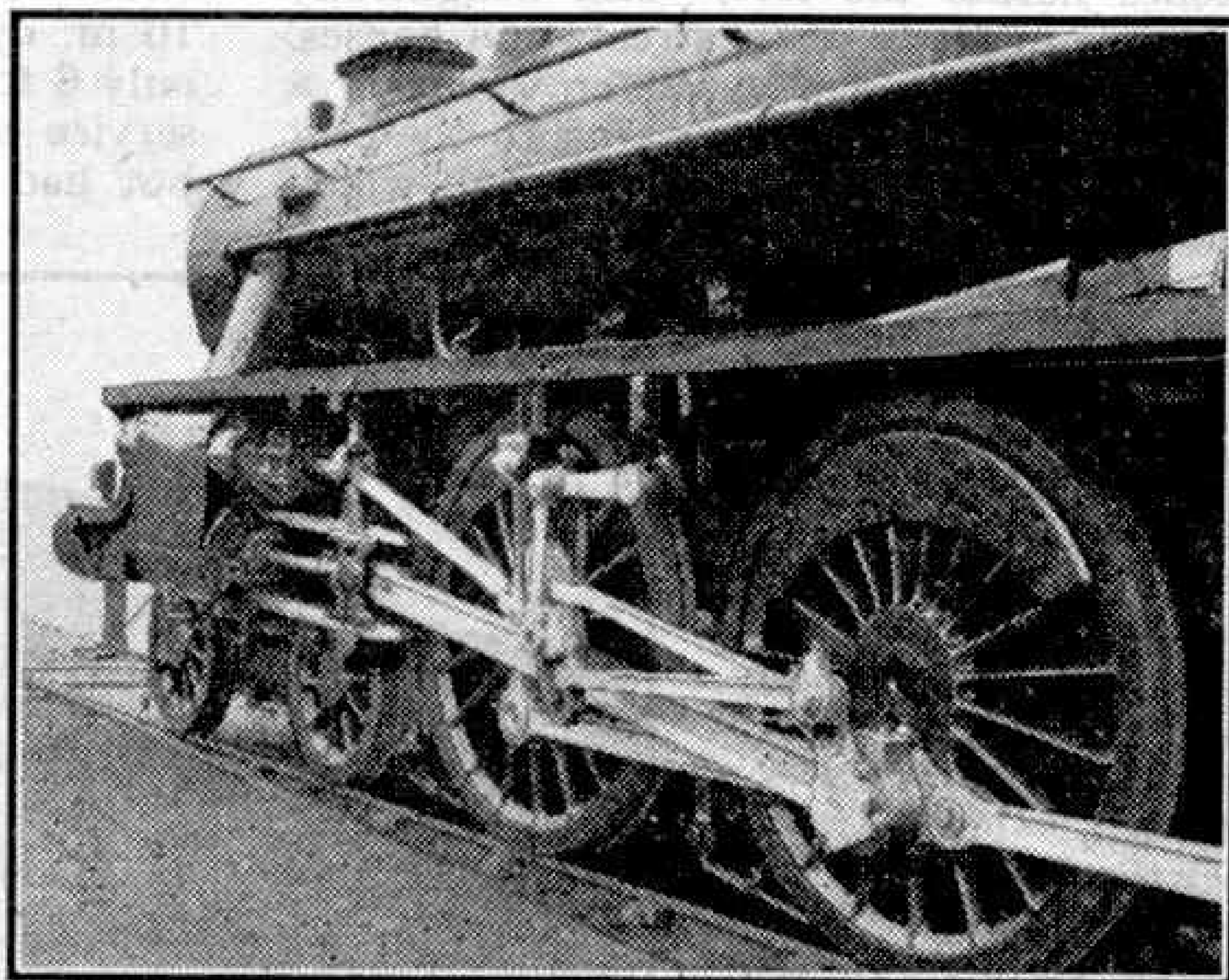
The outside Stephenson link motion applied experimentally to a London Midland 4-6-0. A double chimney and electric lighting are other special features.
