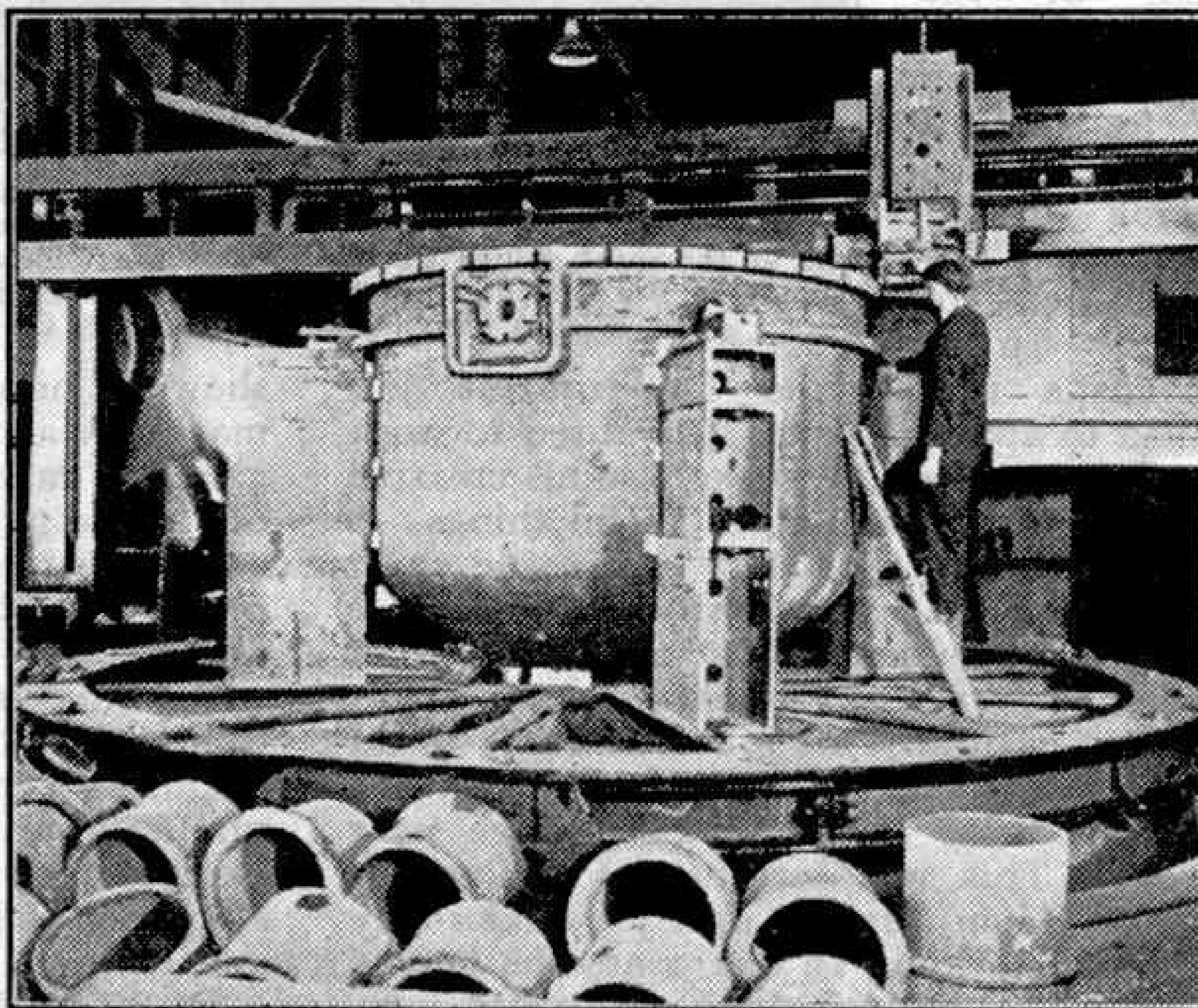
The body of a cast iron still being machined on a vertical boring machine. The table diameter of this machine is 21 ft.
