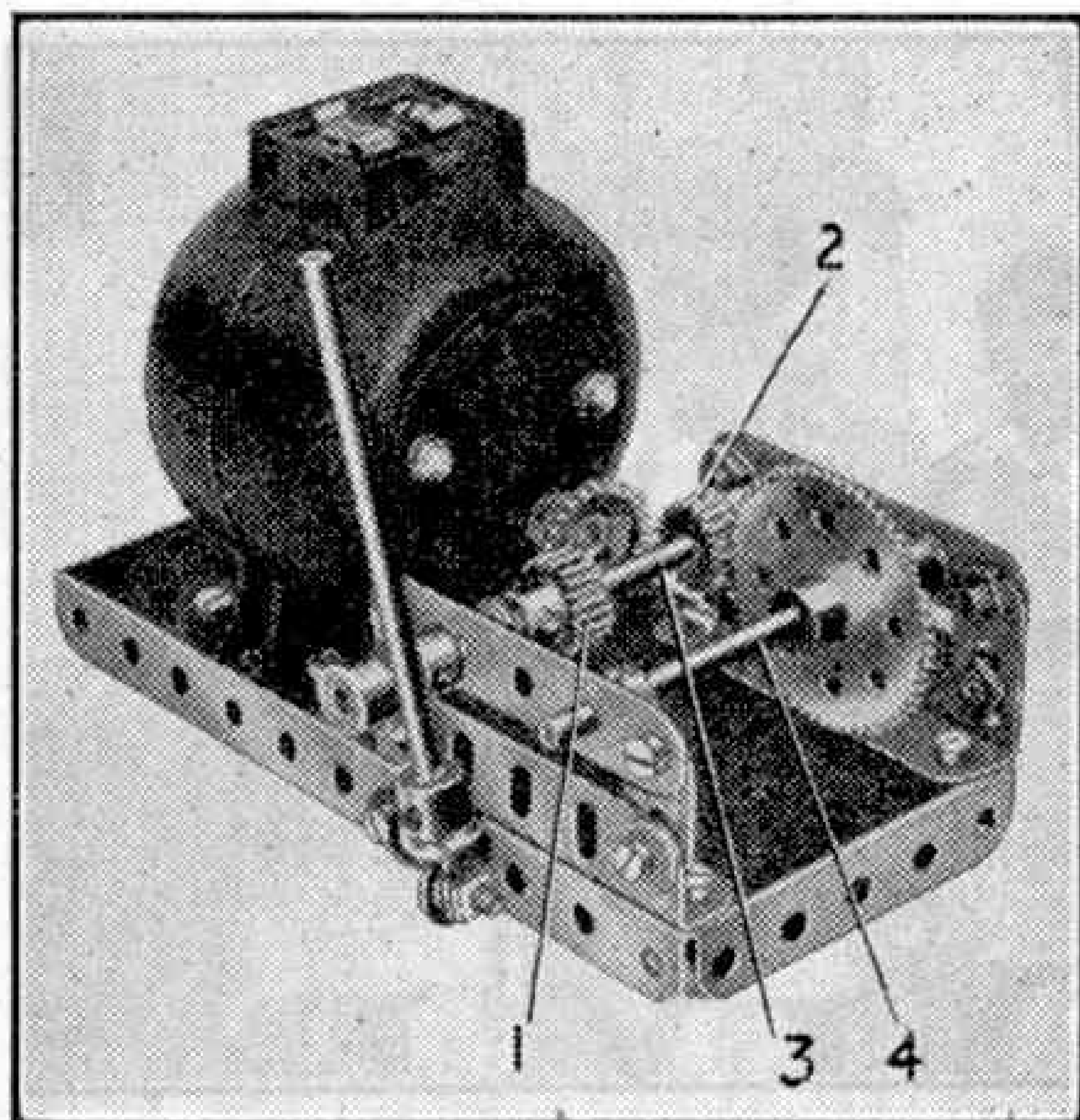
Fig. 1. A useful driving and reversing mechanism fitted to an E06 or E020 type Meccano Electric Motor.
