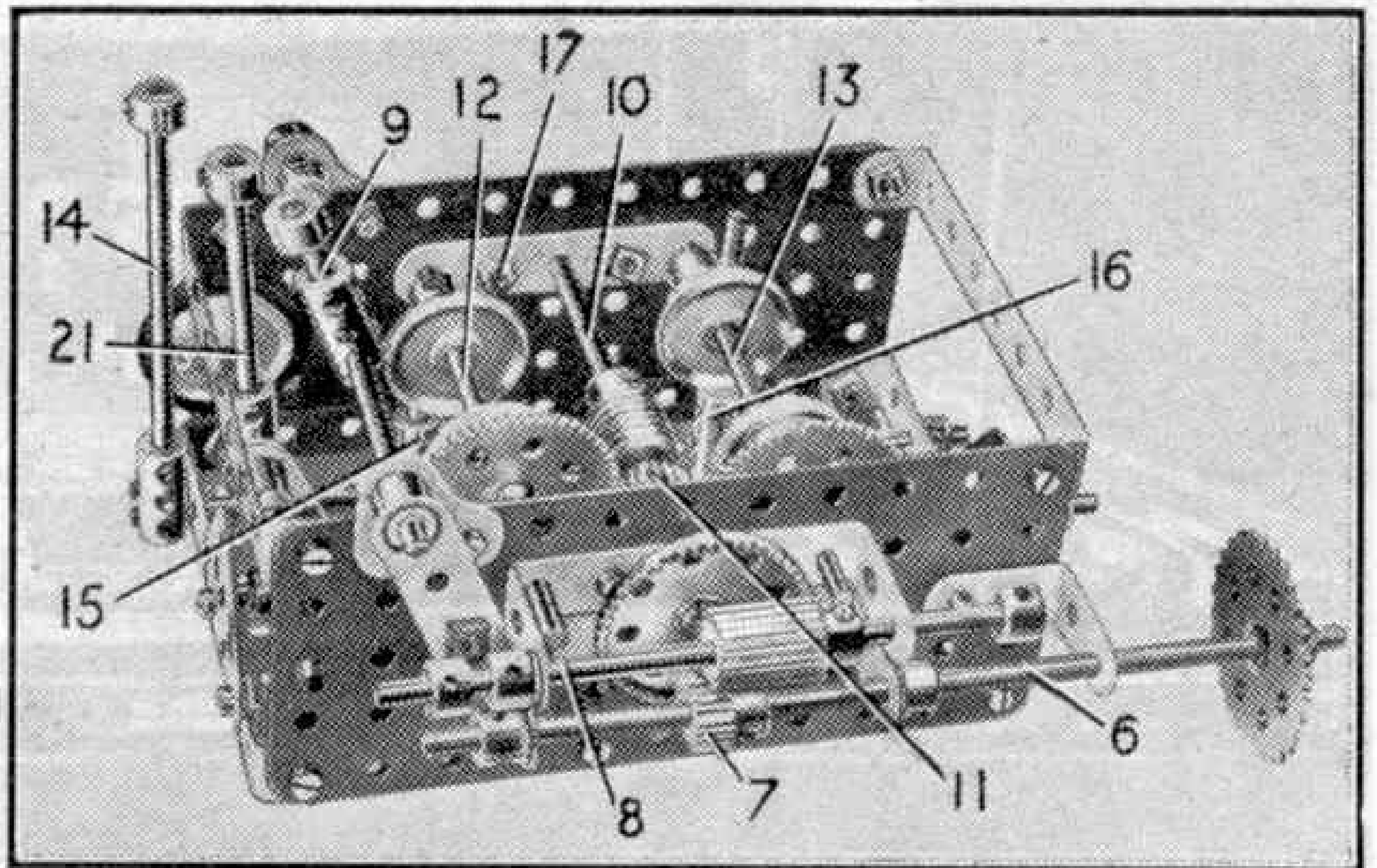
Fig. 3. The gear-box removed from the control cab.
