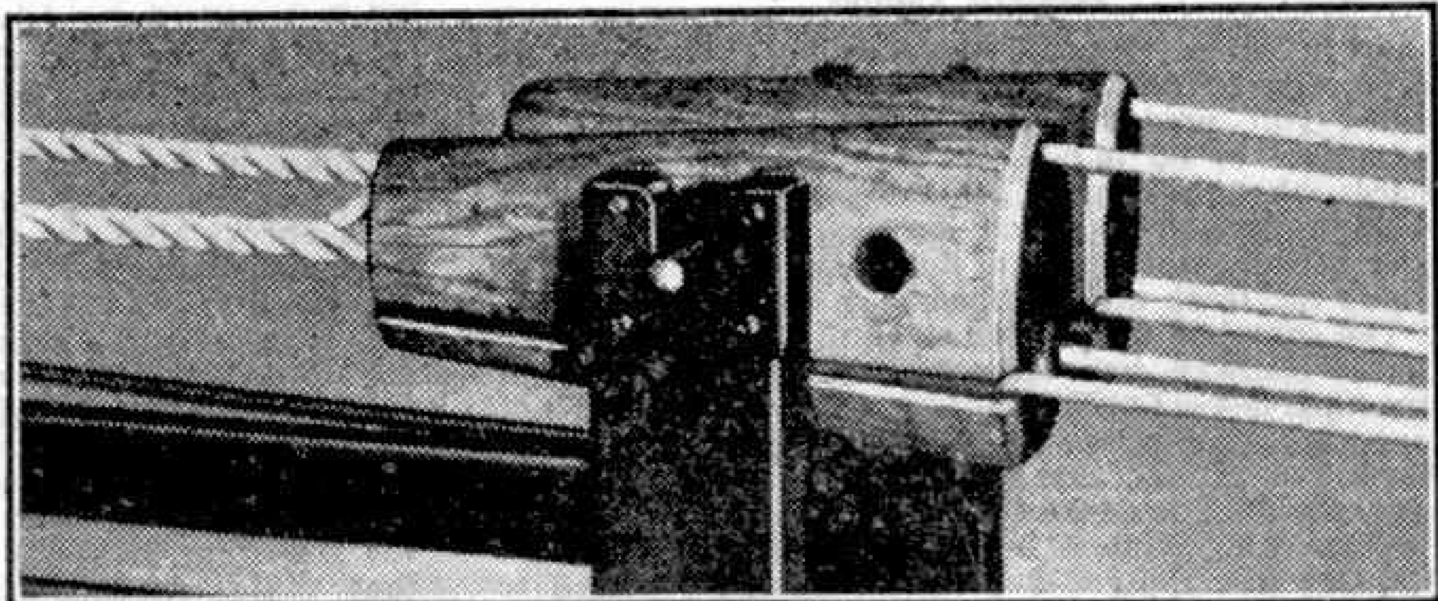
Laying a rope. The strands pass through grooves in a tapered piece of wood before being twisted together.
