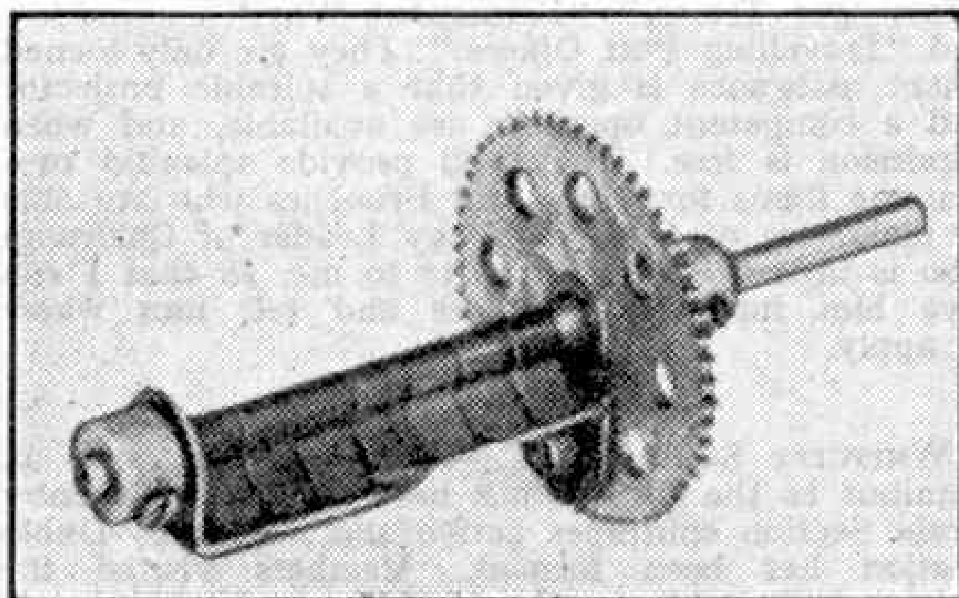
Fig. 2. A novel friction drive device designed by F/Lt. N. C. Ta'Bois, B.A.O.R., Germany, for use in the take-up spool drive of a cinematograph.
