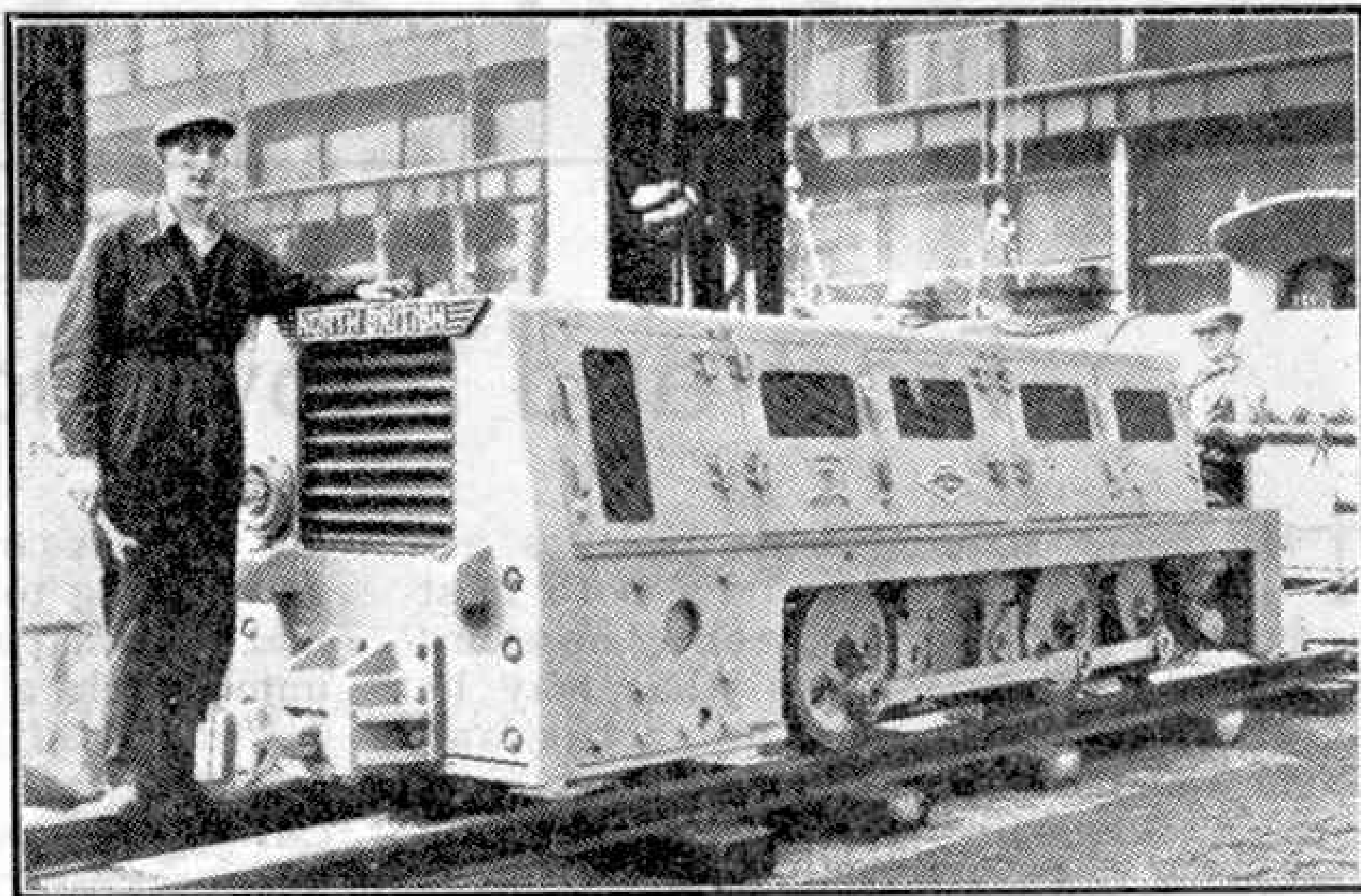
The "North British Miner," a 100 h.p. diesel mine locomotive designed and built by the North British Locomotive Co. Ltd., Glasgow, to whom we are indebted for the illustrations to this article.
