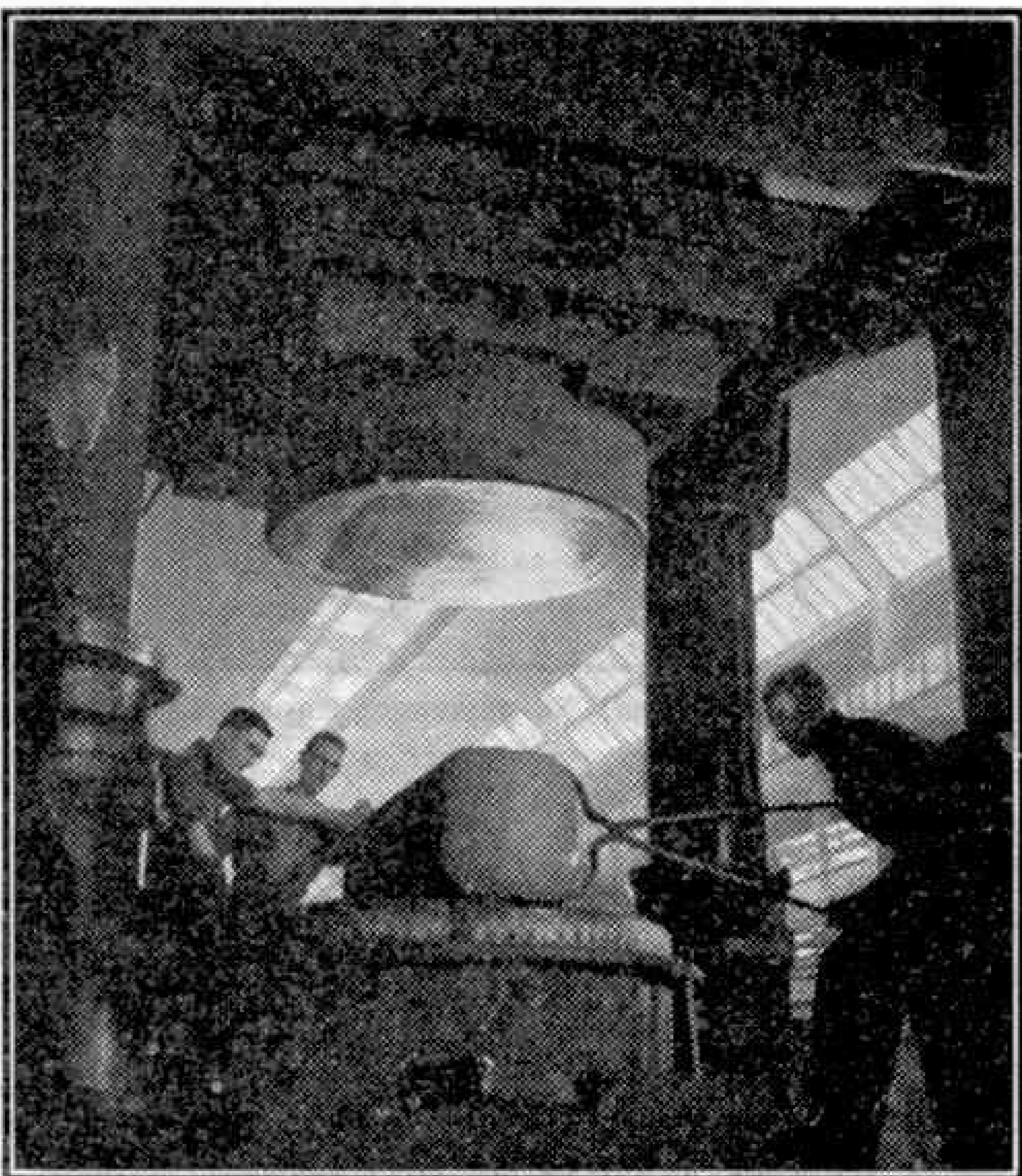
Pre-forging an ingot of "Hiduminium" alloy on a 3,000 ton Schloemann Press. This photograph and that on which our cover is based are by courtesy of High Duty Alloys Ltd.
