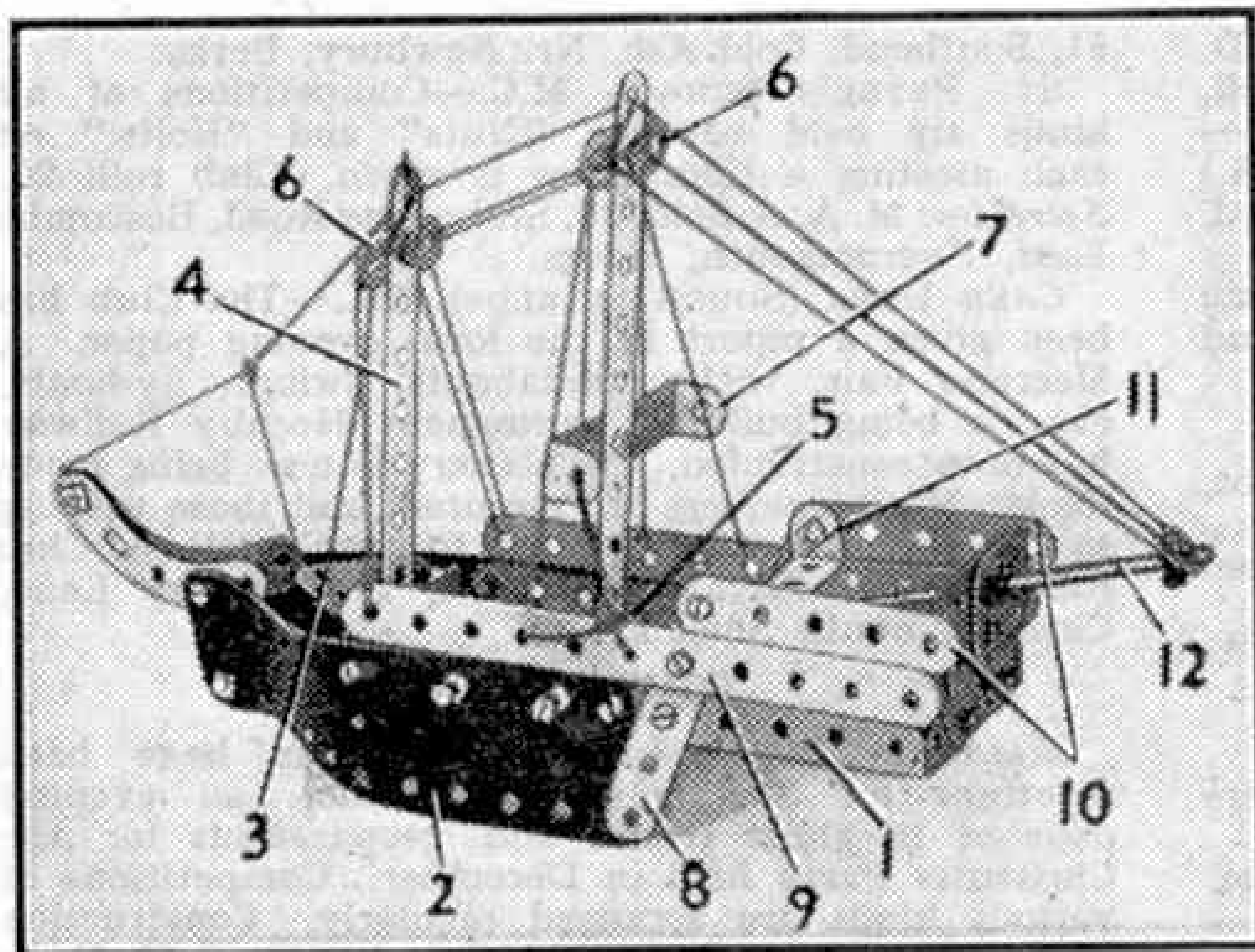
Fig. 3. A realistic galleon-type sailing ship. It can be built from parts in Outfit No. 1.
