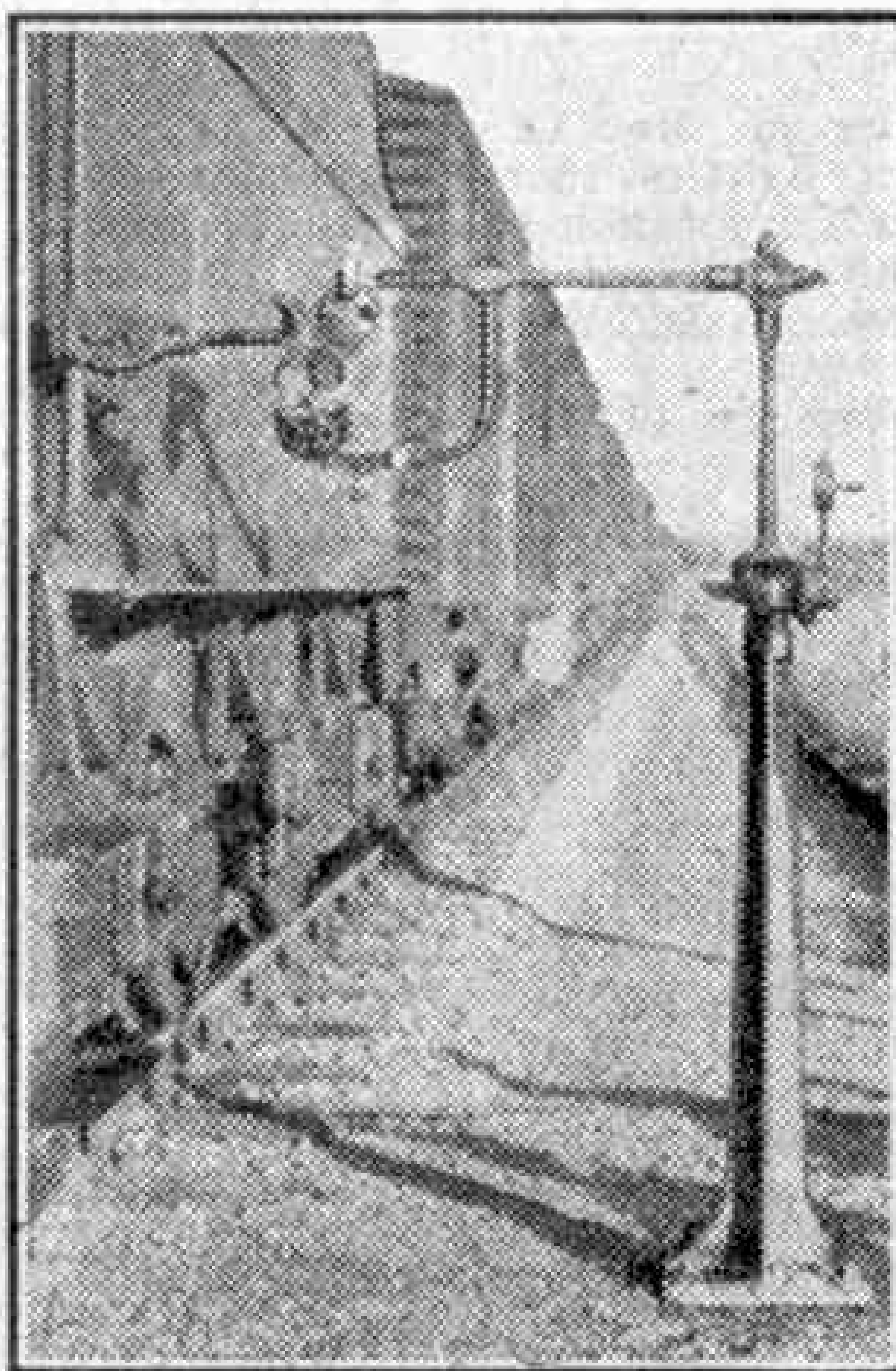
Mechanical exchange of tablets on the Somerset and Dorset line.
