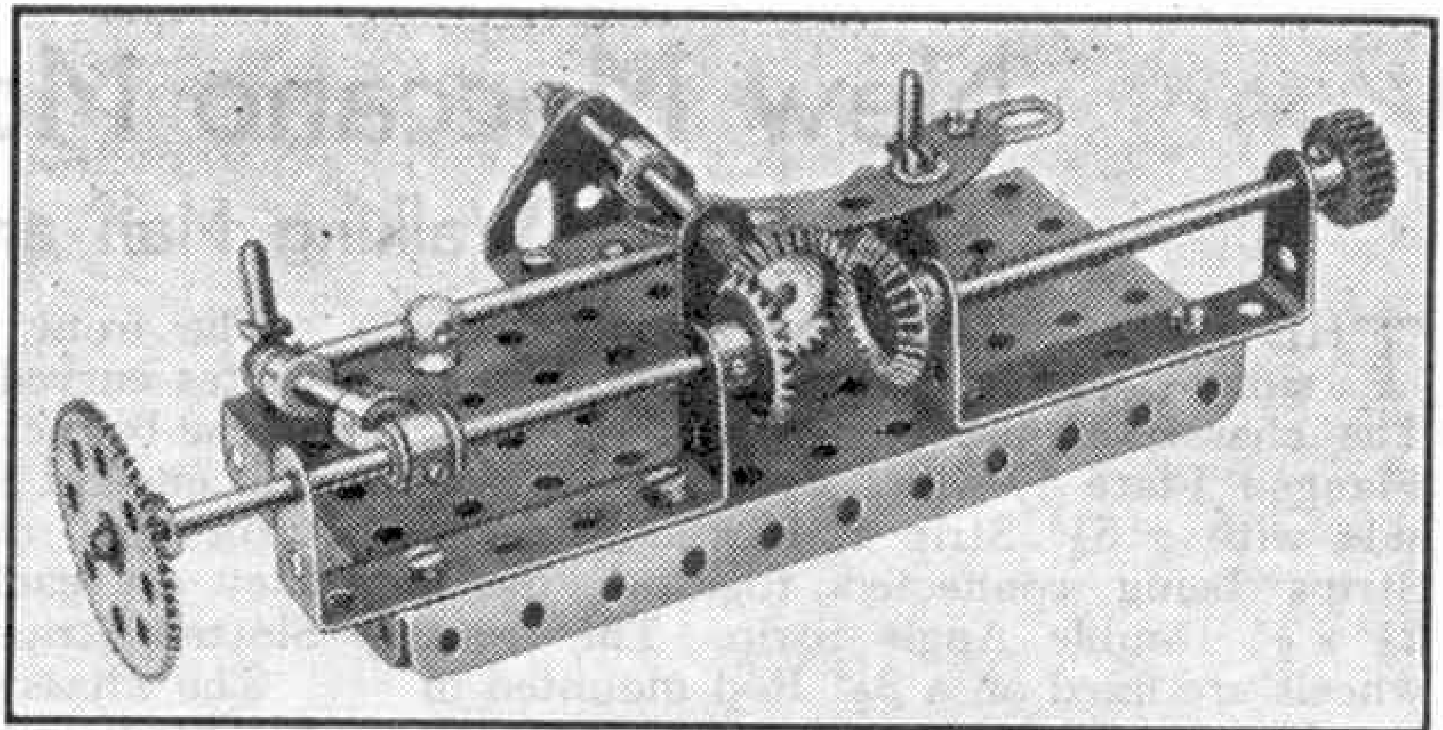
Fig. 2. The reversing mechanism designed by N. C. Ta'Bois, which is described in these pages. The illustration shows the gears in the reverse drive position.
