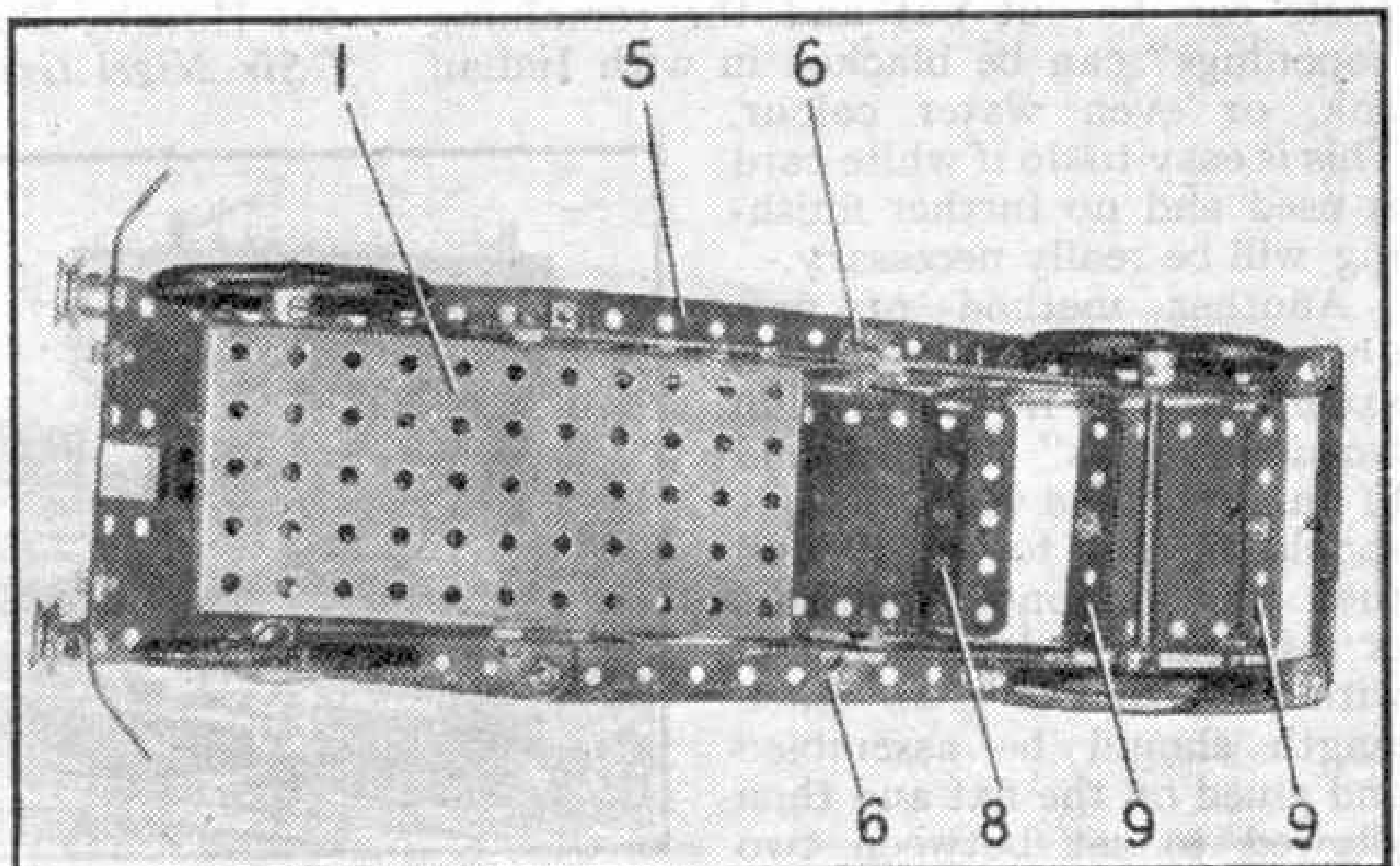
Fig. 3. An underneath view of the chassis of the car seen in Fig. 1.
