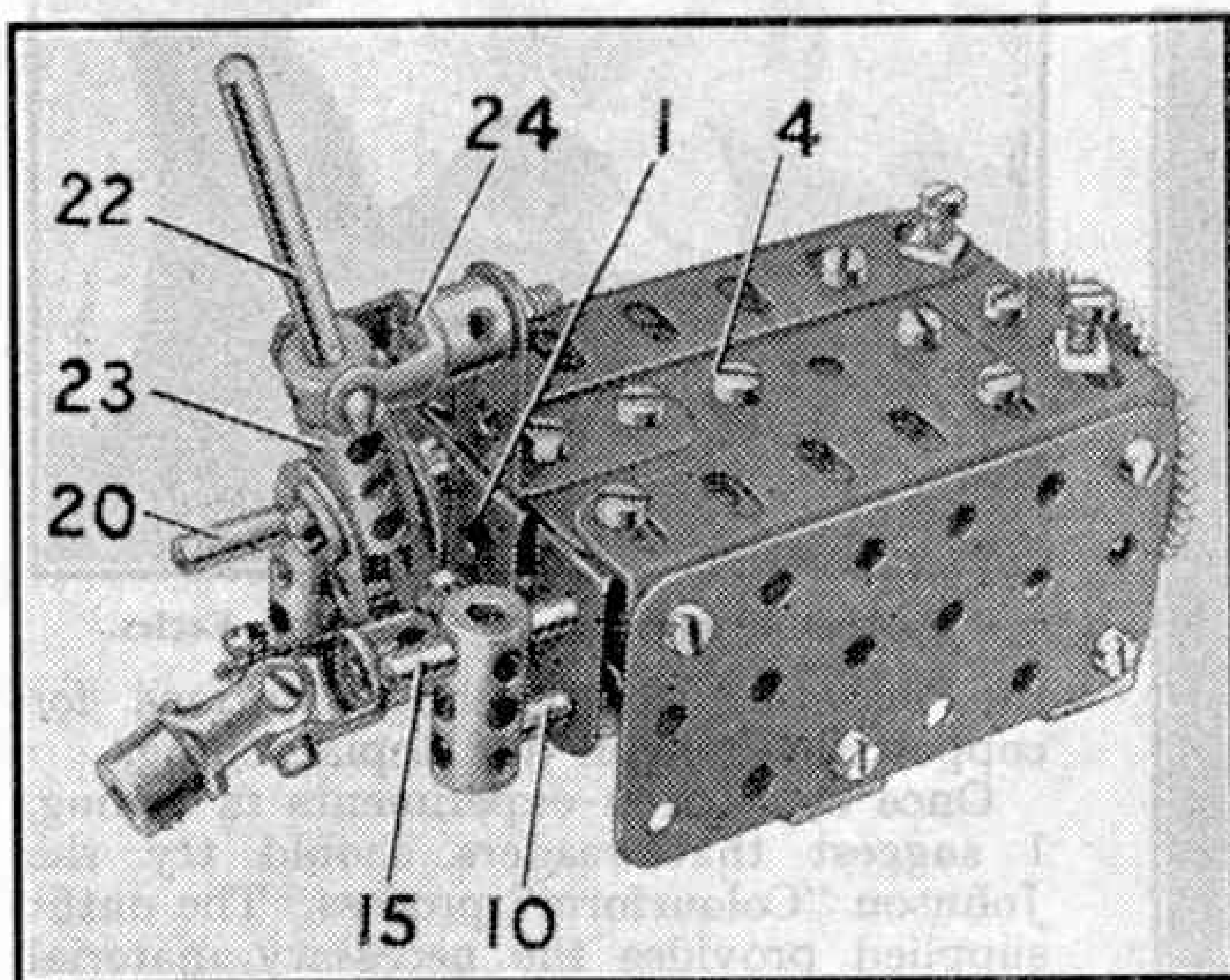
Fig. 1. A compact three-speed and reverse gear-box.
