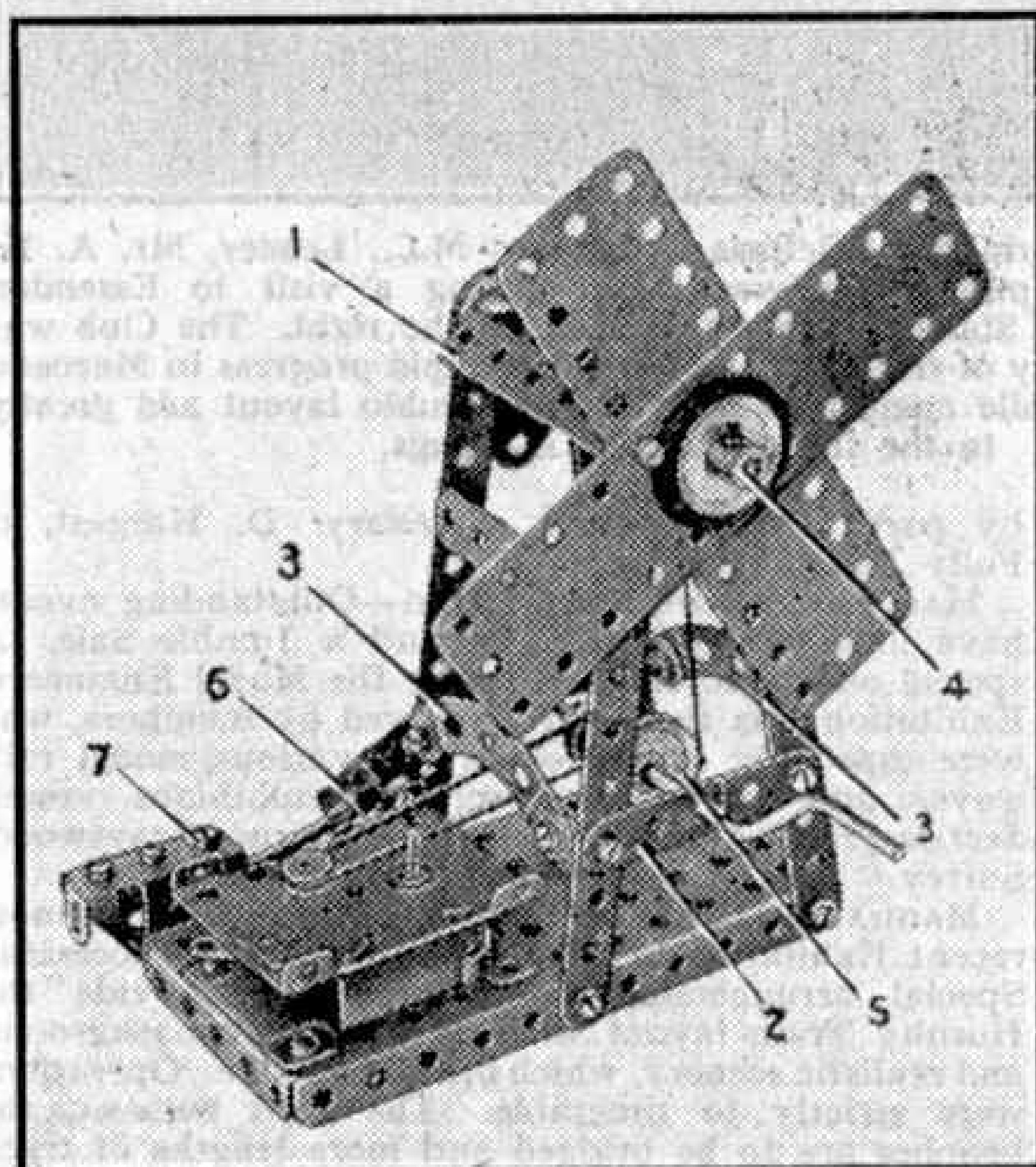
Fig. 4. A simple model windmill pump fitted with a Magic Motor.
