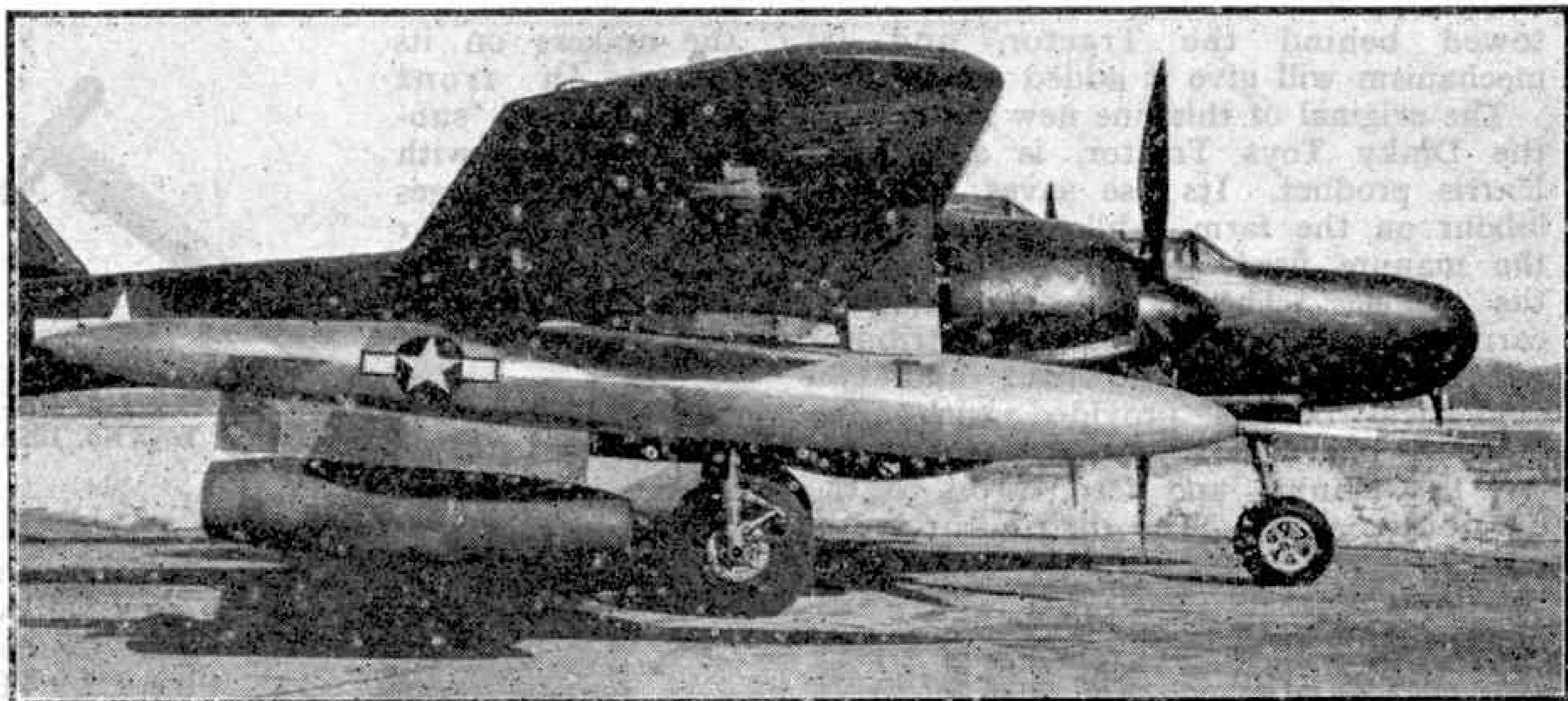
"Gorgon" missile in launching position, under the wing of a "Black Widow" night fighter. Photograph by courtesy of Glenn L. Martin Company, U.S.A.
