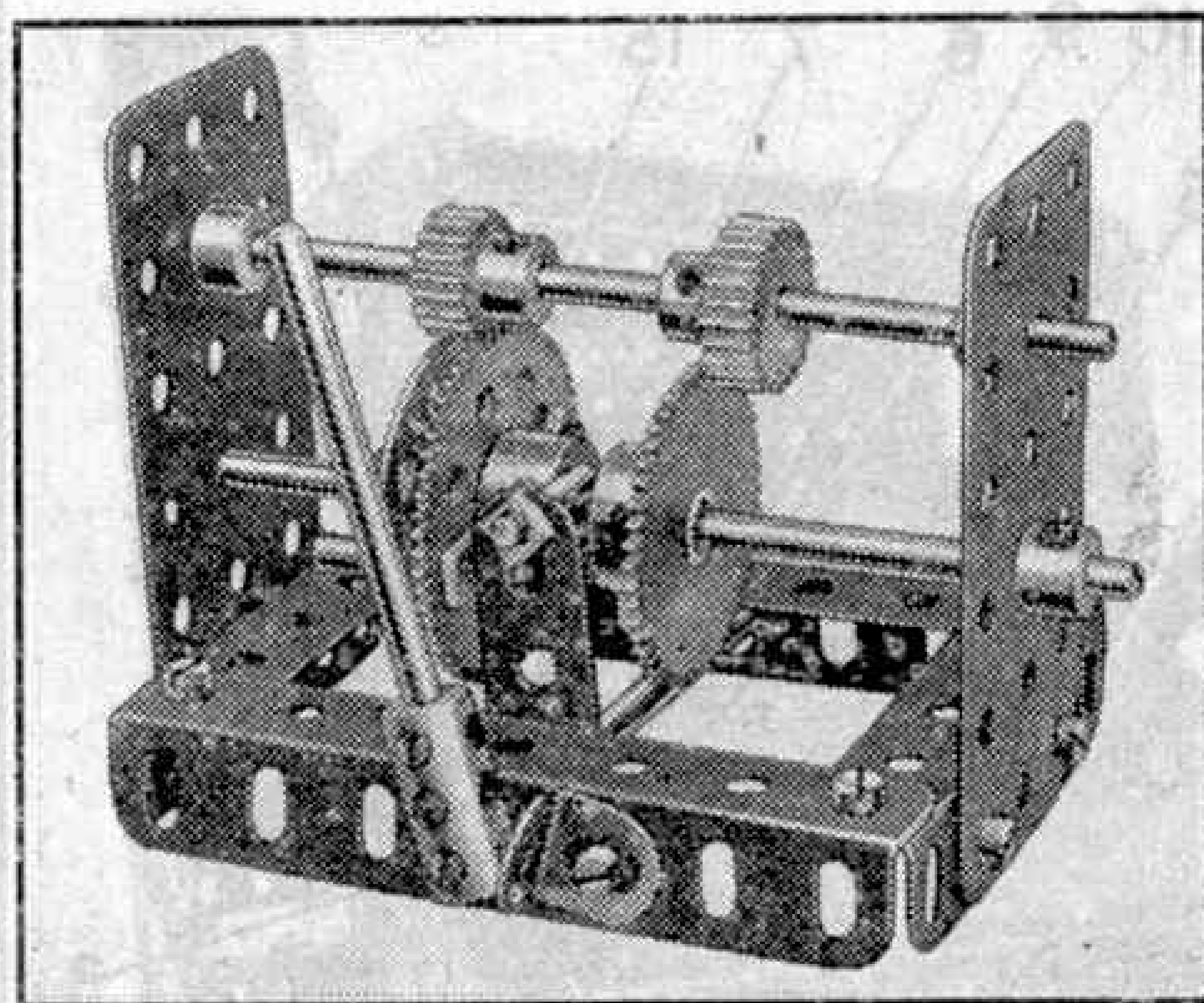
Fig. 4. A sliding change gear unit built up with the aid of a Socket Coupling.
