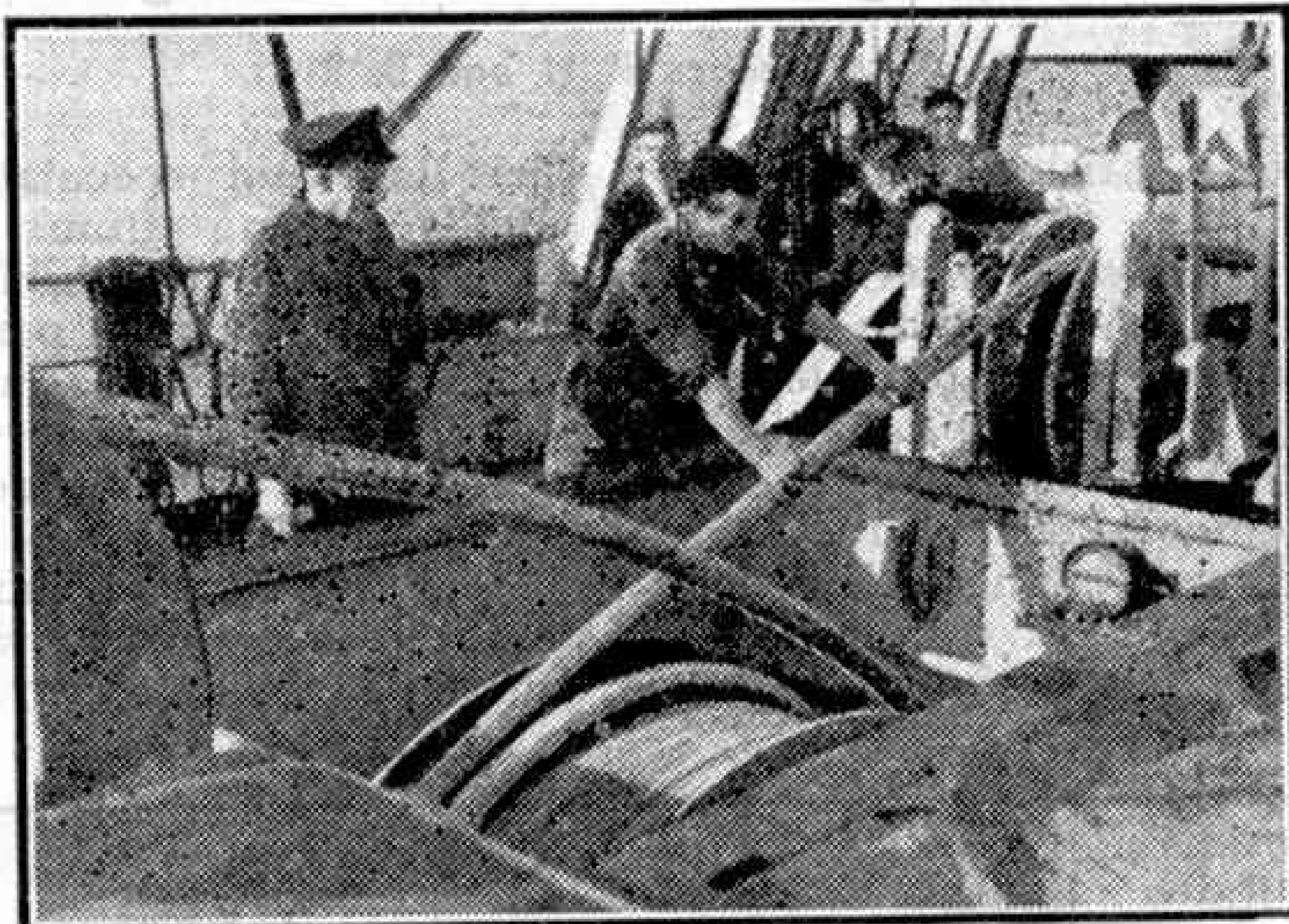
Paying out a cable between Great Britain and Holland from the " Alert ," of the Post Office cable-laying fleet.
