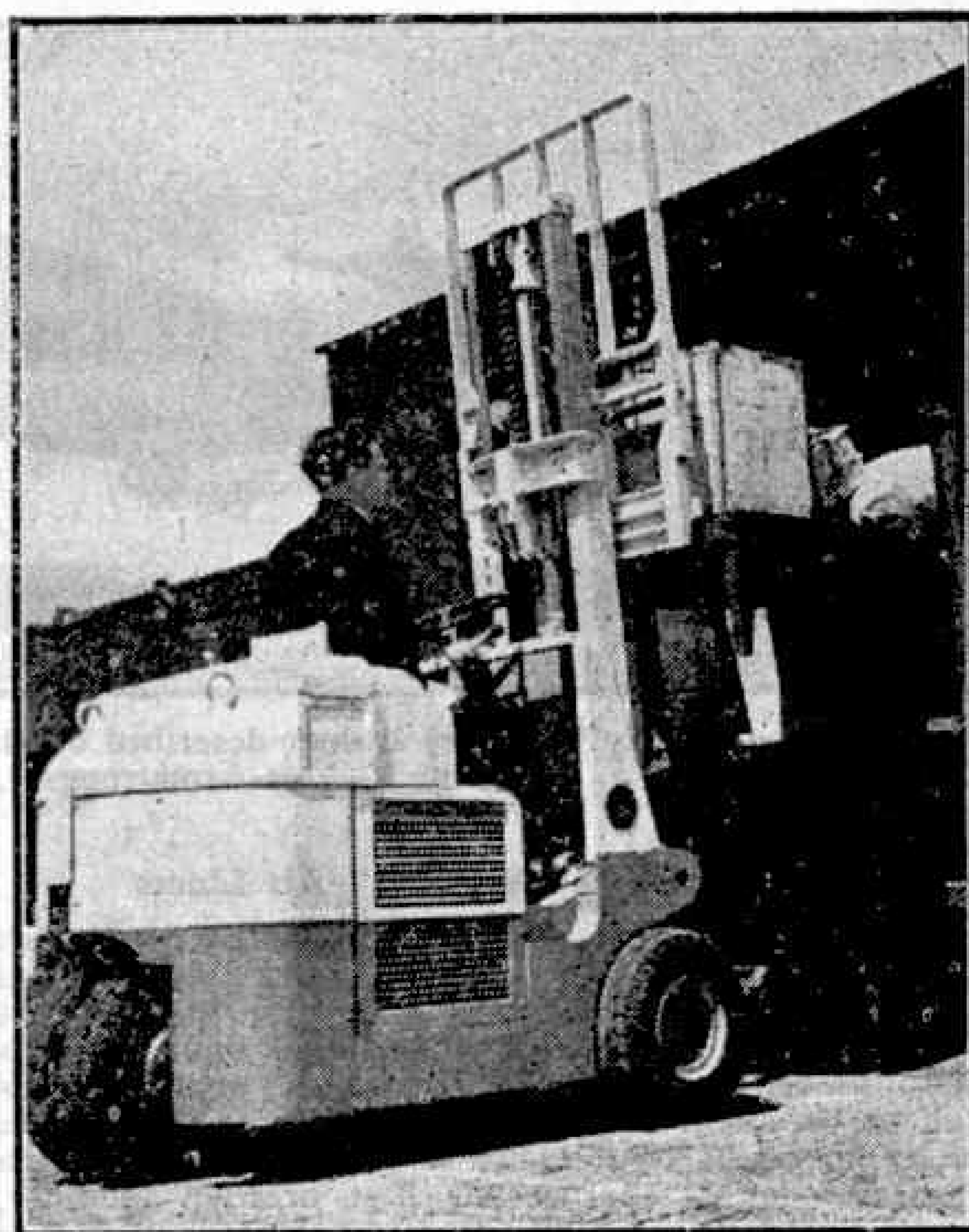
Loads can be placed inside a railway van, or taken out of it, by the fork lift truck.
