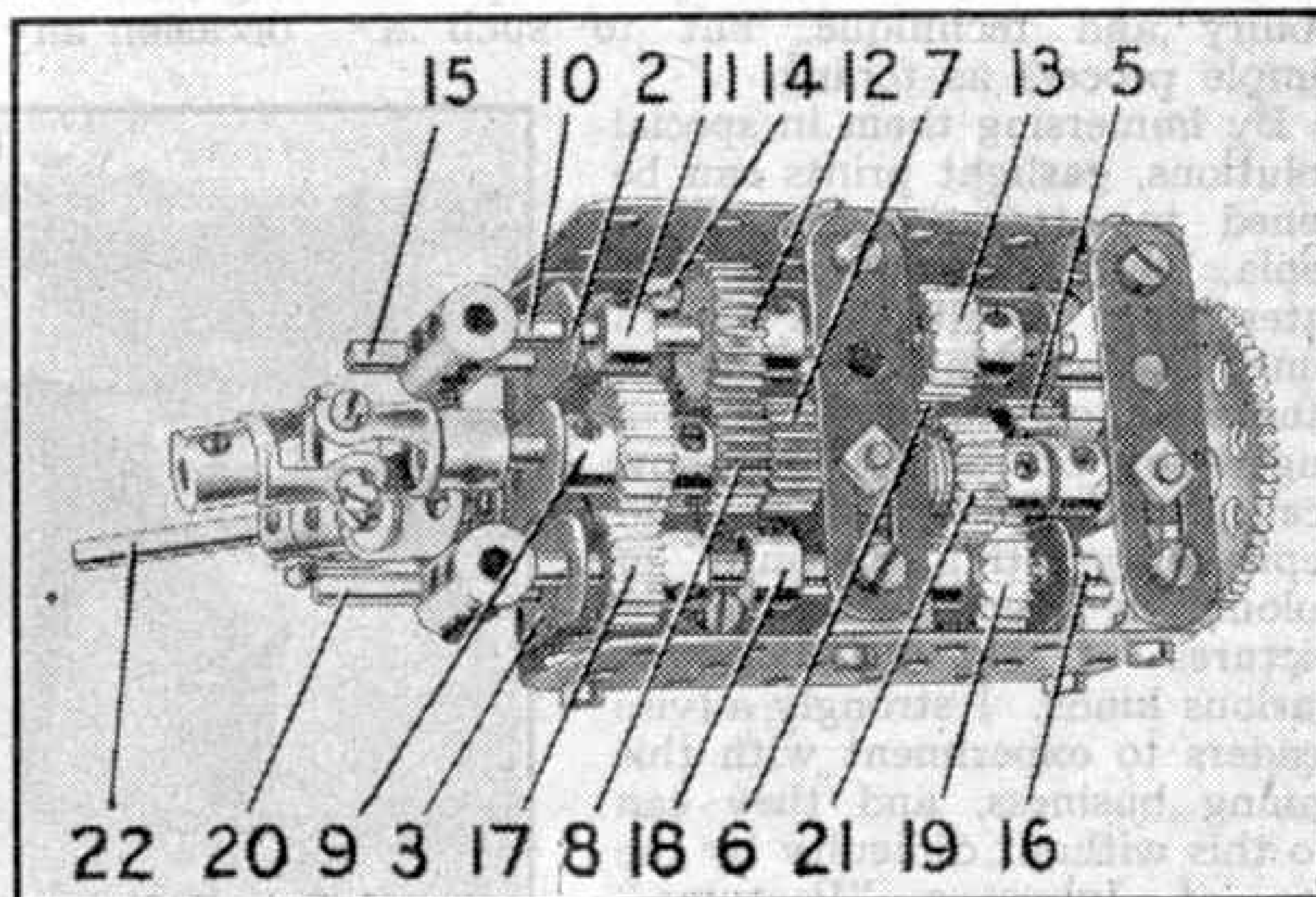
Fig. 2. The inside of the gear-box.
