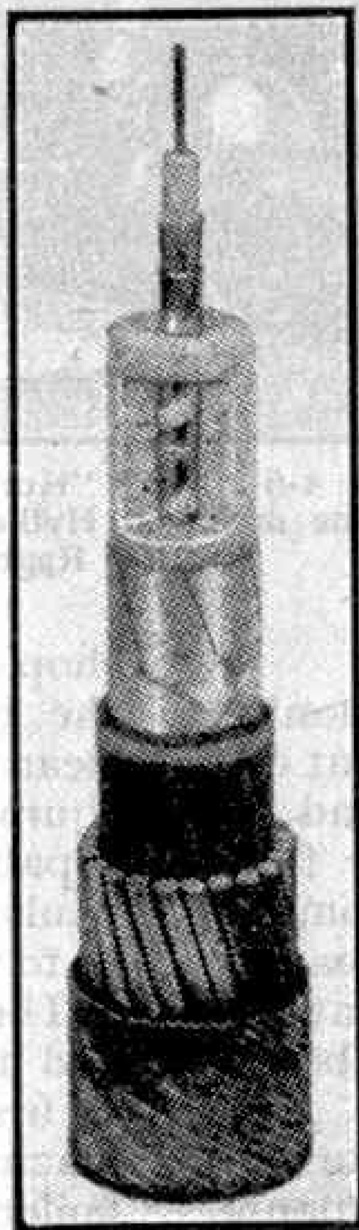
Section of the Anglo-Dutch cable laid in December 1947, showing the insulation and protection.
