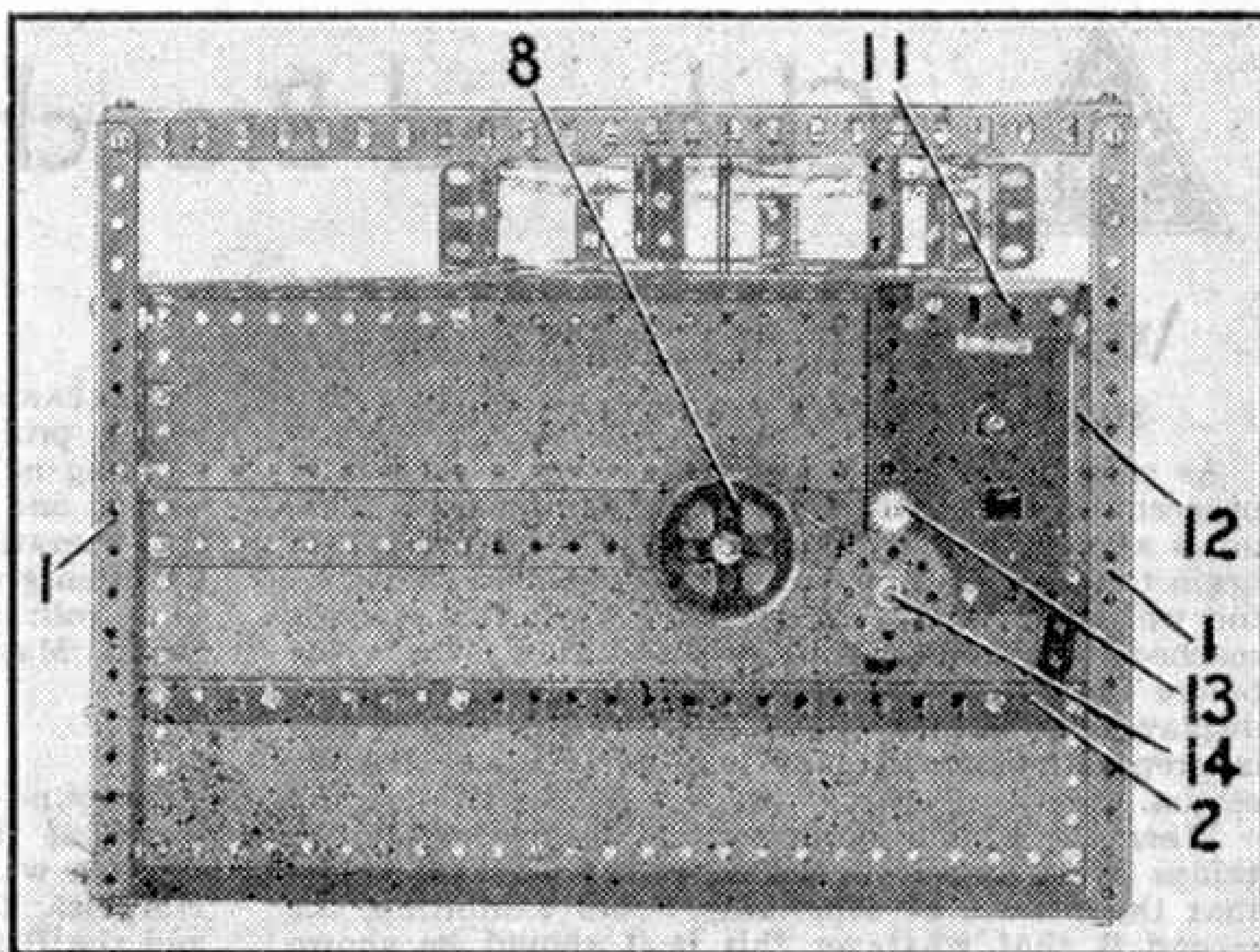
Fig. 3. An underneath view of the mill showing how the Motor drive is arranged.
