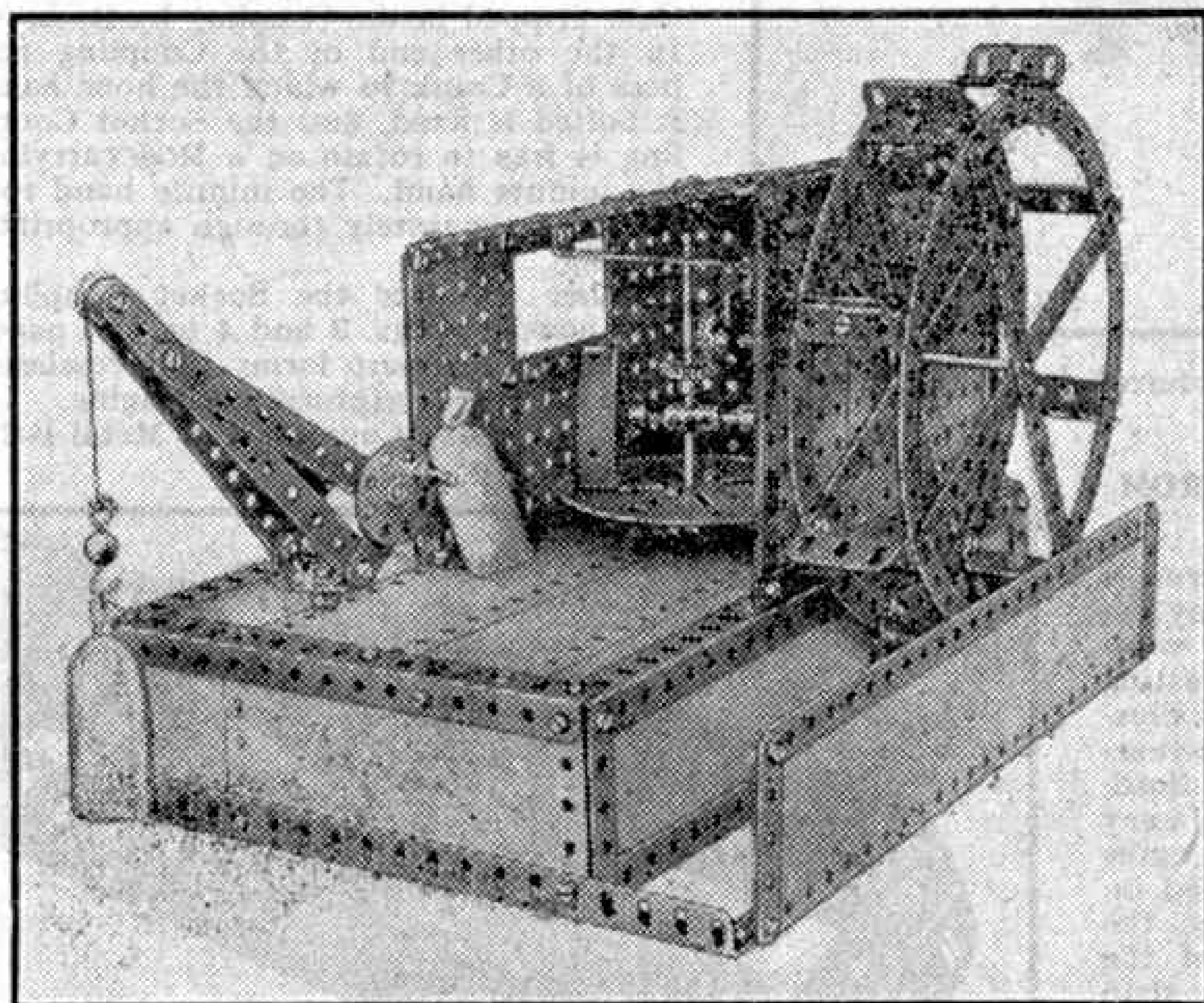
Fig. 1. A model water-wheel mill driven by a No. 1 Clockwork Motor.
