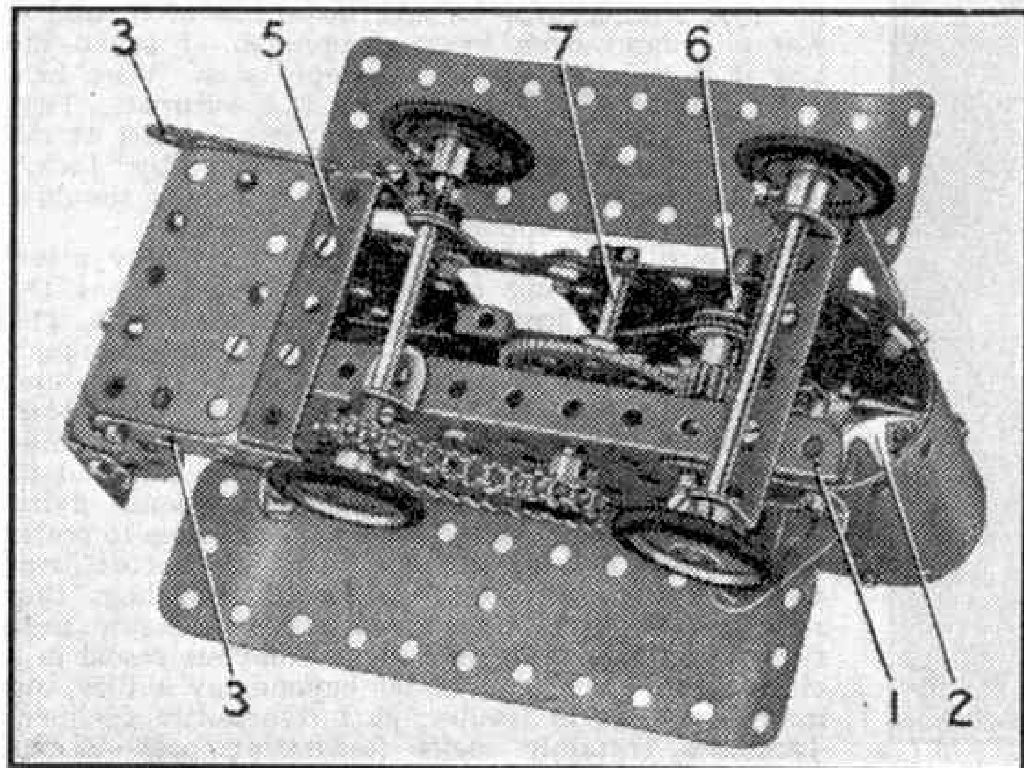
Fig. 2. Underneath view of the tractor.
