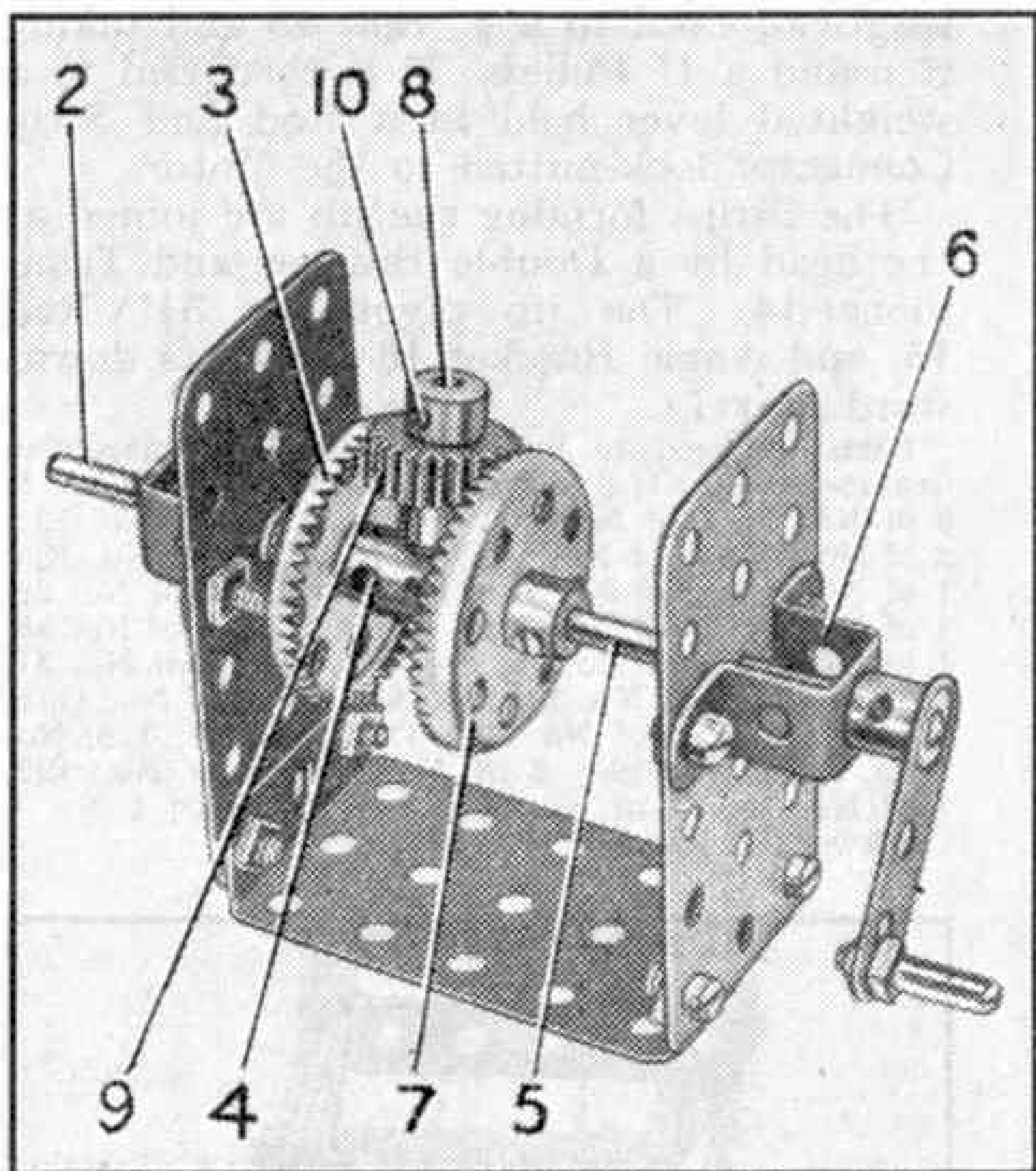
Fig. 1. Compact epicyclic transmission gearing.
