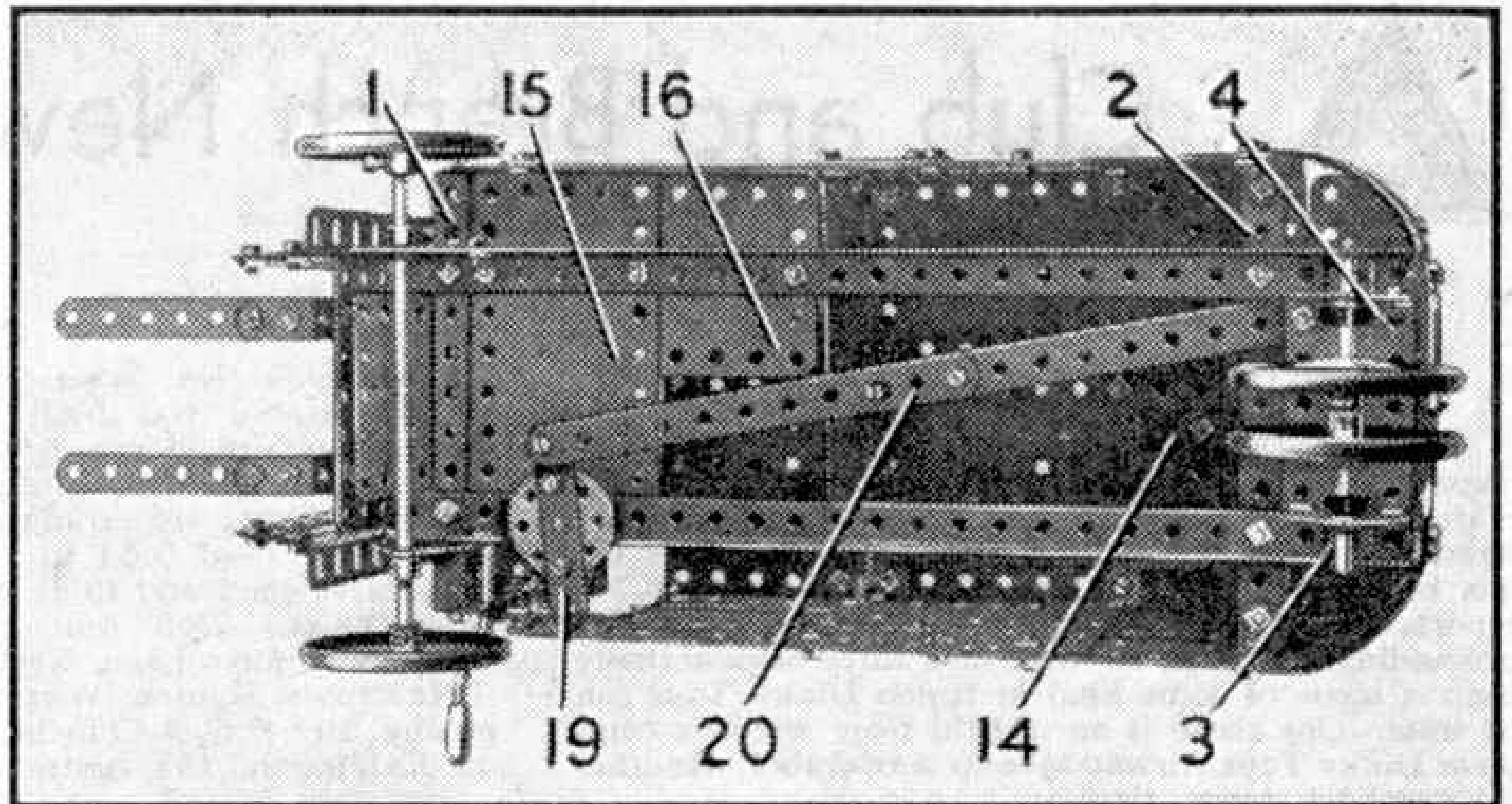
Fig. 2. Underneath view of truck.
