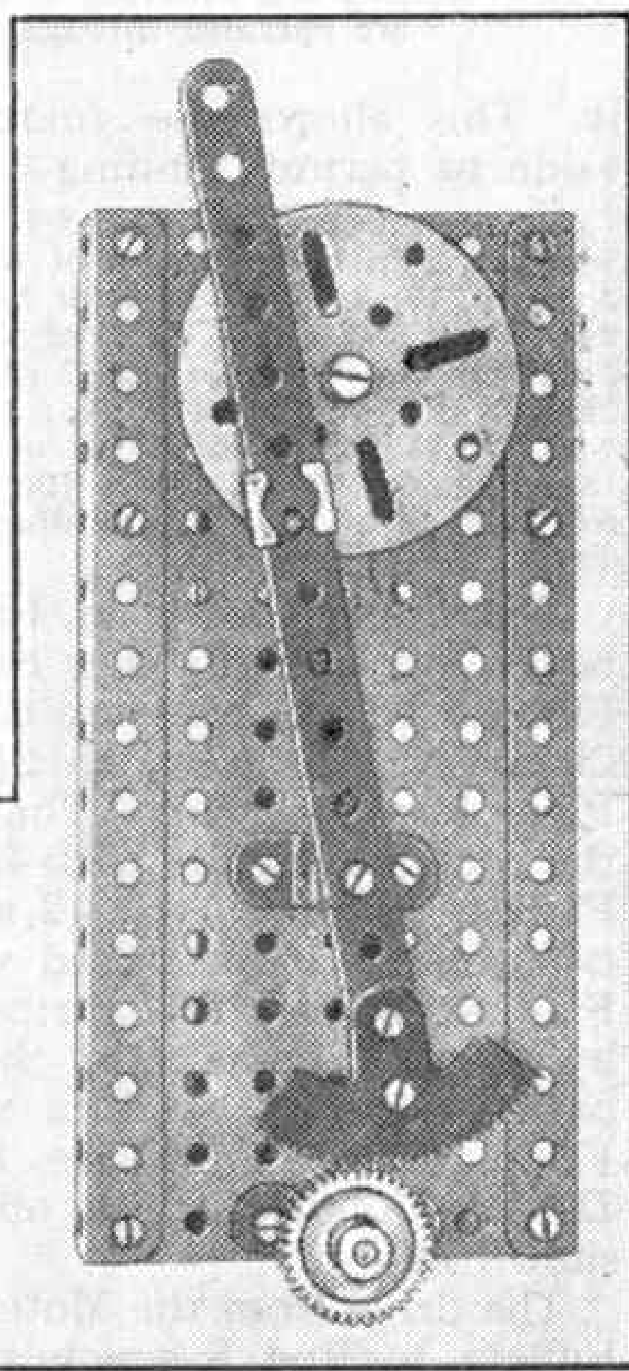
Fig. 2. A Meccano Toothed Segment used to rotate a shaft through part of a revolution.
