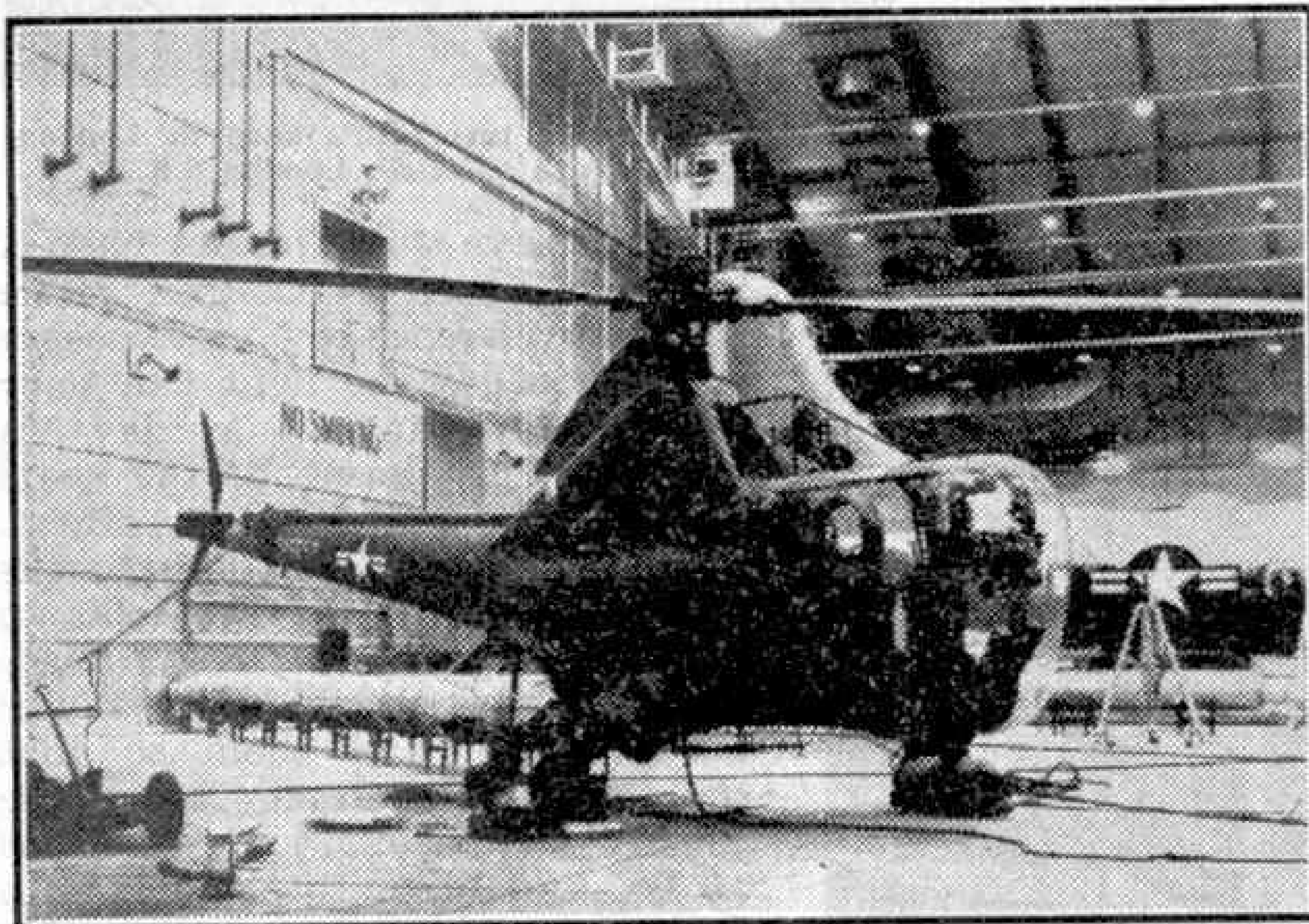
Sikorsky H5G helicopter undergoing climatic tests in the U.S.A.F.'s Climatic Hangar at Eglin Air Force Base, Florida. The illustrations to this article are reproduced by courtesy of the U.S. Air Force, Washington.
