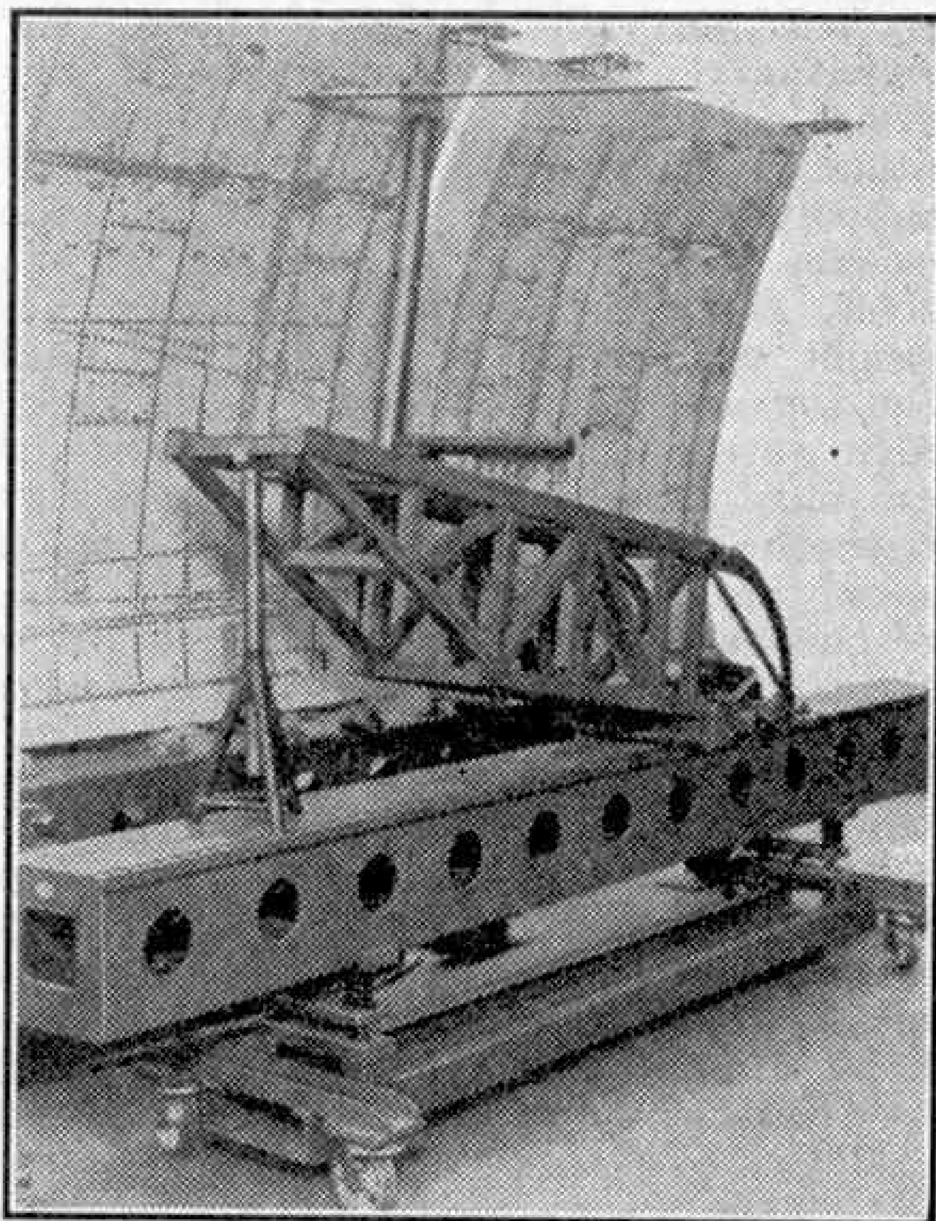
Machine for lofting on curved surface, showing the tower at low angle with jack and scribe in position. The illustrations to this article are reproduced by courtesy of The Fairey Aviation Co. Ltd.
