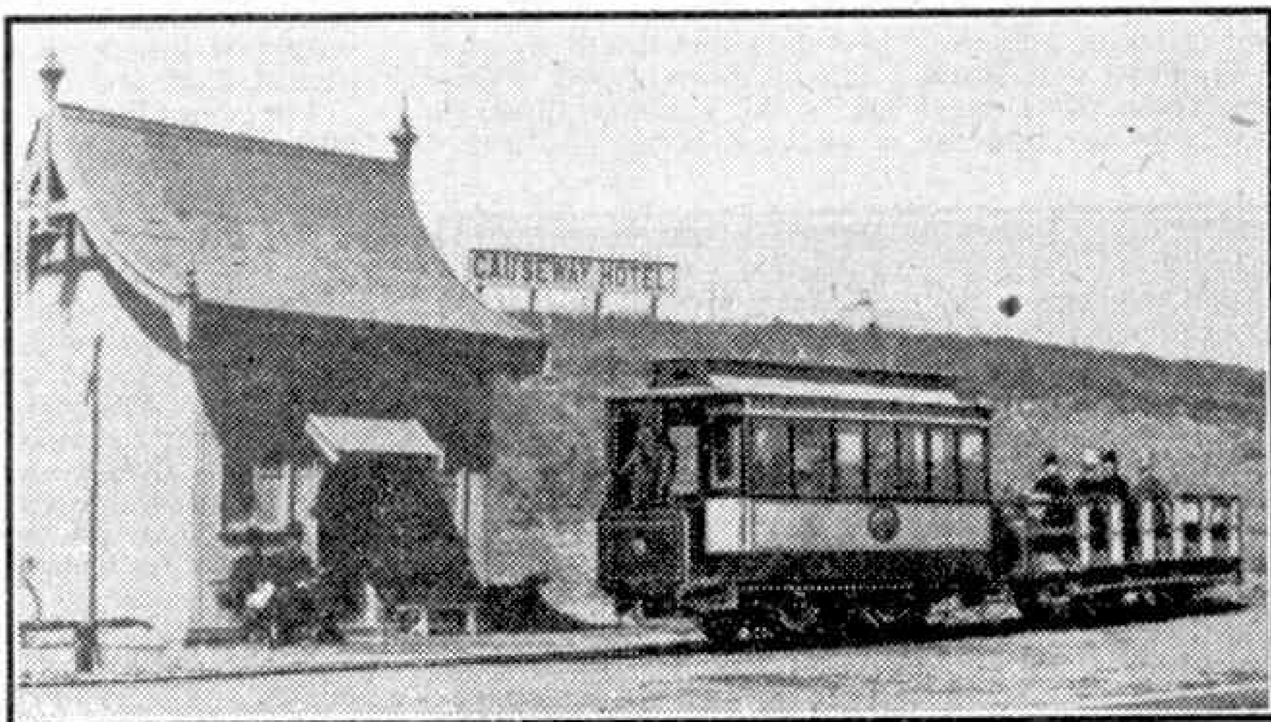
Causeway Hotel terminus, showing an original motor car, No. 9. On the left is one end of the side conductor rail.
