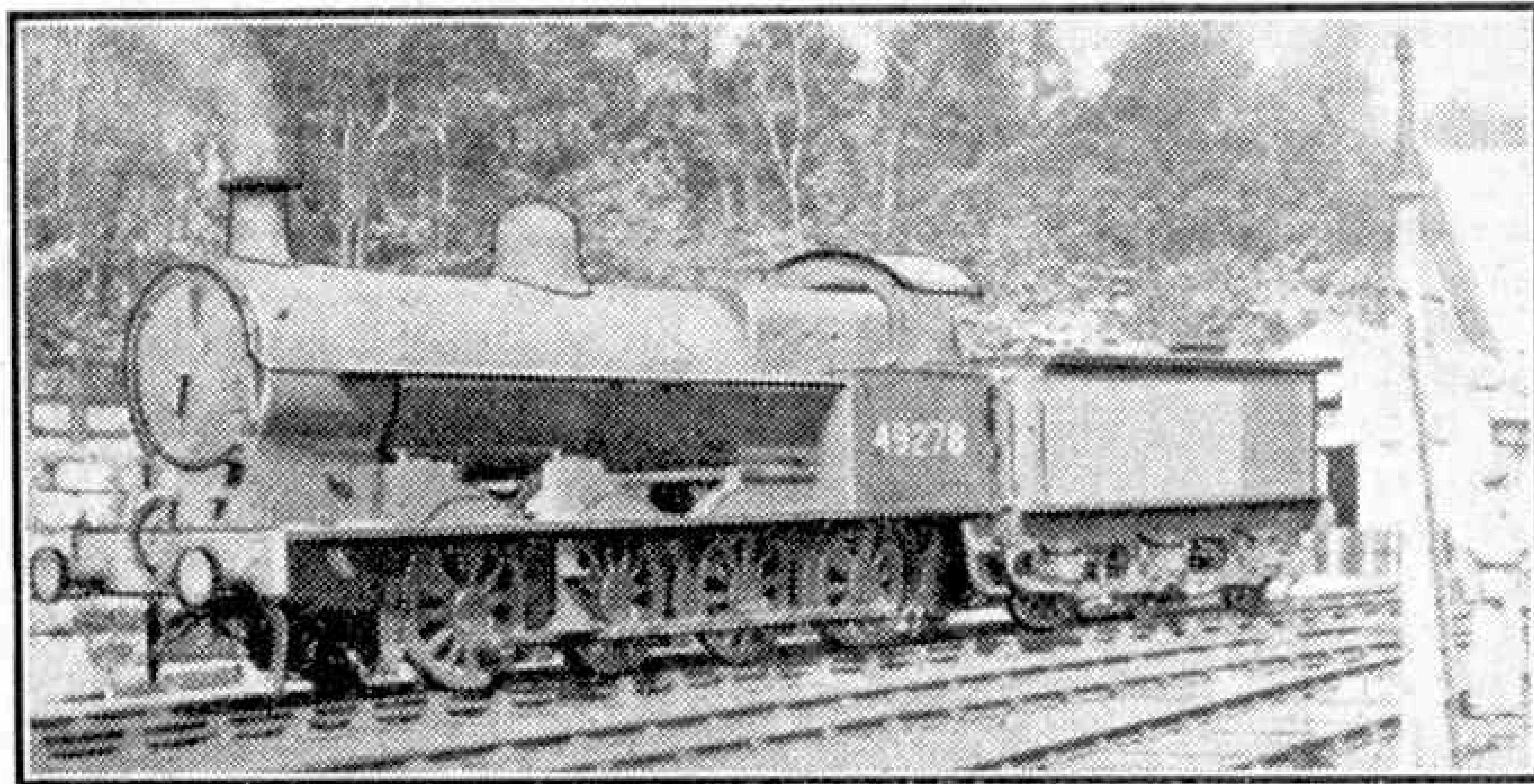
L.M.R. No. 49278, one of the numerous and well known "Super D" 0-8-0 engines of the former L.N.W.R. Photograph by D. W. Backhouse.
