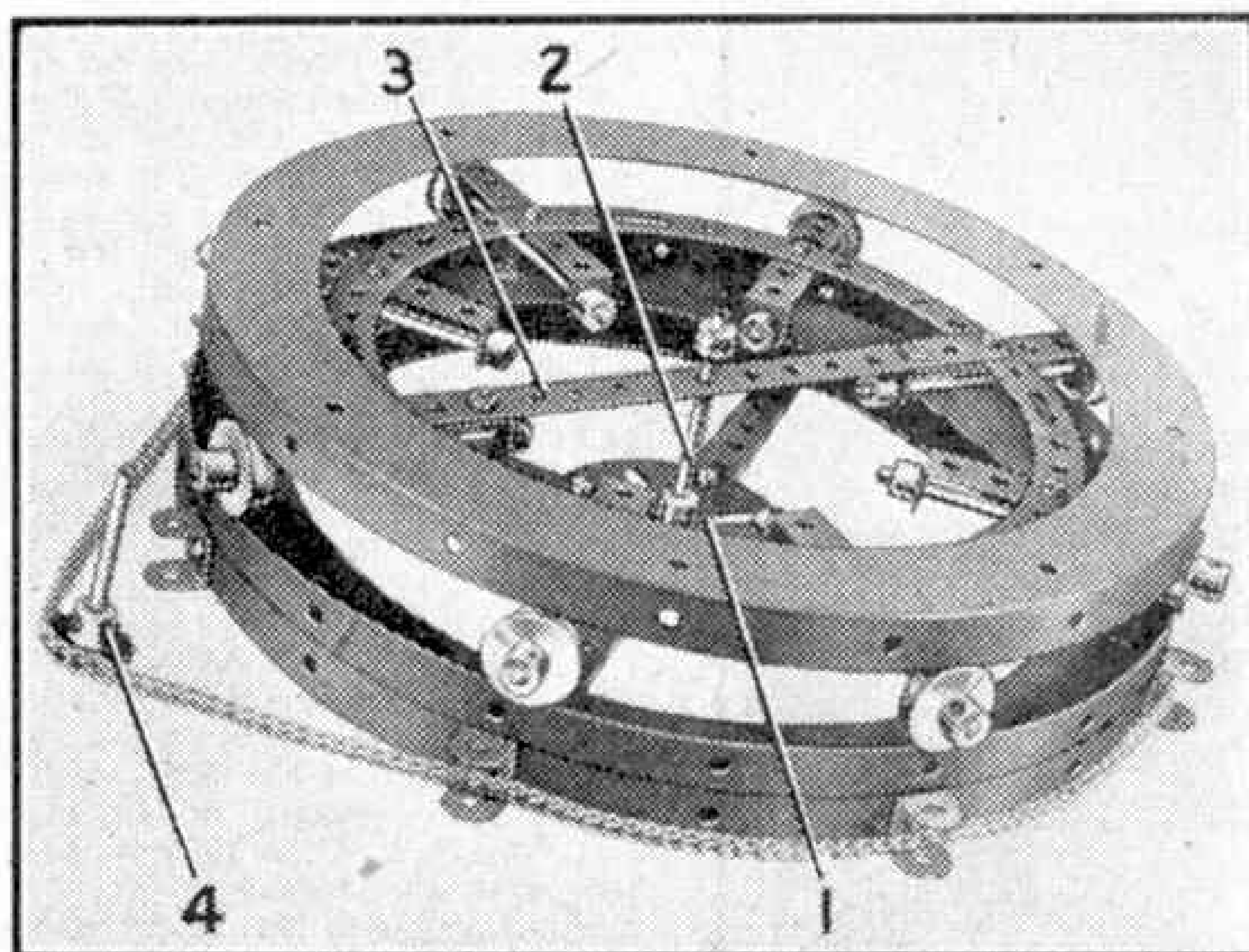
Fig. 2. An arrangement for a large built up roller type bearing. A device of this kind is suitable for use in large hammerhead and blocksetting cranes.
