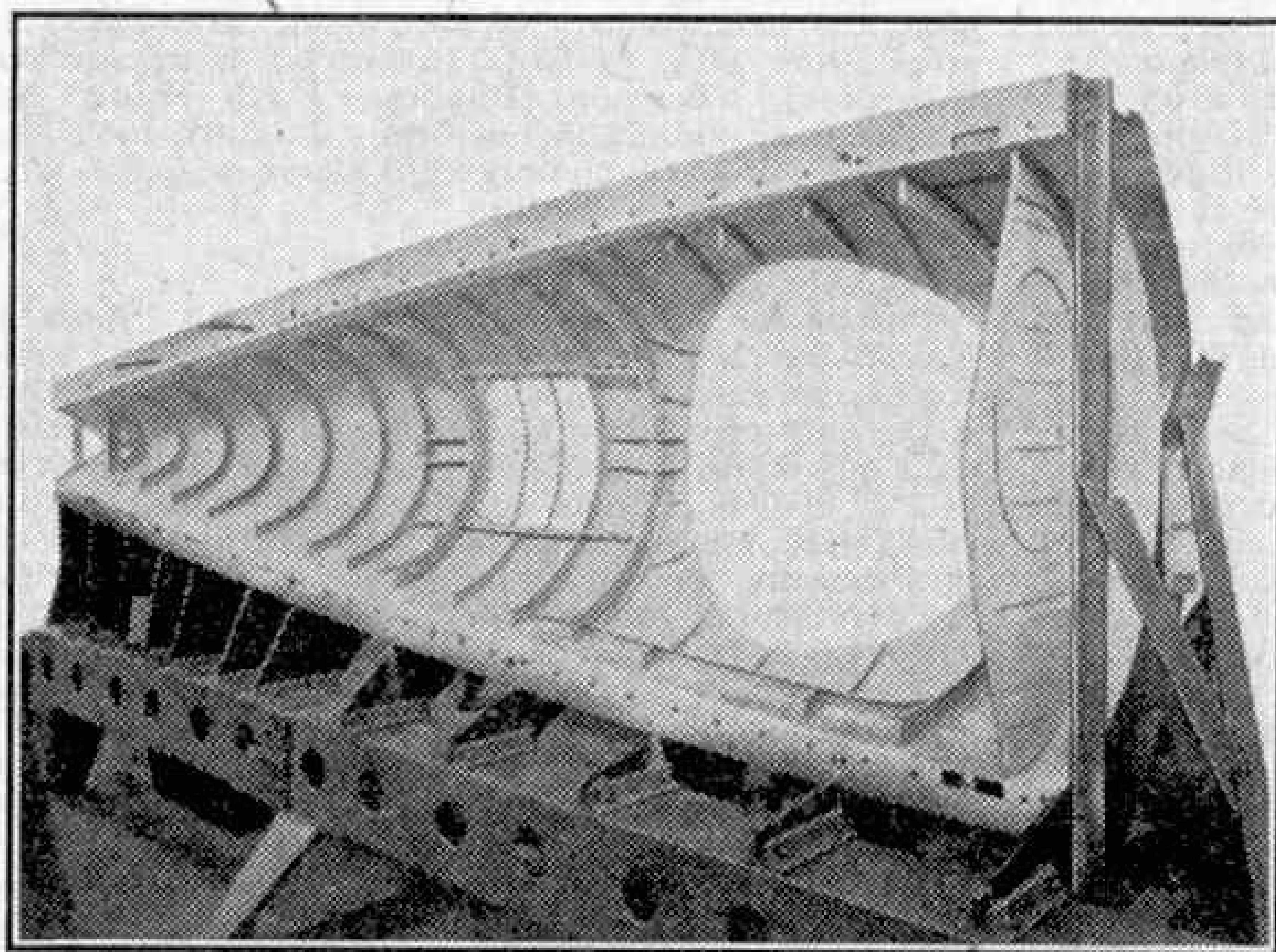
Completed fuselage panel in the jig.
