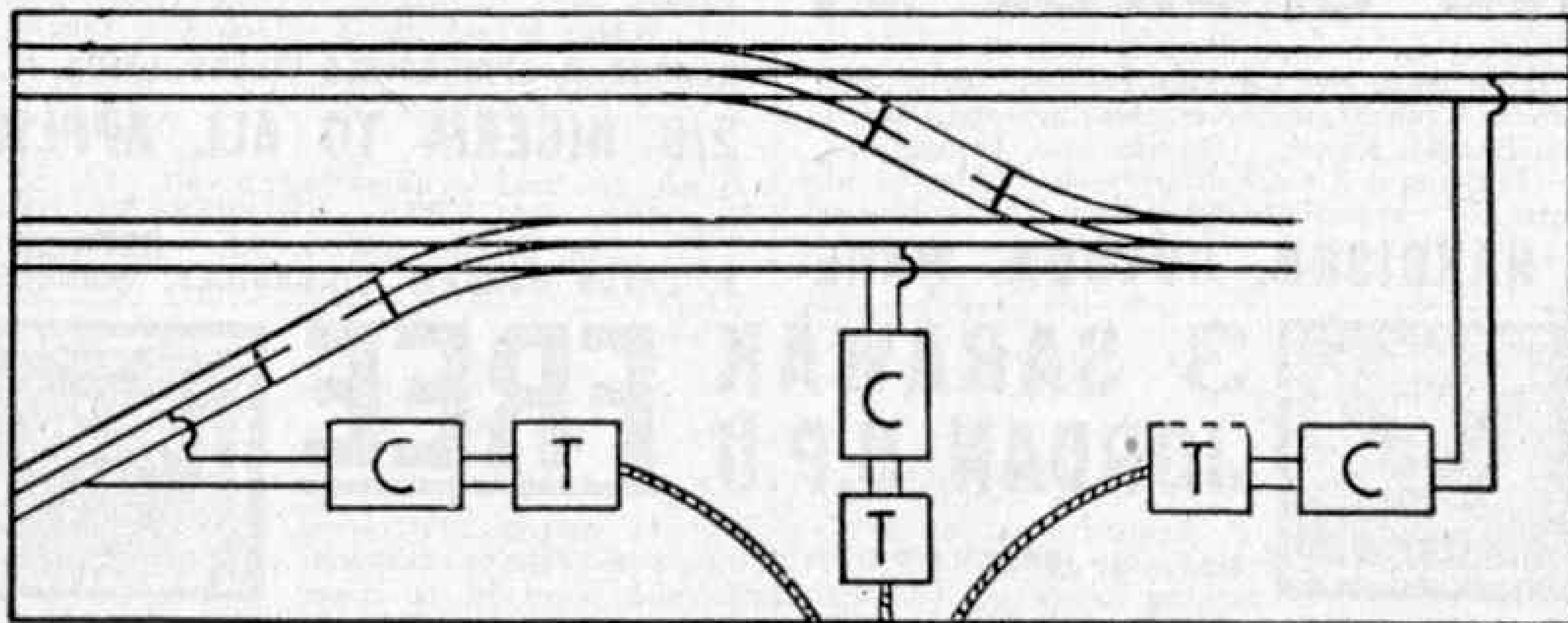
Power supply, connections and arrangements for independent control of three main sections of a Hornby-Dublo layout are shown here in diagram form.
