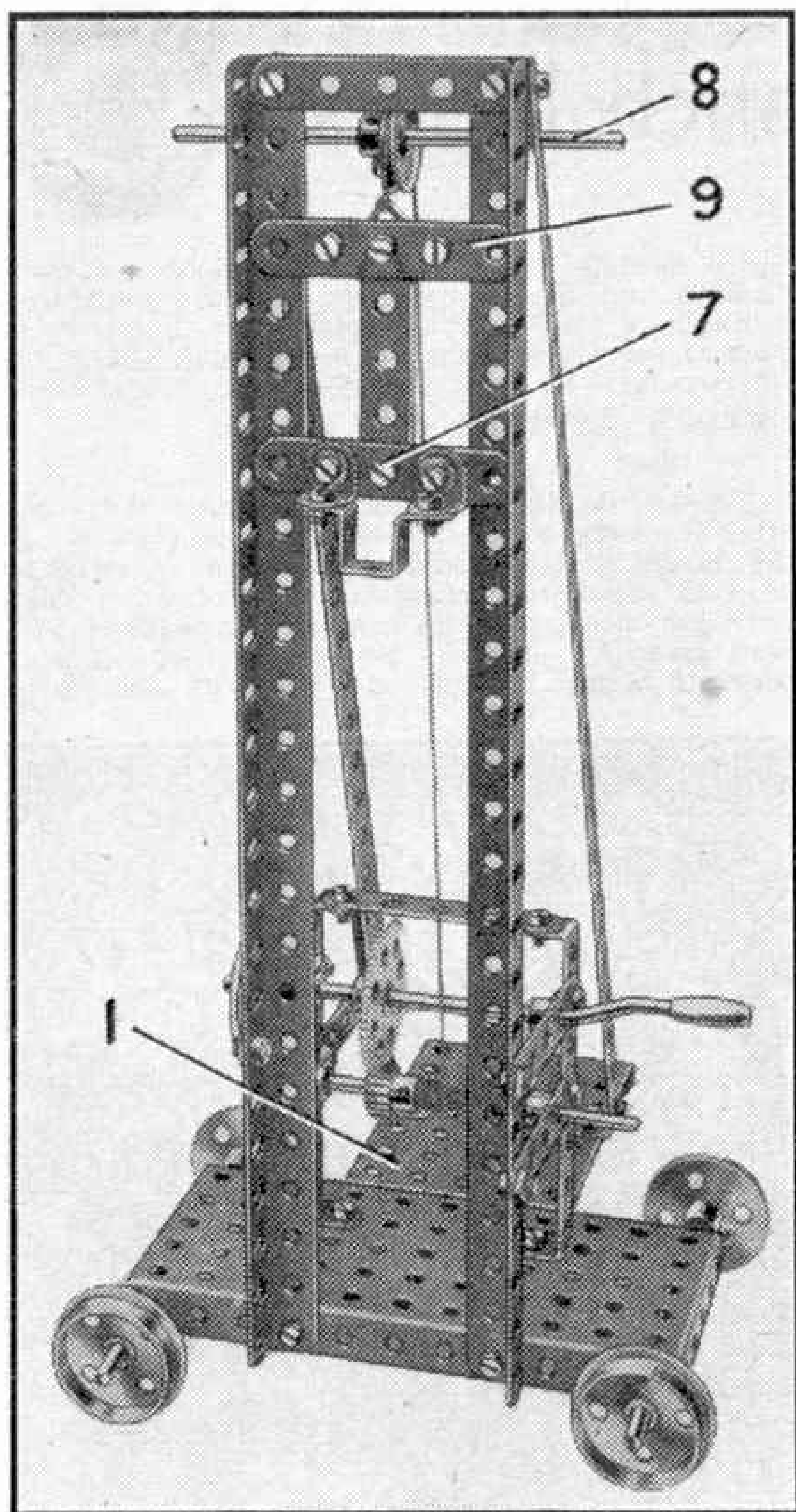
Fig. 3. General view of pile driver.
