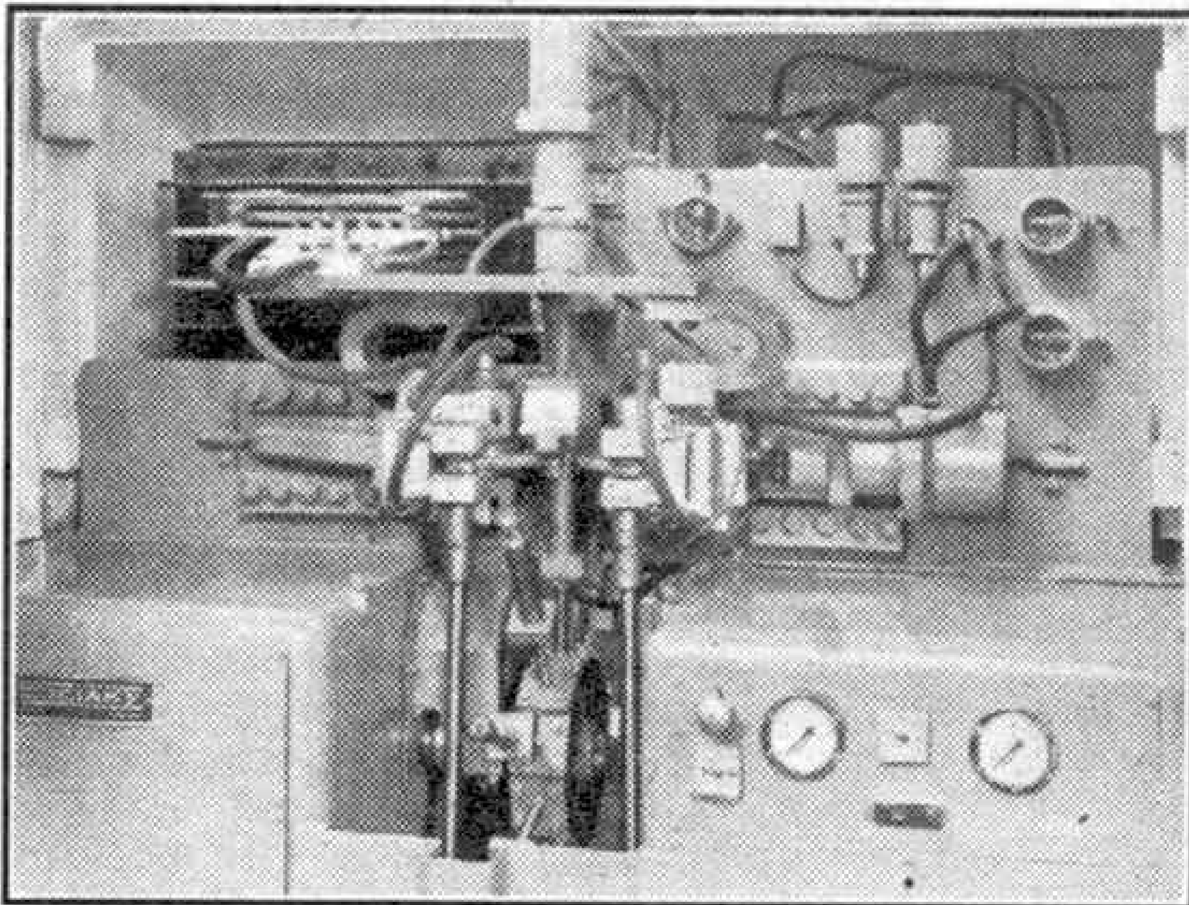
A special purpose resistance welding machine with a vertical indexing mechanism. Component parts are loaded on stations while the previous assembly is being welded.
