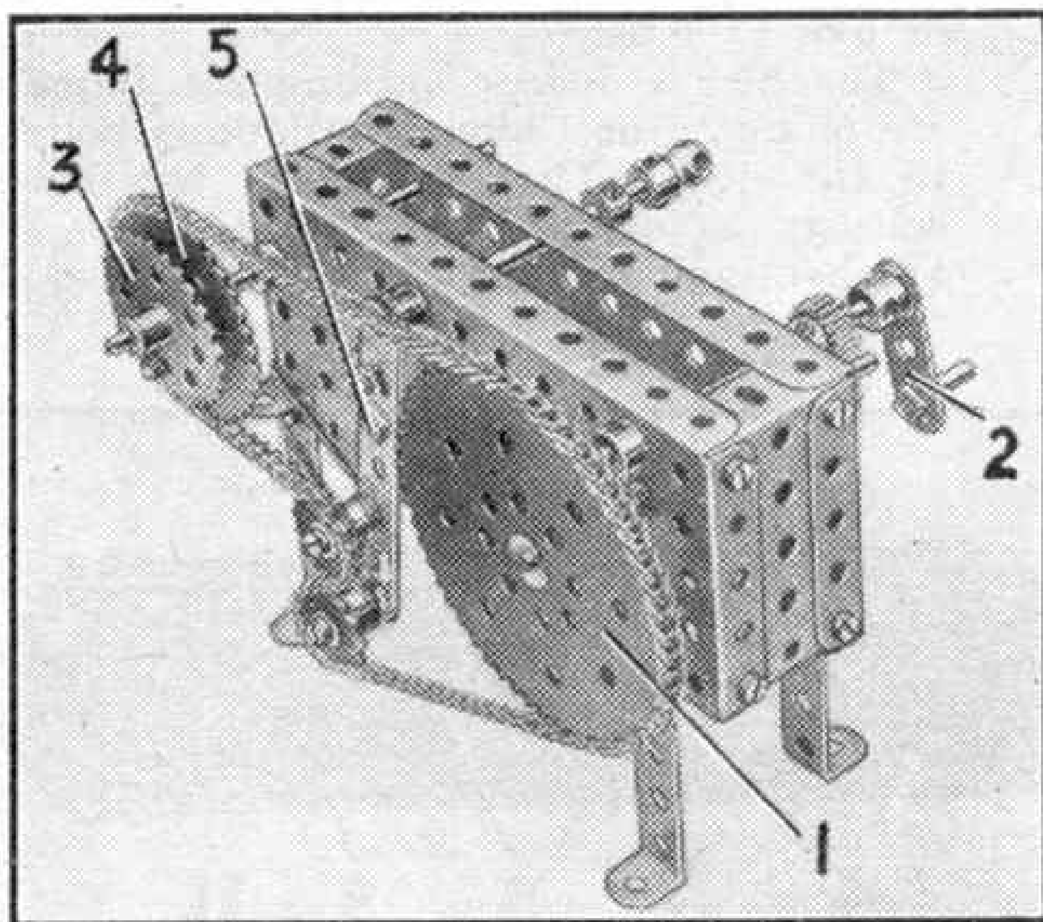
Fig. 5. A Deraileur type change-speed mechanism assembled on a demonstration framework.
