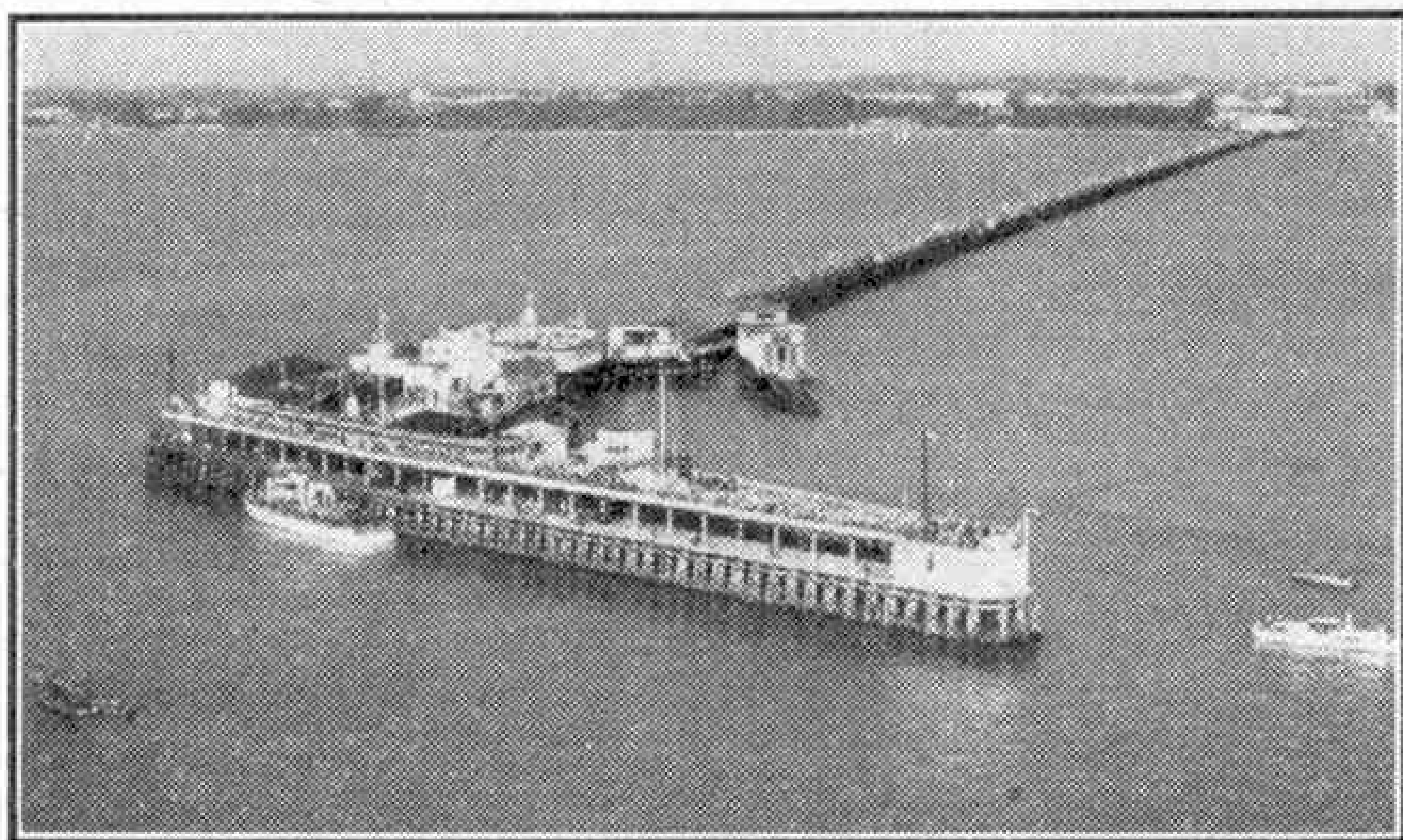
Southend Pier, the largest structure of this kind in the world, seen from the air. A double track electric railway runs along its 1\frac{1}{2} mile length.
