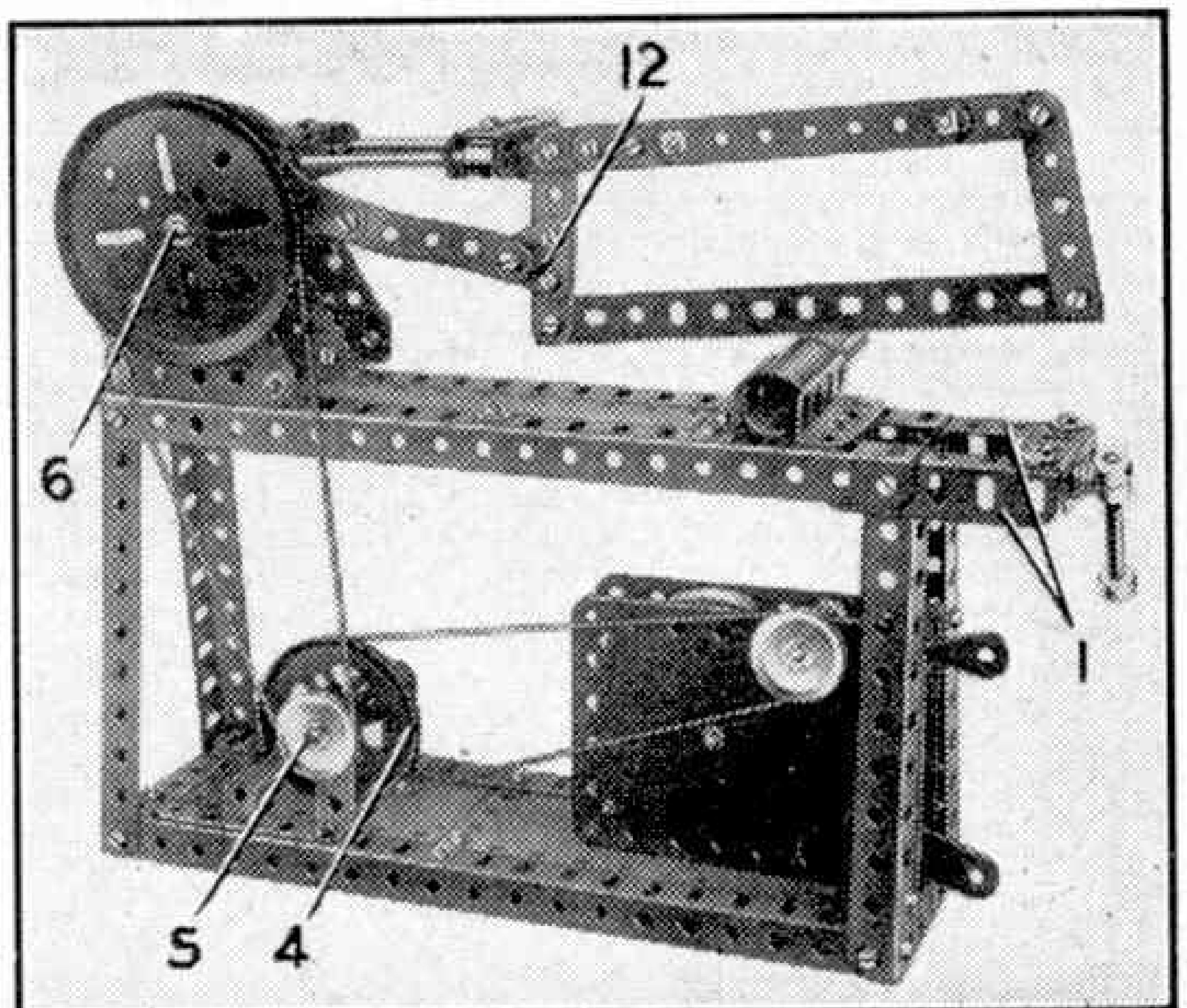
Fig. 4. Another view of the metal sawing machine.
