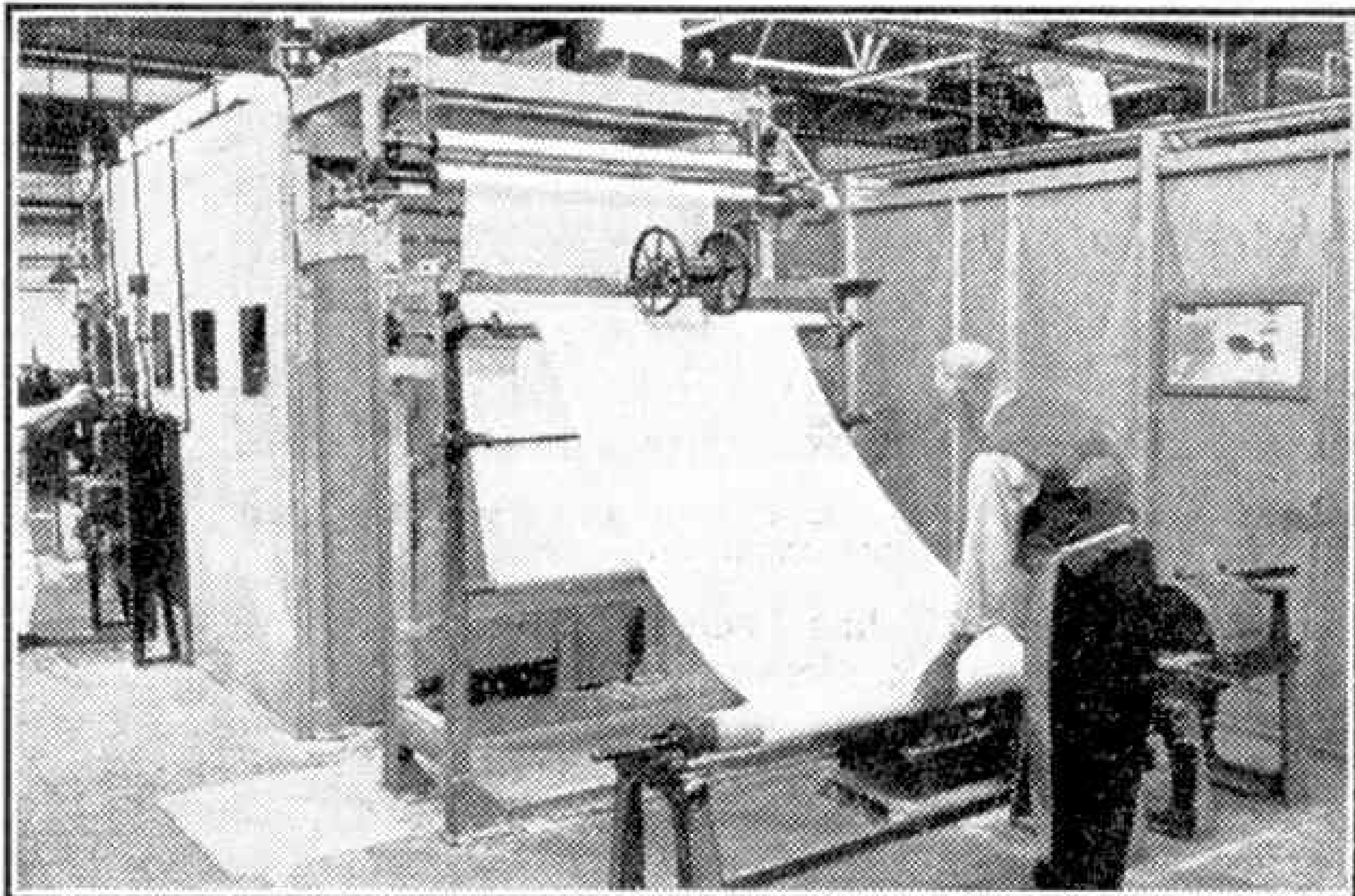
Vinal interlayer, a plastic material, being conditioned and reeled in readiness for use in making laminated safety glass at the works of the Triplex Safety Glass Company Ltd., to whom we are indebted for the illustrations to this article.
