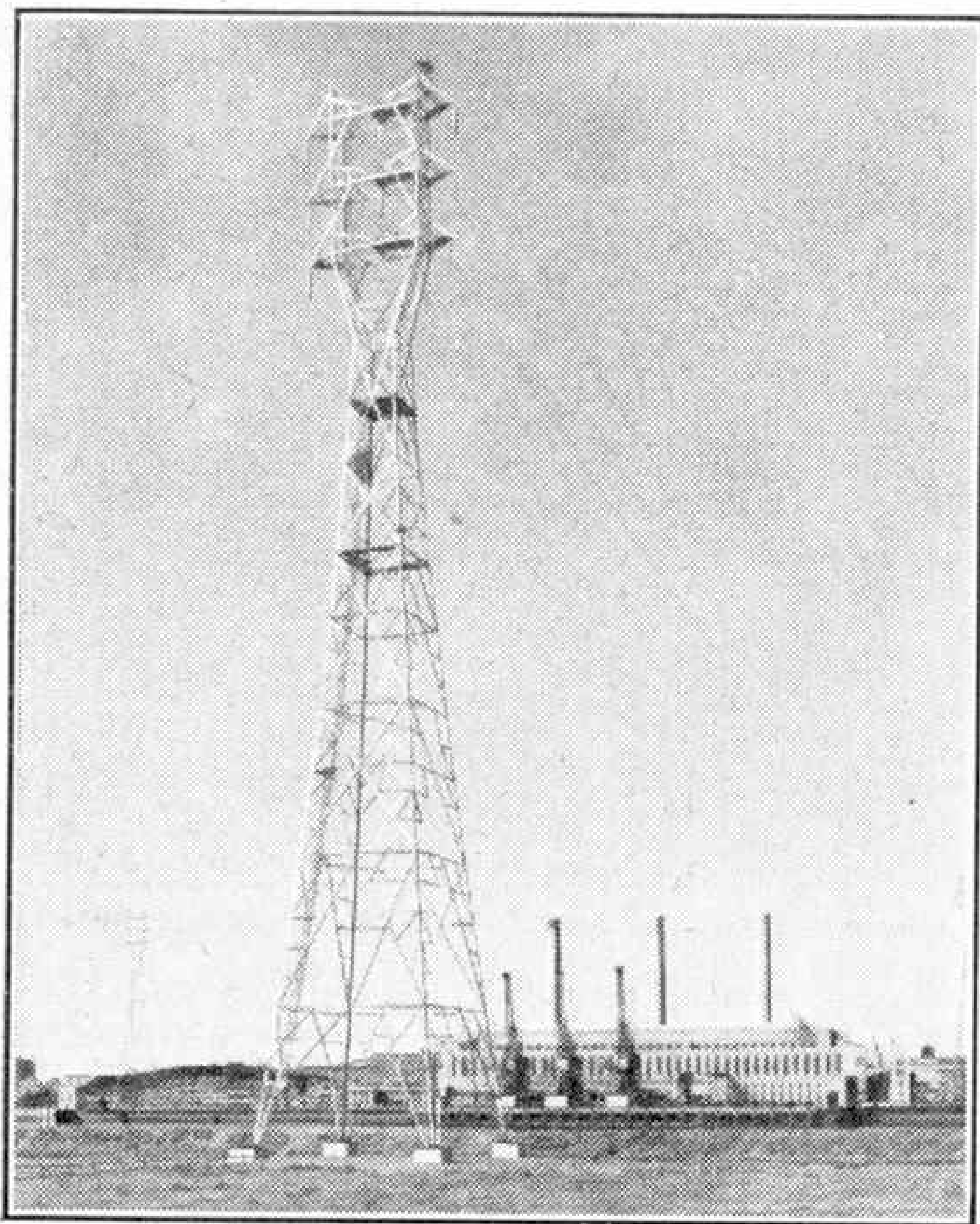
Tall pylons of the high voltage transmission system at Cliff Quay. Photograph by courtesy of B. I. Callender's Cables Co. Ltd.
