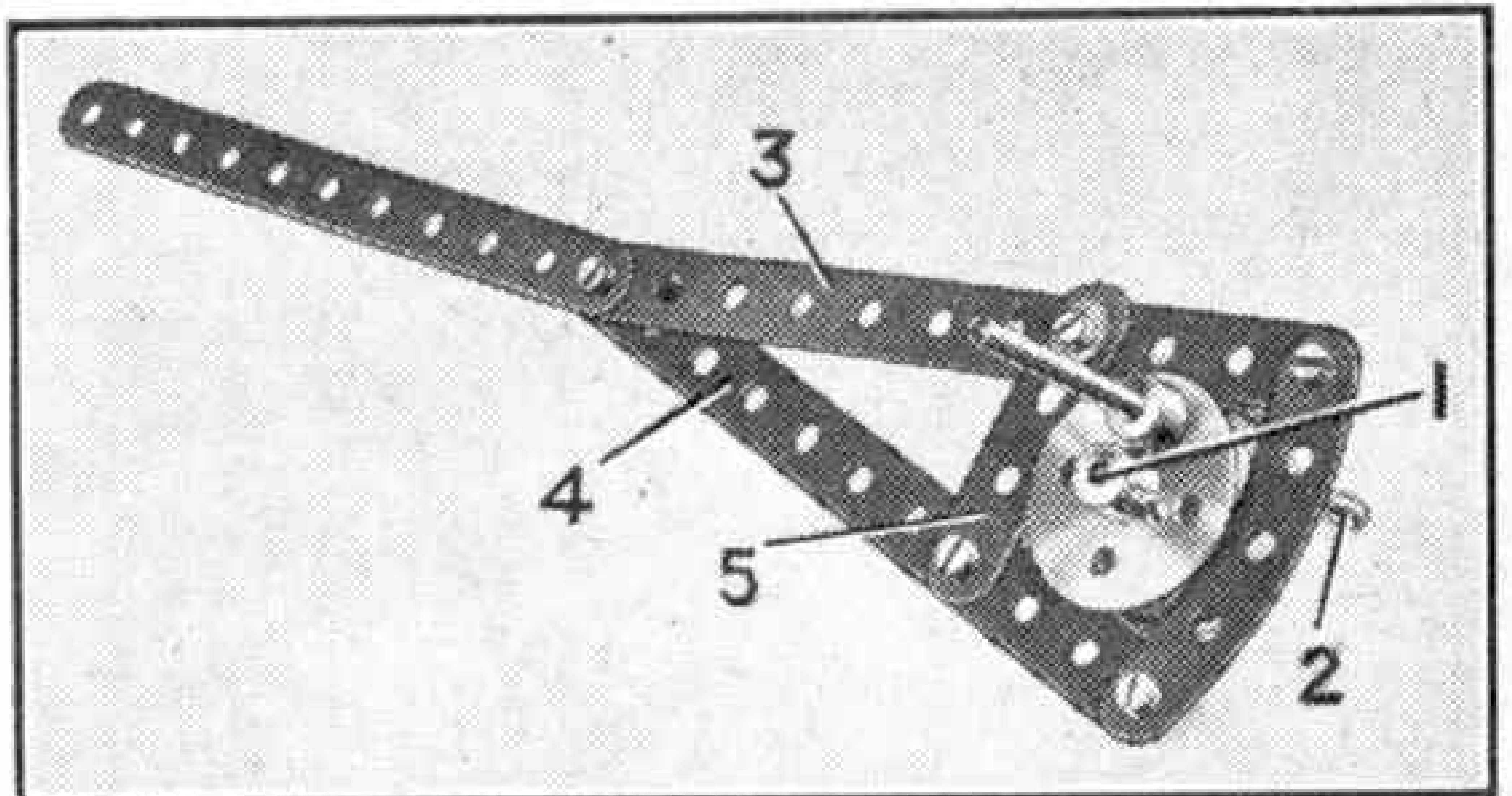
Fig. 5. A built-up eccentric designed by P. Knight, Bristol.
