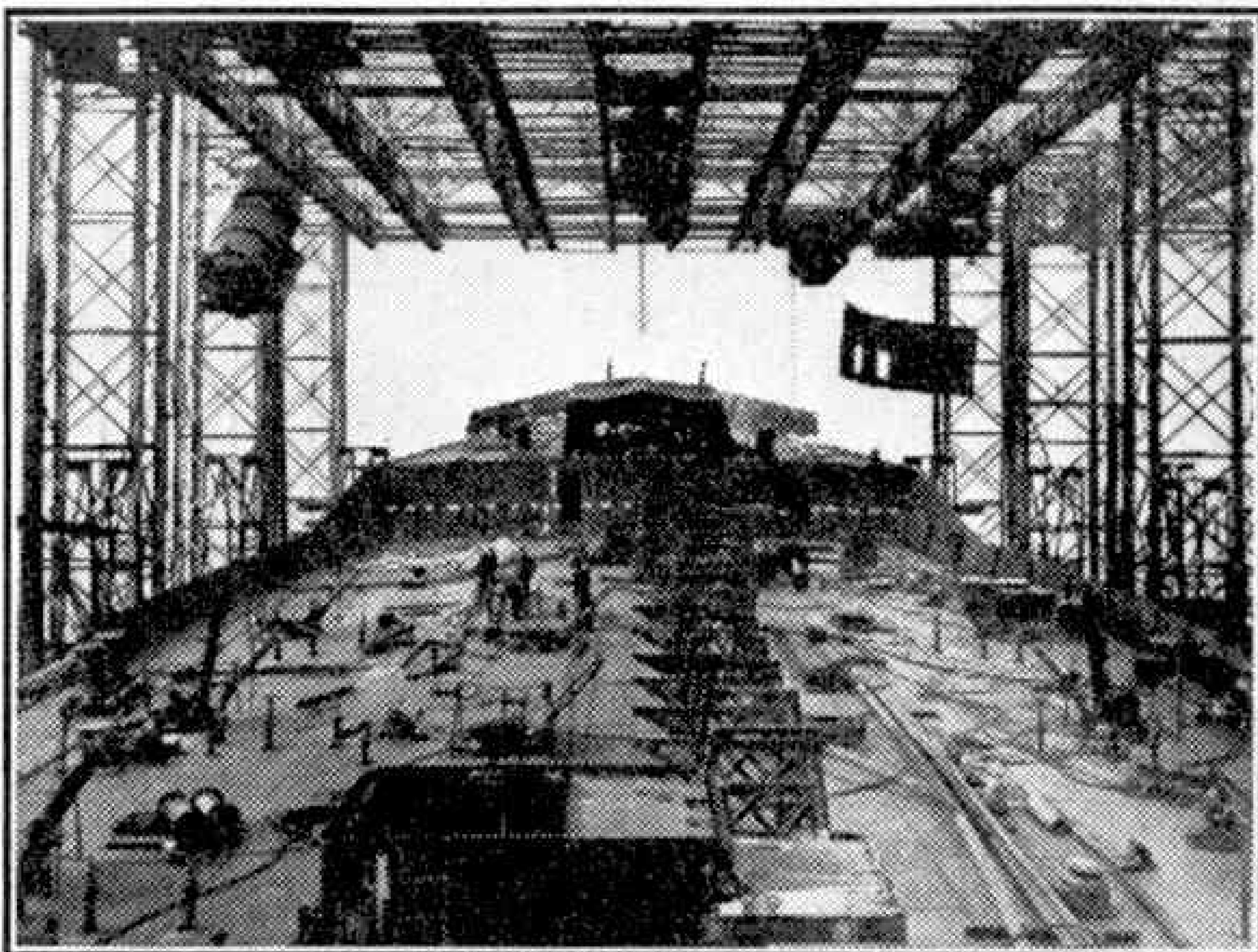
View from the bridge of the "Velutina" during construction, showing the forward pump room entrance and the forecastle deck.
