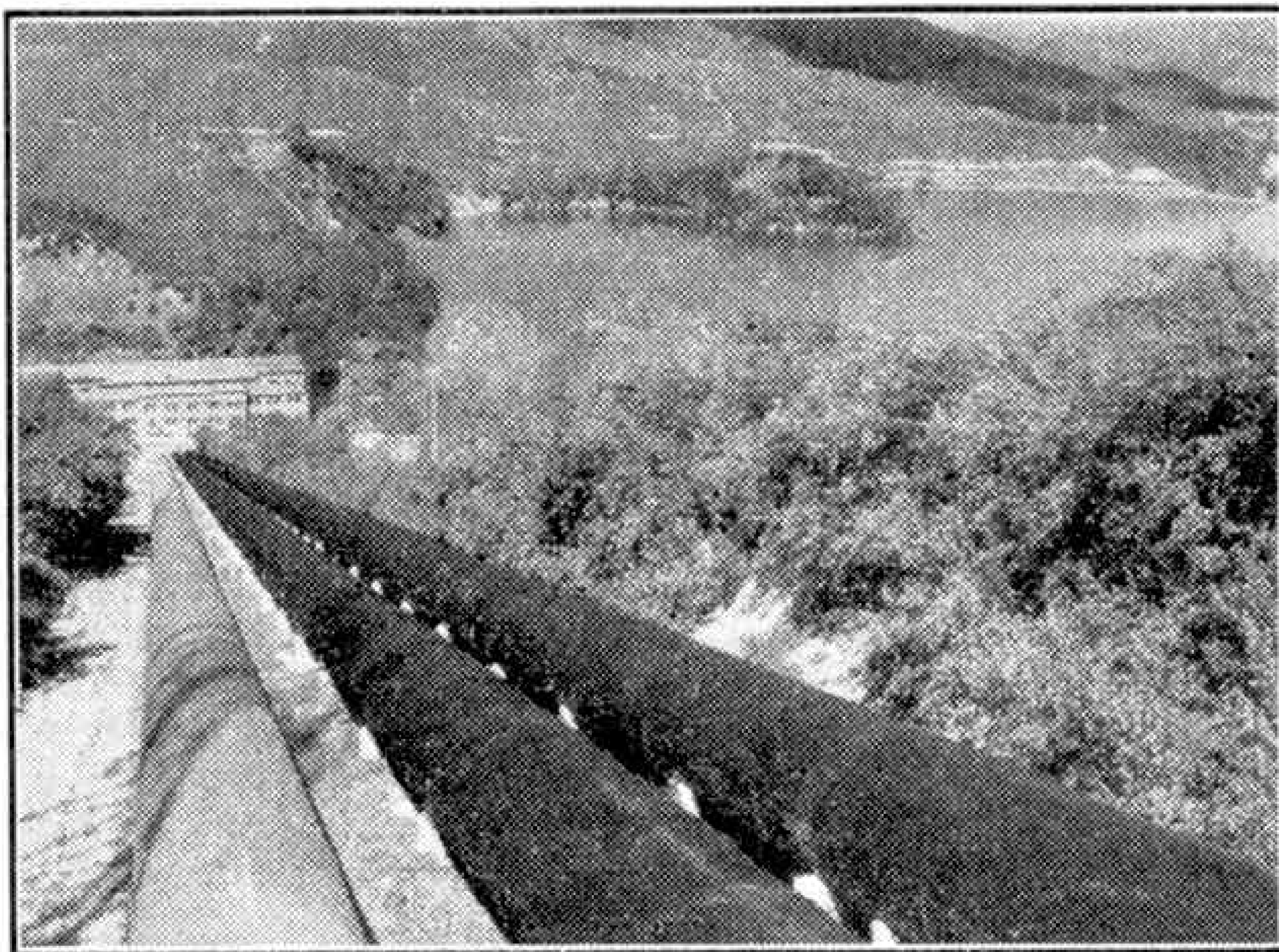
Tuai hydro-electric station.
