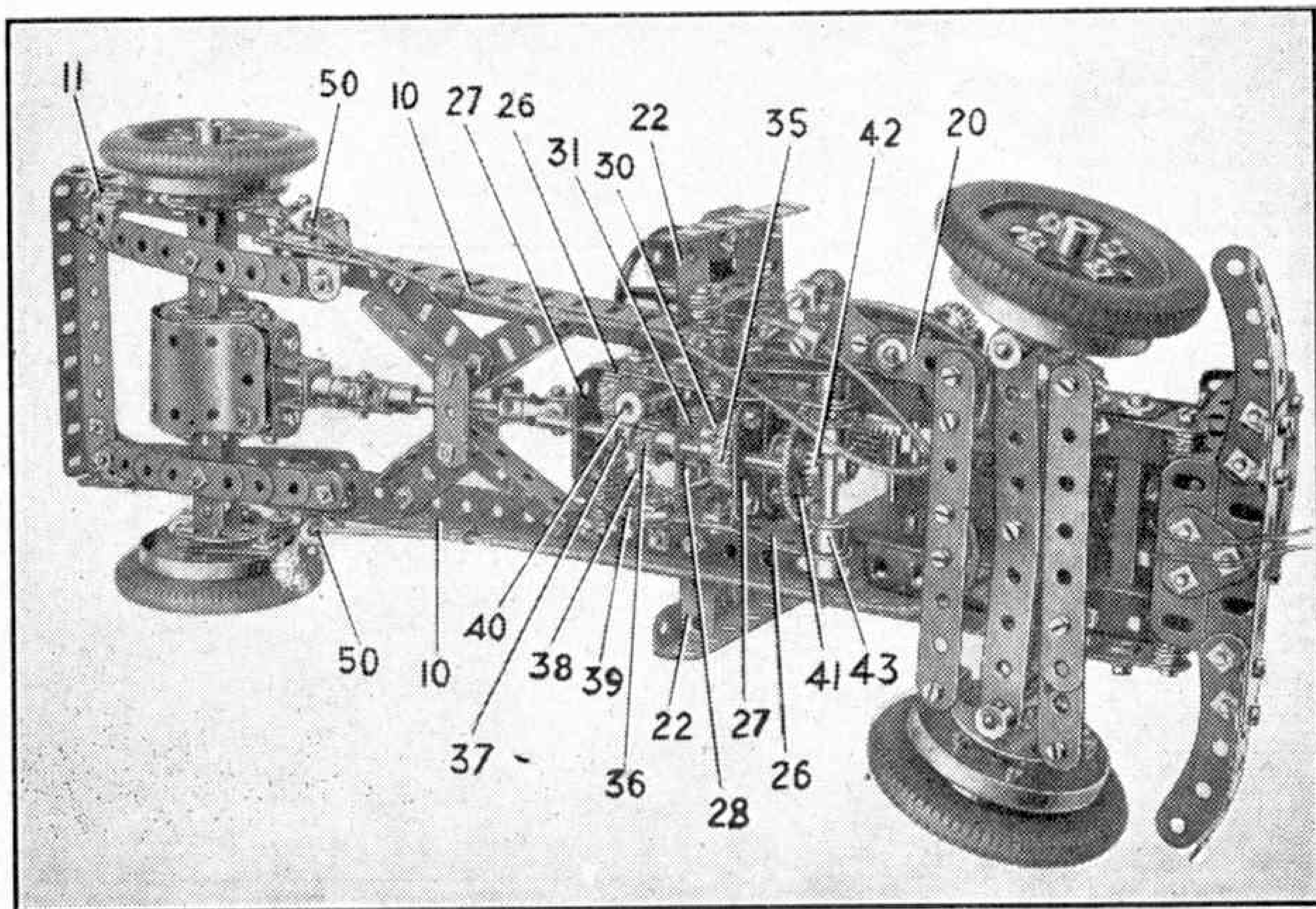
Fig. 4. An underneath view of the chassis showing the steering linkage and details of the clutch and gear-box.
