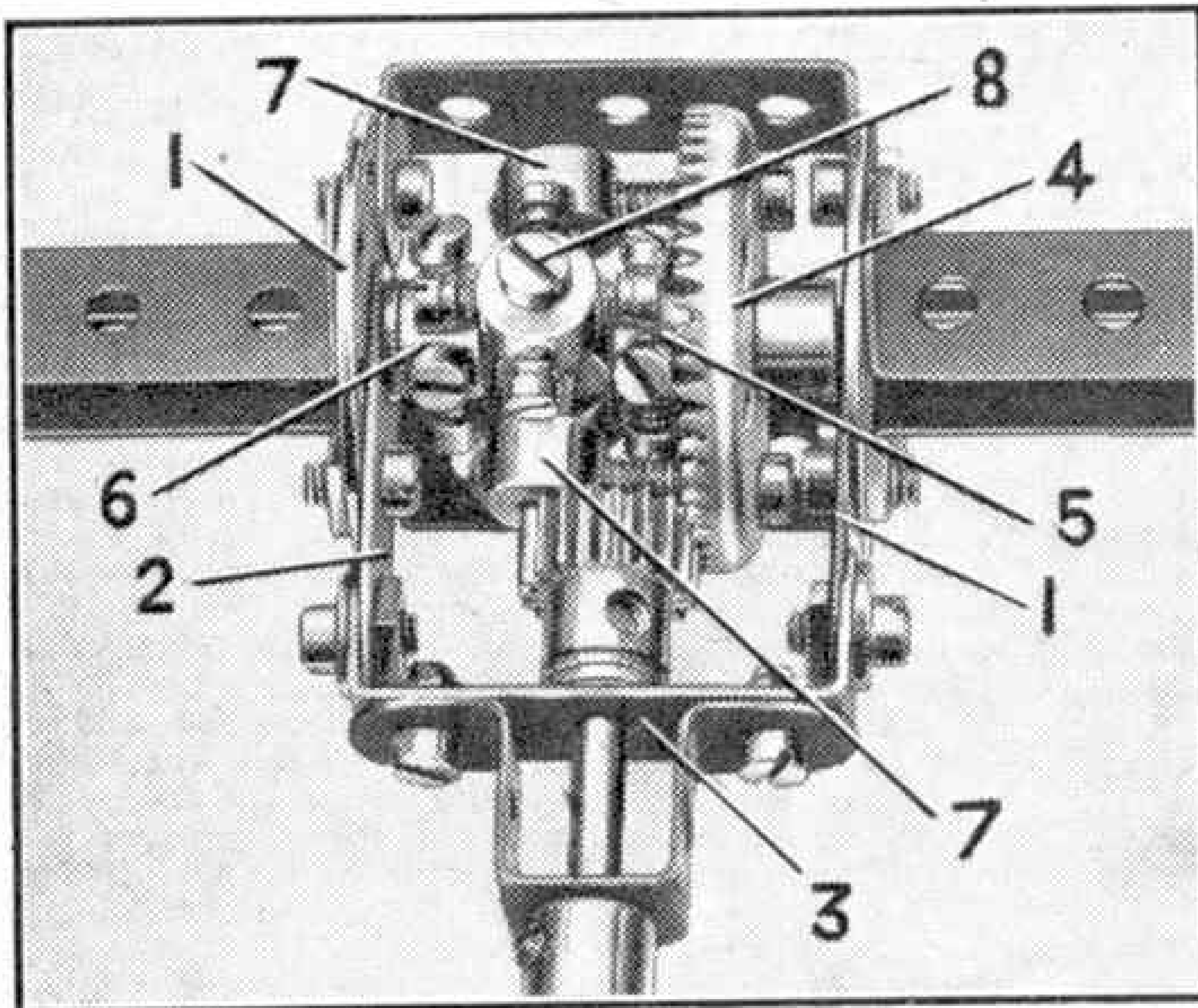
Fig. 4. The novel differential mechanism of Fig. 3, shown here without its casing.
