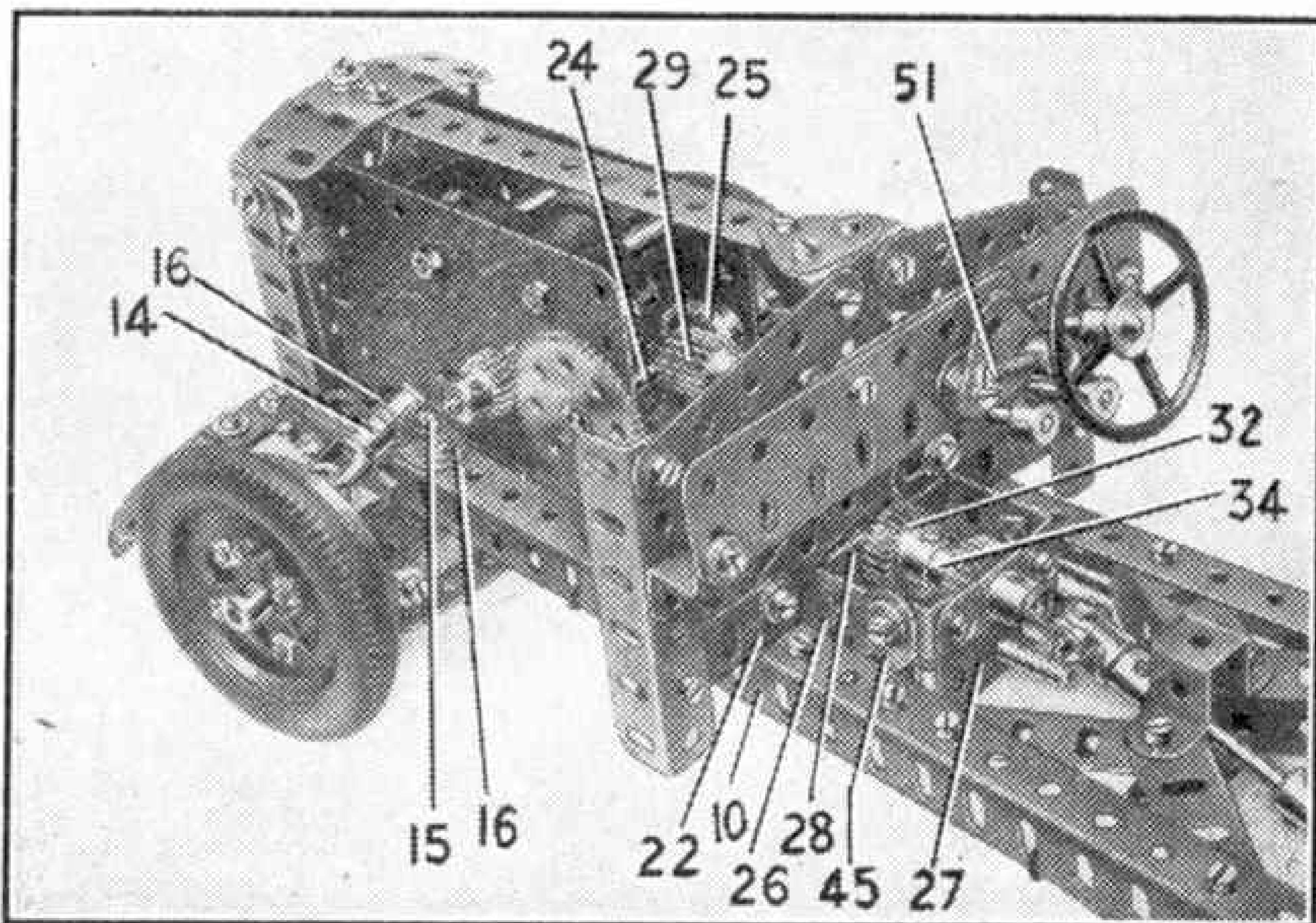
Fig. 6. The arrangement of the reduction gearing between the EZOR Electric Motor and the gear-box is seen clearly in this view.
