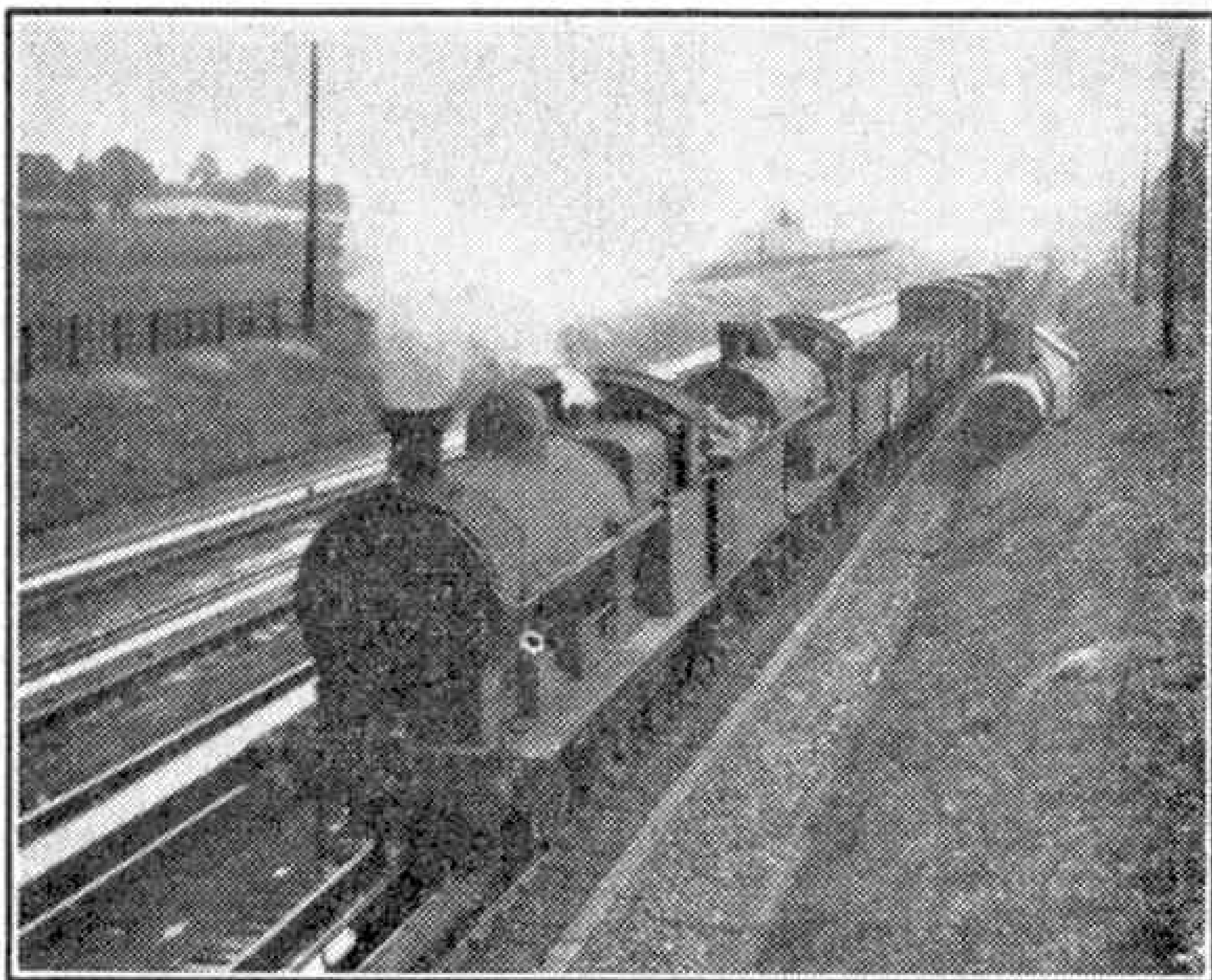
This picture taken some years ago shows one of the familiar ex-L.N.W.R. 0-8-0s at Whitmore troughs. The second engine is a "George the Fifth" 4-4-0 "Widgeon" being hauled to Crewe for scrapping.
