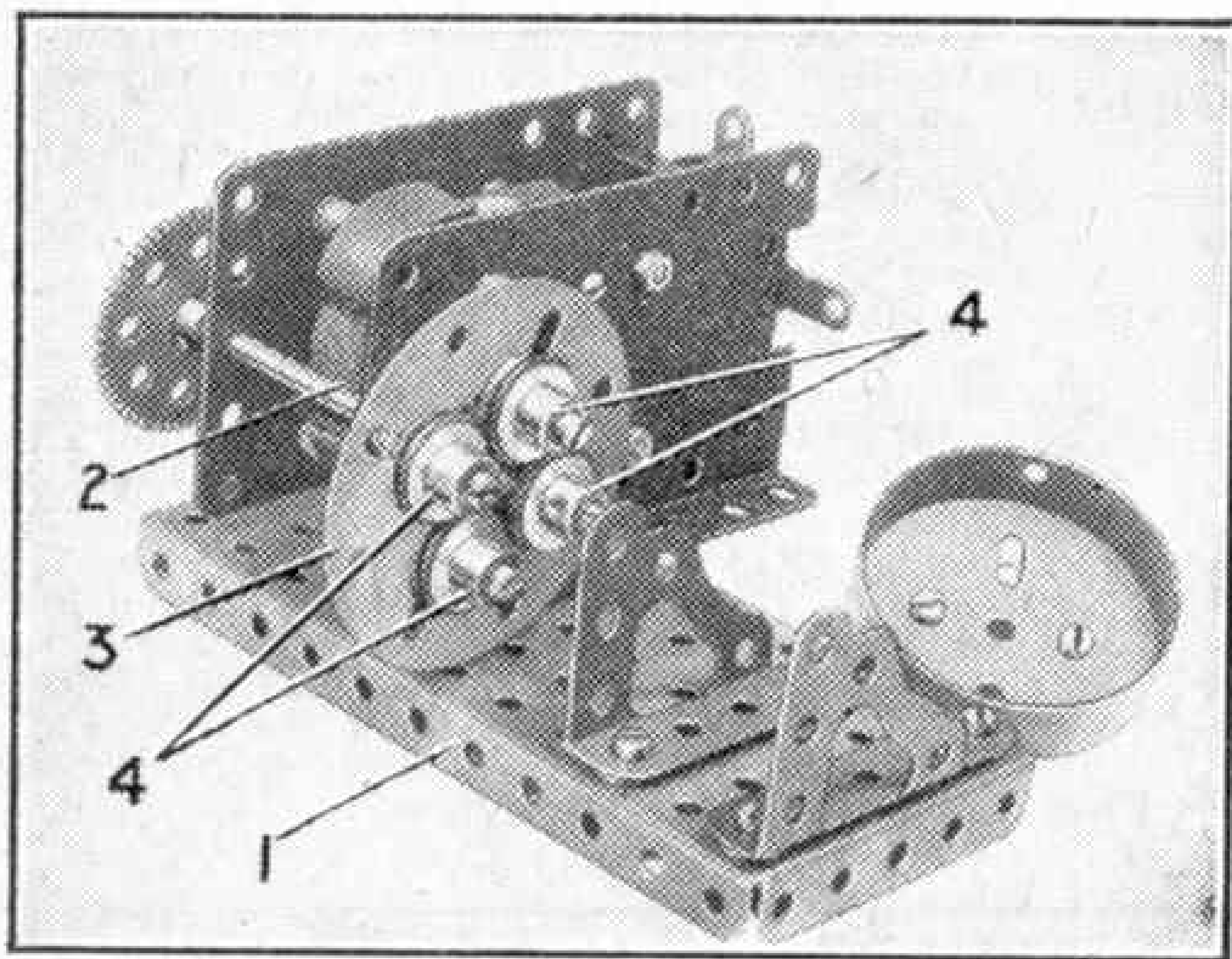
Fig. 2. The centrifugal clutch showing the interior construction.
