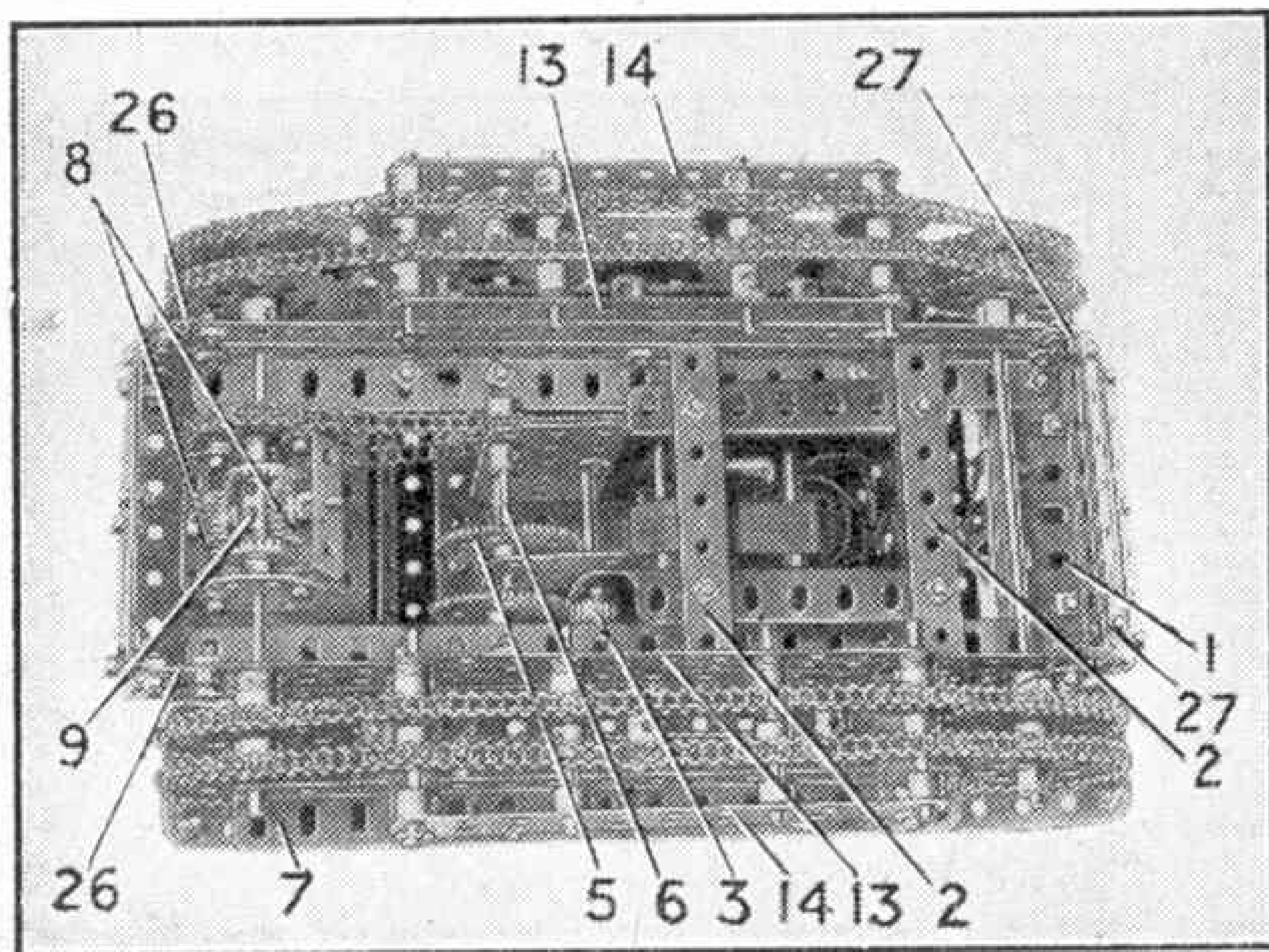
Fig. 2. An underneath view of the tank.
