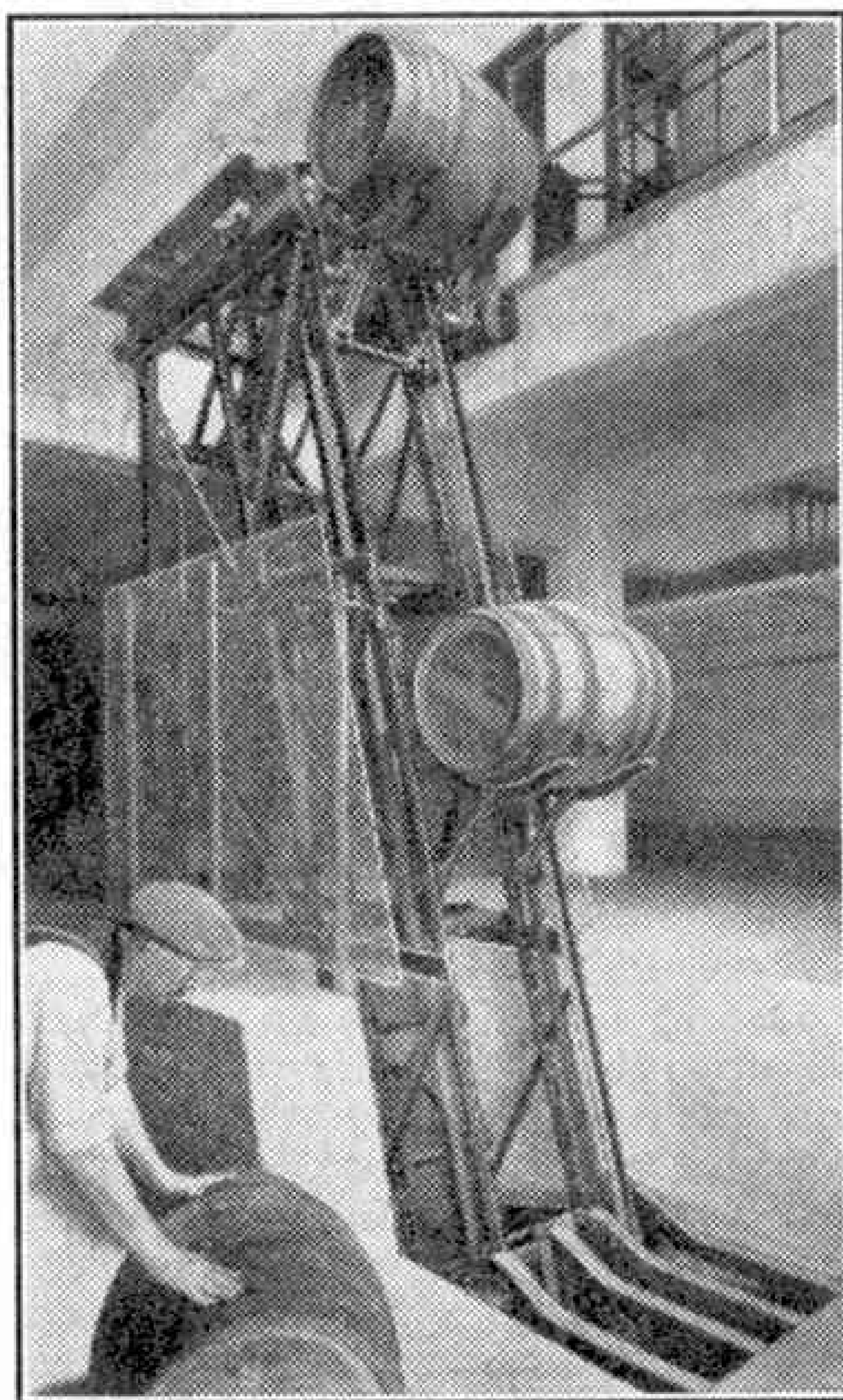
Power-operated barrel conveyor.
