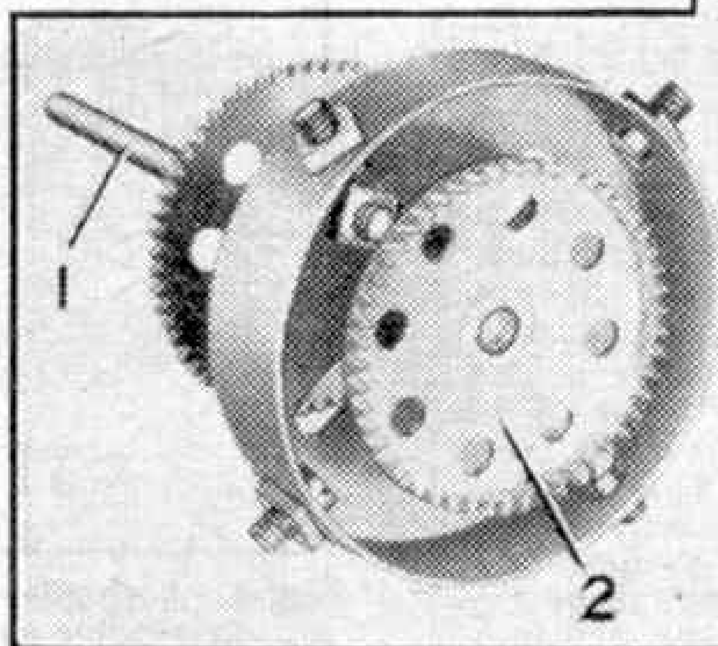
Fig. 4. The clutch unit dismantled to show the internal details.
