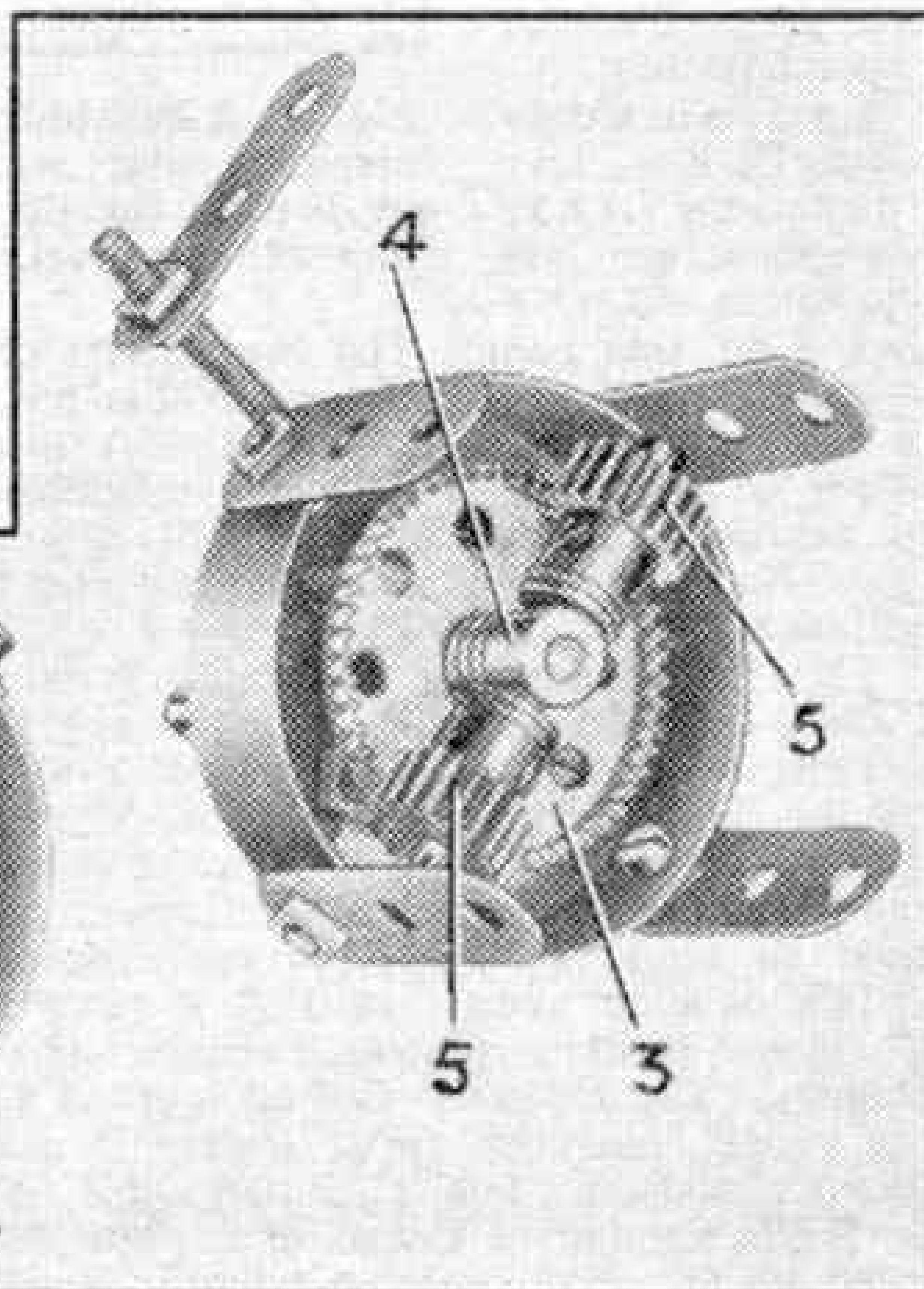
Fig. 4. The clutch unit dismantled to show the internal details.
