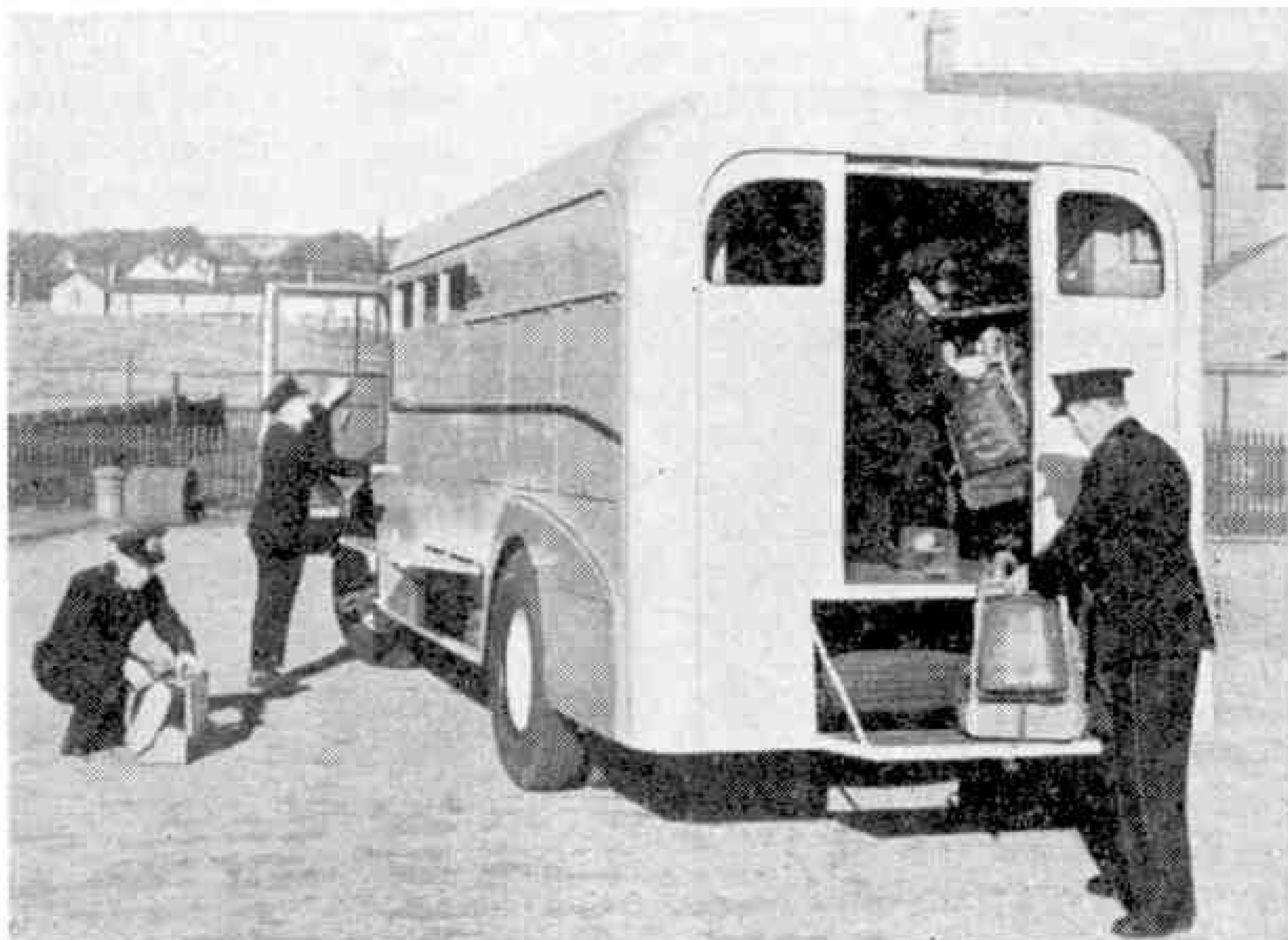
The Leyland Mine Rescue Van described on this page. Photograph by courtesy of Leyland Motors Ltd.
