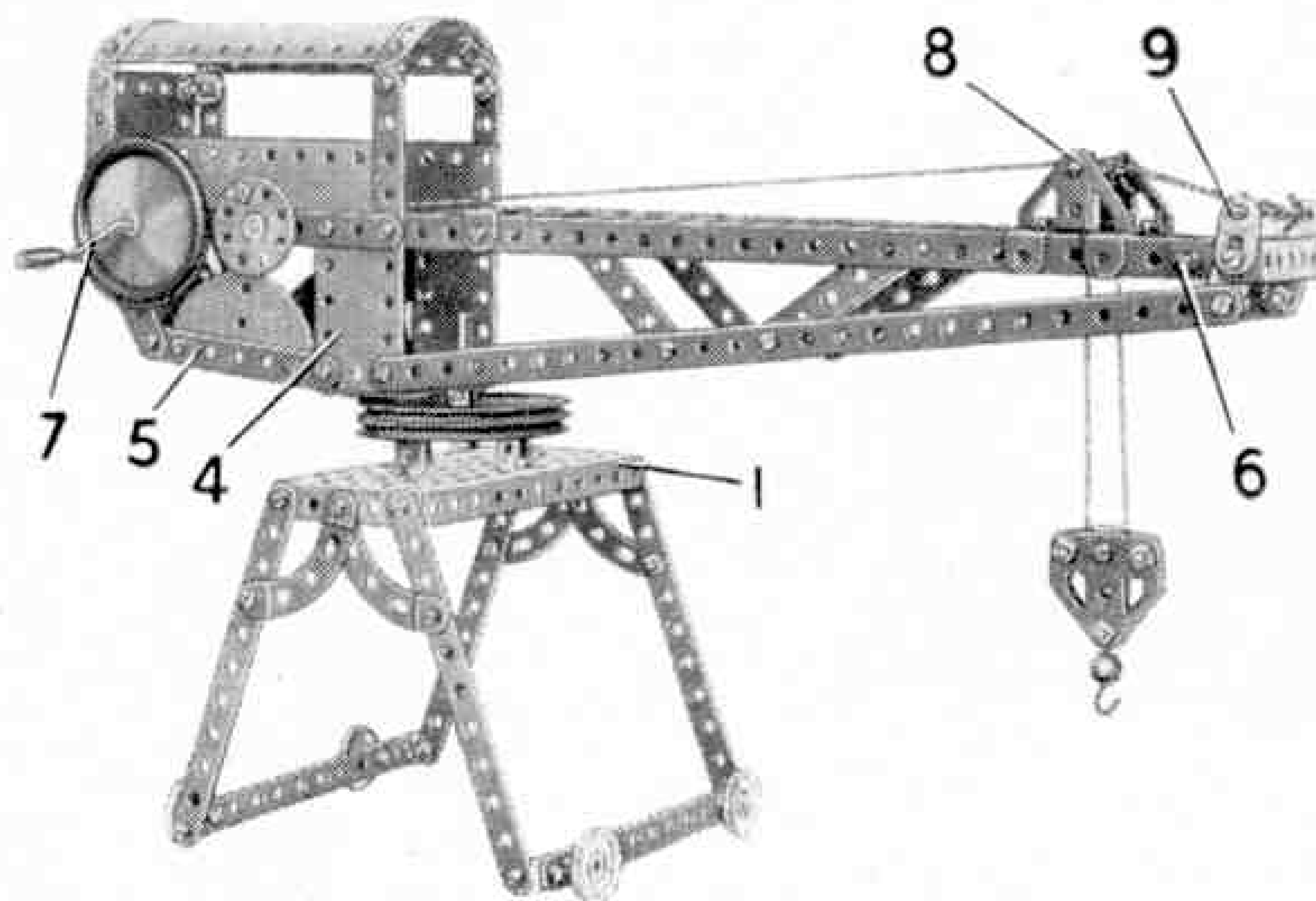
Fig. 1. An easy-to-build crane designed for Outfit No. 4.
