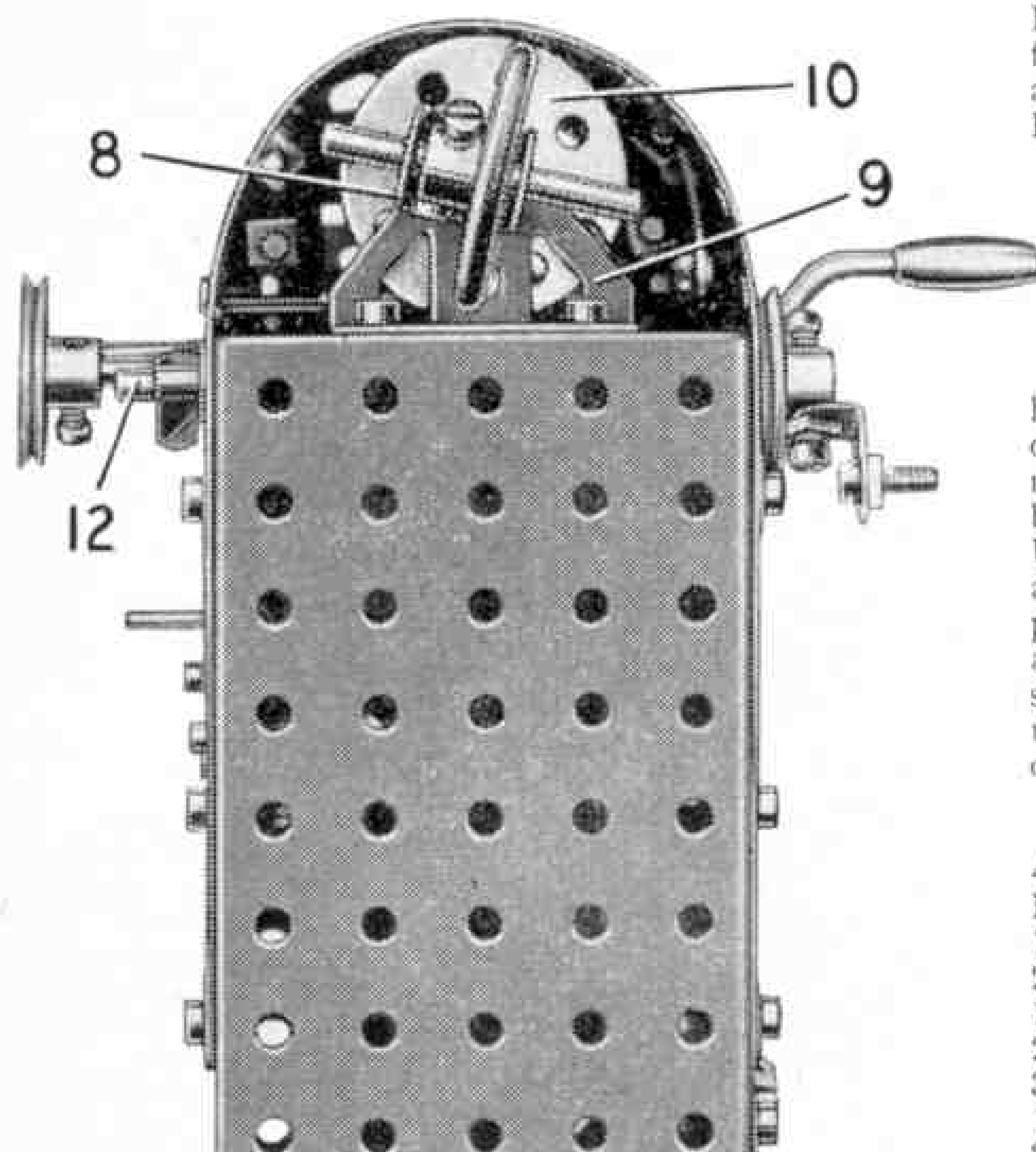
Fig. 4. An underneath view of the mobile crane.
