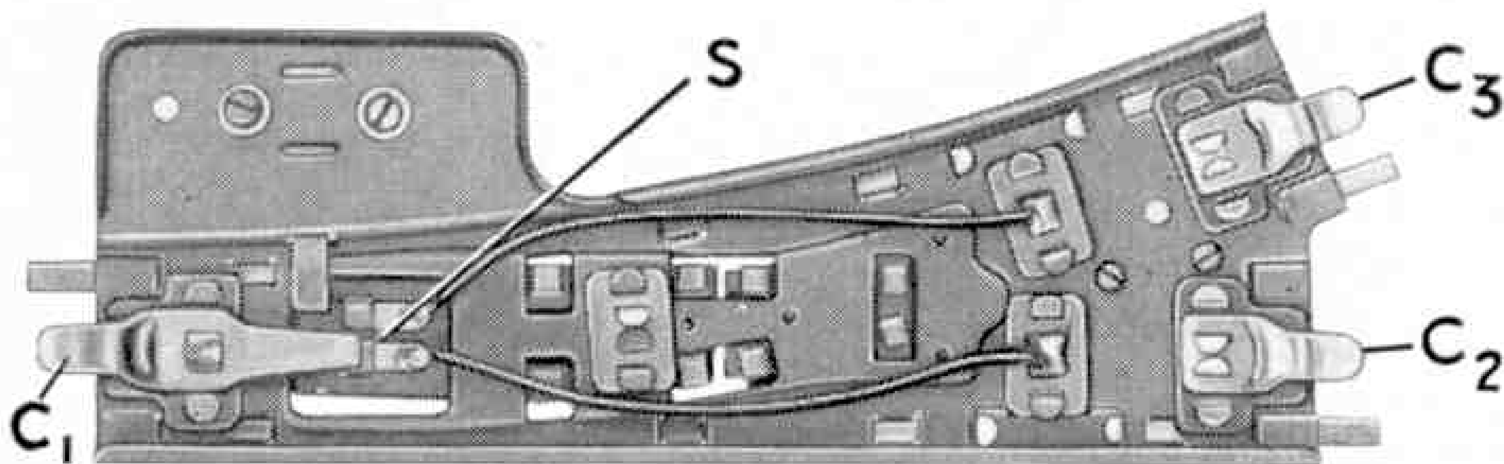
Underneath view of the Isolating Switch Points. Current is fed to the centre rail connecting clip C1 and is directed by the selector switch S to either route C2 or C3 according to the position of the Points blades.
