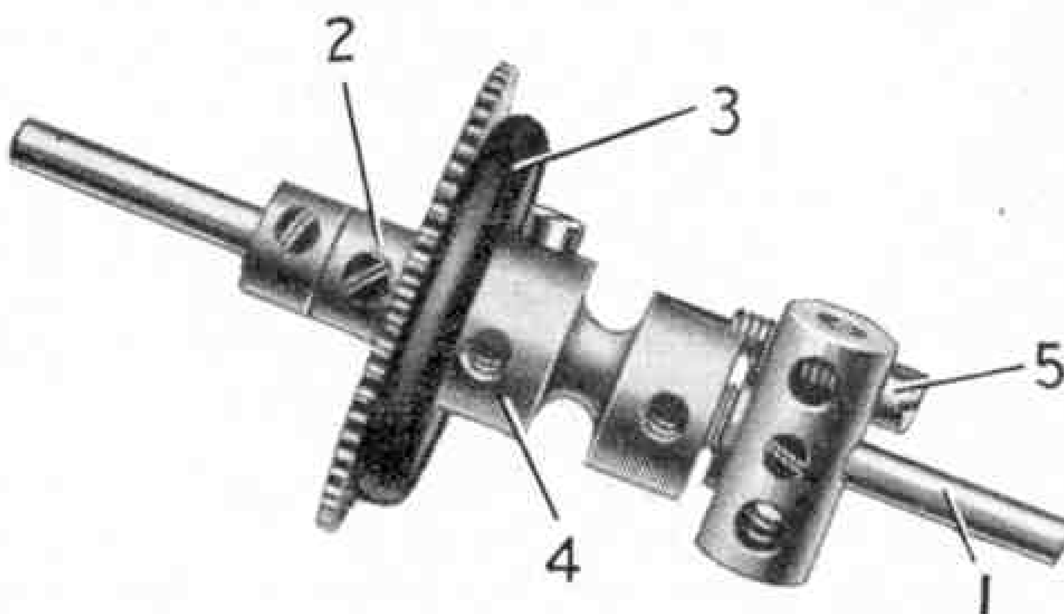
Fig. 1. This compact clutch mechanism is just the thing for disengaging the drive between the power unit and the gear-box of a model chassis. It was built by Mr. E. W. Henry, Sheffield, and details of it are given on this page.
