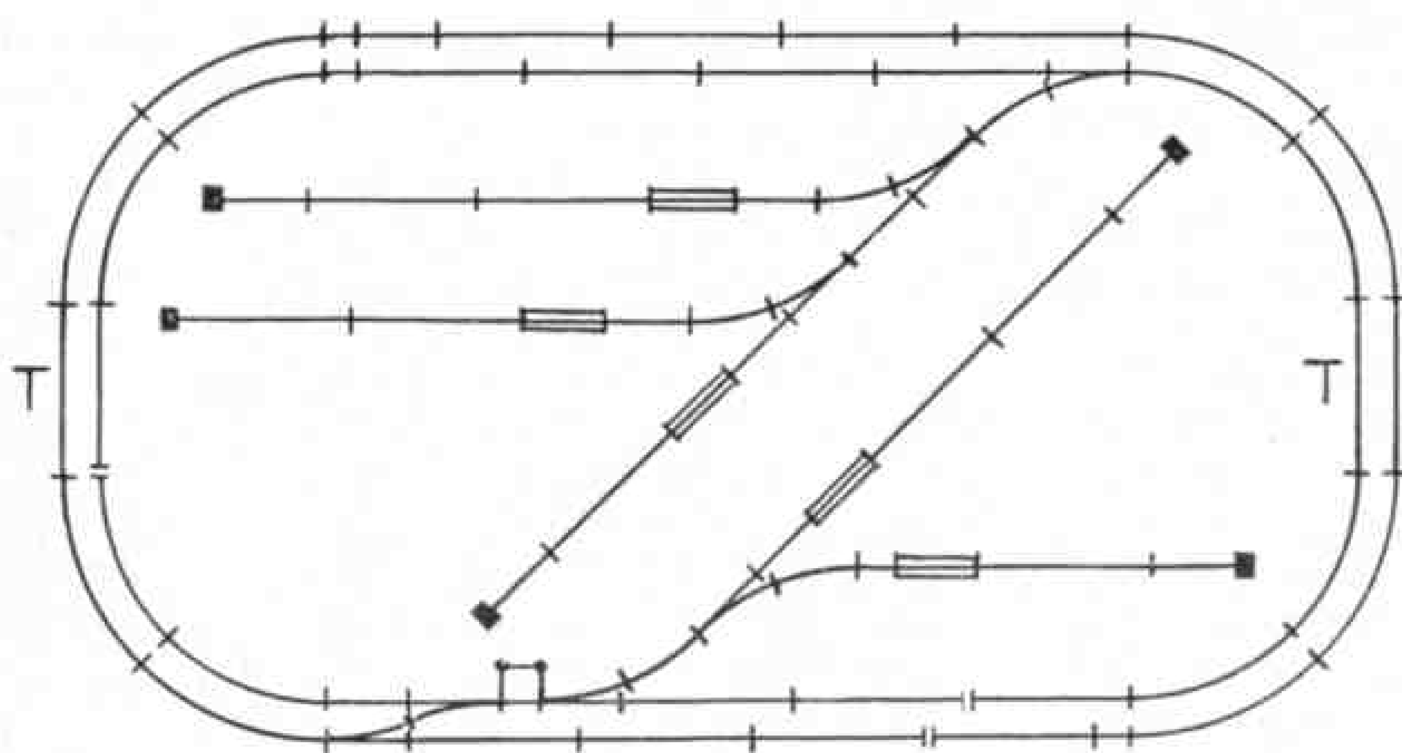
A typical double track formation incorporating the EDA2 Curves in the outer track. Isolating Switch Points are used in this layout and a secondary feeding point is arranged in the usual manner by means of an Isolating Rail.
