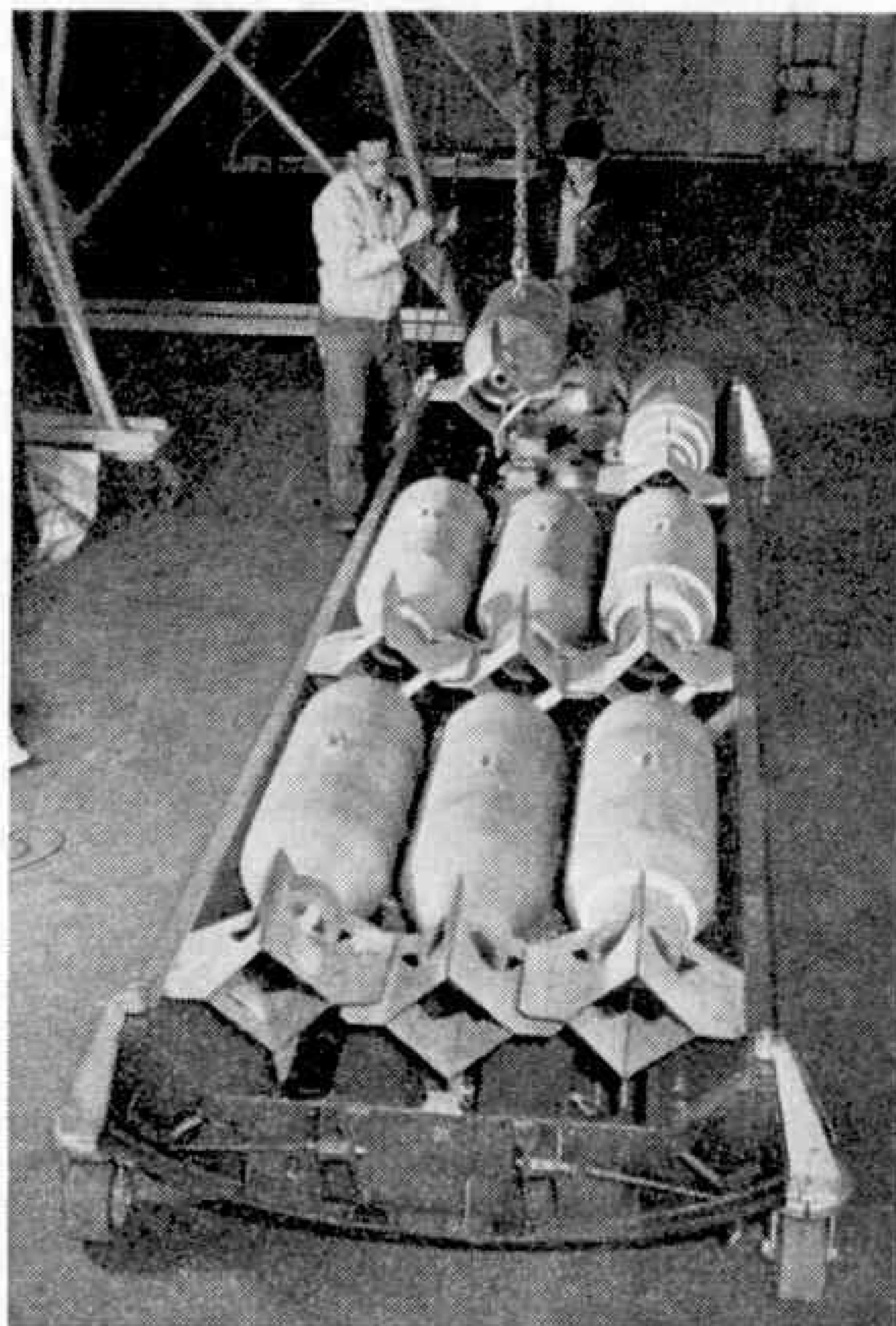
Rotary bomb door of U.S. version of the Canberra shown removed from the aircraft and being loaded. Moving the door about while it is on the ground is made easy by dollies fitted at the corners. Photograph by courtesy of The Glenn L. Martin Company, U.S.A.
