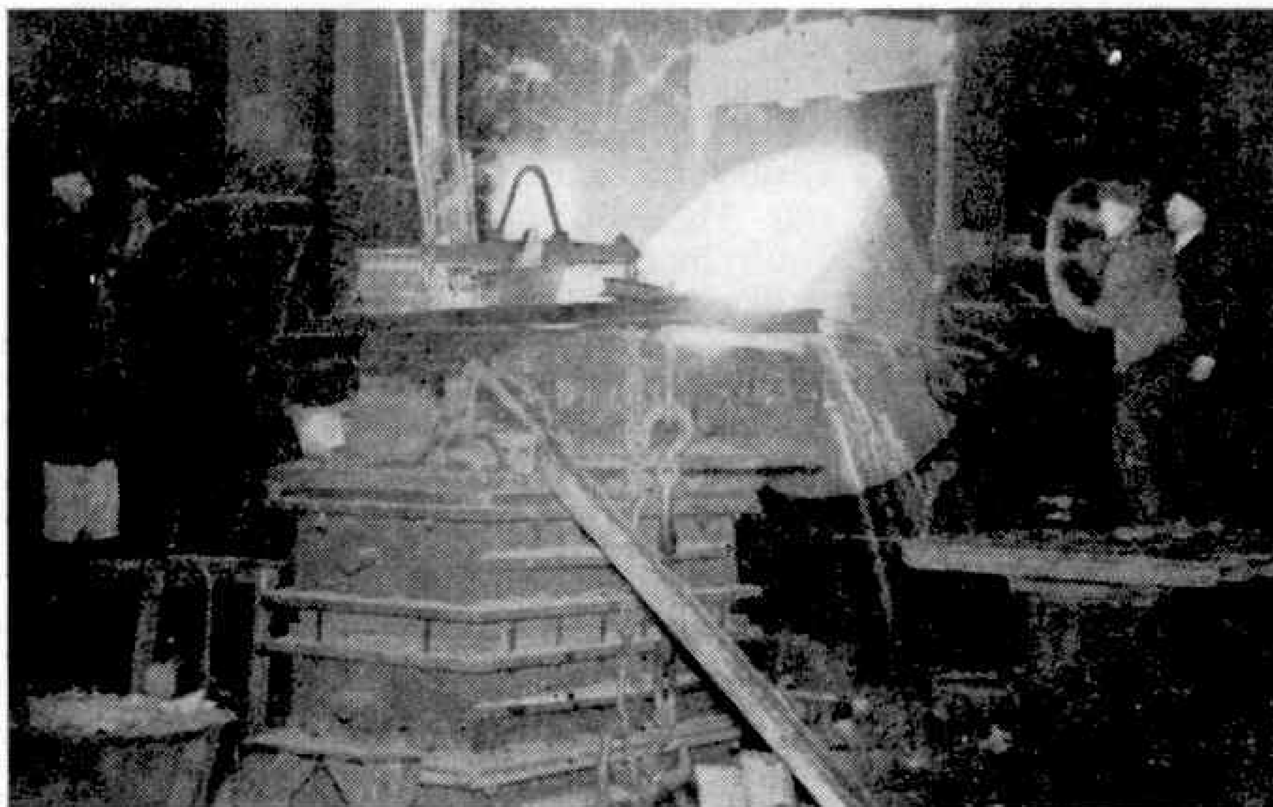
Casting in a dry sand mould to make a gas retort.
