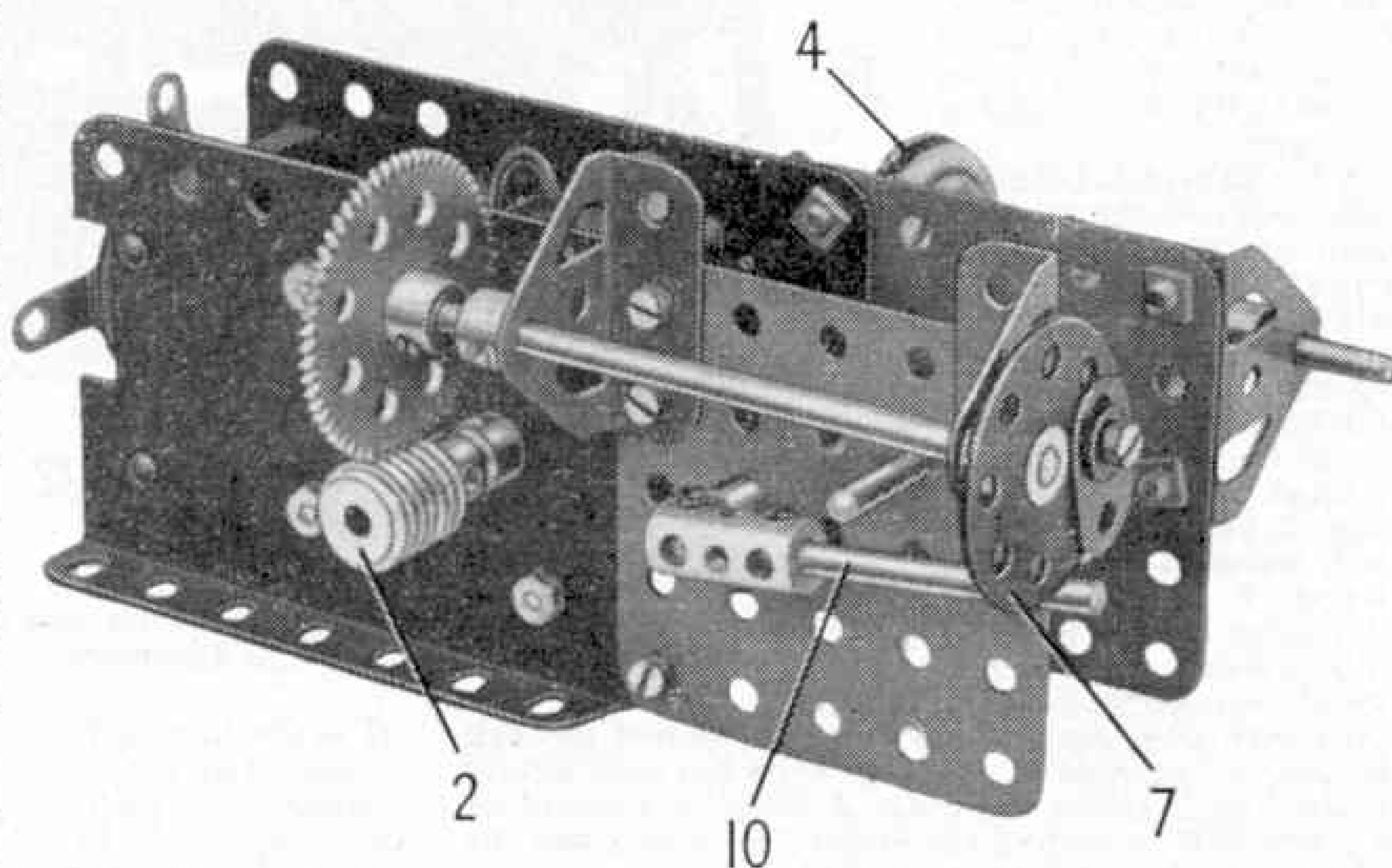
Fig. 3. Another view of the intermittent motion device, showing the drive to the built-up cam that controls the clutch release lever.
