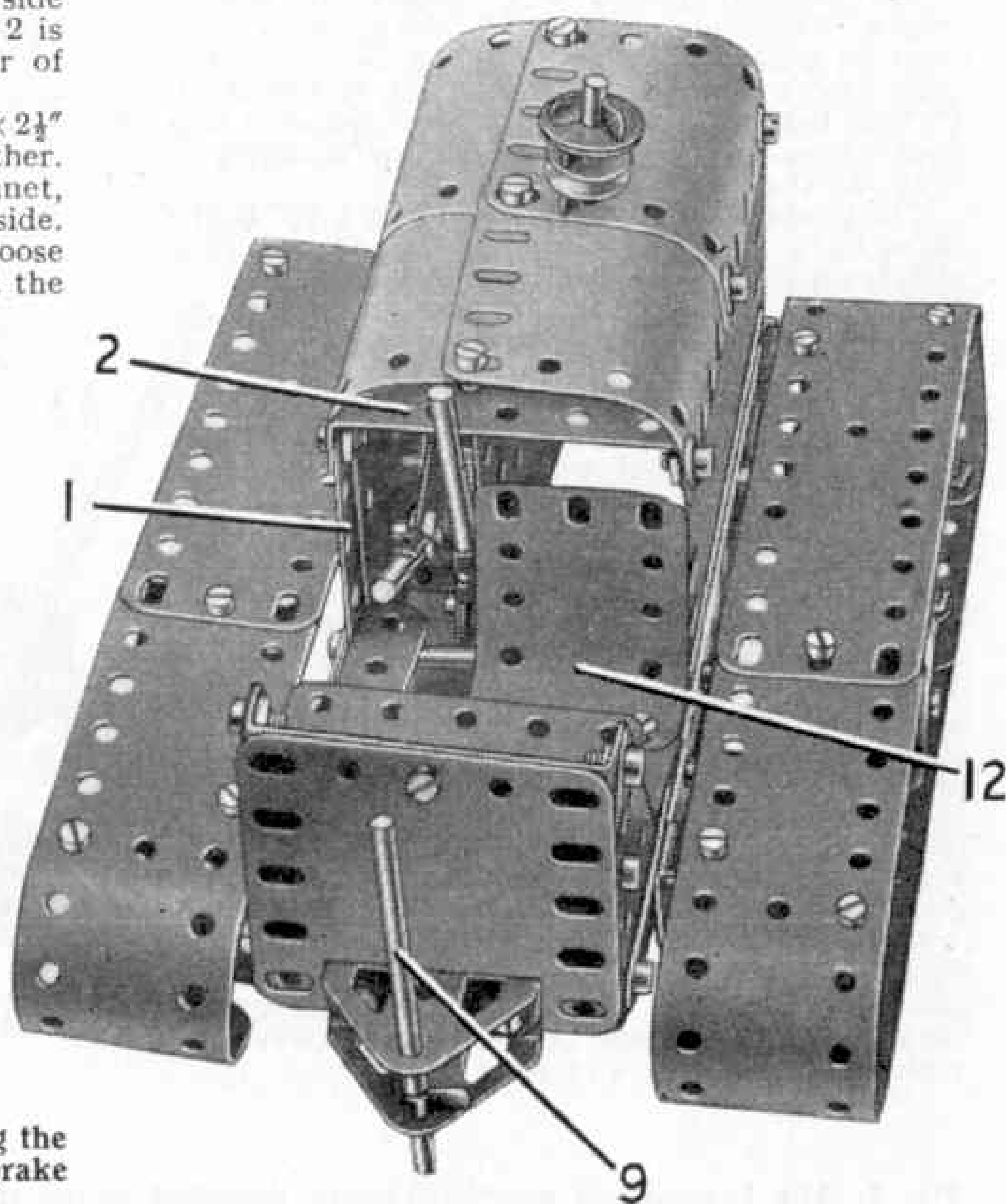
(Above) Fig. 1. This fine Tractor and Bottom Dump Truck can be built with Outfit No. 6, and is driven by a No. 1 Clockwork Motor.
