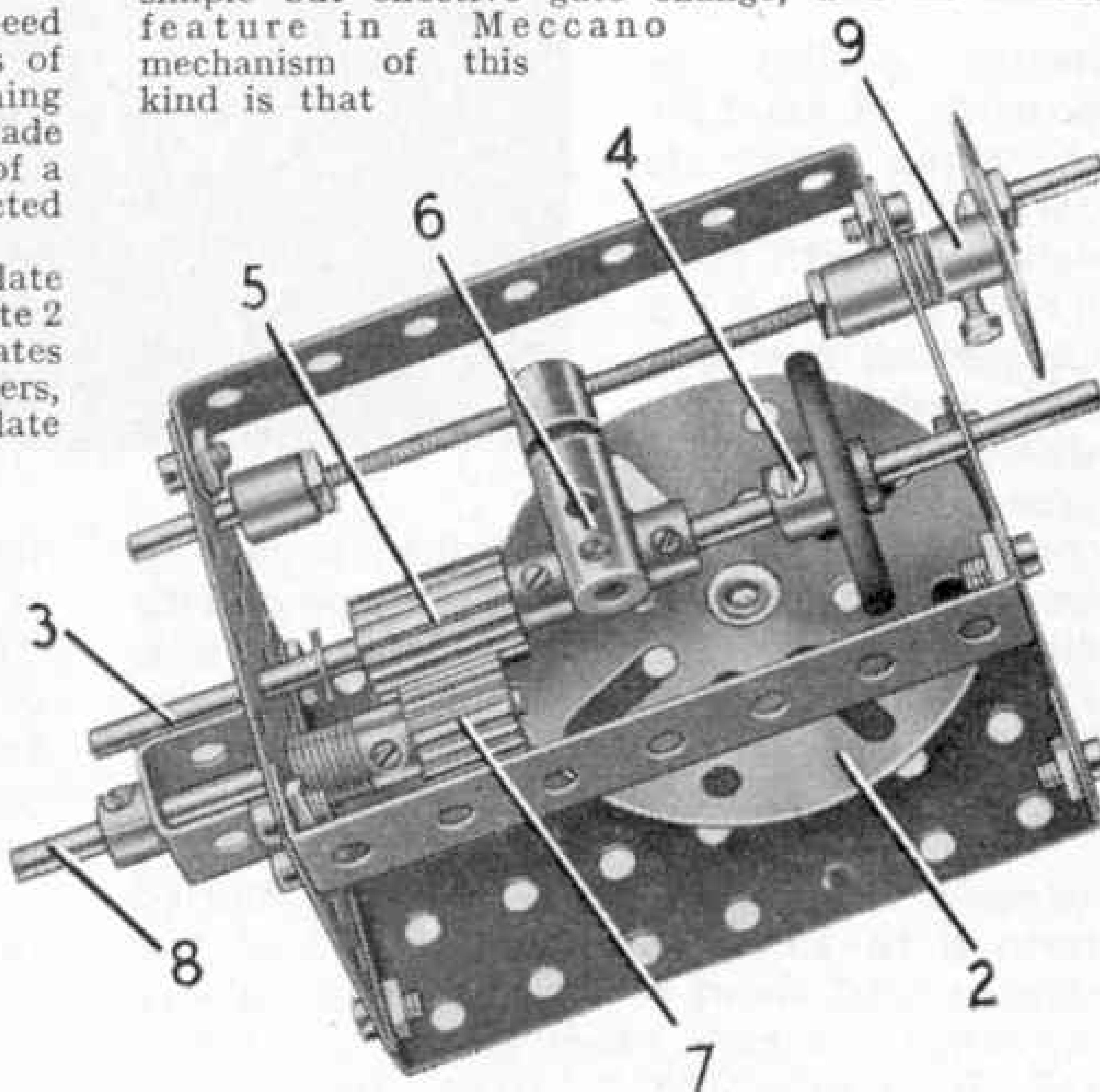
Fig. 3. Another view of the variable speed gear.
