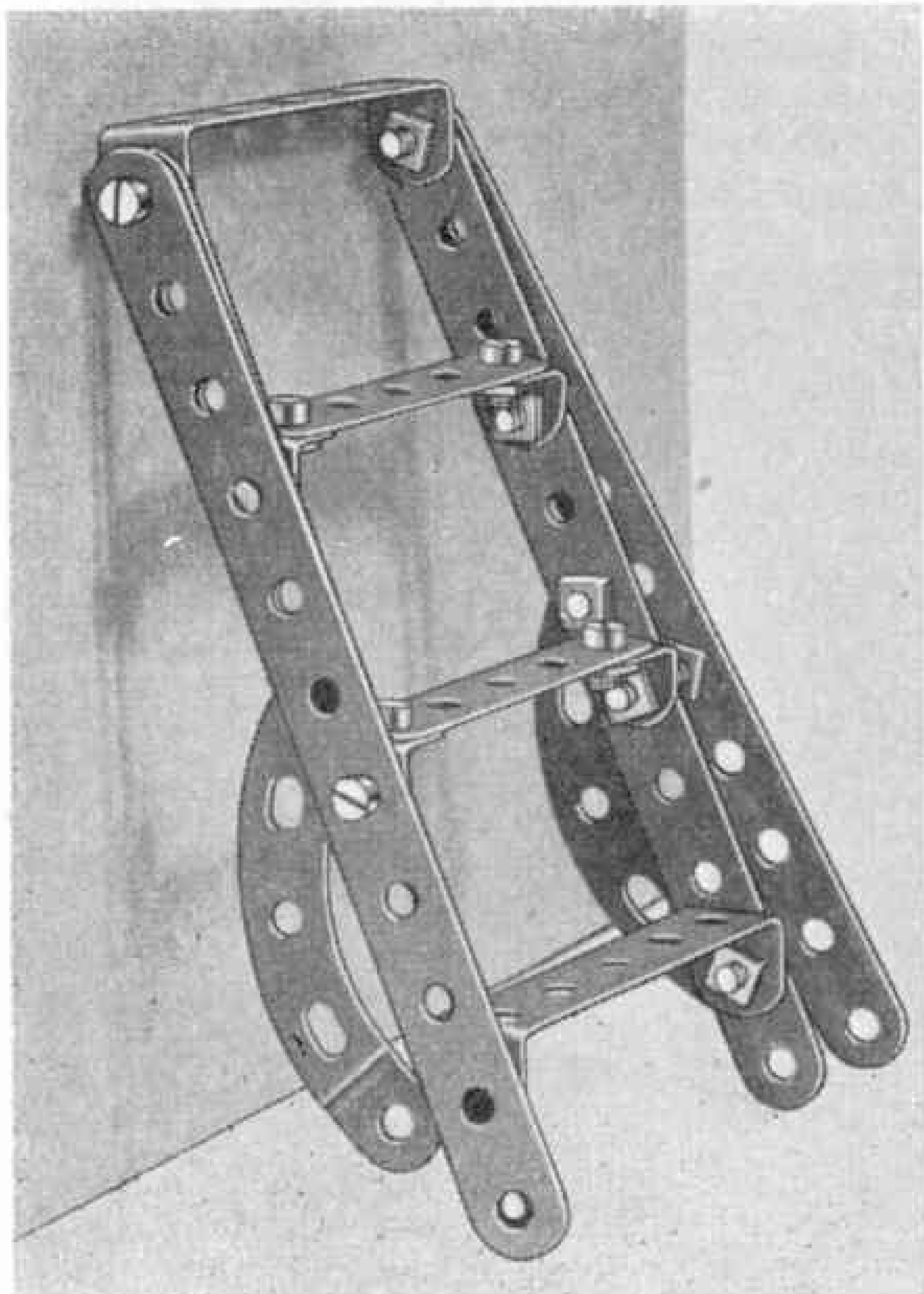
No. 1. The stepladder in the folded position.
