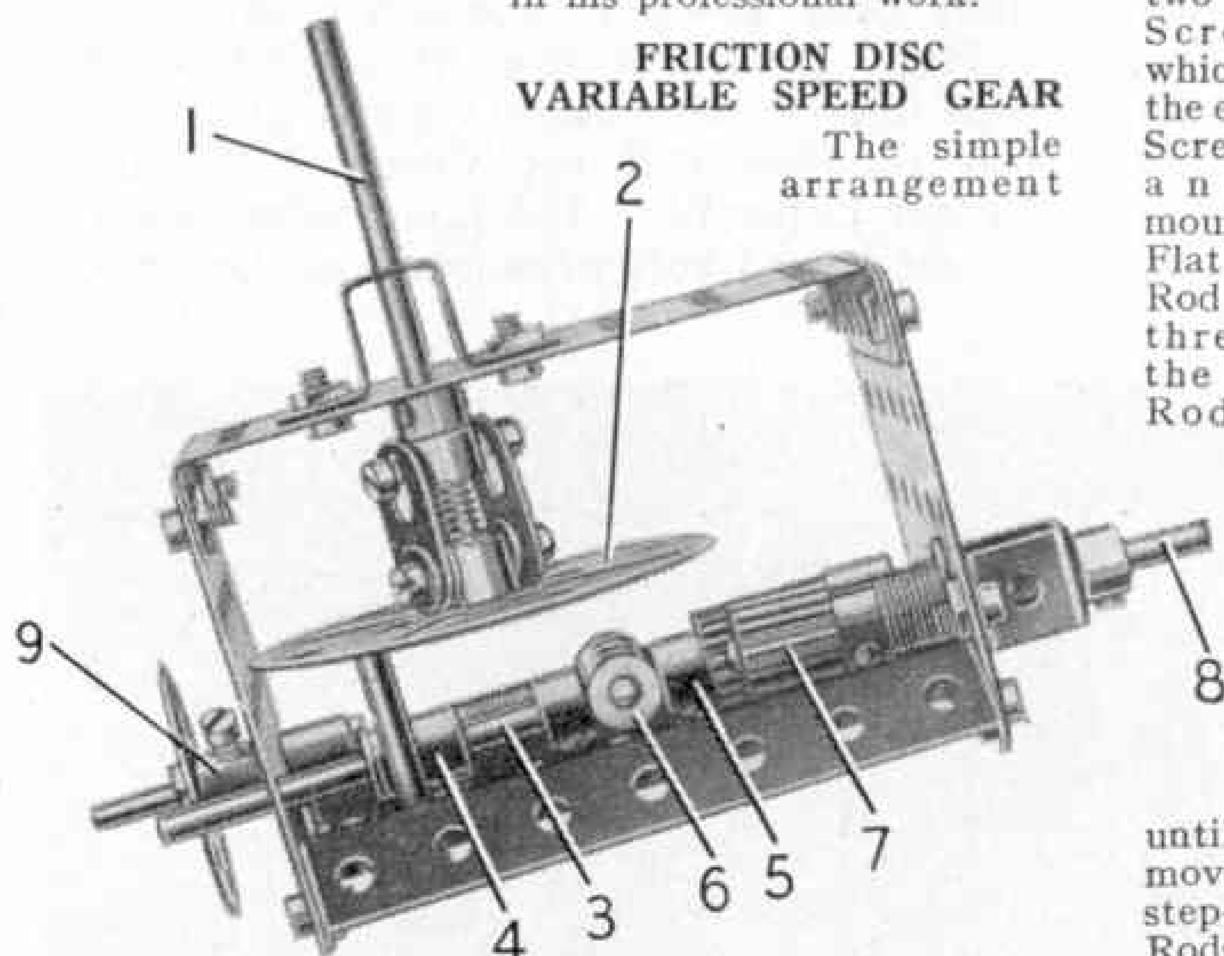
Fig. 2. A friction disc variable speed gear.
