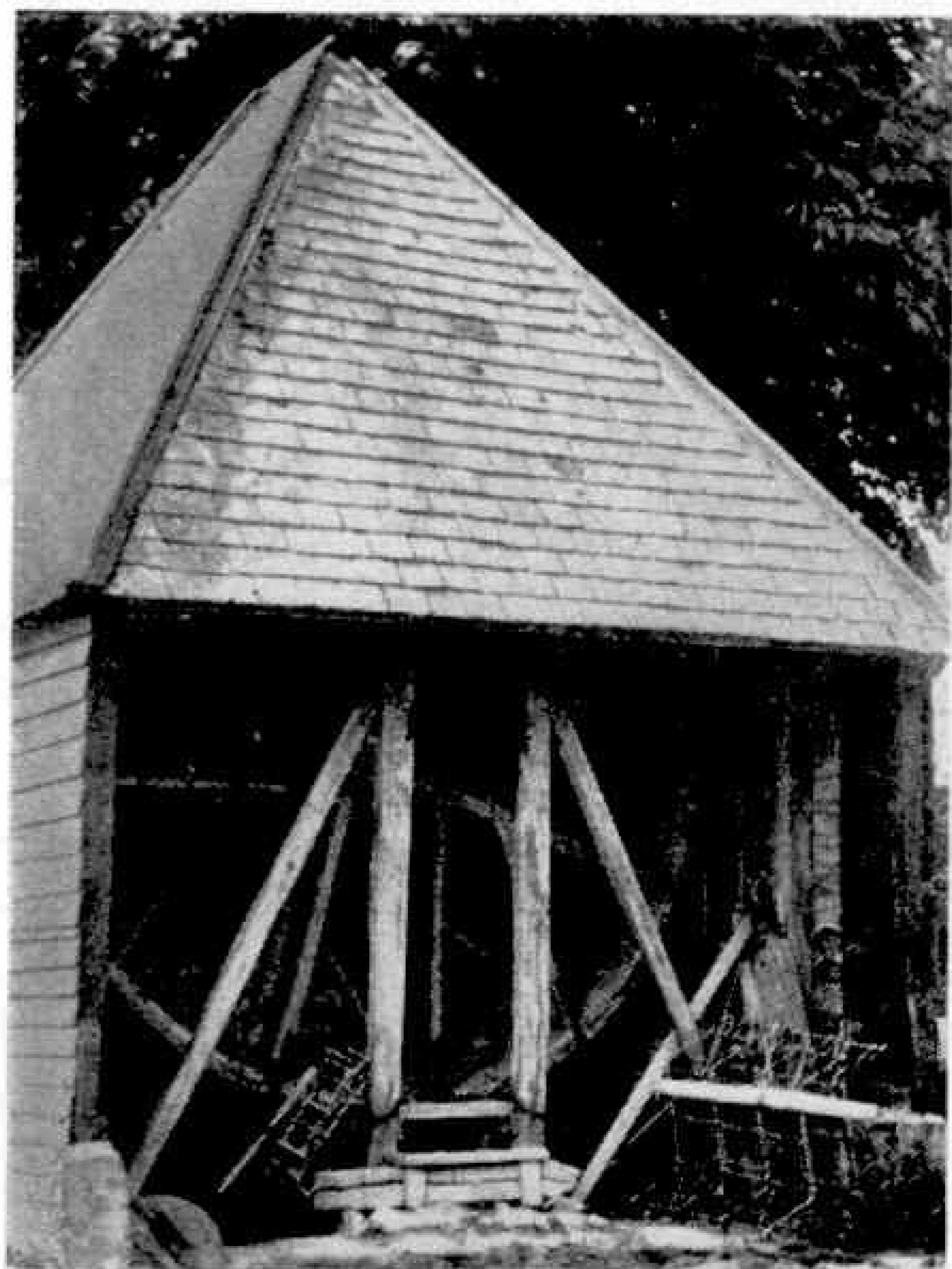
The donkey wheel at Saddlescombe farm, which pumped water until comparatively recently. Photograph by A. Phillip, Hassocks.
