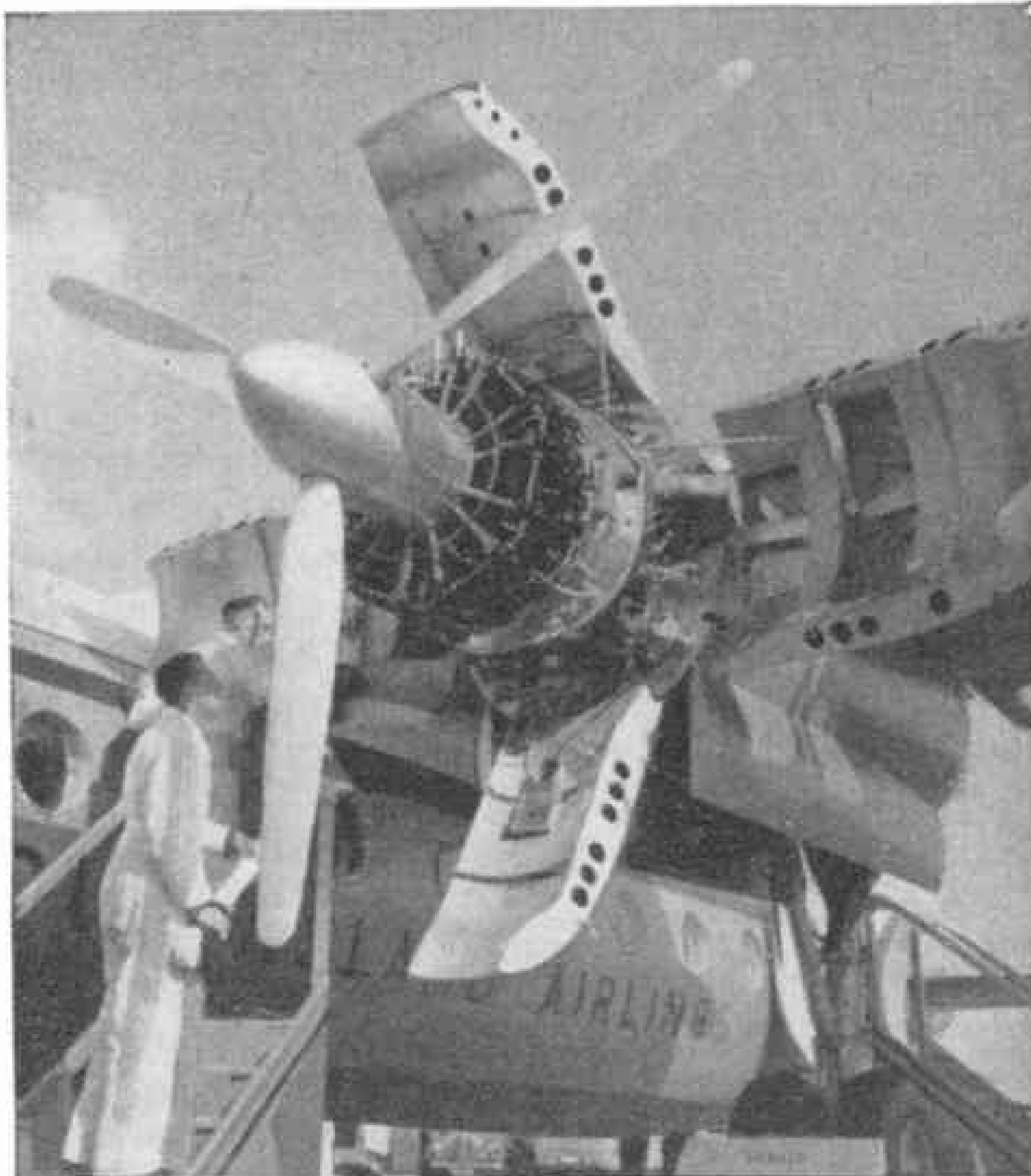
Handley Page Herald of the type ordered for Air Kruise, showing the "petal" engine cowlings open. A Shell photograph.
