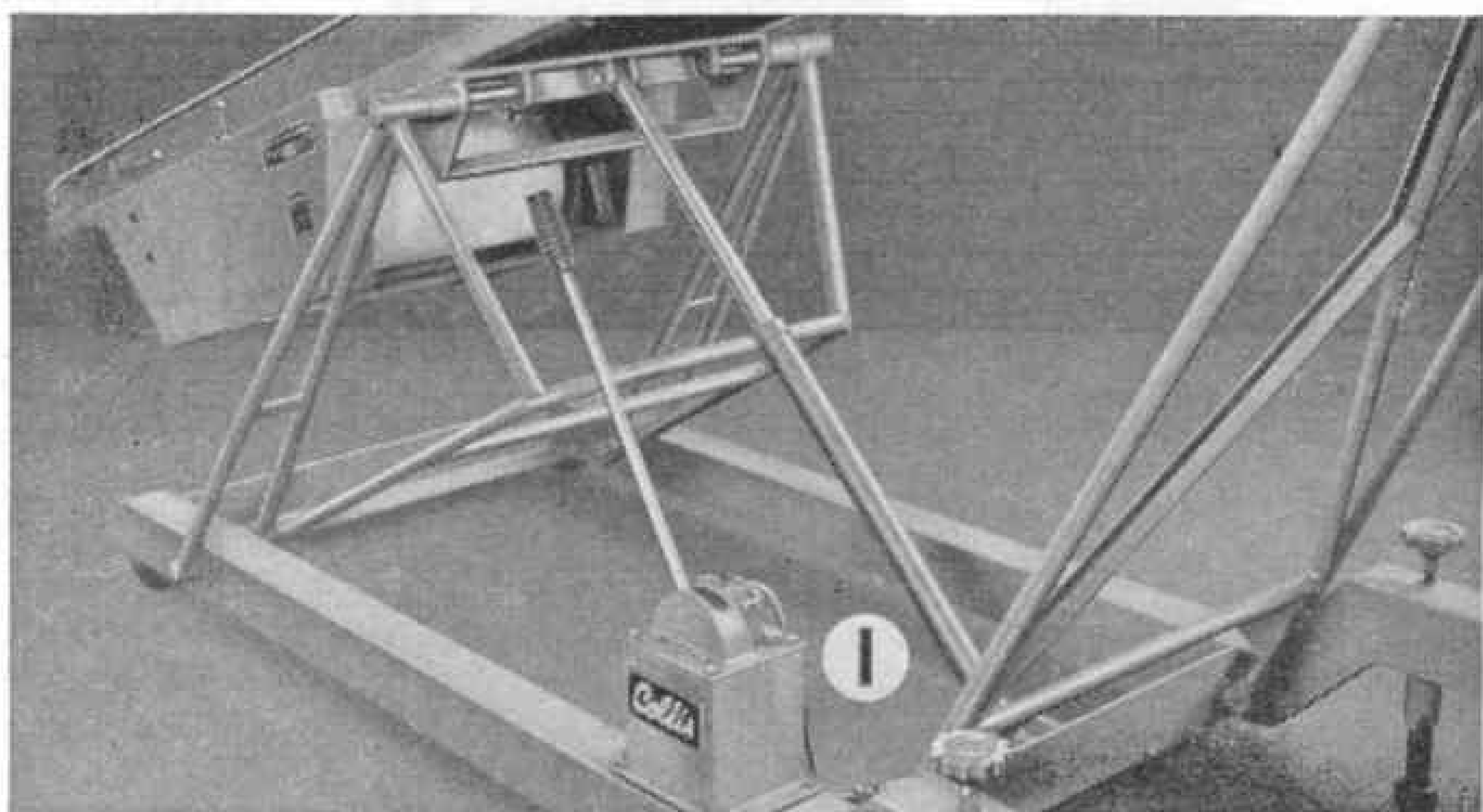
Fig. 3. The cradle on which The LoadaVeyor boom is pivoted is raised by the Collis Hydraulic Unit, the lever of which is seen on the near side at the centre of the picture.
