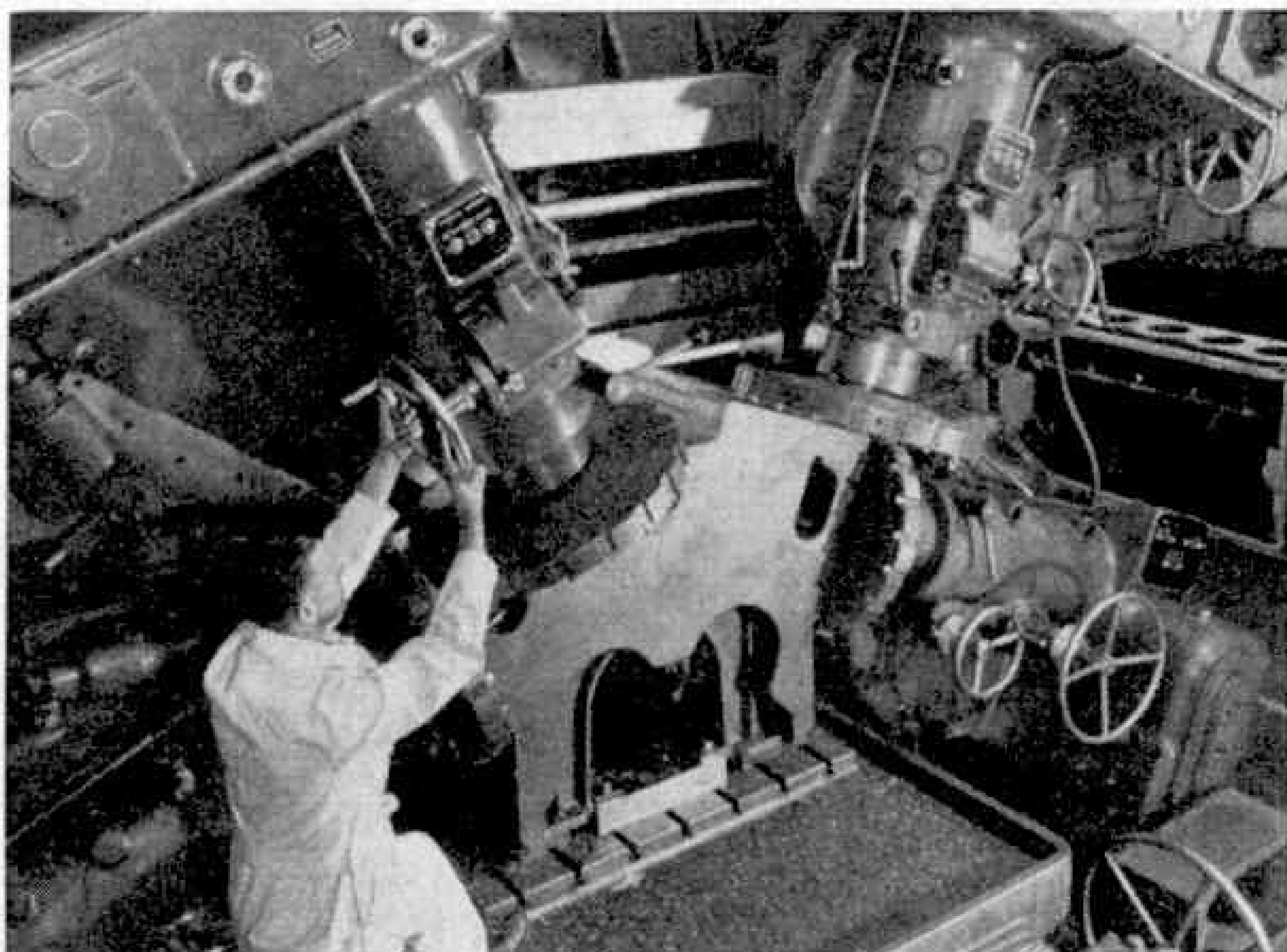
The four cutting heads of a plano-miller machining the faces of a cylinder housing for a large Diesel engine at the works of Mirrlees, Bickerton and Day Ltd., Hazel Grove, Cheshire.
