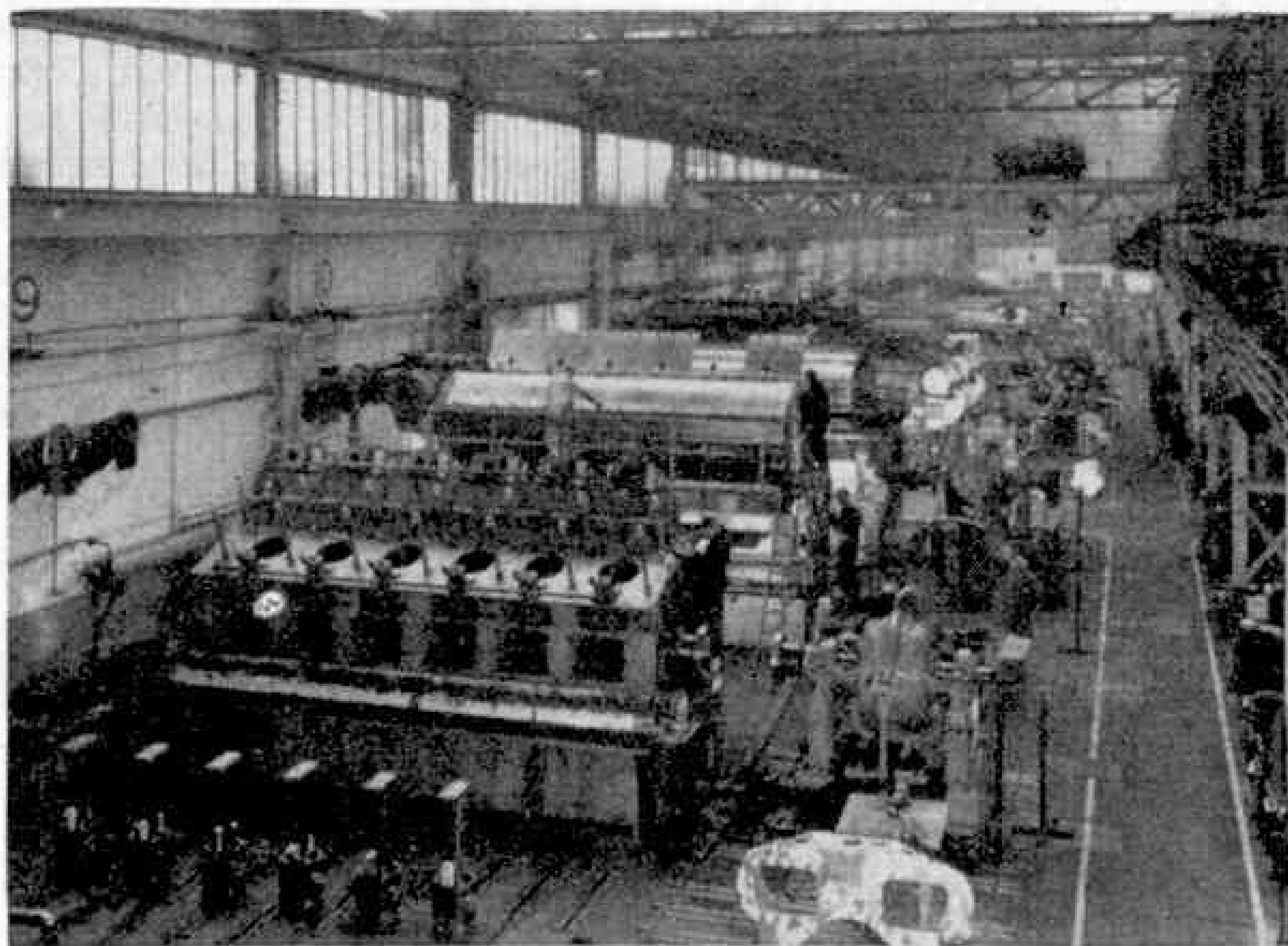
Test bays in which the final erection and testing of heavy diesel engines are carried out.
