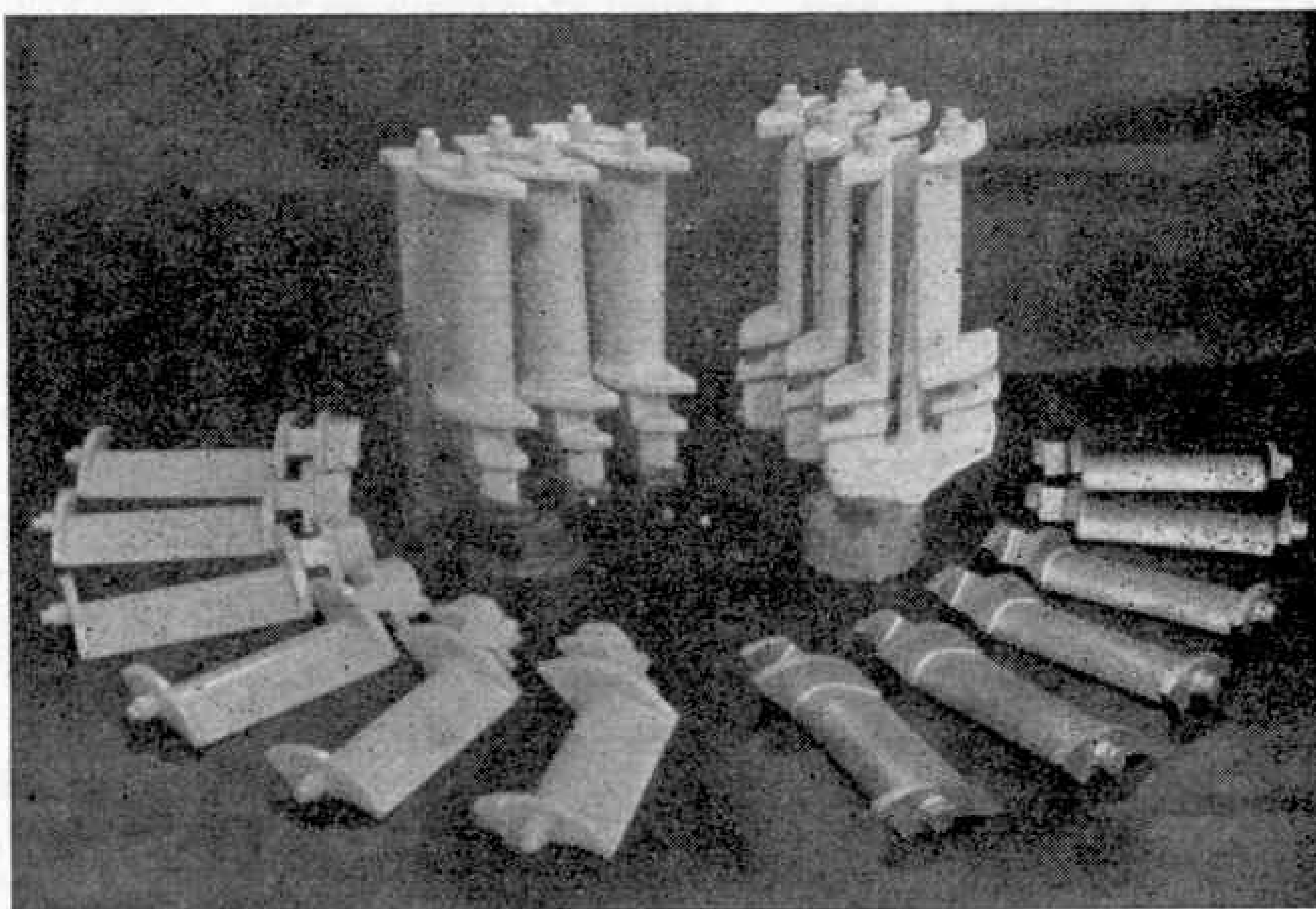
Wax patterns of turbo-jet blades. An early stage of making jet engine blades by the lost wax process, described in this article, is the assembly of the patterns in clusters, as shown in the background.
