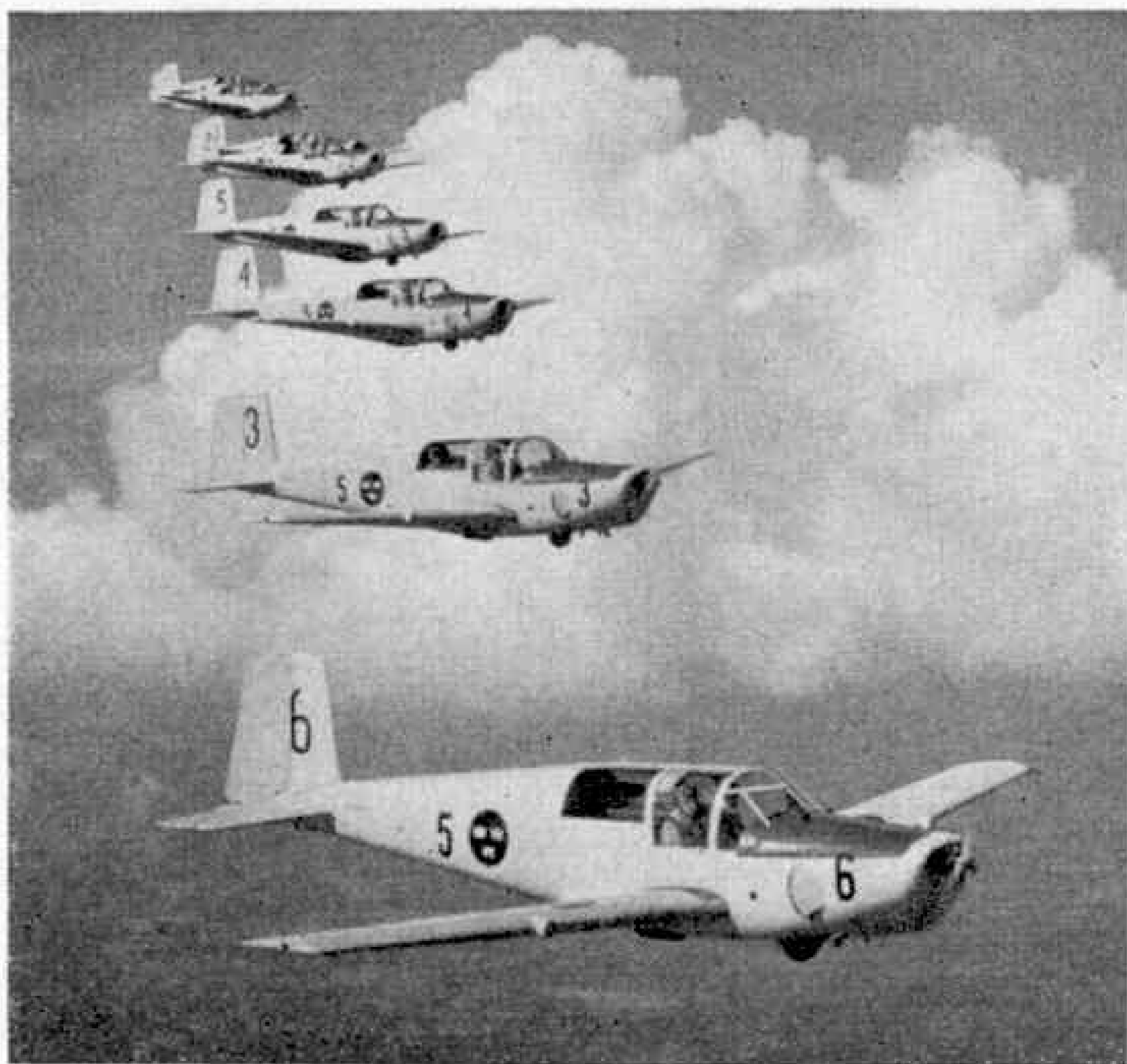
Formation practice by SAAB-91B Safir three-seat training aircraft of the Royal Swedish Air Force. Note the semi-retractable nose wheel which enables the aircraft to make a safe belly landing, with its main wheels retracted, in an emergency. Photograph by courtesy of SAAB, Linköping, Sweden.
