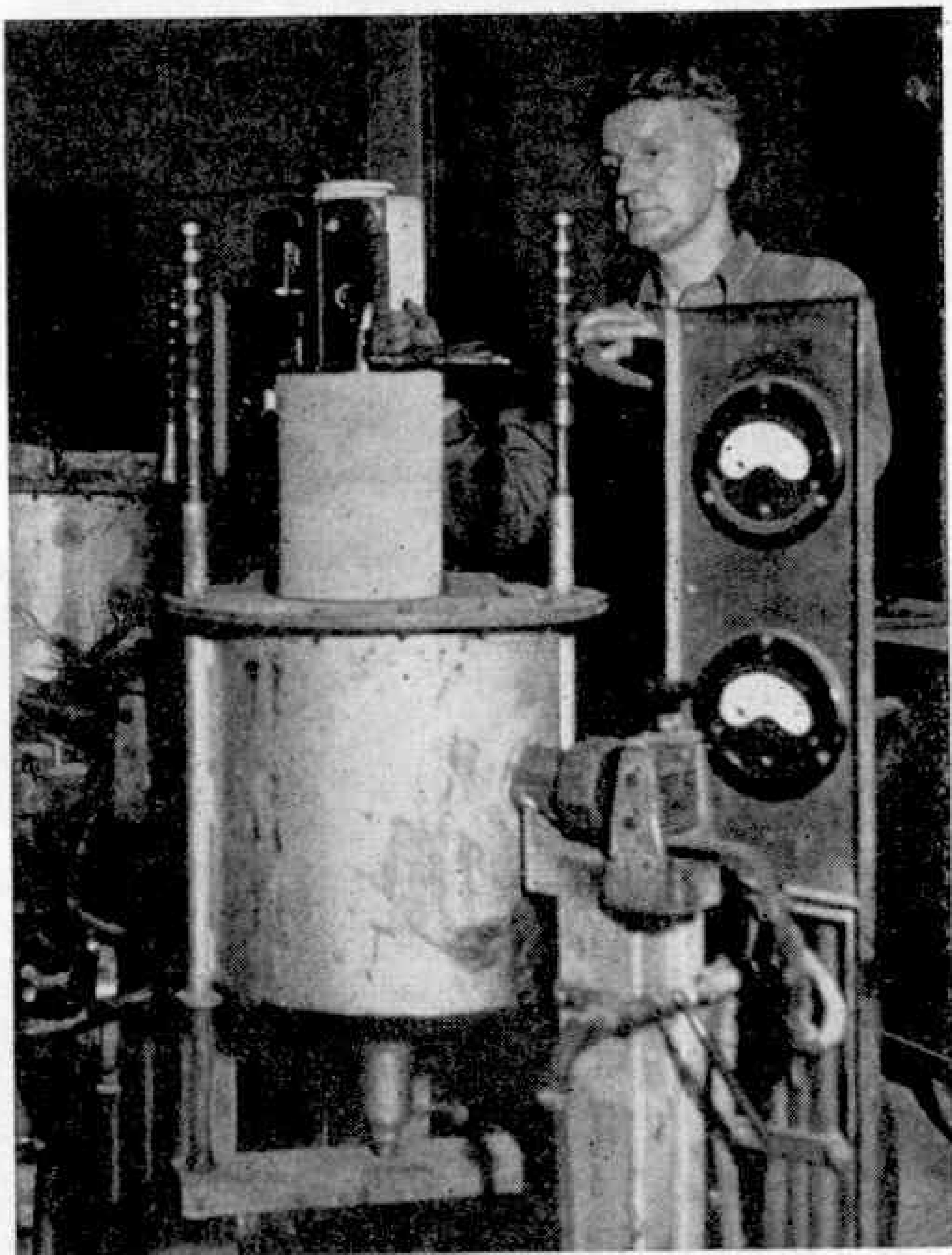
The mould is clamped on top of an arc furnace, and the whole arrangement is inverted, so that molten metal pours into the mould to form the blade.
