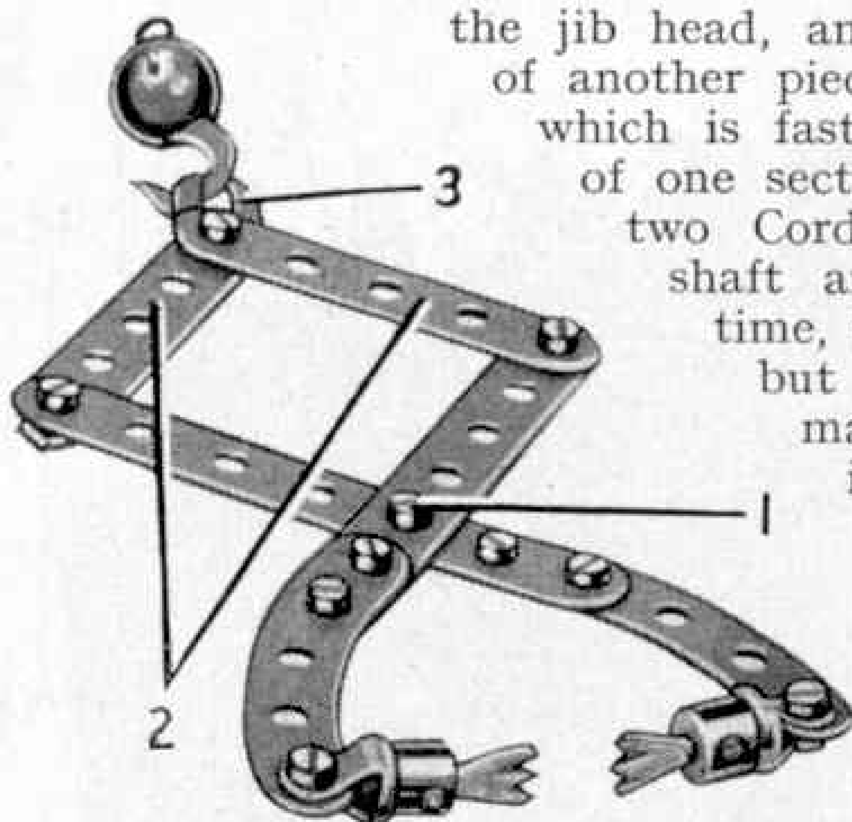
Fig. 4. A pincer grab for model cranes.
