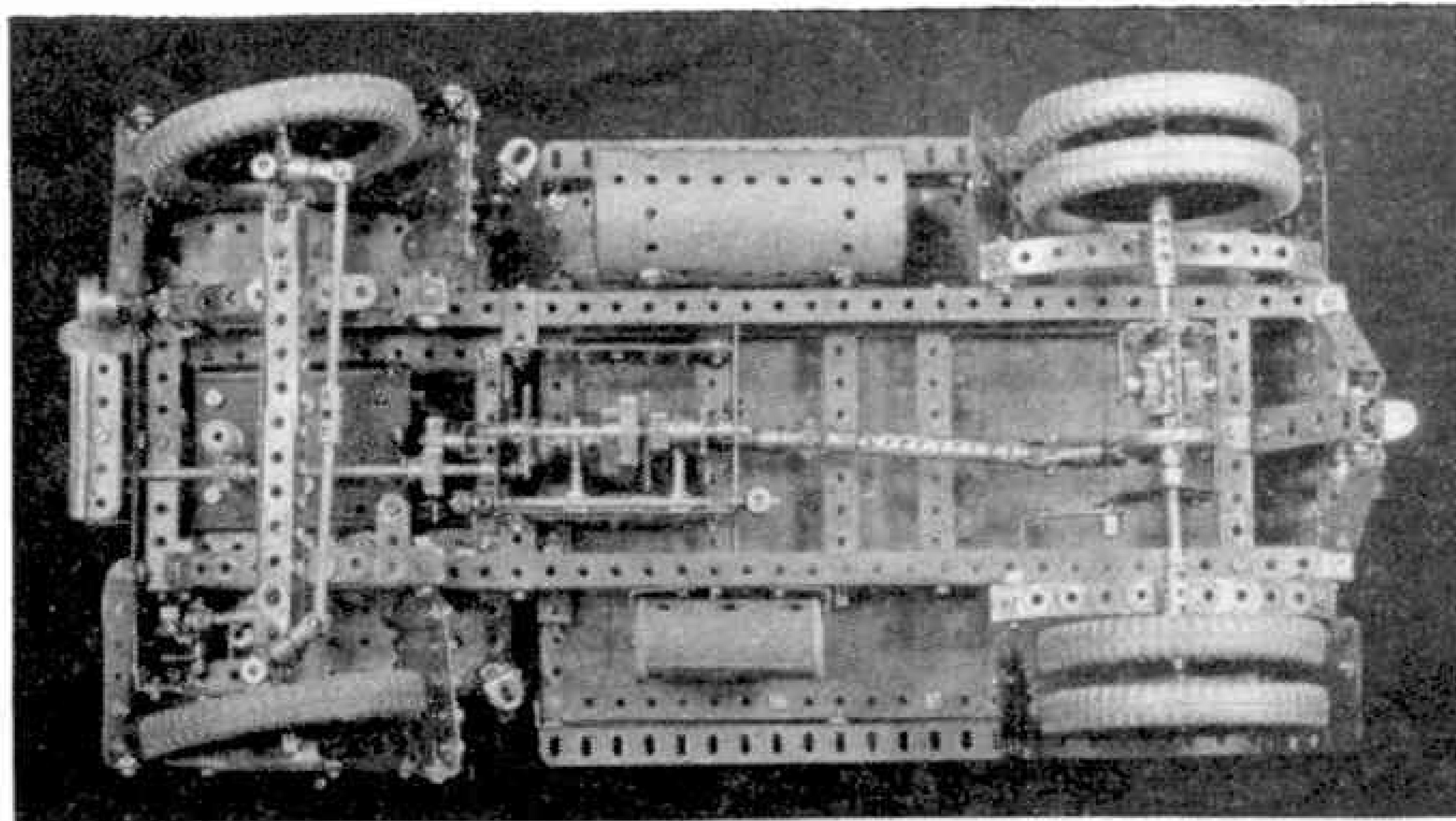
The well-detailed chassis of the Breakdown Lorry built by Mr. Smith.
