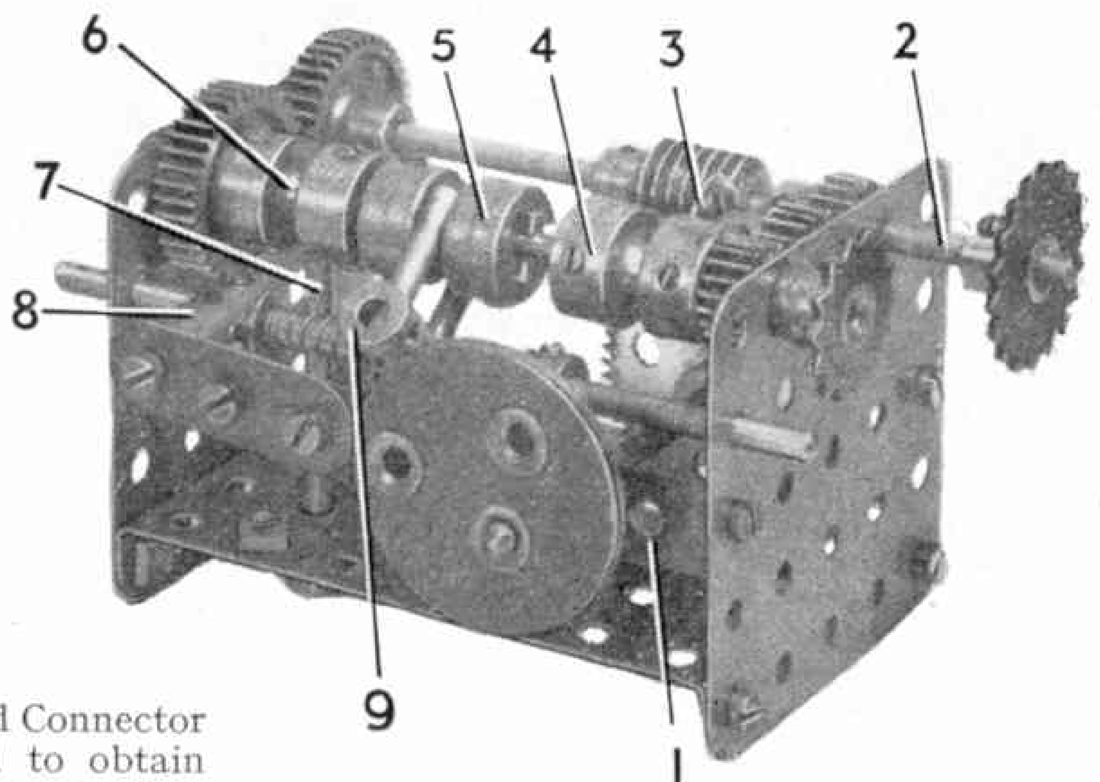
Fig. 3. Another view of the automatic reversing gear-box.
