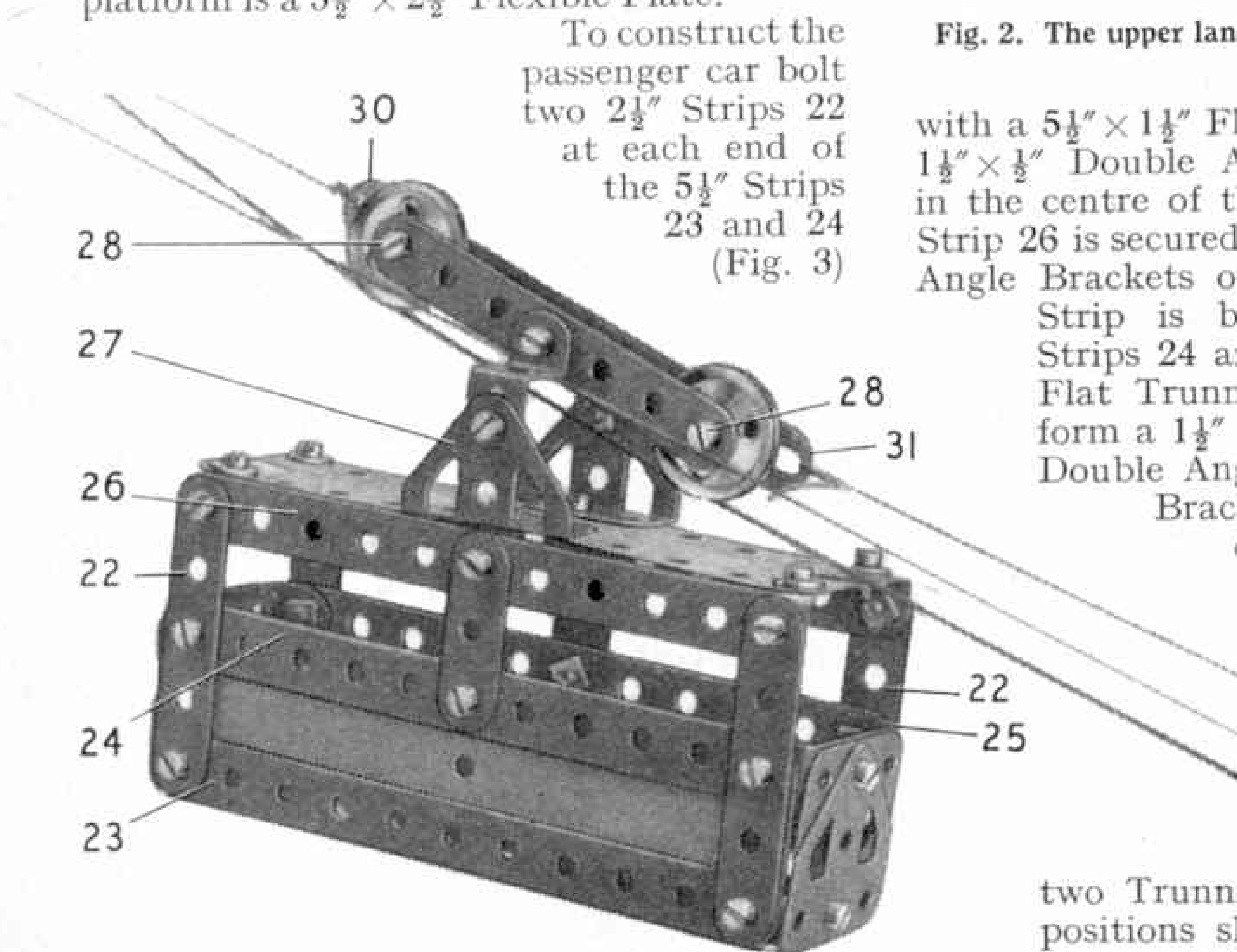
Fig. 3. The passenger car of the Aerial Cableway. Note particularly how the hauling cord is attached.
