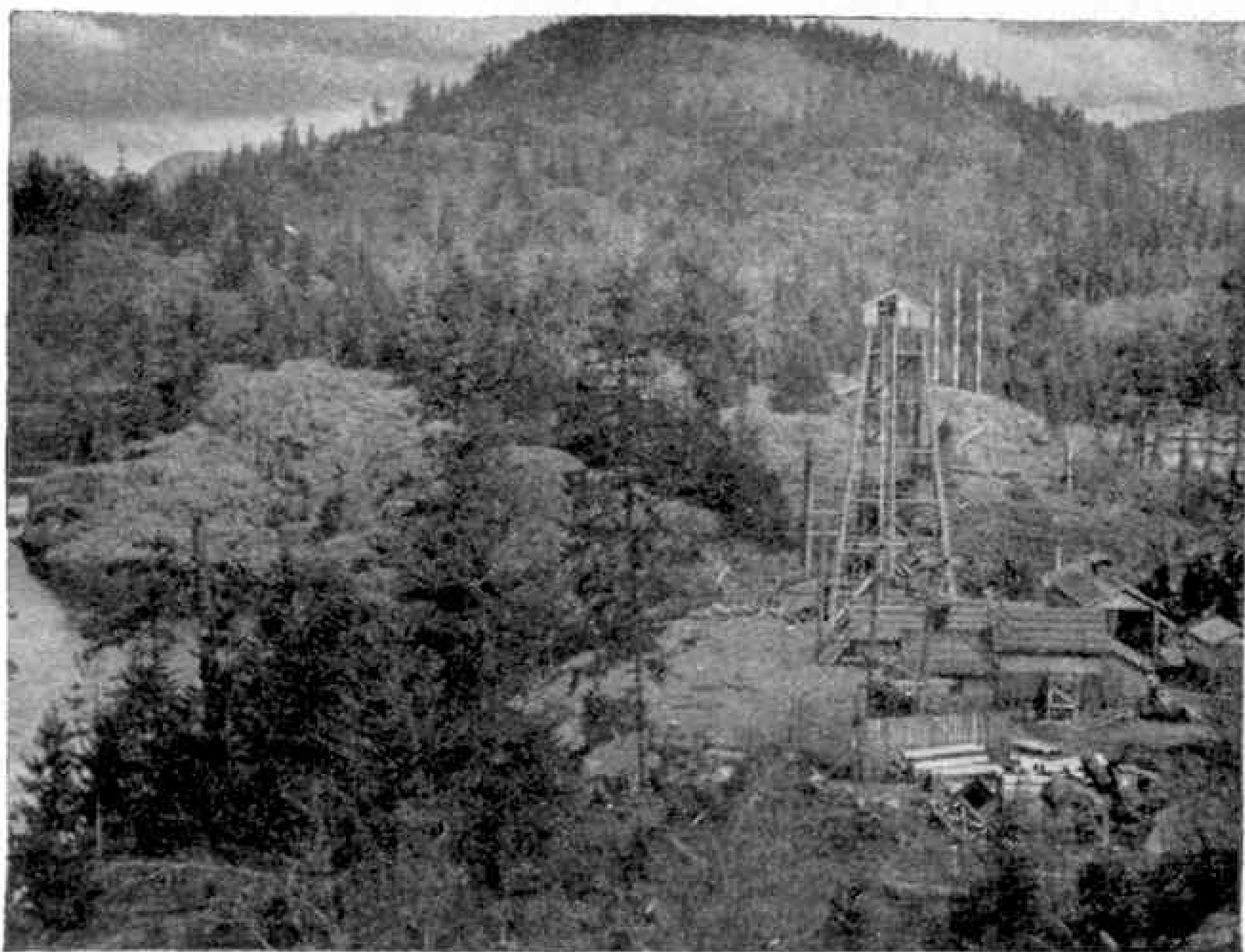
The vertical shaft from the installation in this picture descends 572 ft., and from the bottom a 300 ft. tunnel leads to a maze of galleries packed with explosives inside Ripple Rocks, an underwater mountain in the waterway between Vancouver Island and the mainland of Canada that was eventually blown to pieces. Illustrations from photographs by the author.
