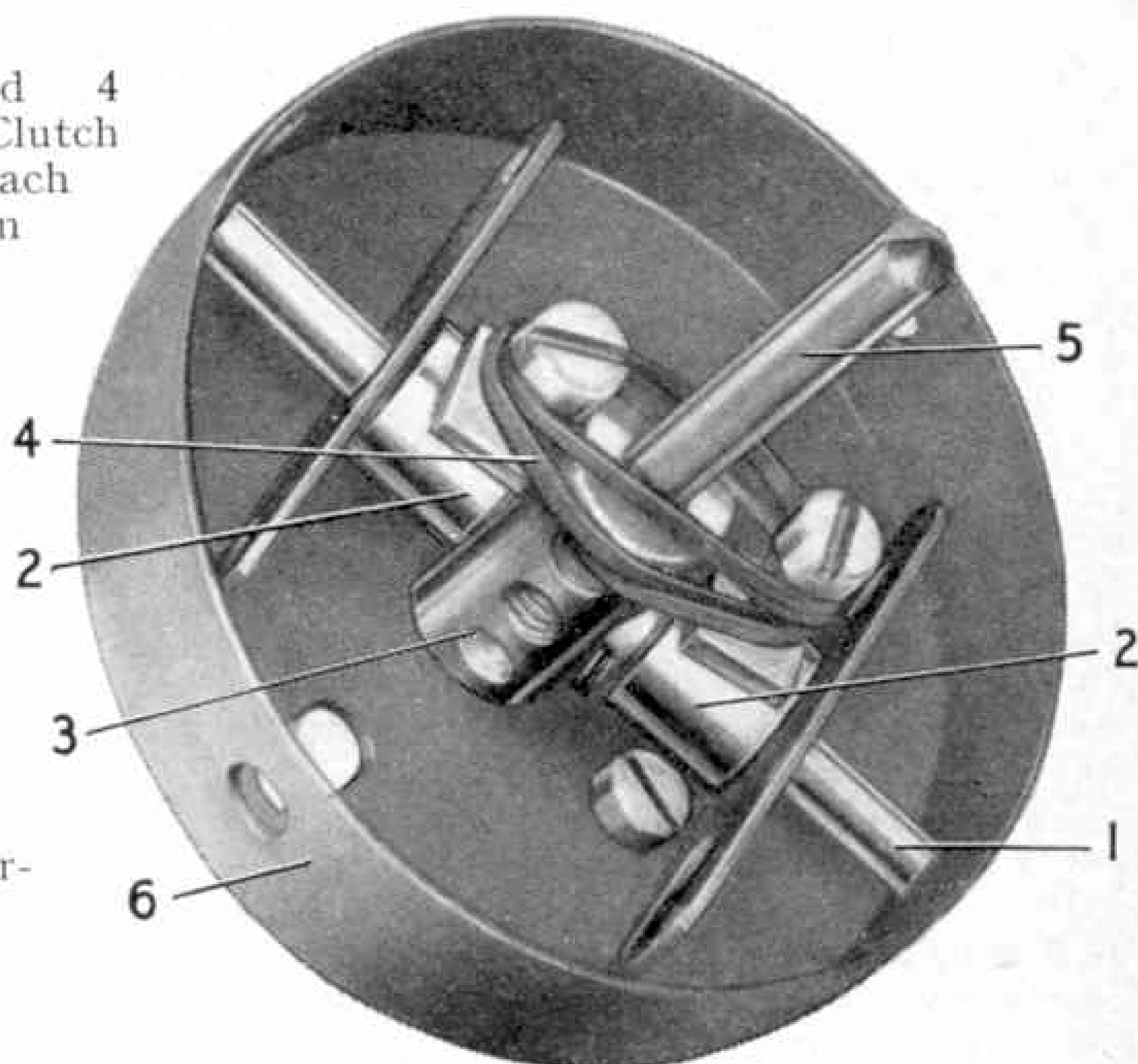
Fig. 3. A centrifugal clutch suitable for light drives.
