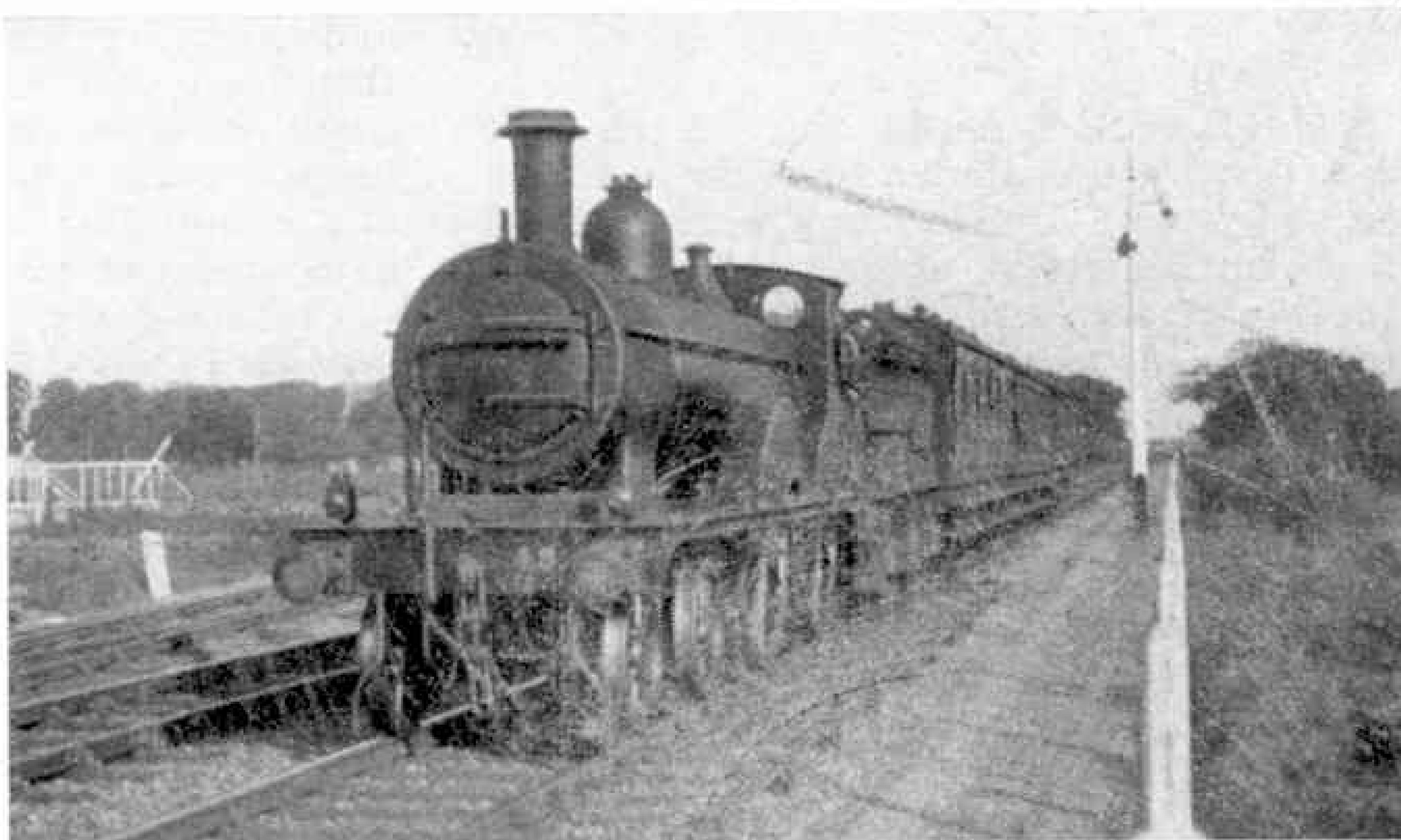
The Johnson origin of Midland and Great Northern 4-4-0 No. 43 is clearly apparent in this photograph taken in 1930 by G. H. Marillier. The engine is on a Bourne train near Sutton Bridge.
