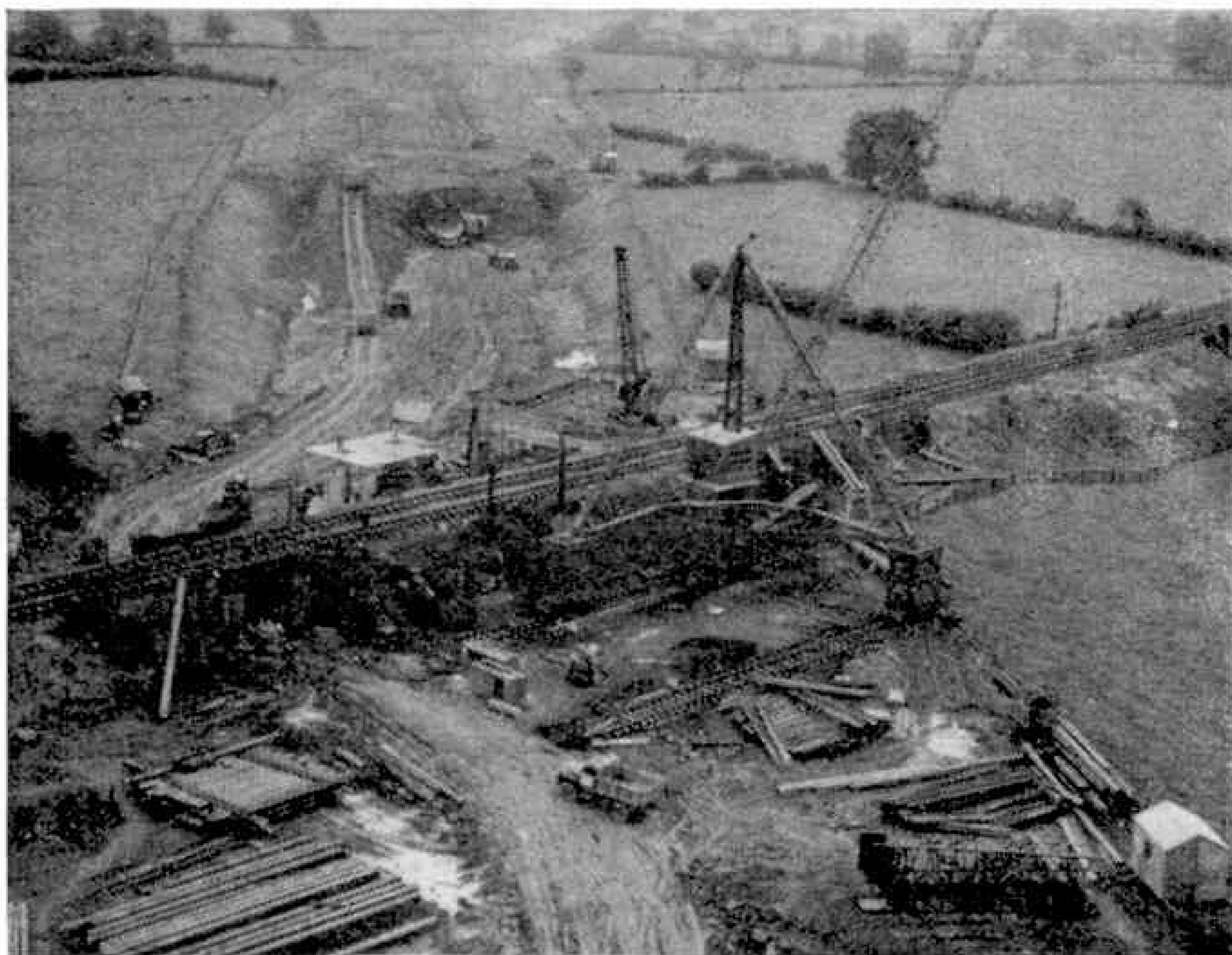
Work in progress on a railway crossing. The illustrations to this article are reproduced by courtesy of John Laing and Son Ltd., the builders of the 53-mile length of the Motorway between Luton and Ashby St. Ledgers.
