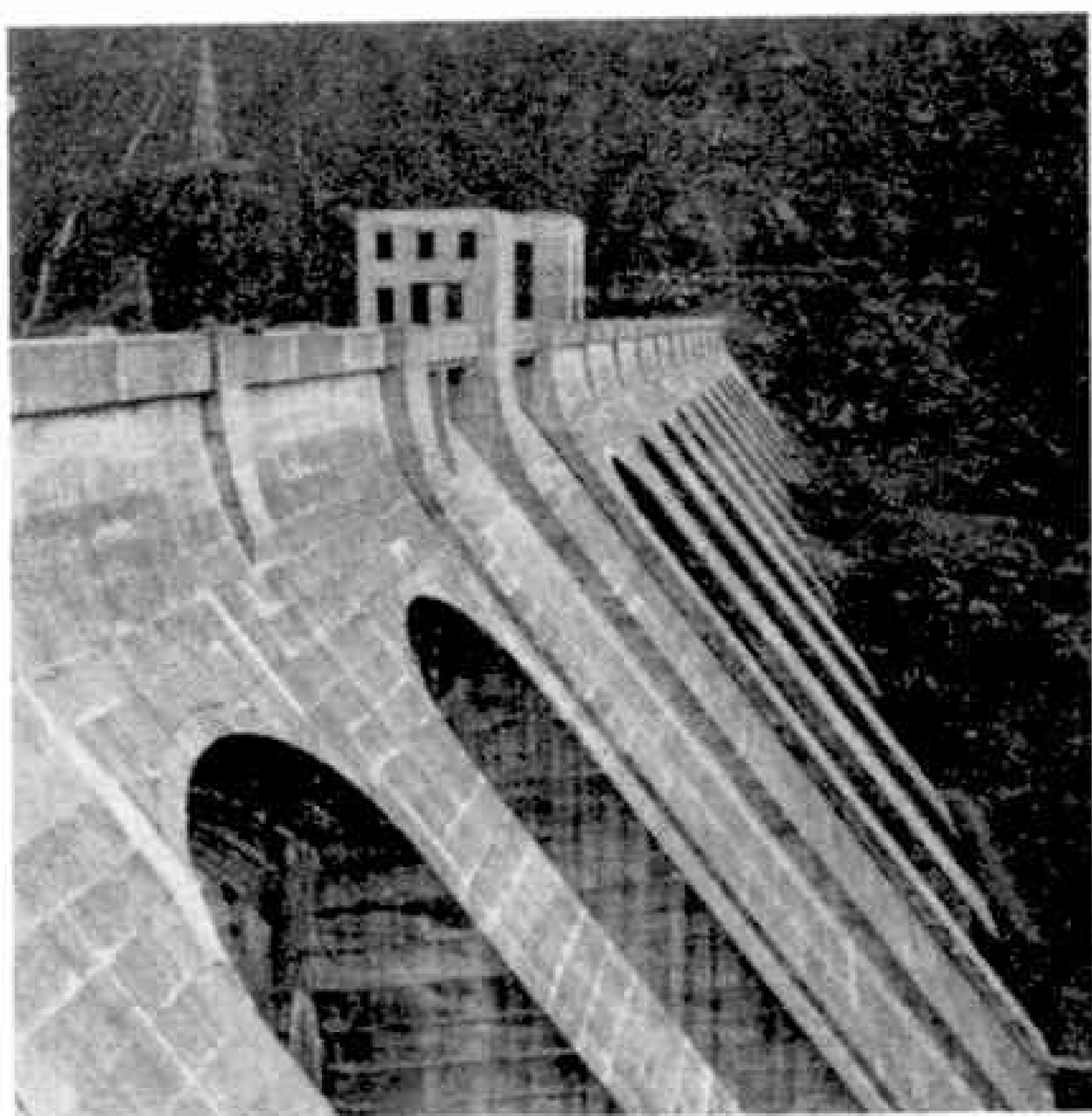
The dam of the Loch Sloy hydro-electric scheme, photographed by F. M. Cazalet, Bingley.
