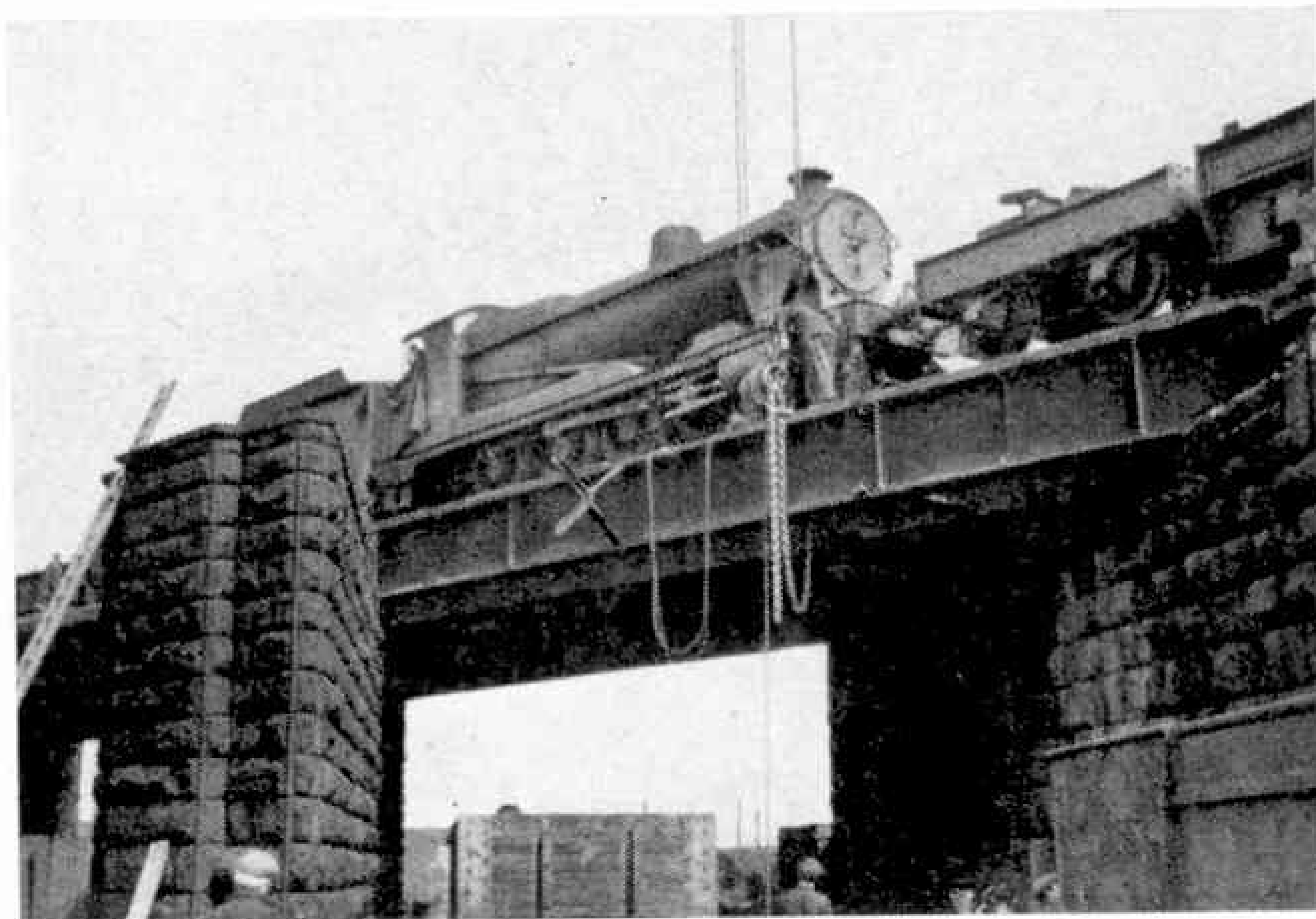
On real railways bridge work often calls for the use of a breakdown crane, as in this picture. One of the relieving bogies of the crane concerned is seen next to the engine. Photograph by K. Field.
