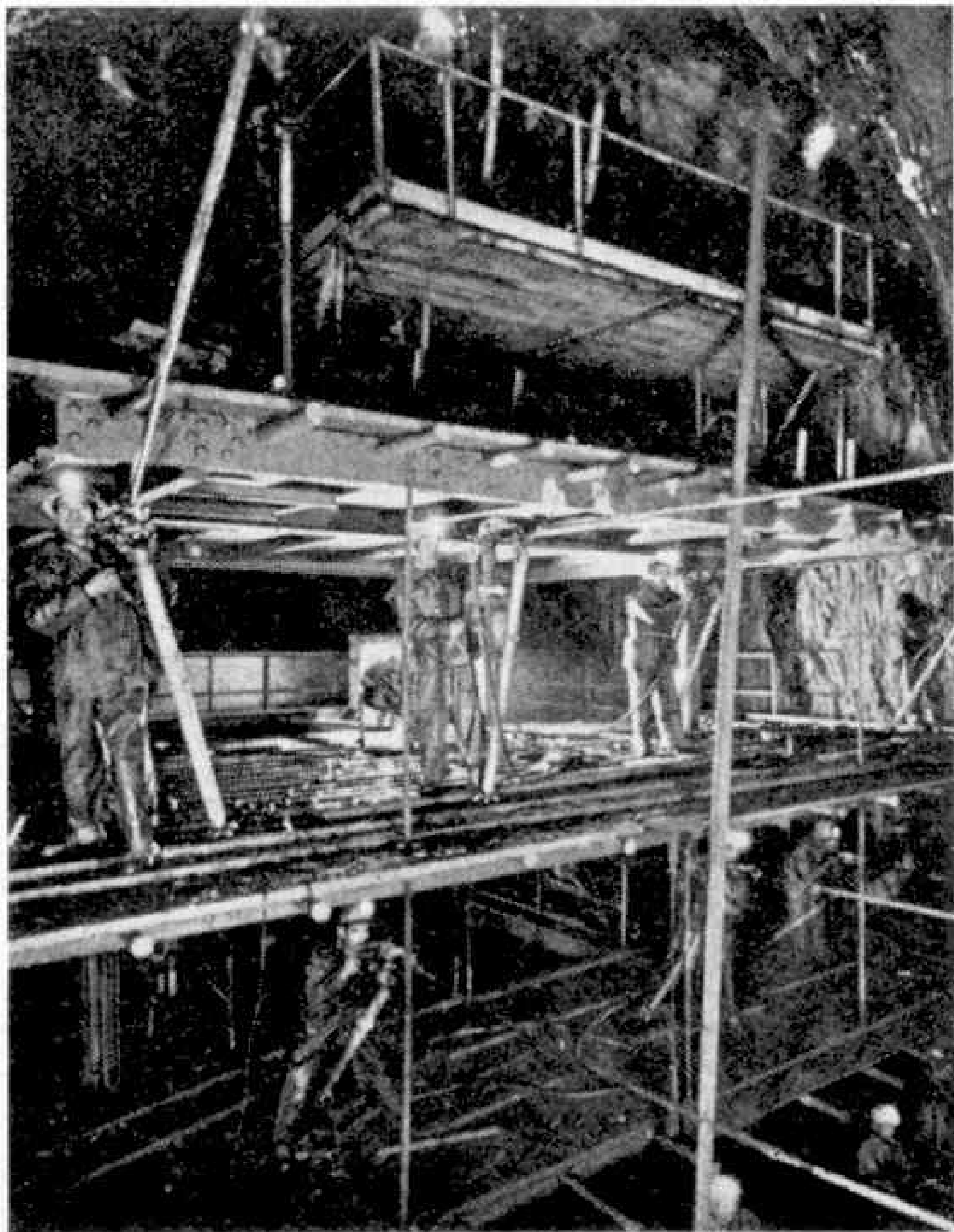
The drilling Jumbo in use in the section of the tunnel now being bored from the Italian side.
