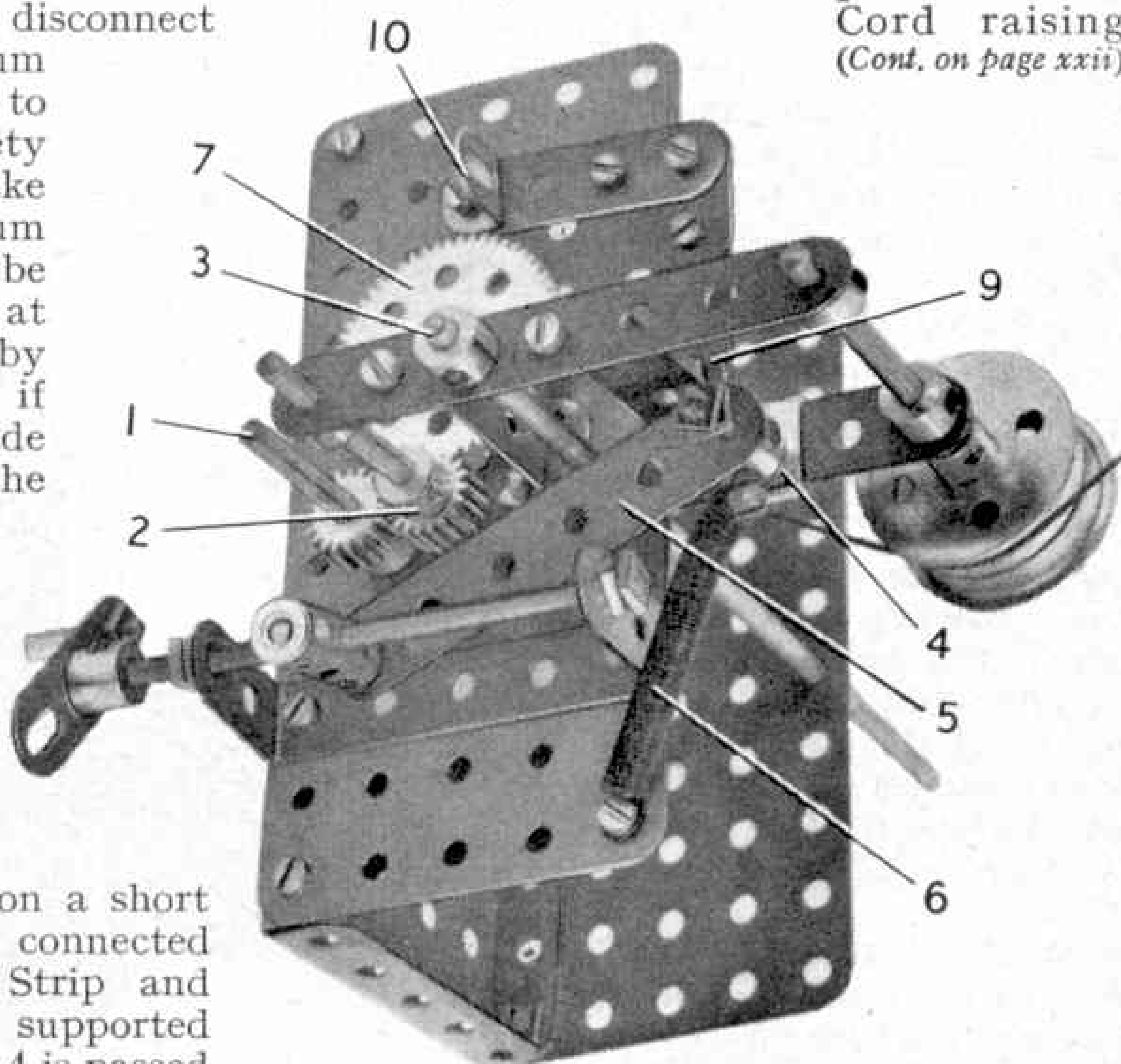
Fig. 3. Another view of the crane safety device.
