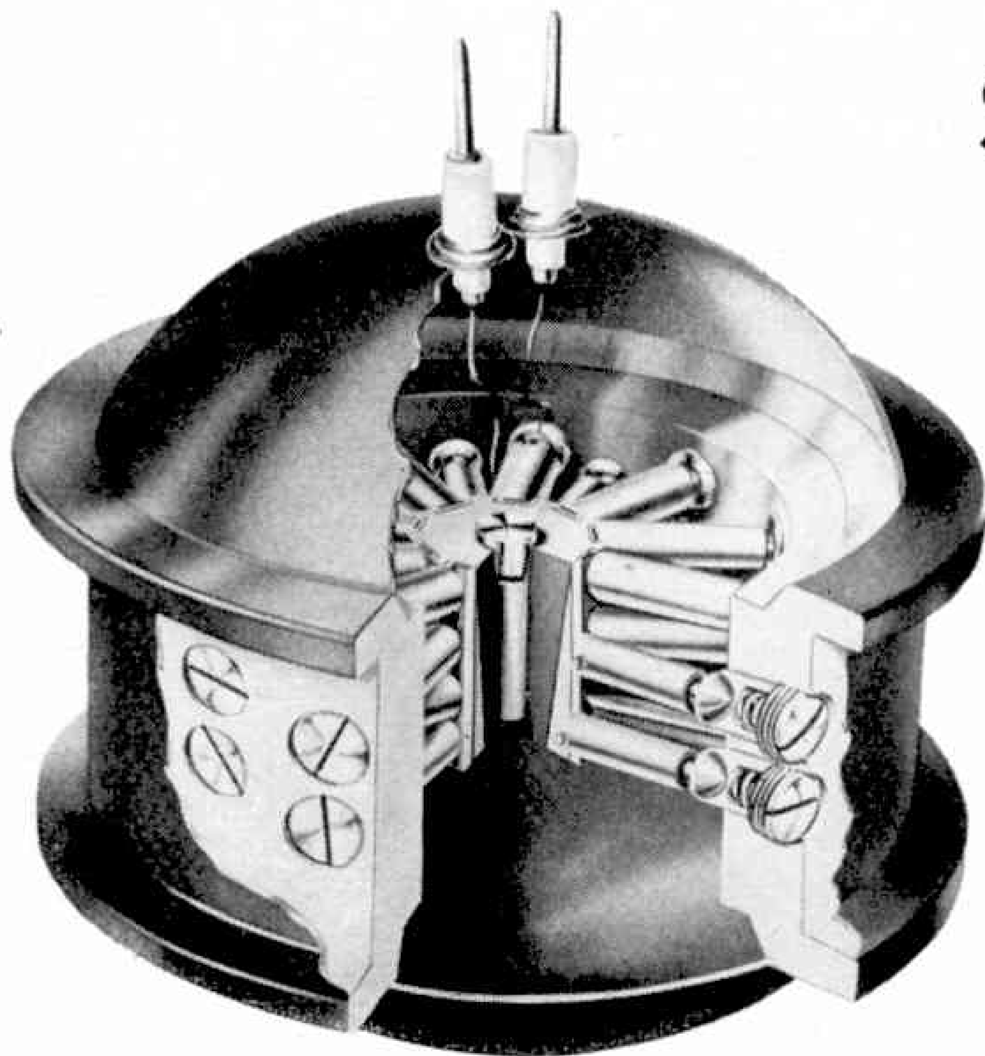
This drawing of SNAP-III, reproduced by courtesy of the Martin Company, shows the central radioisotope holder with thermoelements round it and two output connections at the top.
