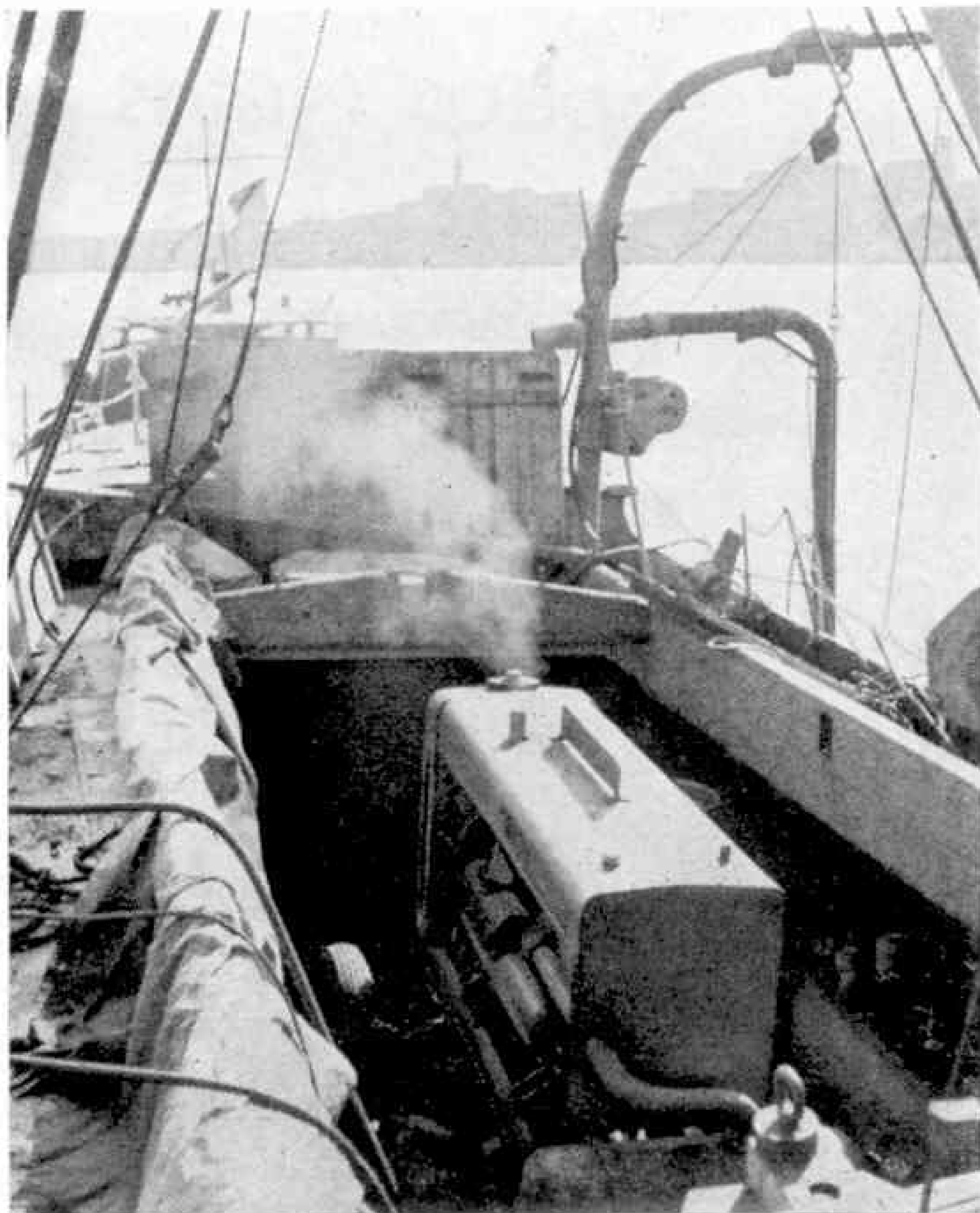
Compressed air for use in the salvaging of the "Vasa" came from this Atlas Copco compressor.
