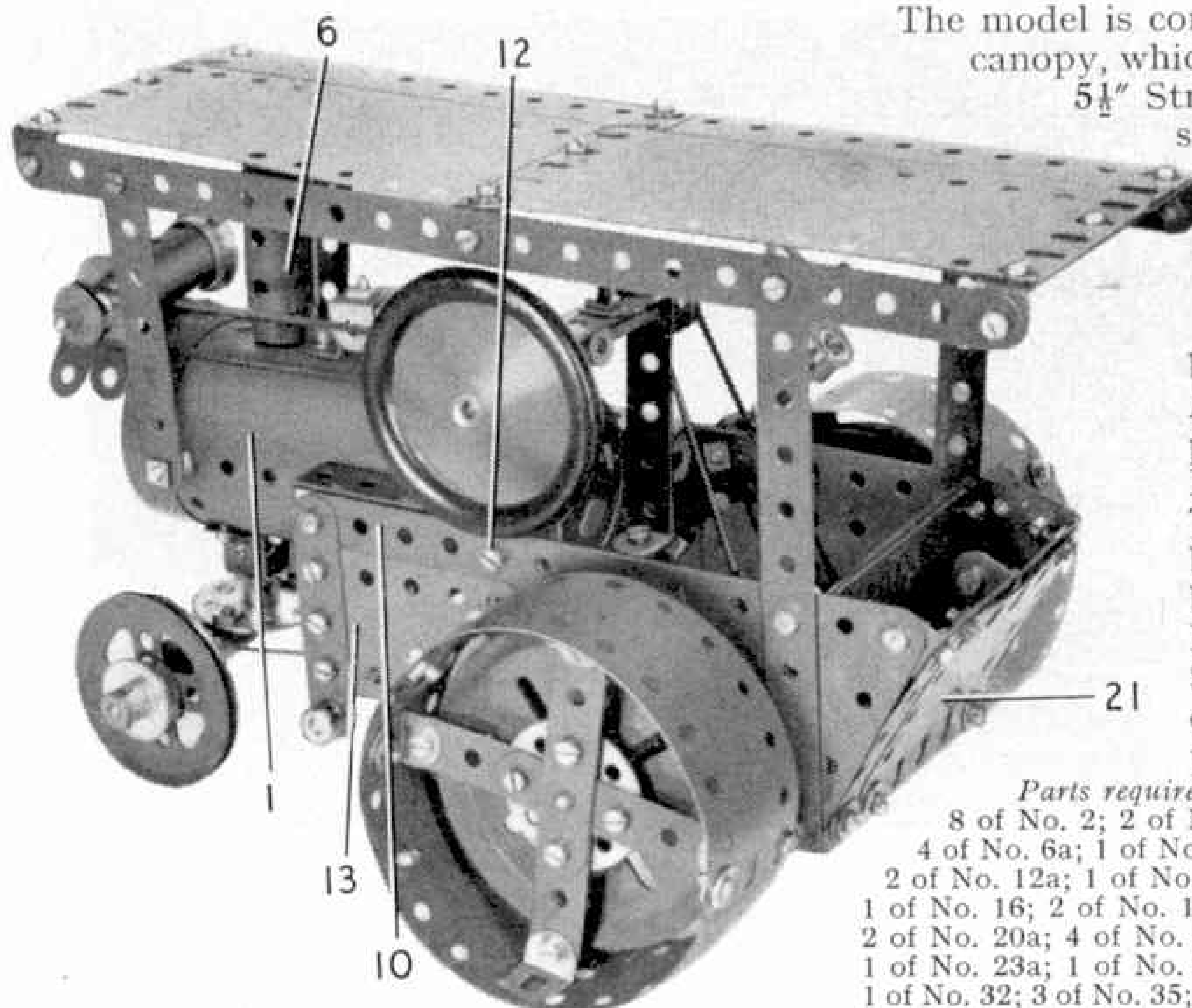
Fig. 2. The near side of the Traction Engine.
