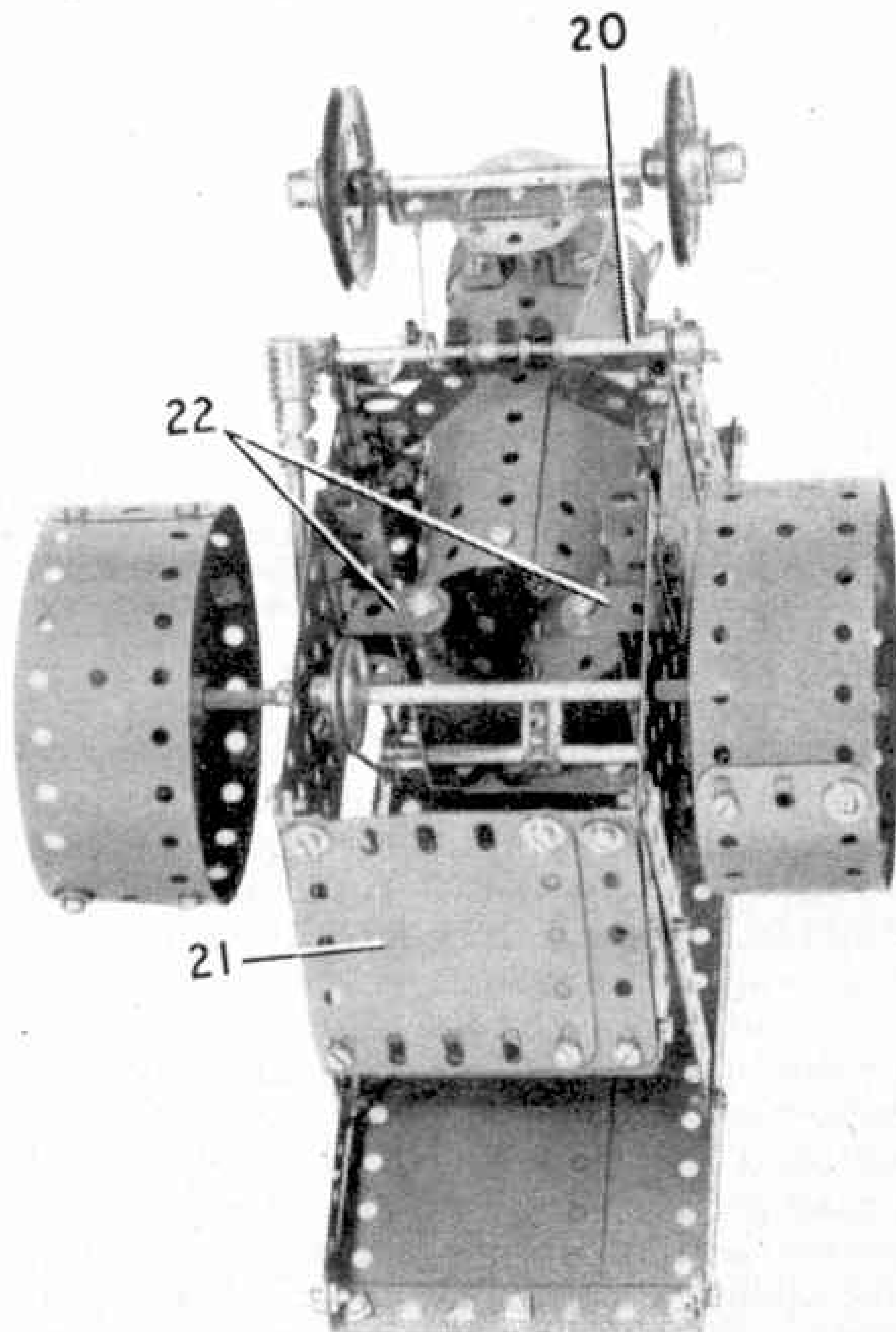
Fig. 3. An underneath view of the Traction Engine.
