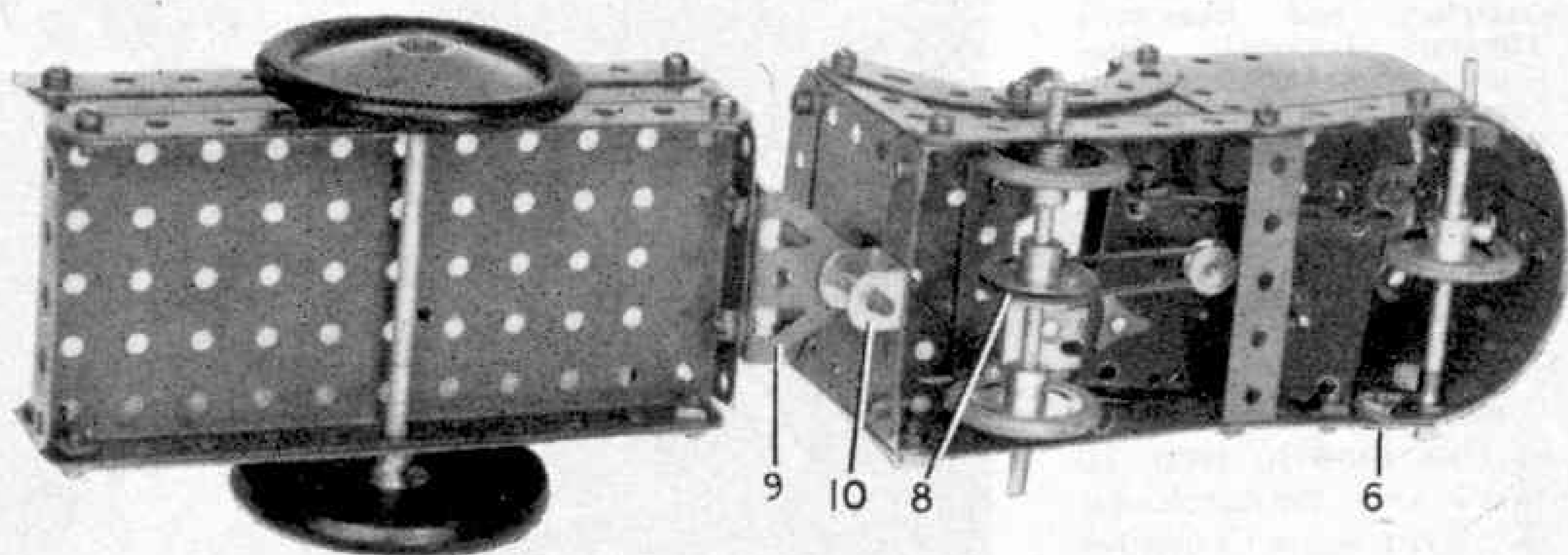
Fig. 3. The underside of the Towing Tractor and Trailer showing how the Magic Motor is fitted.
