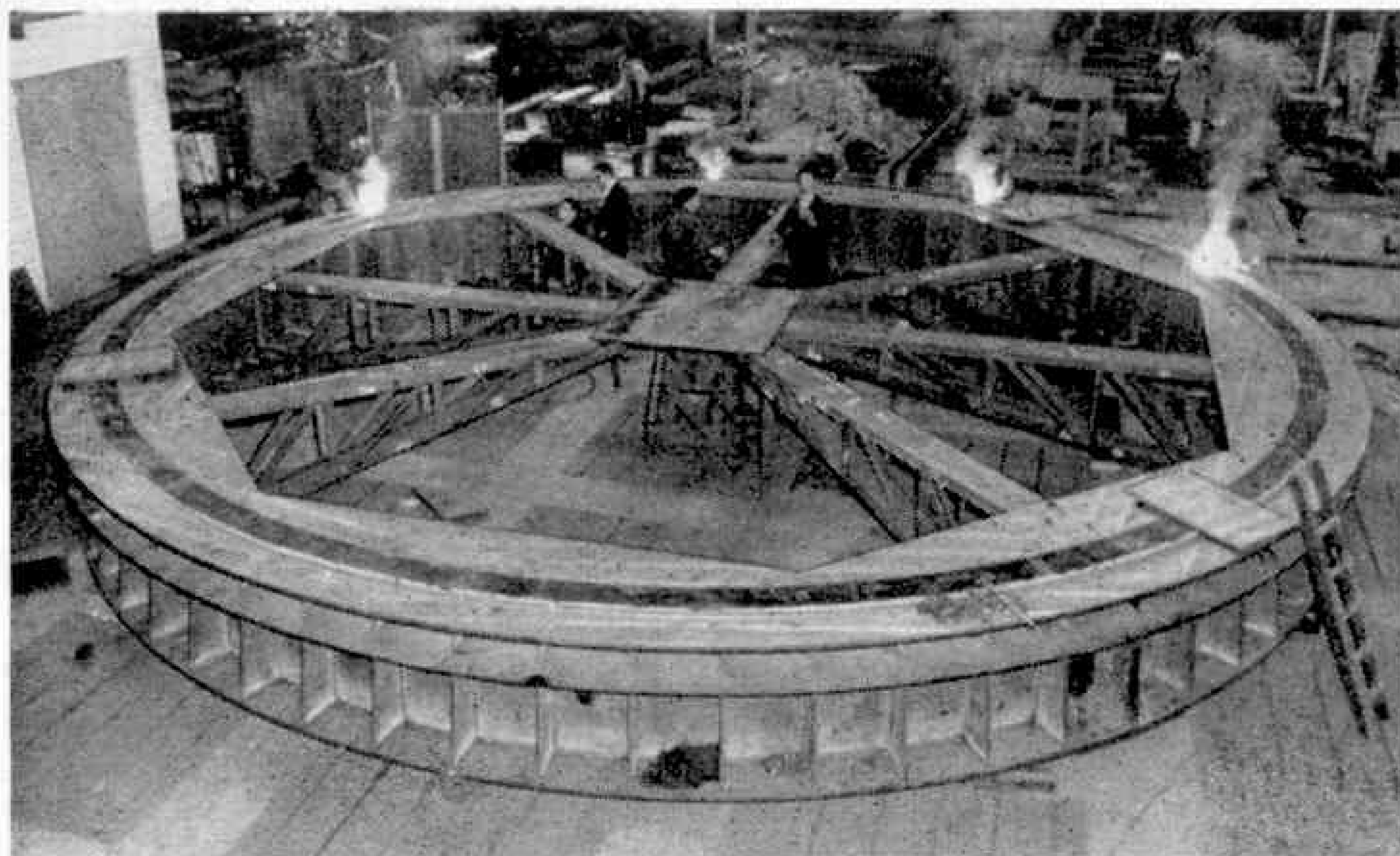
This welded circular girder photographed during assembly in the works of Stothert & Pitt, Ltd. is part of the new level-luffing crane installed at Falmouth.
