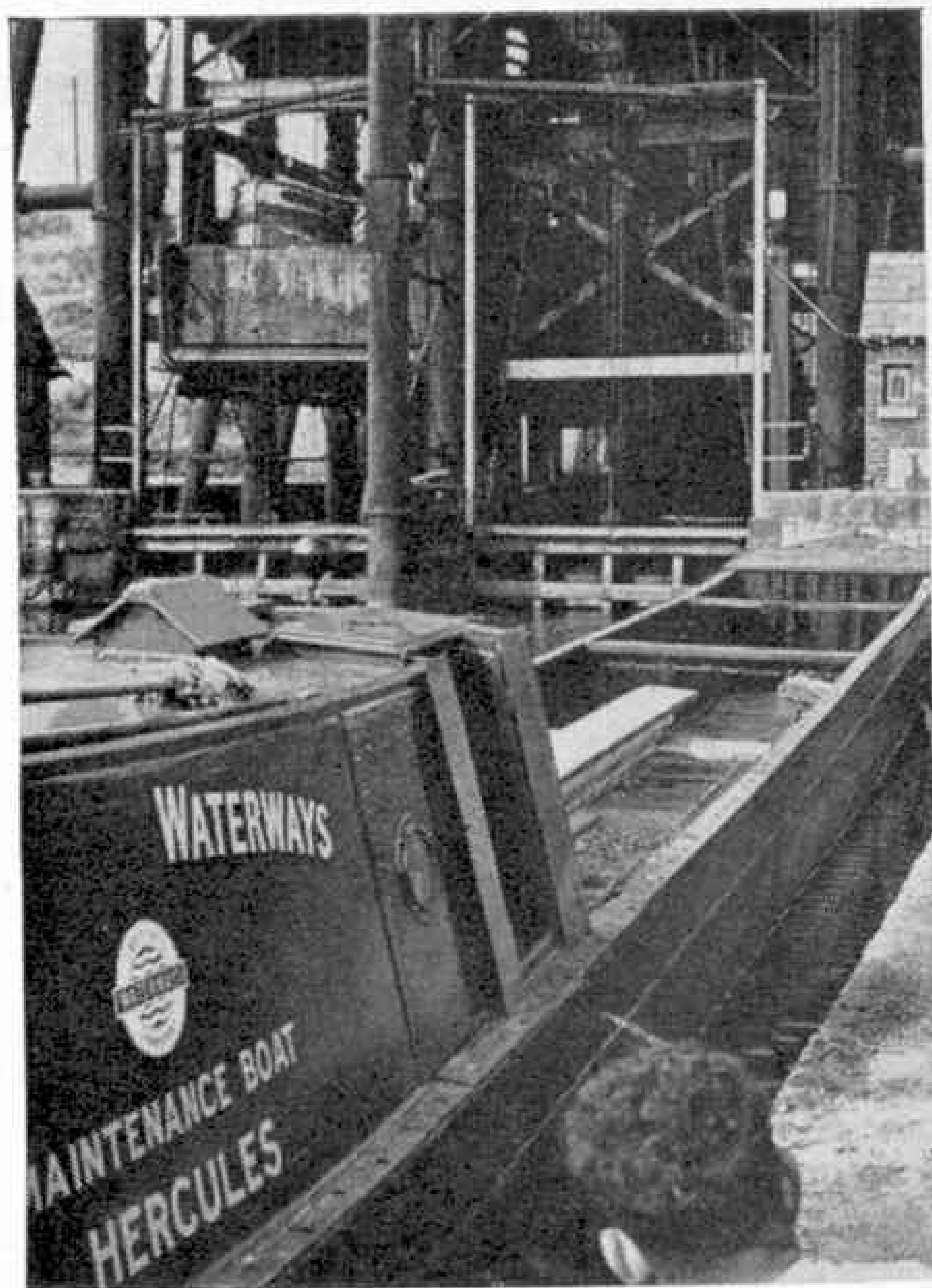
The barge Hercules waits to enter the boat lift at Anderton. When this picture was taken the right hand lift was not in action owing to maintenance work. Picture: N. Jones, Warrington.
