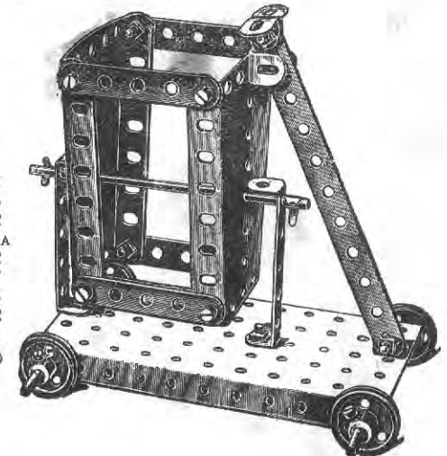
Model No. 51 Tip Wagon
