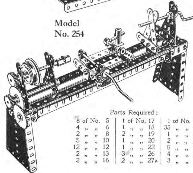
Screw- Cutting Lathe
