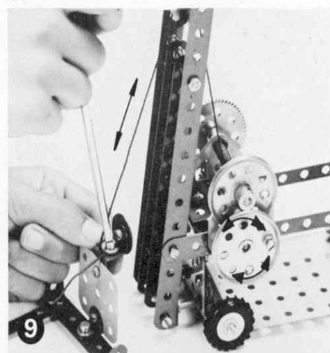
Forklift Truck Camion elevateur vorkhef-truck Gabelstaber Gaffeltruck Carretilla elevadora Carrello elevatore a forza
