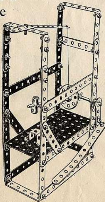
Treadle Hammer
