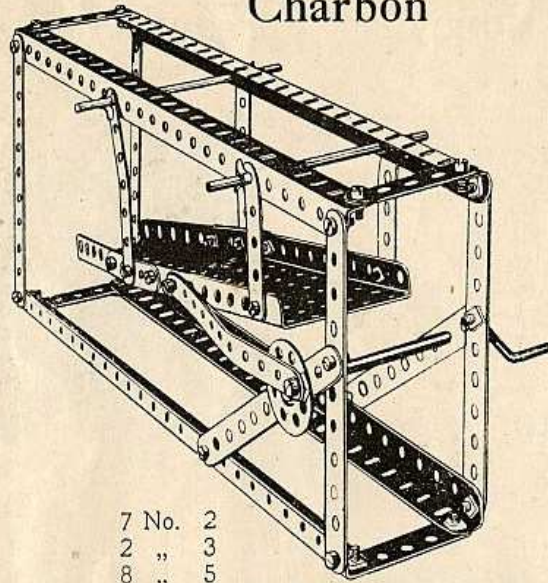
Coal Shaker
