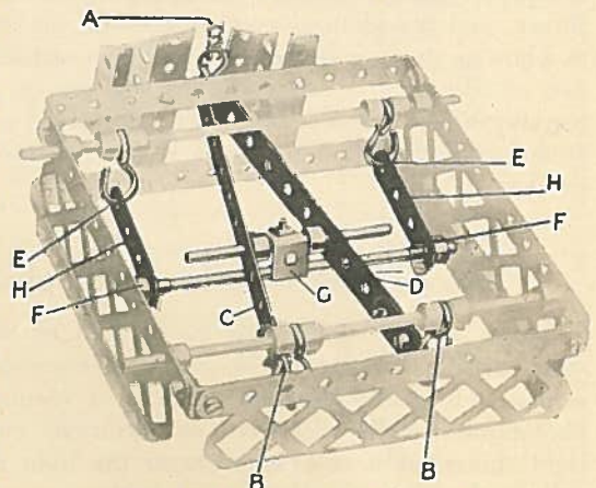
S.M. 51—Levers in platform scales.
